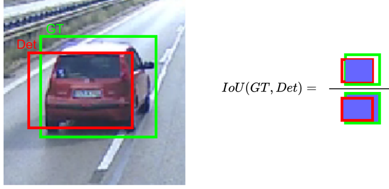
Figure 6.2: IoU for a 2D bounding box in image coordinates. Note, that these metric can also be applied to other types of shapes and volumes, like OBBs.
