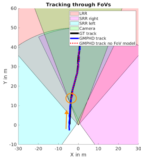
(a) Overtaking car moving in direction of the orange arrow crossing multiple sensor FoVs. A stable tracking without FoV model is reached at the overlap of all sensor FoVs.
