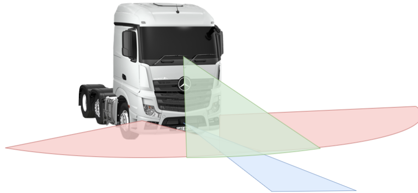
Figure 2.4: Example for truck sensor setup with SRR in red, LRR in blue and camera in green.
