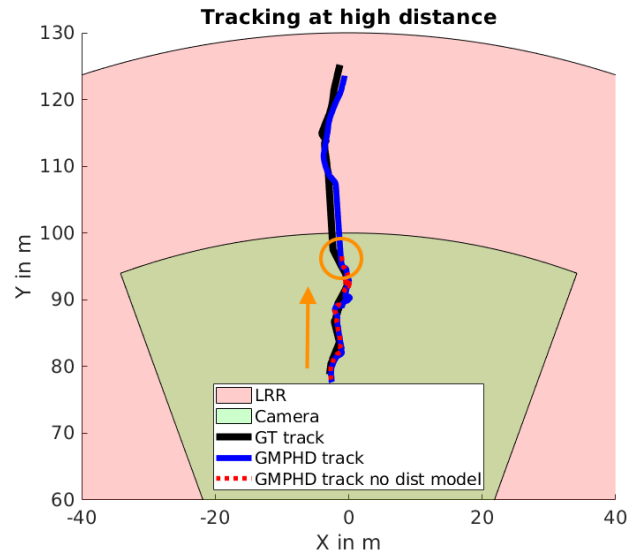
(b) Car moving away in the direction of the orange arrow at higher distance. The track is lost at orange circle without the distance model for the detection probability.
