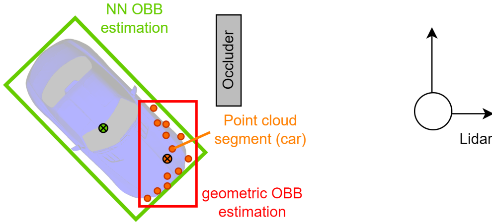
Figure 3.6: Point cloud segment of partially occluded car and example OBB estimations for NN and geometric approach. NN is able to estimate an OBB close to the GT, while geometric approaches are not.
