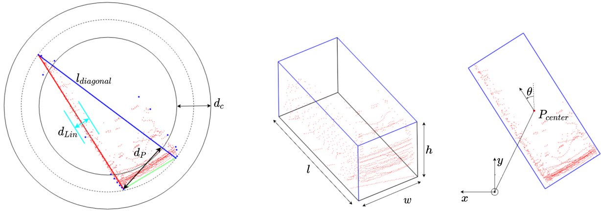
Figure 3.10: Calculation of the oriented bounding box. First, the three triangle lines are searched for. In this example, the diagonal line has a lower number of associated points, so the red line is chosen for orientation. Next, the length, width and height and position are calculated based on the orientation.
