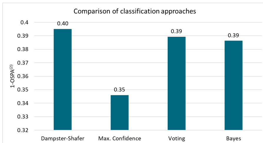
Figure 6.19: Comparison of different classification approaches on Fused Truck dataset with GM-PHD filter.
