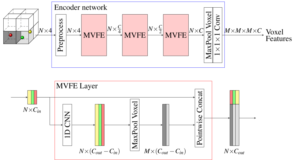
Figure 3.12: On top, the structure of the encoder network is shown, which consists of three MVFE layers and creates features for each voxel. The lower half shows the structure of the MVFE layer. In this visualization, an example with 3 points spread across two voxels is shown (Bader et al. 2021).
