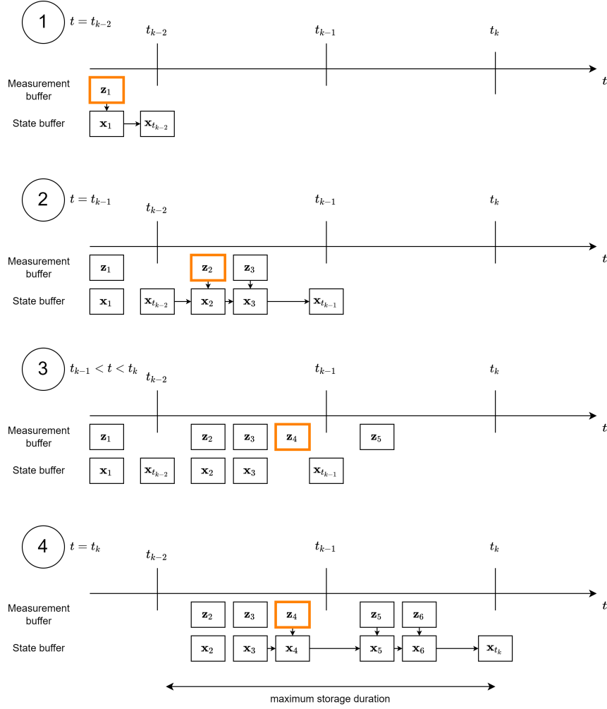
Figure 5.2: Scheme of the temporal management, that is responsible for the correct buffering.
