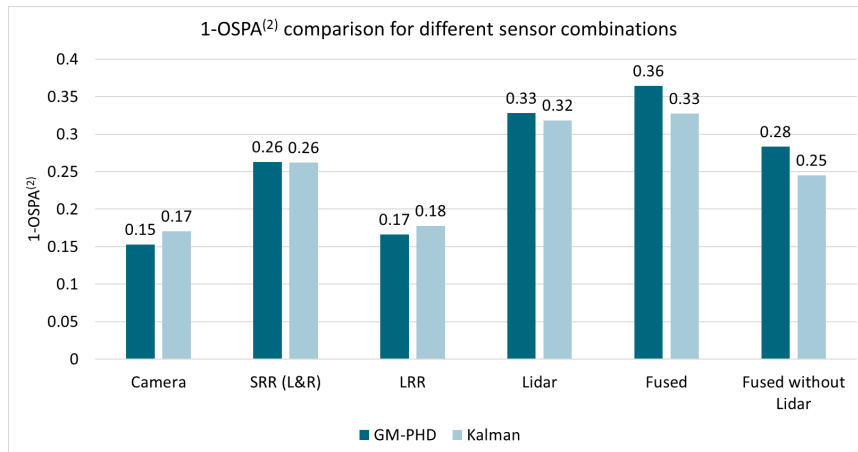
Figure 6.12: Comparison of GM-PHD and KF using the OSPA (2) metric on the truck dataset with different sensor combinations.
