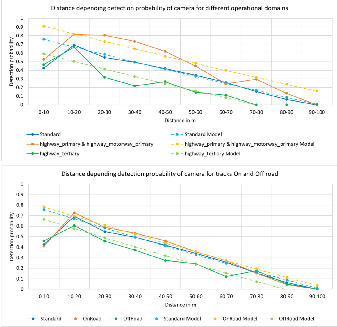
Figure 5.11: Models of detection probability for camera detector in different operational domains and tracks on/off the road for class "Car".
