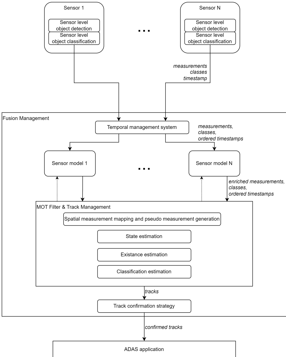
Figure 5.1: Overview of the proposed fusion framework. The top section shows the individual detection and classification of each sensor, while the blocks below show the tasks of fusion, which include estimation of states, existence and classification with inputs from multiple sensors over time.
