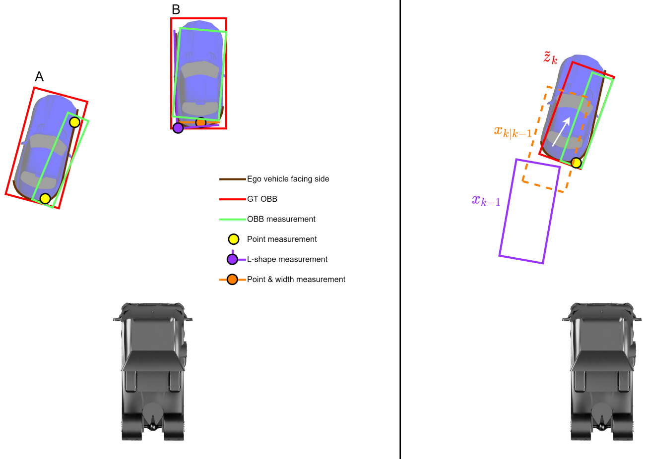
Figure 5.4: Examples of faulty measurements based on real-world targets (left). Example for pseudo measurement creation using point- and wrong sized OBB (right).
