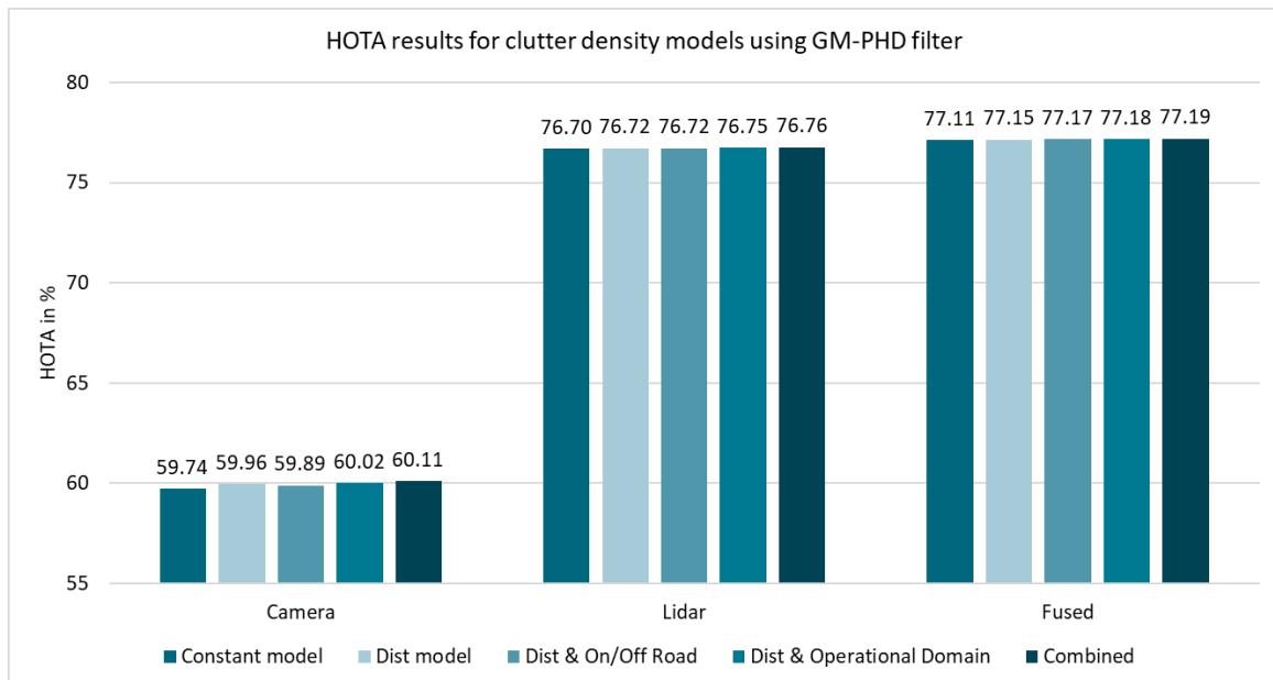
Figure 6.14: Comparison of clutter density model impact on HOTA results of the KITTI dataset.
