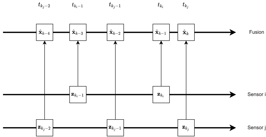
Figure 4.6: Scheme of direct update sensor fusion without delay. Multiple sensors update the states at different time stamps. This idealized system does not include delays between measurement and fusion.
