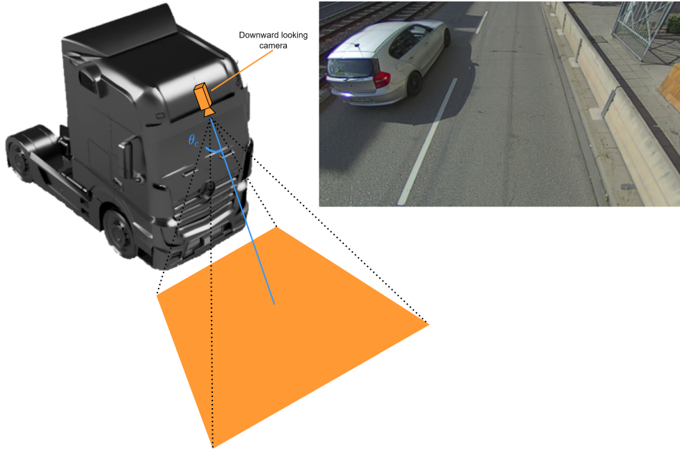
Figure 3.19: Front mirror replacement camera position and rectified example image.
