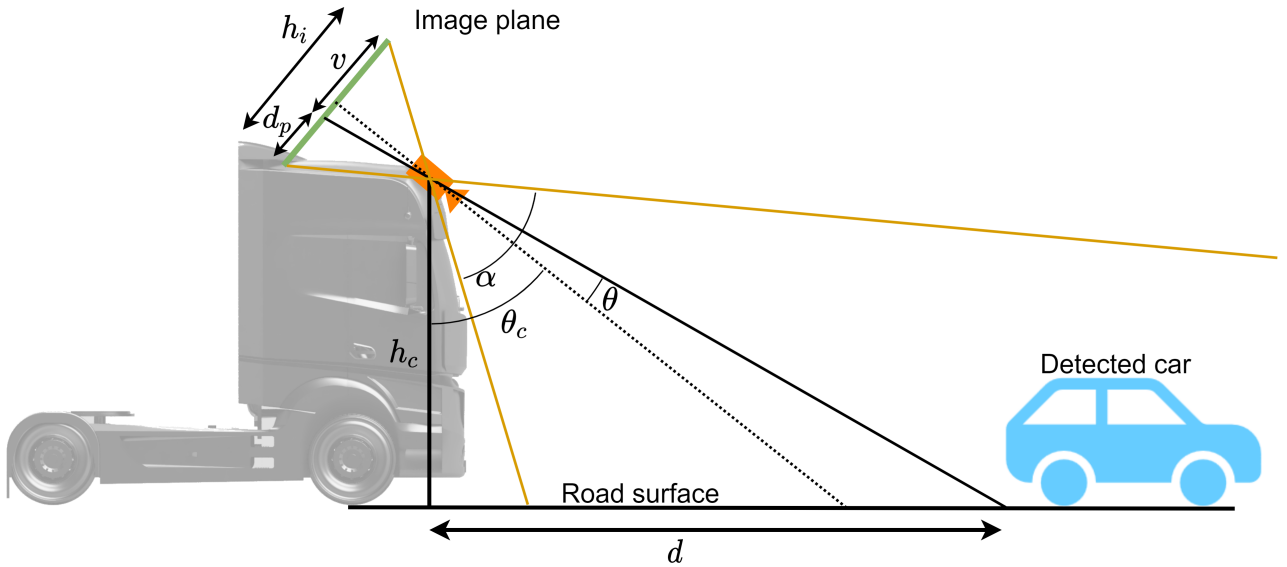
Figure 3.17: Distance estimation using the projection to the ground surface with a camera mounted to the truck cabin. Based on figure from Rezaei et al. (2015), but applied to truck.
