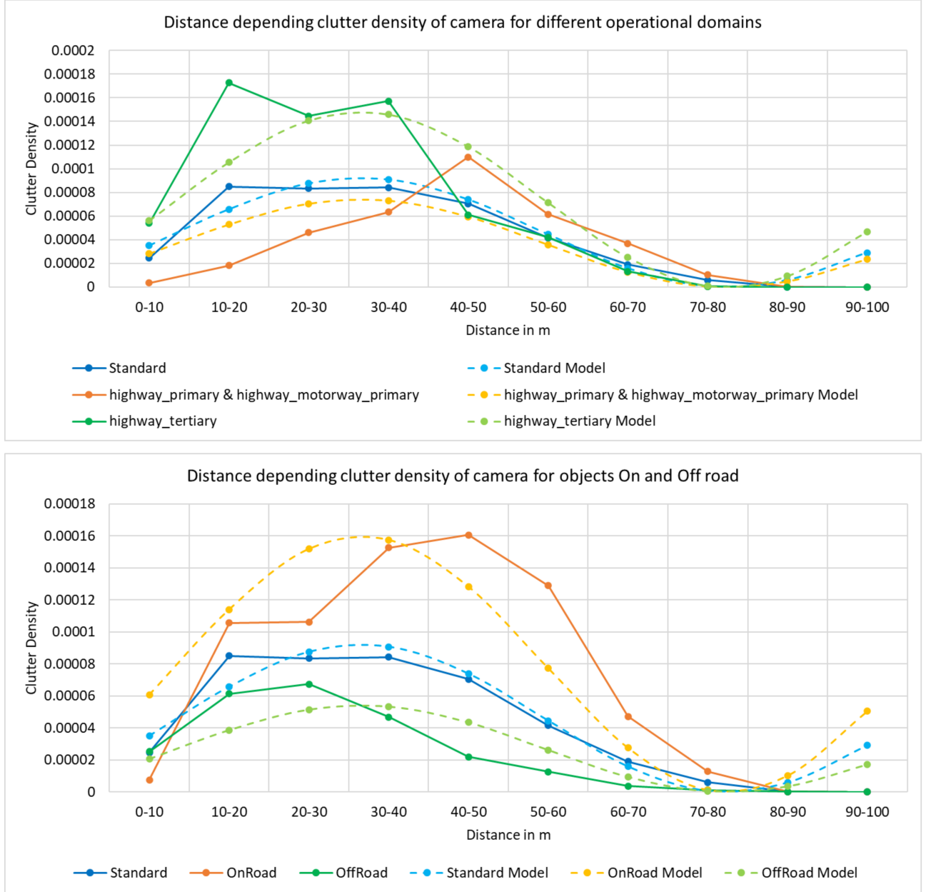
Figure 5.14: Models of clutter density for camera detector in different operational domains and tracks on/off the road for class "Car".
