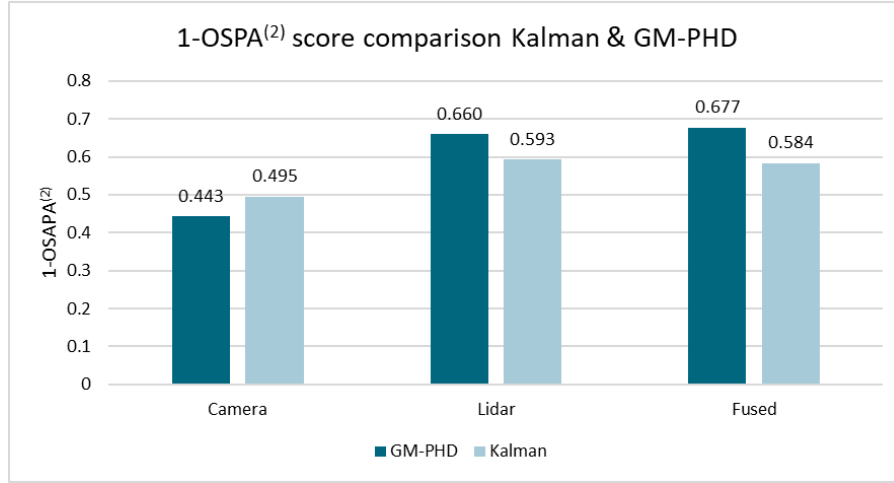
Figure 6.11: Comparison of GM-PHD and KF using the mean OSPA (2) score on the KITTI dataset. Displayed as 1-OSPA (2) for visual comparison to HOTA.
