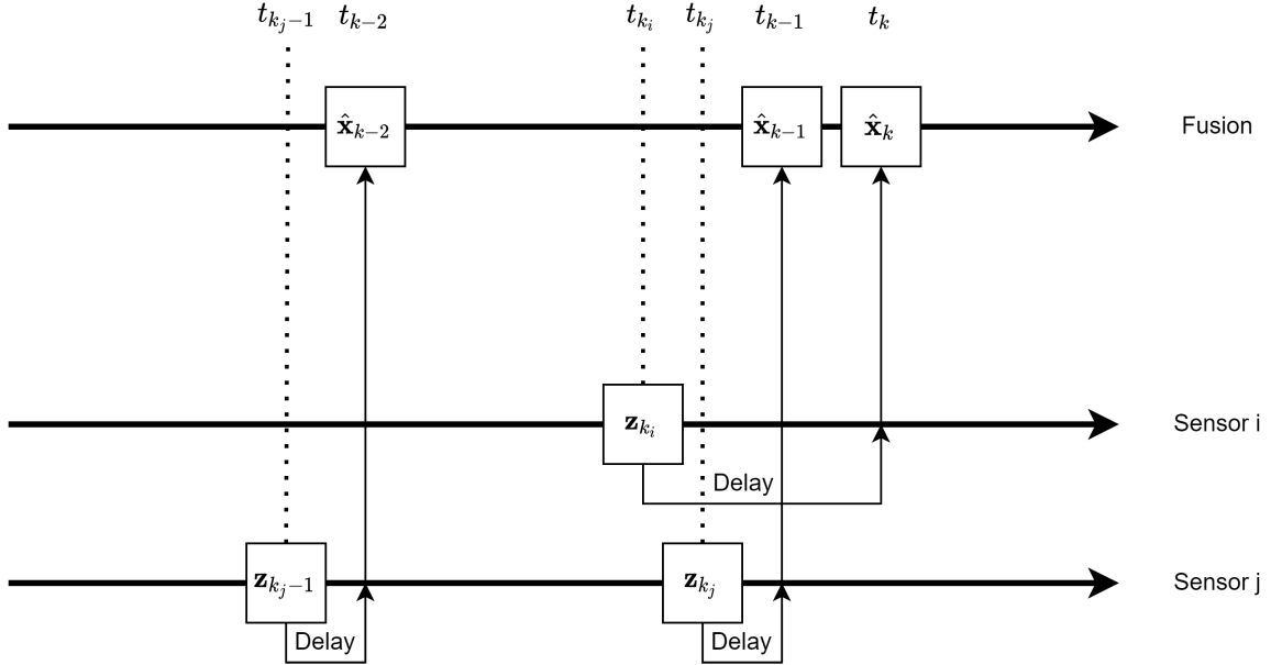
Figure 4.7: Scheme of sensor fusion with different sensor delays. Two sensors i and j with different delays result in the out-of-sequence measurement \mathbf{z}_{k_i} .
