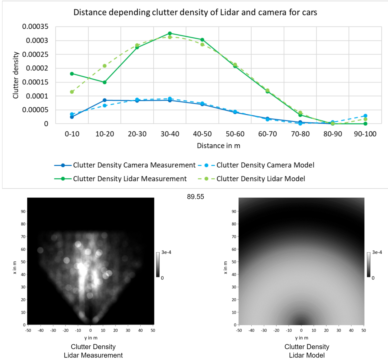
Figure 5.13: Clutter density distance model for class "Car". On top, the models of camera and Lidar with respect to the distance are shown, on bottom the Lidar measurement and model are shown in BEV.
