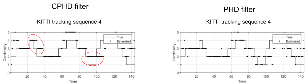
Figure 6.6: Comparison of cardinality estimation of GM-CPHD and GM-PHD filter on KITTI dataset sequence 4. Situations of the GM-CPHD filter reacting slowly to changes are marked in red.
