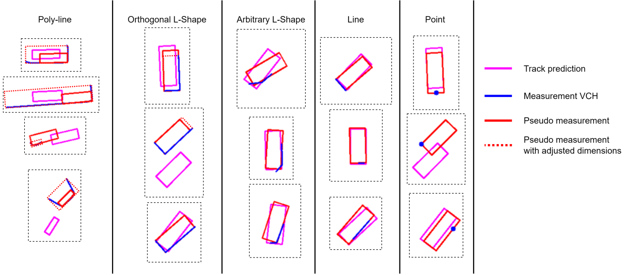
Figure 5.6: Mappings of proposed pseudo measurement generation approach using different input data formats.
