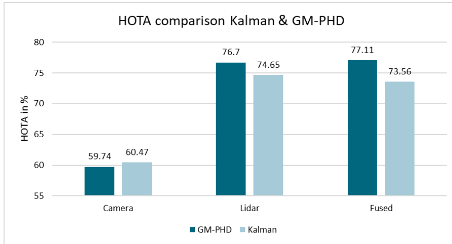
Figure 6.9: Comparison of GM-PHD and KF using HOTA metric on the KITTI dataset.
