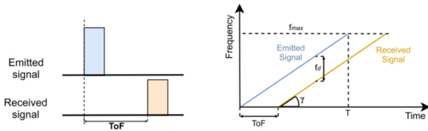
Figure 2.7: Examples of different measurement types of Lidar sensors by showing the emitted and received signals of ToF (left side) and FMCW (right side) Lidar sensors. For FMCW, the emitted and received frequency is shown which is used to calculate the target's velocity, composed from (Roriz et al. 2021).
