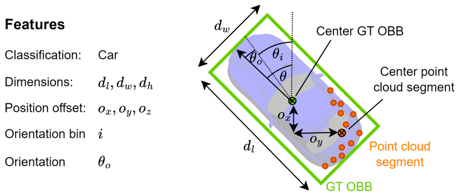
Figure 3.15: Features calculated by each branch visualized.
