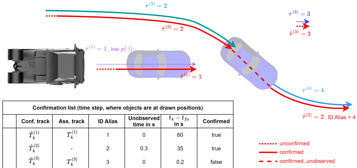
Figure 5.15: Example situation with track confirmation strategy. The trajectories of the confirmation list are drawn in red, while the trajectories of the track set have different colors. The confirmation list table shows example values at the time where the objects are at the cars positions.
