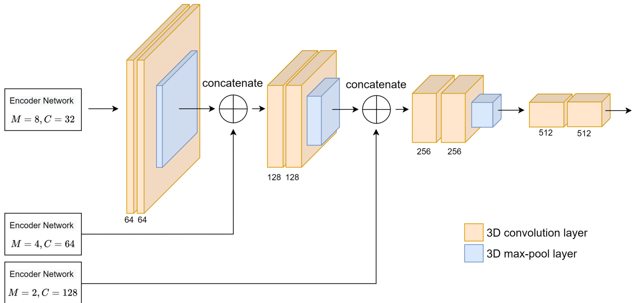
Figure 3.13: Backbone of NN consisting mainly of convolutional and max-pool layers. For simplicity, the 3-dimensional grid is reduced to 2D in the Figure. The number of feature channels is described below each convolutional layer.
