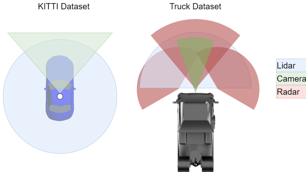
Figure 6.1: Comparison of the sensor setups and FoV of the KITTI and the truck dataset.
