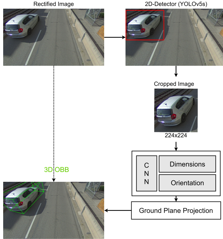
Figure 3.21: Scheme of 3D OBB generation approach: 2D bounding box detection, cropping and rescaling, CNN-based orientation and dimension estimation, geometric road surface projection.
