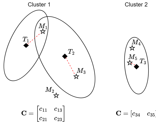
Figure 4.3: Example of data association and gating with two clusters, 3 tracks T and 5 measurements M . In the example, two clusters are generated. The first cluster contains T_1 , T_2 , M_1 and M_3 , while the second cluster contains T_3 , M_4 and M_5 . M_2 is not located in either cluster and therefore cannot be assigned to any track. The result of the association is indicated by red dotted lines.
