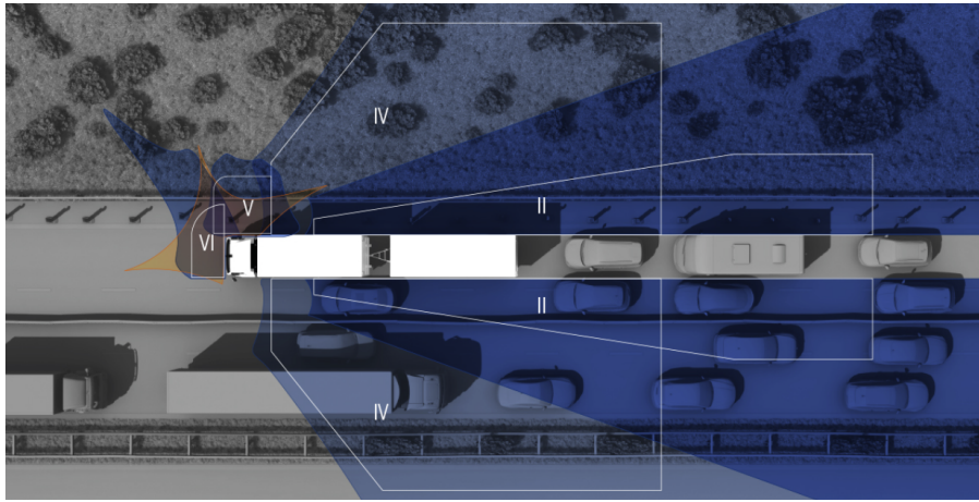
Figure 3.18: FoV areas of mirror classes for trucks following UN ECE R46/04 (UNECE 2014) projected on ground level (MEKRA Lang GmbH & Co. KG 2023).
