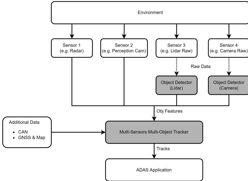
Figure 2.1: General pipeline used for this thesis. The environment is captured by sensors, which either directly process the data to object features or provide their raw output (e.g. image or point cloud) to detection algorithms. Next, the tracking and fusion is performed. Dark gray modules are developed in this thesis.
