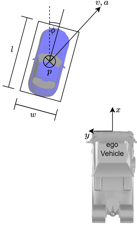
Figure 5.3: Visualization of ego vehicle and one tracked object, all states except h are visualized. Note, that \phi and \Psi do not necessarily need to align.
