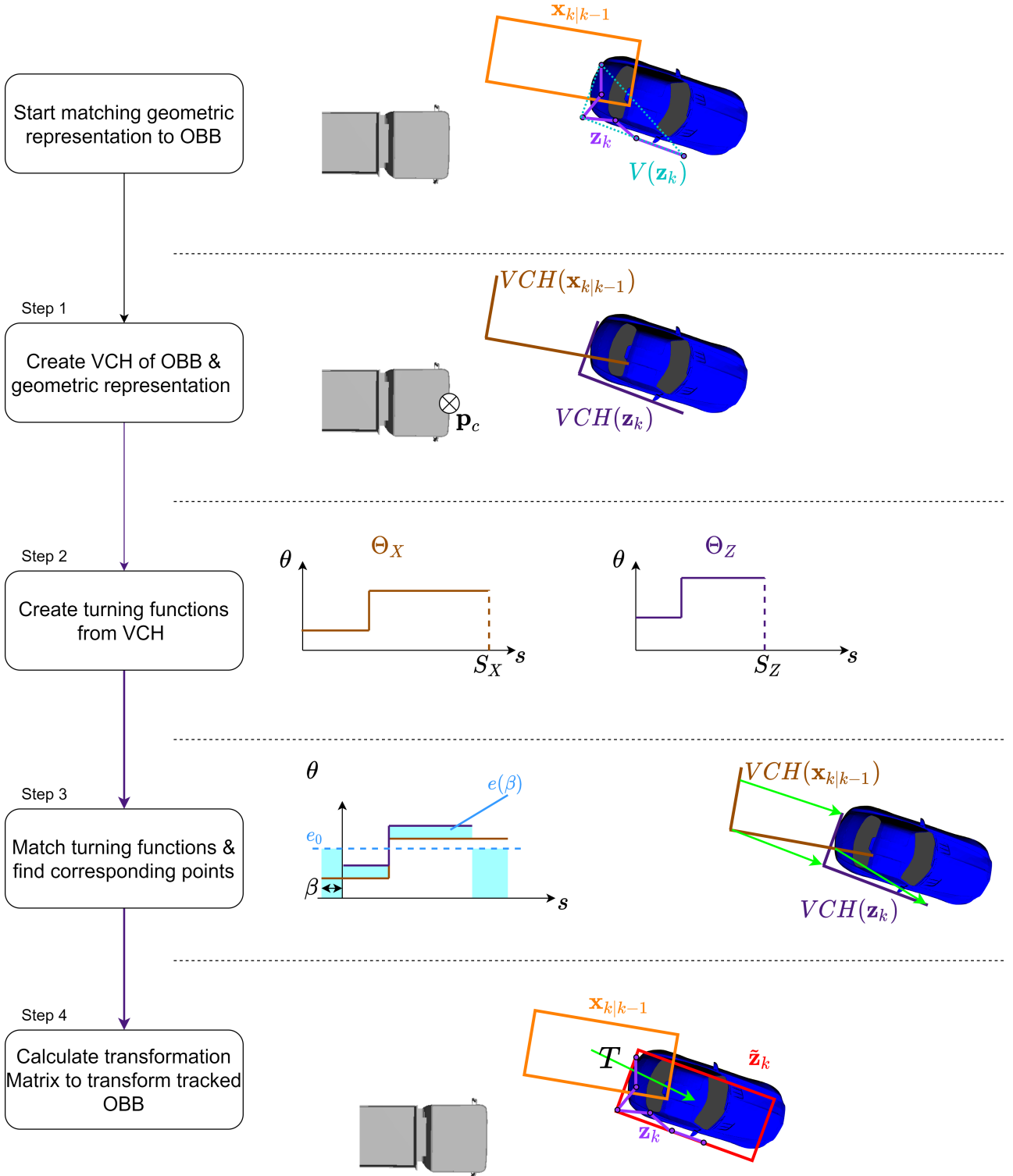
Figure 5.5: Schematic illustration of all steps to generate OBB pseudo measurements from geometric formats. Exemplary done with polyline geometry.
