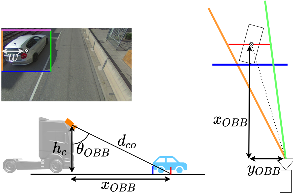
Figure 3.22: The center of the bounding box is fitted to the center of the left (orange) and right (green) 2D bounding box borders. The closest point is fitted to the distance line (blue), which in combination defines the X- and Y-Position of the 3D OBB in vehicle coordinates
