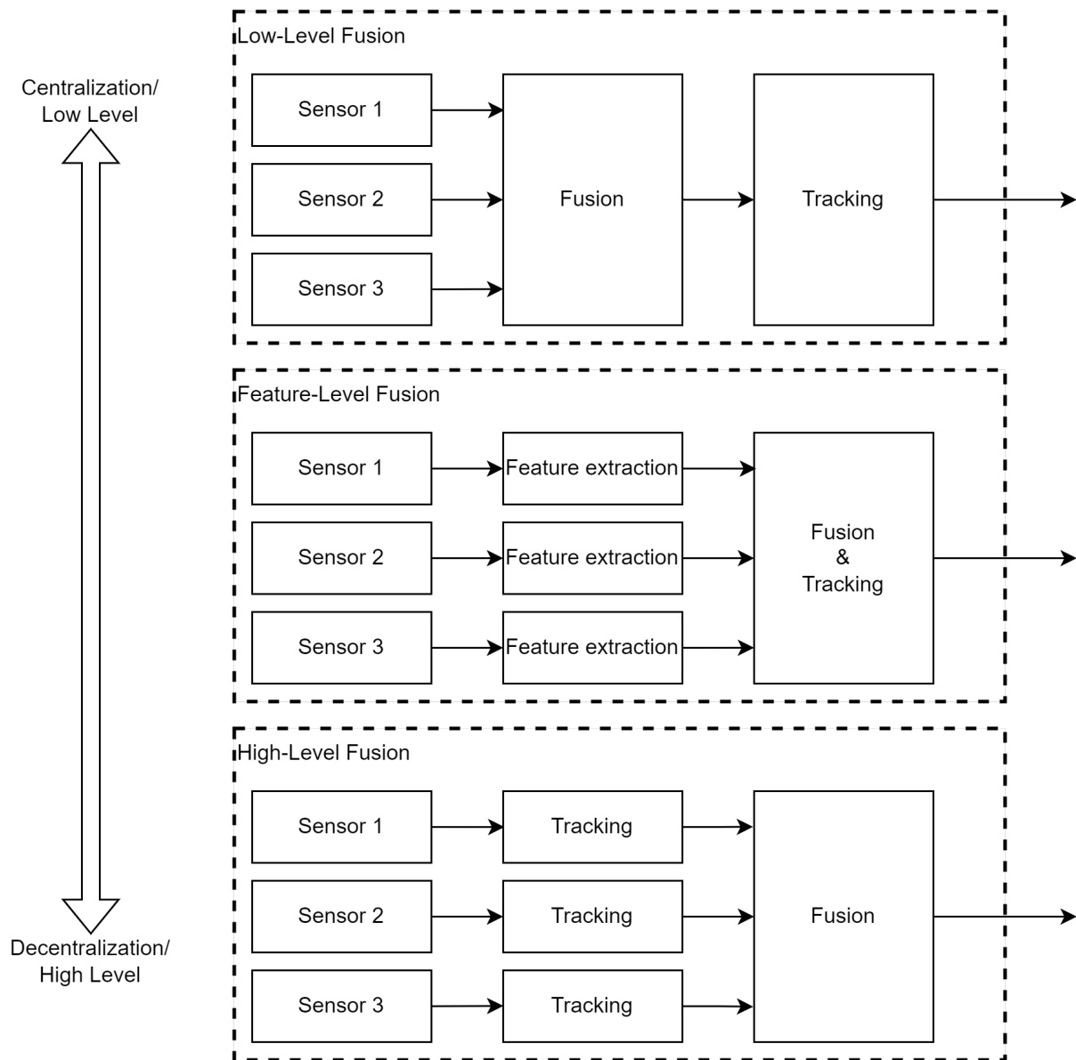
Figure 4.5: Scheme of high-level, feature-level and low-level fusion concepts.
