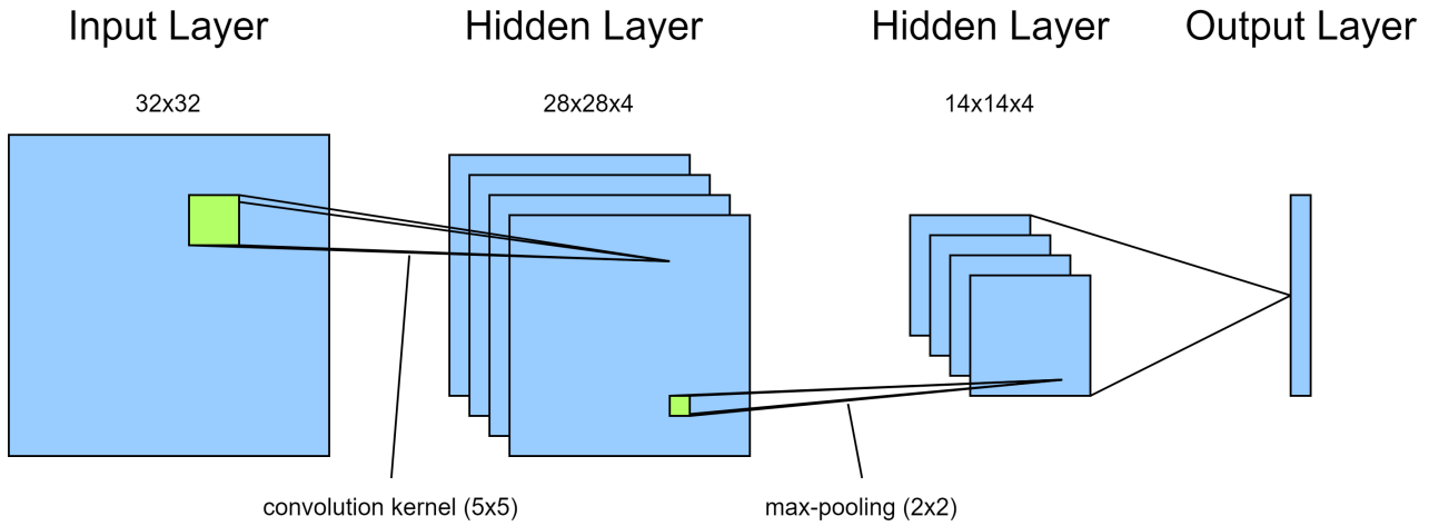
Figure 3.4: Example for CNN with one hidden convolutional layer and one hidden max-pooling layer.
