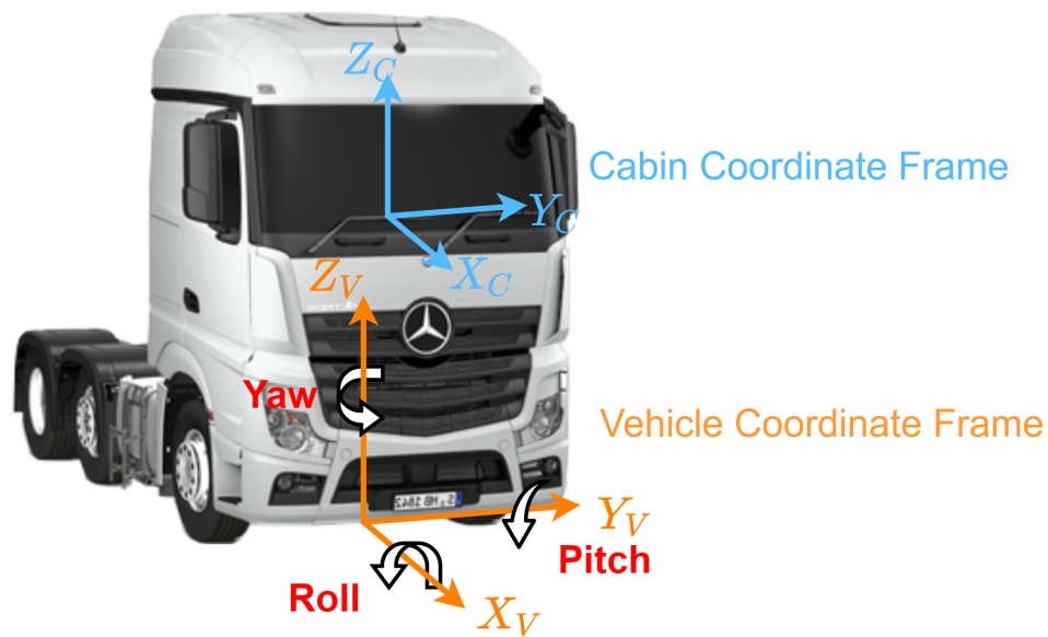
Figure 2.10: Vehicle and cabin coordinate system definition.
