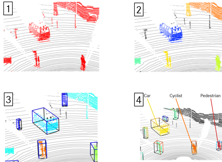
Figure 3.5: Four steps of a traditional Lidar object detection pipeline: 1. ground extraction, 2. object segmentation, 3. OBB generation, 4. classification of objects.
