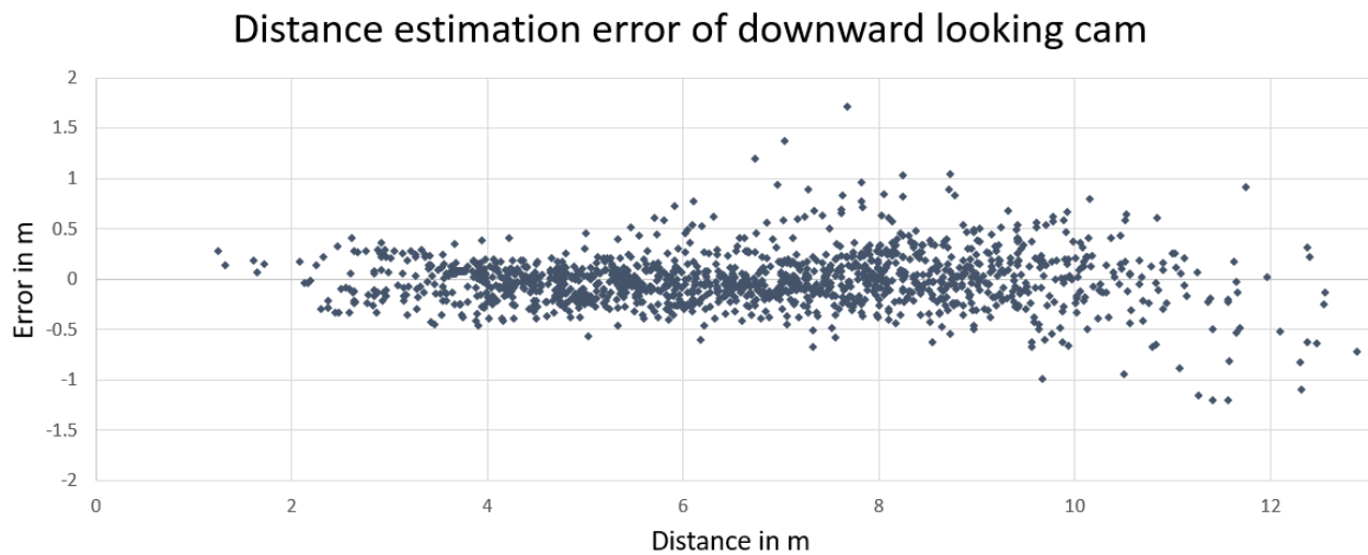
Figure 6.4: Distance error of camera detections to GT from Lidar over the object distance.
