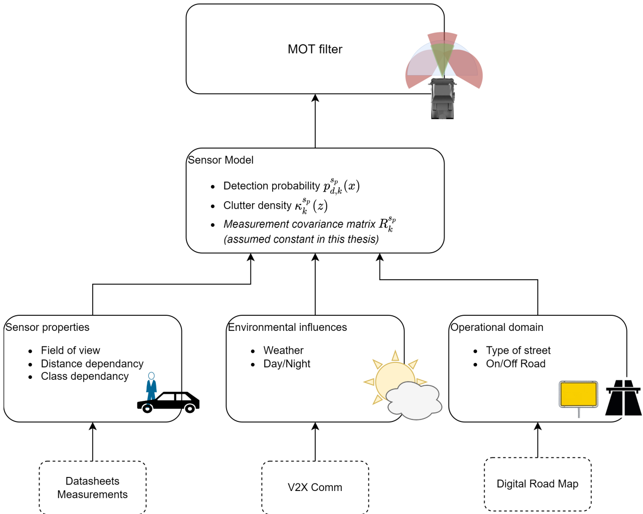
Figure 5.7: Examples of influences on the measurement model and data sources for information on influences.
