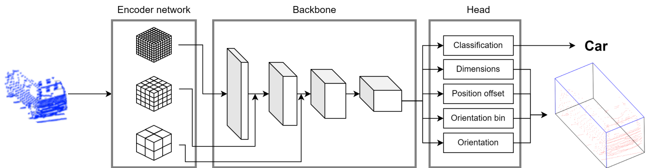
Figure 3.11: Architecture of network, which consists of an encoder network, a backbone and a several heads to output the classification and OBB regression.
