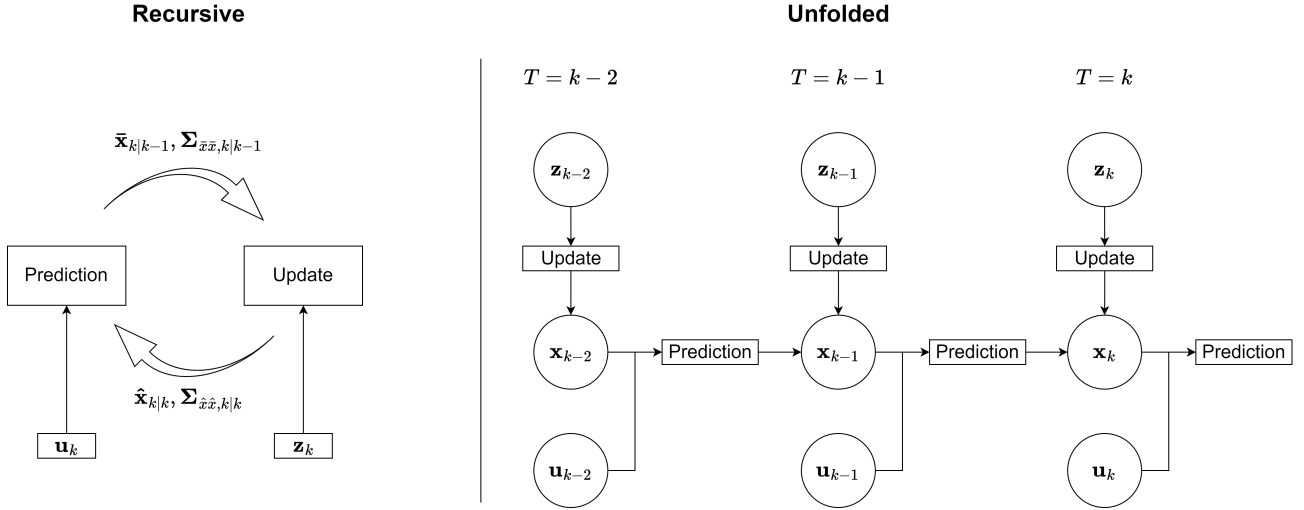
Figure 4.1: Scheme of Kalman filter calculation steps. Shown recursive on the left side and unfolded on the right side.
