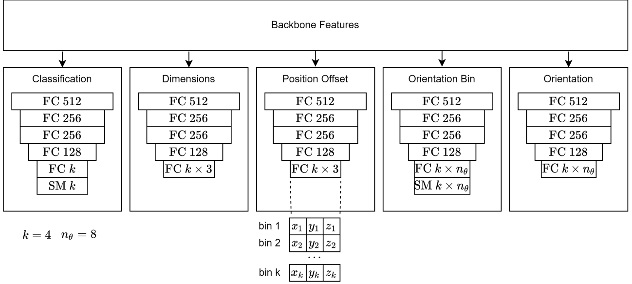
Figure 3.14: Architecture of head with multiple branches. Inside of each branch, the layers are described by the number of fully connected (FC) neurons. For classification and orientation bin branch, a softmax (SM) layer is added. The outputs of all branches except classification consist of k bins, where k is the number of classes. For the position offset branch, the structure of the bins in the output layer is shown.
