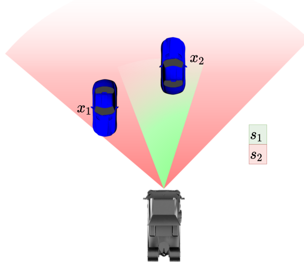
Figure 5.8: Example of two sensors s_1 and s_2 covering different FoVs and two tracked objects.
