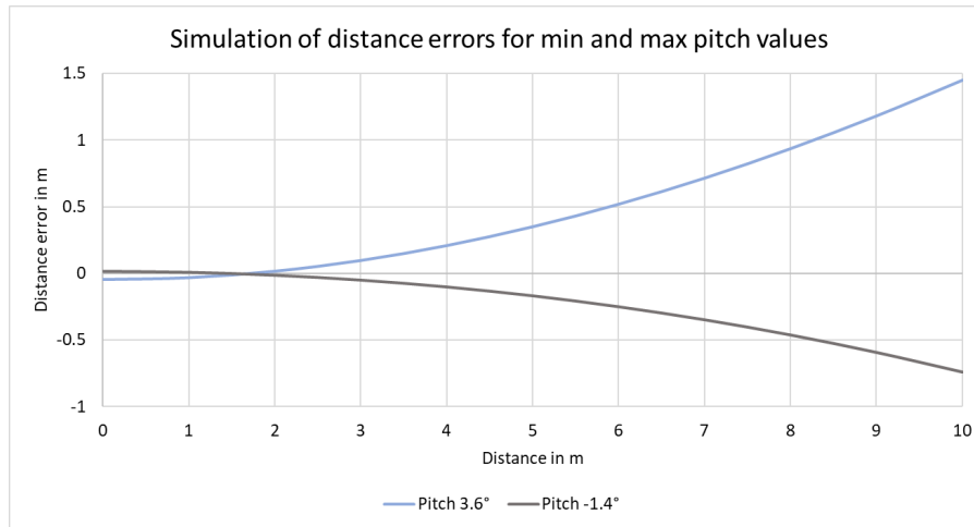
Figure 3.20: Simulation of distance estimation error using minimum and maximum pitch angle at height of h_c = 3.5 m.
