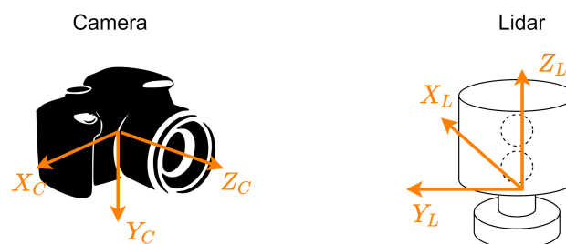
Figure 2.11: Sensor coordinate system examples for Camera and Lidar.
