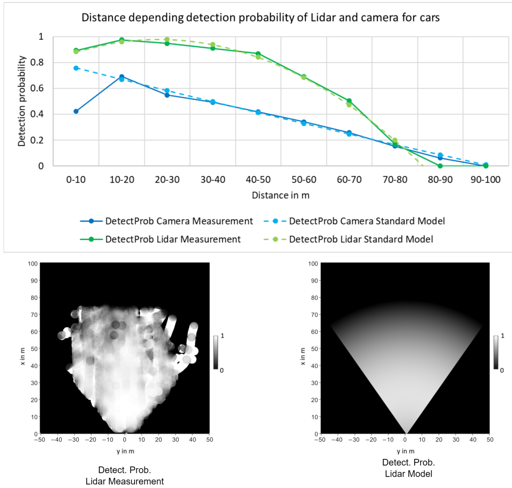
Figure 5.10: Detection probability distance model for class "Car". On top, detection probability models of camera and Lidar with respect to the distance is shown, on bottom the detection probability measurements and model are shown in BEV.
