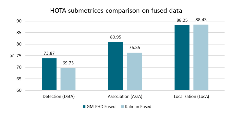
Figure 6.10: Comparison of GM-PHD and KF using the HOTA submetrics on the KITTI dataset for deeper insight.
