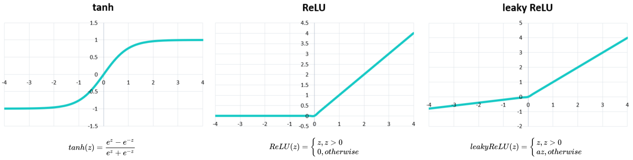
Figure 3.2: Visualization of tanh, ReLU and leaky ReLU activation functions with formulas. a for leaky ReLU is a constant factor.
