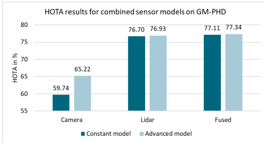
Figure 6.15: Influence of combined parameter models on HOTA results of the KITTI dataset.
