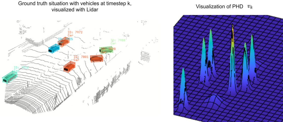
Figure 4.4: Intuition of GM-PHD filter shown by visualization of intensity on right side based on situation on left side. The visualization is an example to gain intuition and does not focus on accuracy.
