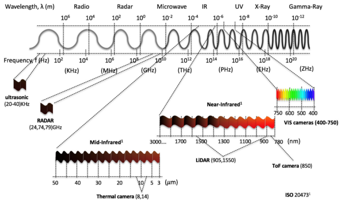
Figure 2.5: Magnetic spectrum including the ranges of different sensing principles, like camera, Lidar and radar (Rosique et al. 2019).
