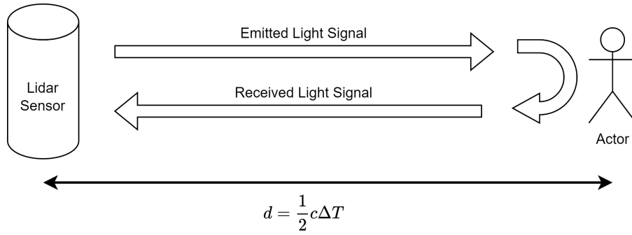
Figure 2.6: Basic working principle of a Lidar sensor. c is the speed of light in air, \Delta T is the ToF of the light signal.
