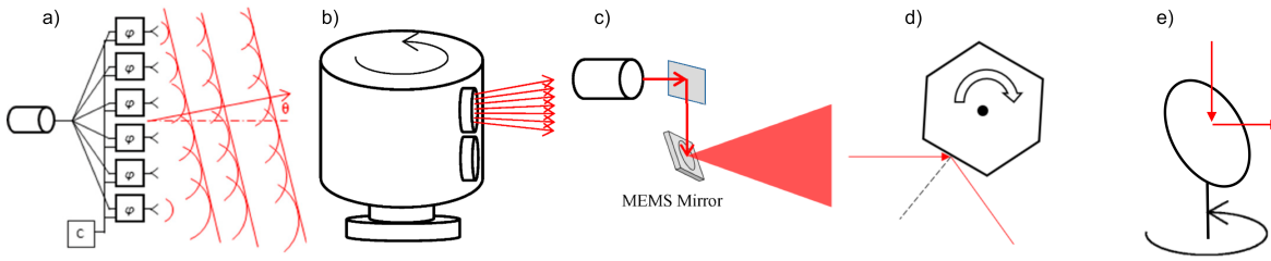
Figure 2.8: Comparison of different Lidar scanning principles: a) Optical Phase Array, b) rotating sensor platform, c) MEMS Mirror beam steering, d) rotating polygon mirror, e) rotating flat mirror. The principles shown in a) and c) are considered solid state, composed from Raj et al. (2020) and Wang et al. (2020).
