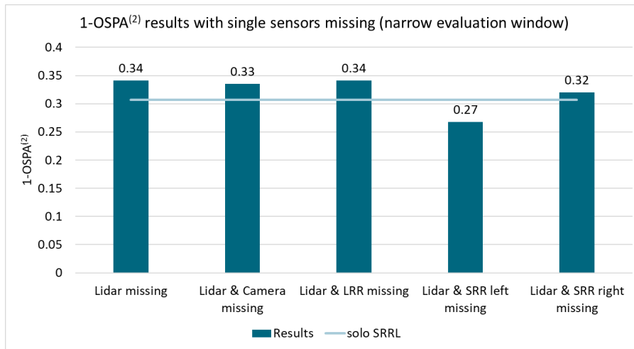
Figure 6.17: Sensor failure analysis with different sensors missing, using the narrow evaluation window on the truck dataset.
