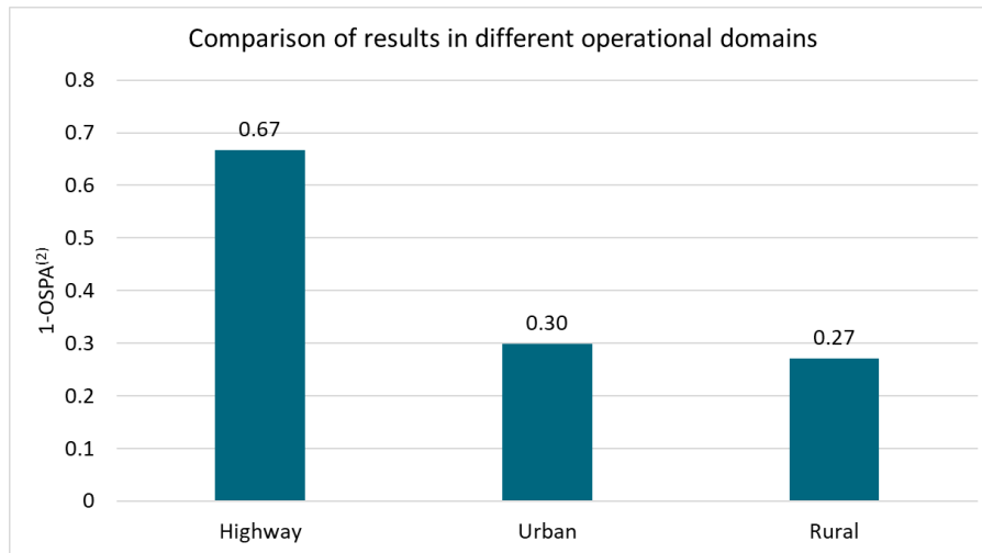
Figure 6.18: Comparison of OSPA^{(2)} results in different ODDs of the truck dataset.
