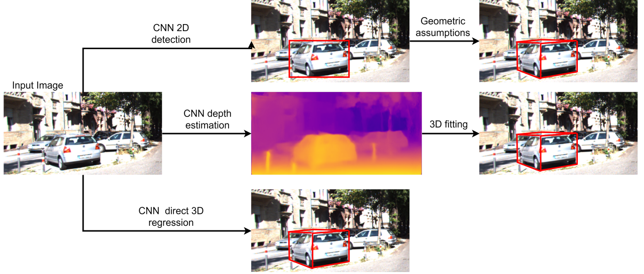
Figure 3.16: Visualization of different groups of monocular 3D camera detection. On top, multi-stage approaches, in the middle depth estimation approaches and on bottom direct 3D regression approaches are shown. The actual implementation may vary from approach to approach.
