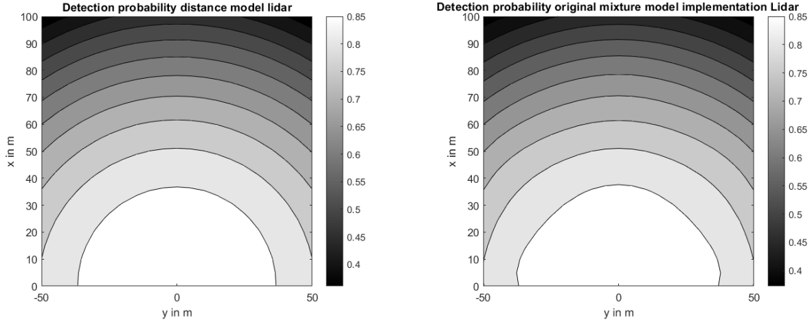
Figure 5.12: Comparison of detection probability model p_{Dm,k}^{sp}(\mathbf{x}_k) (left) and the mixture approximation p_{De,k}(\mathbf{x}) using 7 Gaussian components (right).
