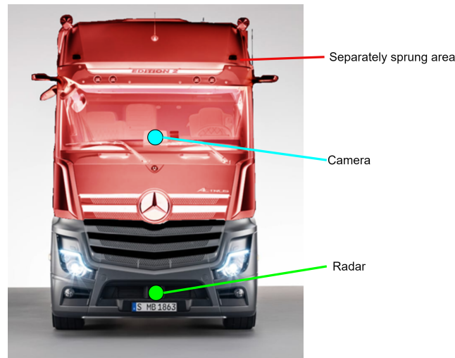
Figure 1.2: Red area marks separately sprung cabin are with camera sensor mounted behind windshield. The radar is mounted on the chassis.
