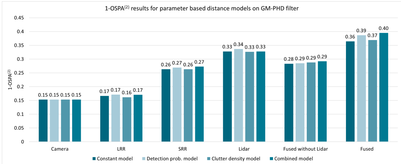
Figure 6.16: Influence of distance-dependent detection probability model on the truck dataset.
