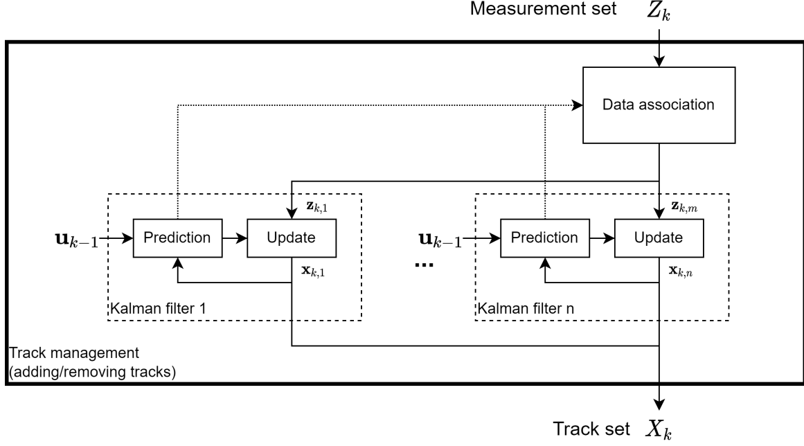
Figure 4.2: Scheme of a KF in an MOT framework including track management and data association.
