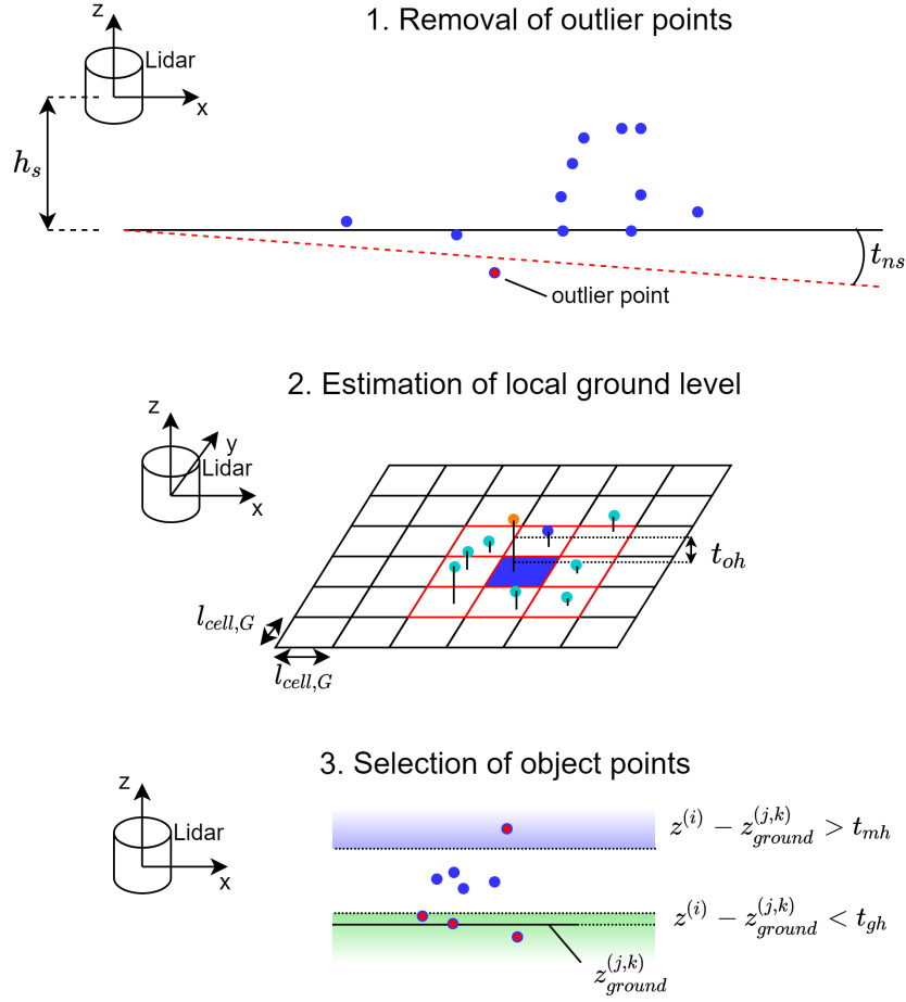
Figure 3.8: Scheme of ground extraction process in three steps. The first step shows the outlier removal based on a negative slope between an assumed flat ground plane and each point. The second step shows the estimation of the local ground height. The point with the lowest z -value of each cell is sketched. The dark blue-marked point has the median z -value, while the orange marked point is from the currently evaluated cell, which is outside the object height threshold t_{oh} . The third step shows the selection of the object points within one cell, where all points in the green area are ground points and all points in the blue area are out of reach.
