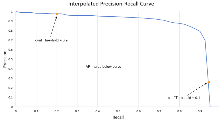
Figure 6.3: Exemplary interpolated precision-recall curve showing the tradeoff between both values. The area below the curve is the AP and is calculated by numerically integrating the curve.
