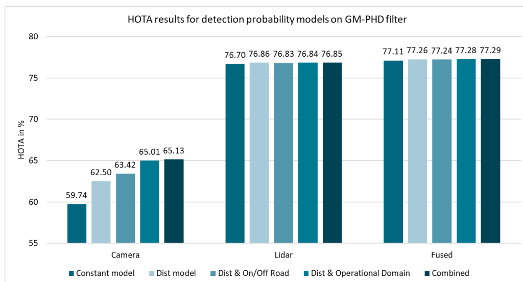
Figure 6.13: Comparison of detection probability model impact on HOTA results of the KITTI dataset.
