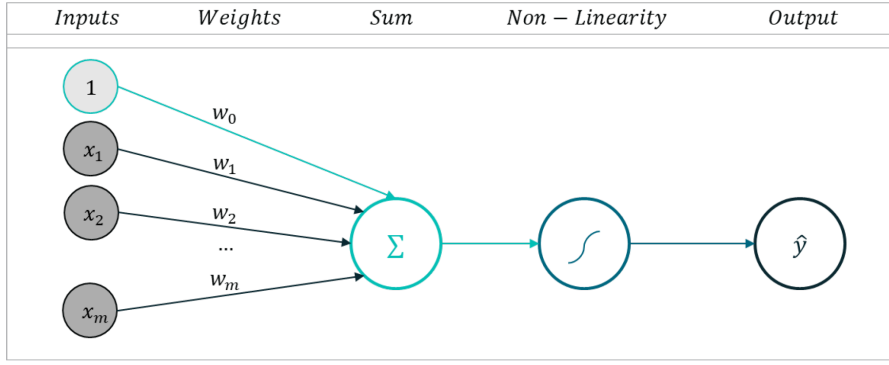
Figure 3.1: Schematic representation of a perceptron (Holz 2023).
