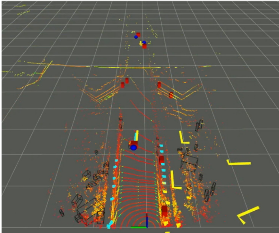
Figure 3.23: Example of radar detections from various radar sensors and a Lidar point cloud in a highway scenario. Radar detections shown in yellow, turquoise, red and blue are available as point, box or L-shape objects.
