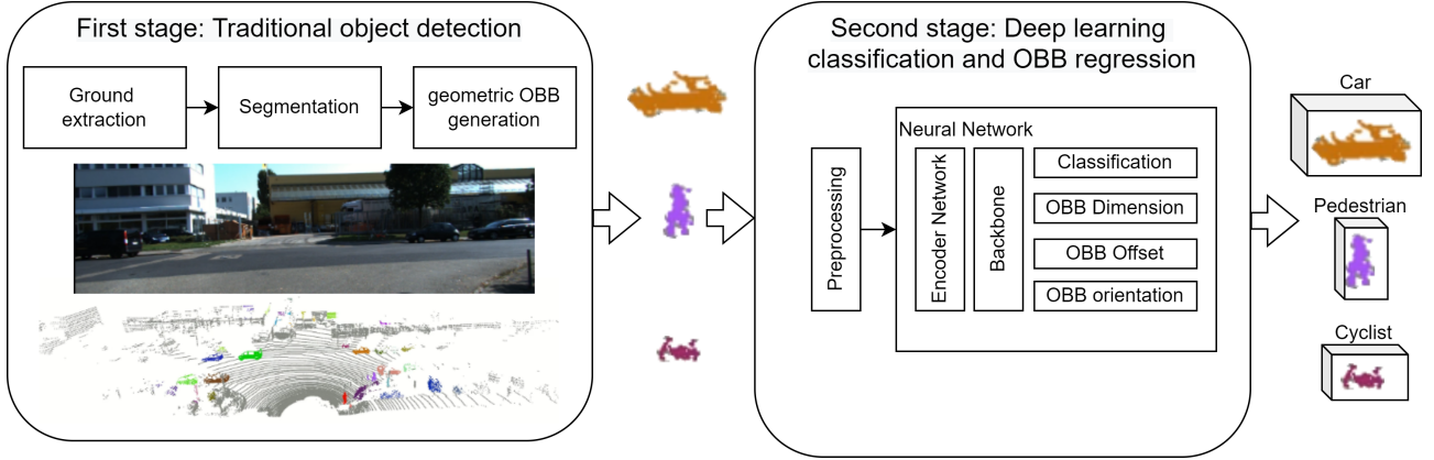
Figure 3.7: Overview of two-stage Lidar detection approach. The first stage consists of ground extraction, segmentation and geometric OBB generation. The point cloud segments are then passed to the second stage, which consists of a preprocessing and a neural network to estimate the class and OBB properties.
