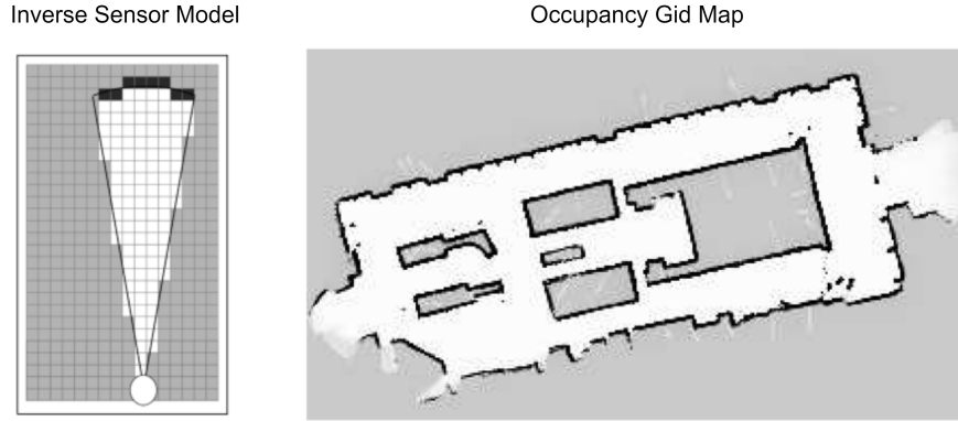
Figure 2.2: Example of occupancy grid and inverse sensor model (Thrun et al. 2005).
