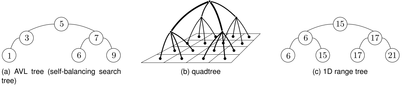
Figure 3.1: Tree data structures.
