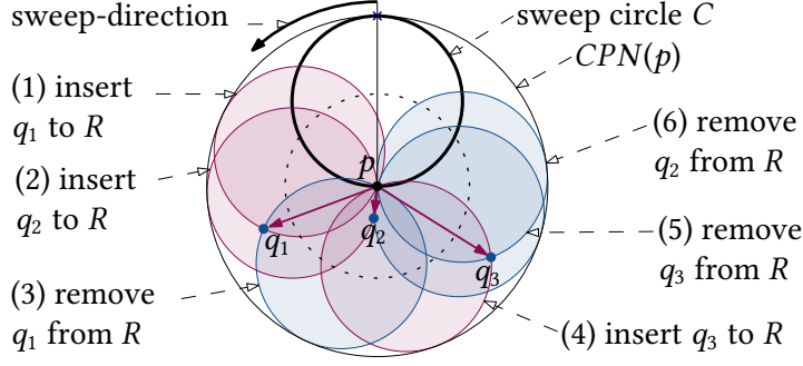
Figure 5.6: Rotational sweep at p with CPN(p) = \{q_1, q_2, q_3\} .
