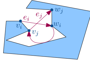
Figure 11.6: Illustration of proof for Theorem 1. Due to the order of the vertices of P the edges e_i and e_j cannot be both part of S .
