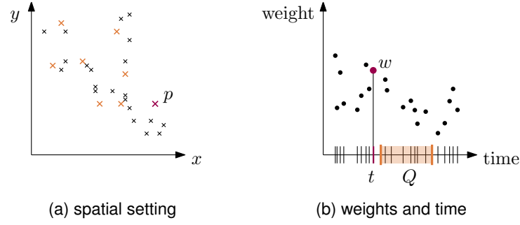
Figure 6.4: The events are given as a point set. Each point p is annotated with a timestamp t and optionally with a weight w . The core problem is to evaluate for an arbitrary query Q all points (orange) whose timestamps lie in Q .
