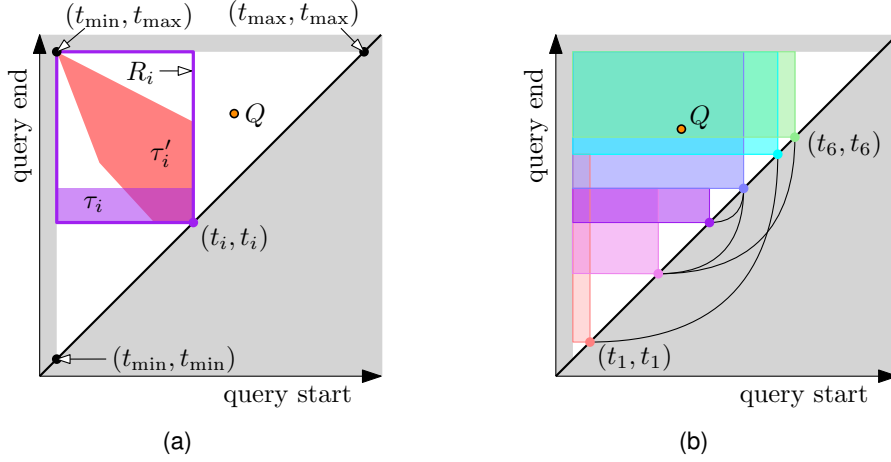
Figure 7.5: Time-window query Q and query region (white triangle). (a) Activity range R_i , activity regions \tau_i and \tau'_i , \tau'_i is never part of an optimal activity diagram. (b) Valid activity diagram of events presented in Figure 7.5; pairs of conflicting events are connected with a curve
