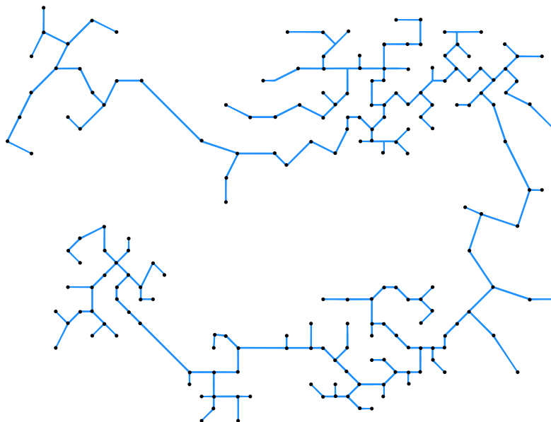
Figure 10.3: A minimum spanning tree T (blue edges) of a set of points.
