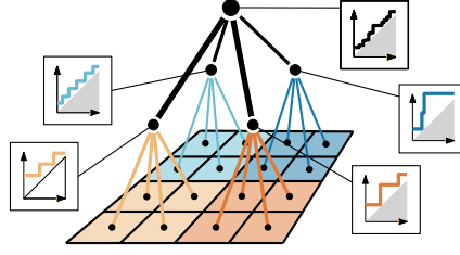
Figure 6.6: The \theta -structure is a search tree built on top of the given grid. Each node is associated with a time structure that is queried to early exclude cells that are not reported.
