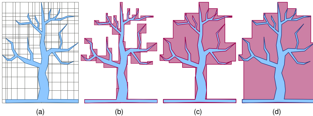
Figure 12.1: Tight \mathcal{C} -hulls. (a) Input polygon P and grid \mathcal{C} based on the segments of P and vertical and horizontal rays emanating from the vertices of P . (b)–(d) Different balances between the perimeter and area of the simplification.
