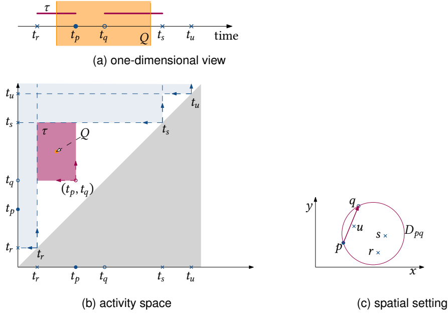
Figure 5.4: Query Q = [t, t'] that yields an edge pq .
