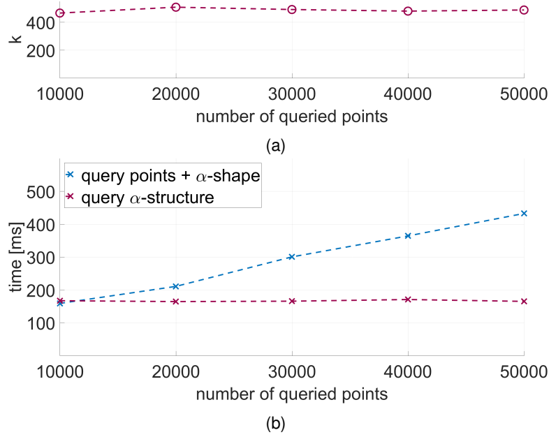
Figure 5.15: Performance of querying the \alpha -structure ( \alpha_{200} ) of storm data set. (a) Number of queried edges k . (b) Query phase time.
