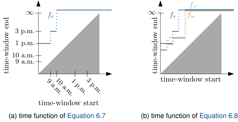
Figure 6.15: Time function. (a) The time function for one leaf node of the \theta^* -structure. (b) The time functions of two sibling nodes f_v and f_{v'} and their parent node f_w .
