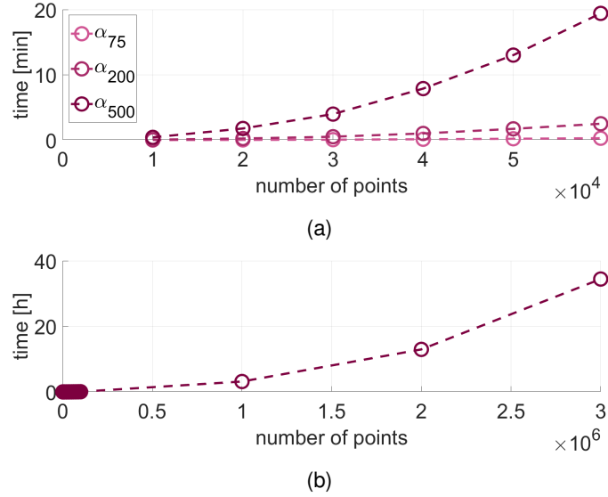
Figure 5.19: Evaluation of the construction of an \alpha -structure. (a) Construction time for the data set storm . (b) Construction time for the data set socialmedia .
