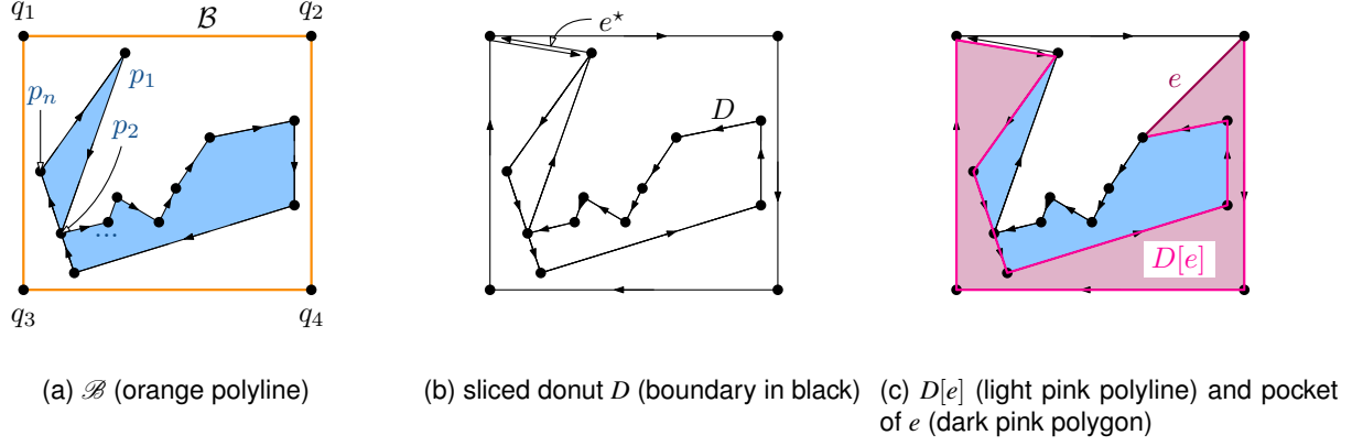
Figure 11.7: Containing box \mathcal{B} and sliced donut D of P .
