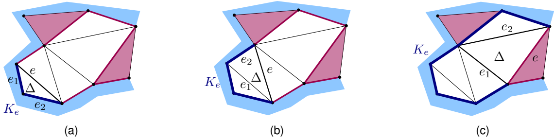
Figure 11.10: Inductive construction of the boundary path K_e of an edge e that is a base edge of an inactive triangle \Delta . (a) Base case. (b) e_1 is a base edge of an inactive triangle, and e_2 is a separator. (c) Both e_1 and e_2 are base edges of inactive triangles.
