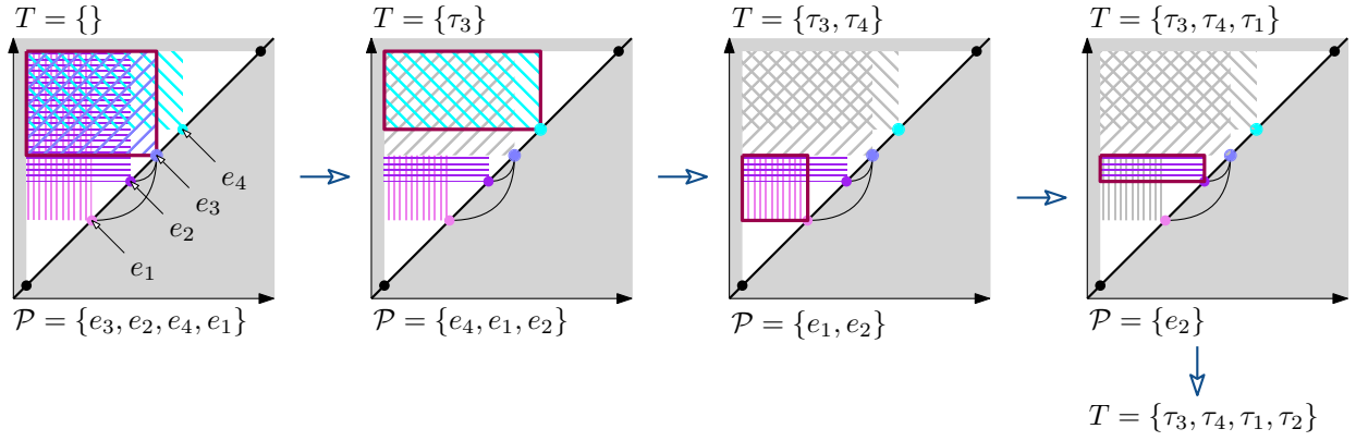
Figure 7.11: Greedy algorithm for four events e_1, e_2, e_3, e_4 and equal weights. There is a label conflict for the pairs (e_1, e_3) and (e_2, e_3) .
