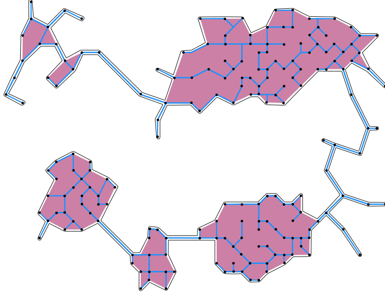
Figure 11.3: Shortcut hull Q of a minimum spanning tree T (blue edges). The boundary of Q is sketched with some offset (black edges). Edges of T that occur twice on the boundary of Q are also accounted twice for the perimeter of Q .
