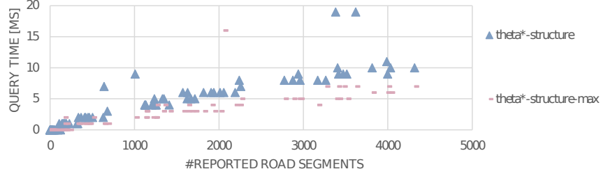
(b) query times for \theta^* -structure with and without max-order
