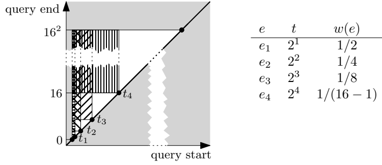
Figure 7.12: Instance with arbitrarily bad approximation ratio for b = 16 .
