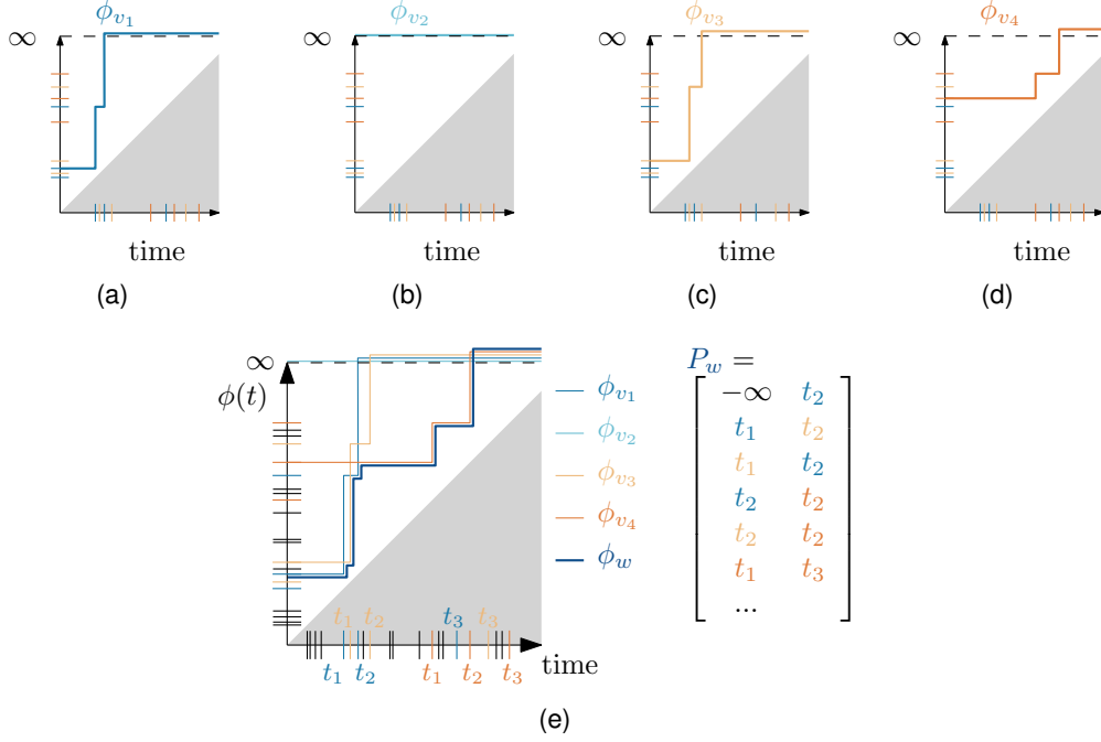
Figure 6.7: Time functions for D_{\text{count}} with \theta = 2 stored at each node of the \theta -structure. (a)-(d) Time function for leaf nodes v_1, v_2, v_3, v_4 of Figure 6.5. (e) Time function for internal node w and its child nodes v_1, v_2, v_3 , and v_4 .
