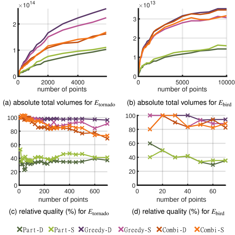
Figure 7.13: Results for the quality of the data structures obtained by the approximation algorithm (Part-D, Part-S), by the greedy heuristic (Greedy-D, Greedy-S), and by the combination of the approximation and greedy (Combi-D, Combi-S). (a),(b) Total volumes for E_{\text{tornado}} and E_{\text{bird}} , respectively. (c),(d) The relative quality for E_{\text{tornado}} and E_{\text{bird}} , respectively; see Section 7.6.2.
