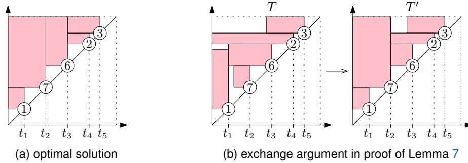
Figure 7.9: Proof of Lemma 7 illustrated for events e_1, \dots, e_5 with timestamps t_1, \dots, t_5 , respectively. The weights of the events are given as numbers in the circles. (a) Due to the process, we insert the activity regions in the following order: e_2, e_1, e_3, e_5, e_4 . (b) An arbitrary activity diagram T and a solution T' that is based on T but where the activity region of e_2 is maximized. The objective of T' is larger.
