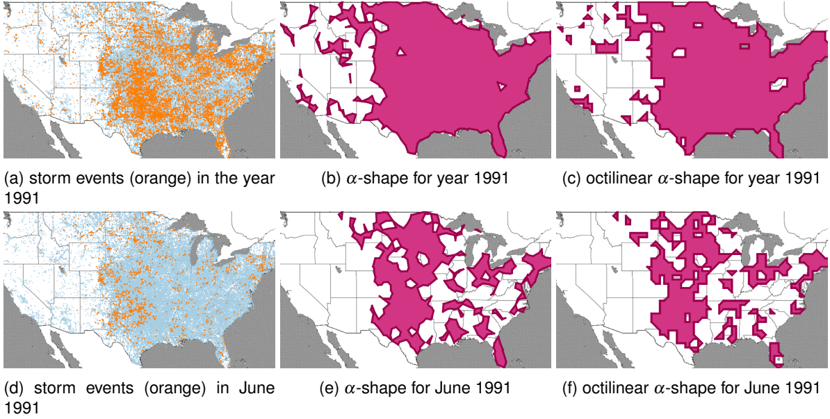
Figure 5.1: Storm events (light blue) in the United States in the years 1991–2001. Each row highlights the storm events in a time window (orange) together with two polygonal representations (lilac). The polygons were generated with our approach. Data retrieved from Data.gov.Map tiles by Stamen Design, under CC BY 3.0. Map data by OpenStreetMap, under ODbL.
