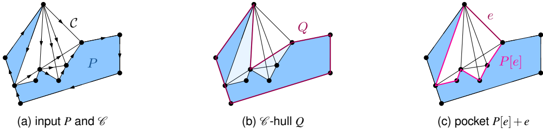
Figure 11.4: The input, a solution, and a subinstance for an instance of the problem.
