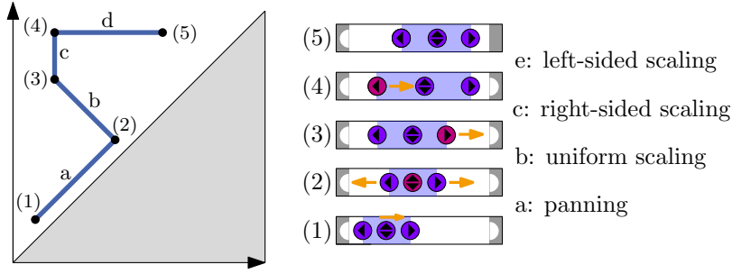
Figure 7.7: Illustration of a query path. (1)–(5): the time windows at the vertices of the query path.
