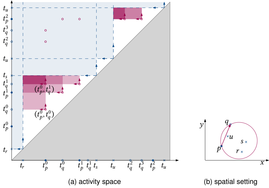
Figure 5.7: Activity region of pq for multiple timestamps.
