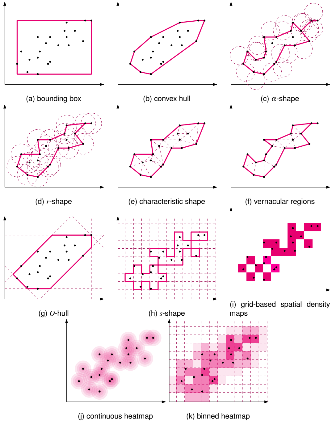
Figure 2.1: Representing a point set. The dashed lines are not part of the visualization, but they are part of the model of the representation. E.g, the \alpha -shapes are defined by the shown set of empty discs.
