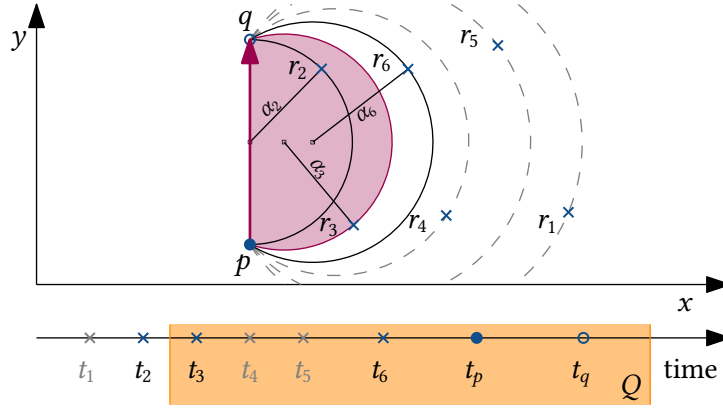
Figure 5.13: Edge in a multi- \alpha -structure.
