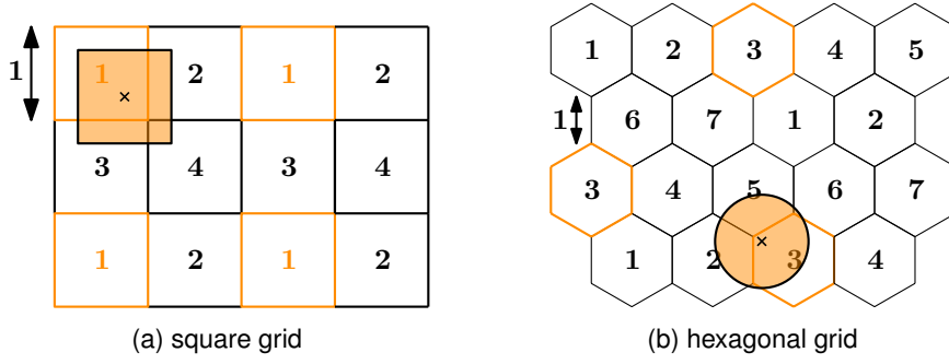
Figure 7.10: Grids used to partition a set of (a) unit-square labels and (b) unit-disk labels into four and seven subsets, respectively.
