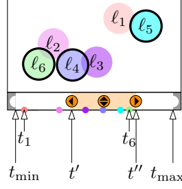
Figure 7.4: Map and time-slider for events e_1, \dots, e_6 , time-window query Q = [t', t''] and labeling for [t', t''] consisting of \ell_4, \ell_5, \ell_6 (illustrated with black stroke).
