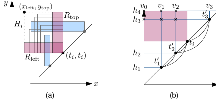
Figure 7.6: (a) Proof of Lemma 5. Illustrated is event e_i with timestamp t_i ; range R_{\text{left}} with minimal x-coordinate x_{\text{left}} and R_{\text{top}} with maximal y-coordinate y_{\text{top}} of e_i ; and rectangle H_i spanned by the lower-right corner (t_i, t_i) and the upper-left corner (x_{\text{left}}, y_{\text{top}}) . Any activity region (blue) of other events that intersects H_i also intersects either R_{\text{left}} or R_{\text{top}} . (b) Discretization of solution space. Shooting vertical and horizontal rays from the timestamps induces a grid that is the basis for the candidate activity regions.
