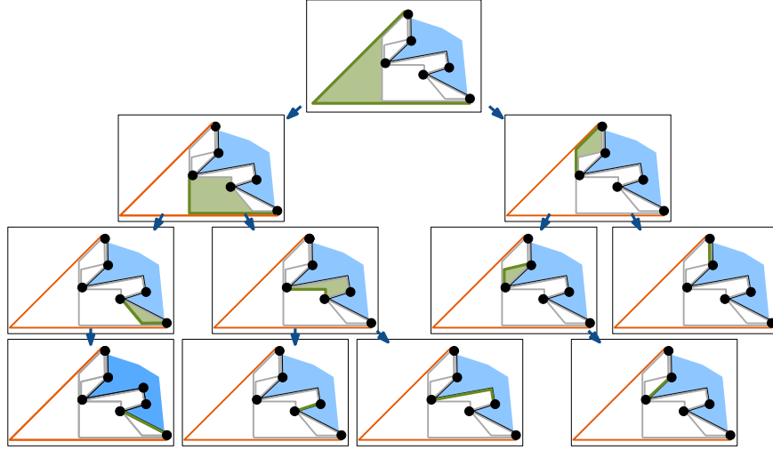
Figure 12.3: The refinement tree of a part of the polygon illustrated in Figure 12.2.
