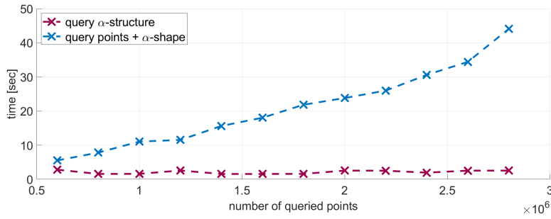
Figure 5.16: Query phase time of the \alpha -structure of socialmedia data set.
