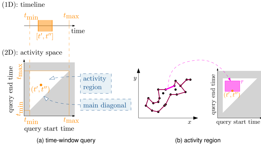
Figure 4.3: Basic Concepts. (a) Time-window query Q = [t', t''] in the one-dimensional view and the activity space. (b) Activity region \tau of an edge (highlighted) of the \alpha -shape for time-window query (t', t'') .
