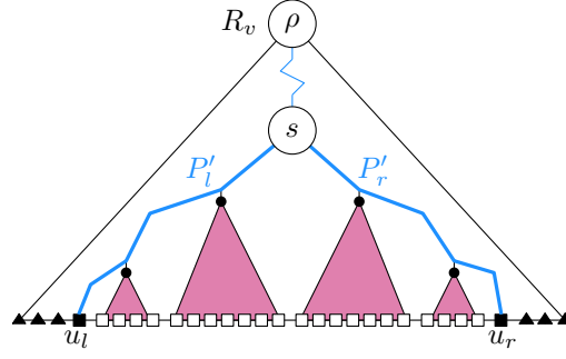
Figure 6.10: Illustration of a range tree R_v . The path from \rho to u_l and the path from \rho to u_r have a common prefix that ends at s . The suffixes P'_l and P'_r separate the queried events (squares) from the others (triangles).
