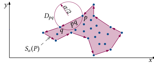
Figure 5.2: \alpha -shape (lilac) for a point set (blue).
