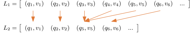
Figure 3.2: Fractional cascading for two arrays L_1 and L_2 of key-value pairs (q_i, v_i) where L_2 \subset L_1 . The pointers from elements of L_1 to elements of L_2 are illustrated in orange.
