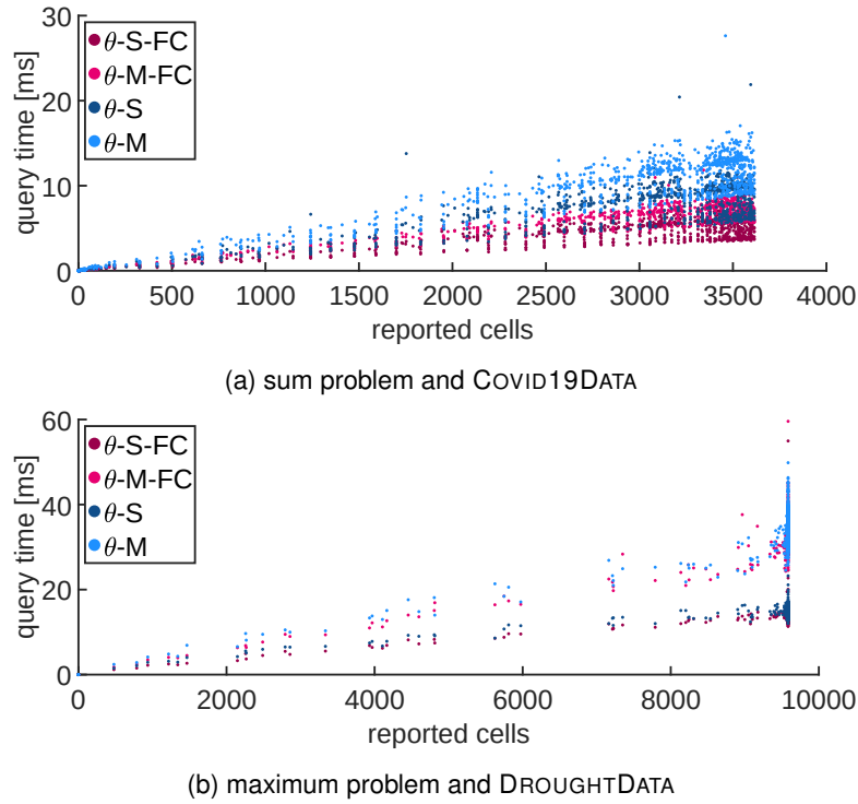
Figure 6.13: Query time for the sum and maximum problem.
