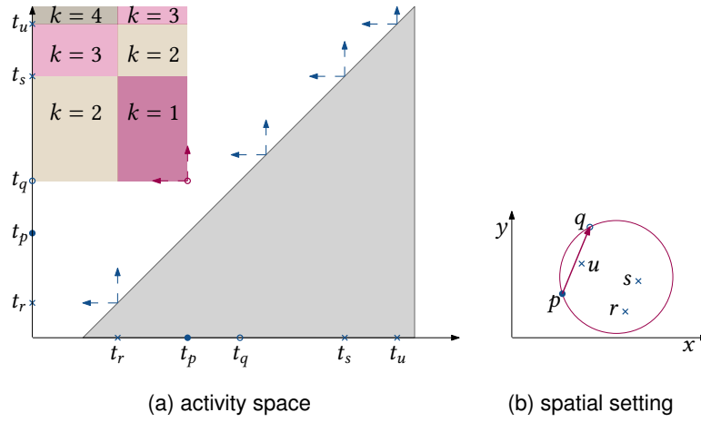
Figure 5.12: Order- k activity regions for k = 1, \dots, 4 of edge pq .
