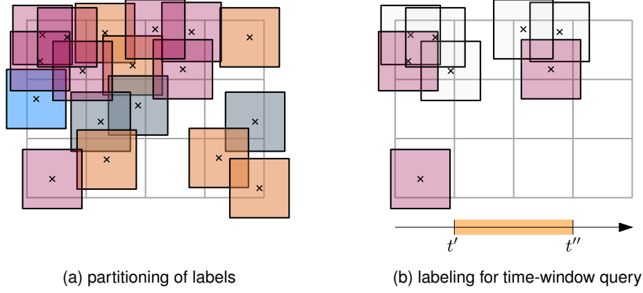
Figure 7.8: Approximation algorithm for unit-square labels (see Figure 7.10a). (a) Labels of one color correspond to one subset. (b) Assume that the solution for the red subset is best. Then, the labeling of a time-window query contains only labels from the red subset.
