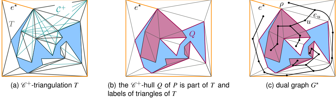
Figure 11.8: \mathcal{C}^+ -triangulation T . (a) All depicted edges belong to \mathcal{C}^+ , while only green edges do not belong to T . (b) The red triangles are active, while all other triangles are inactive. (c) The dual graph G^* of T forms a tree with root \rho .
