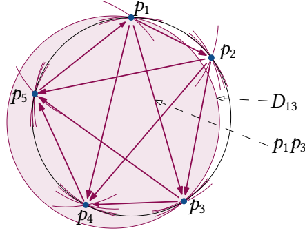
Figure 5.5: Worst-case example for the size of the \alpha -structure.
