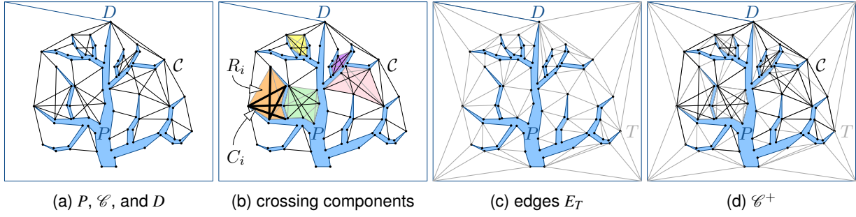
Figure 11.11: Obtaining the enrichment \mathcal{C}^+ from \mathcal{C} .
