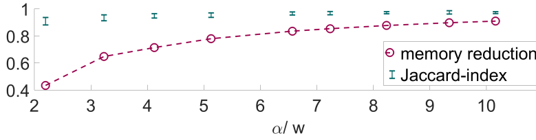
Figure 5.18: Memory reduction of schematized \alpha -structure ( \alpha_{200} ) and shape similarity for schematized \alpha -shapes, i.e., the range of Jaccard index over all queries in \mathcal{Q} . On the x -axis we display the ratio between \alpha and the grid width w .
