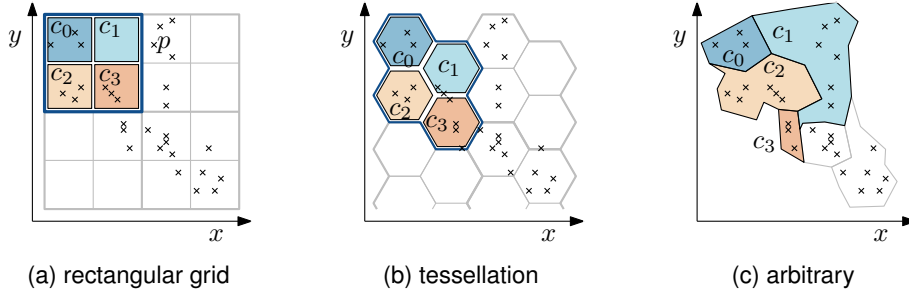
Figure 6.5: Partitions of the map for various types of cells.
