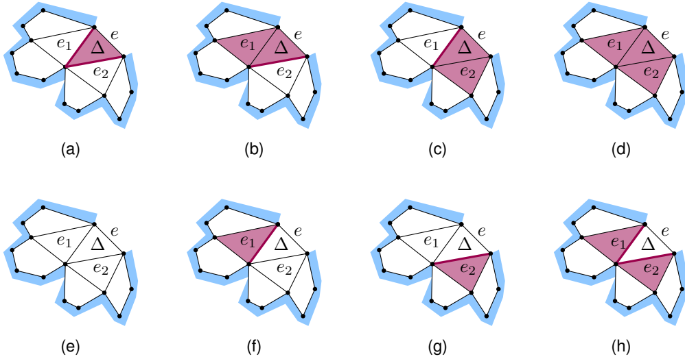
Figure 11.12: The possible cases for the (a)–(d) active (red) and (e)–(h) inactive cost of a triangle \Delta .
