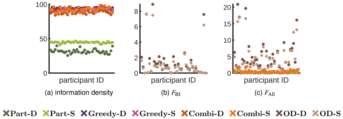
Figure 7.16: Results for analysis of the query phase for Task 4. We compare the data structure obtained by the approximation algorithm (Part-D, Part-S), by the greedy heuristic (Greedy-D, Greedy-S), by the combination of the approximation and greedy (Combi-D, Combi-S) with on-demand implementations (OD-D, OD-S) that do not take any consistency criteria into account. (a) The ratio between the weight of the labeling with respect to the optimal weight obtained by OD-D and OD-S, respectively. (b) Average degree of flickering. (c) Average degree of flickering over all queries within a query path P .
