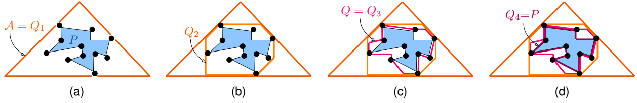
Figure 12.2: Refinement process. (a) Precomputed tight \mathcal{C} -hull \mathcal{A} of the input polygon P . (b) Refinement Q_2 of Q_1 . (c) Refinement of Q_3 of Q_2 . (d) Refinement Q_4 that corresponds to the optimal tight \mathcal{C} -hull of P .
