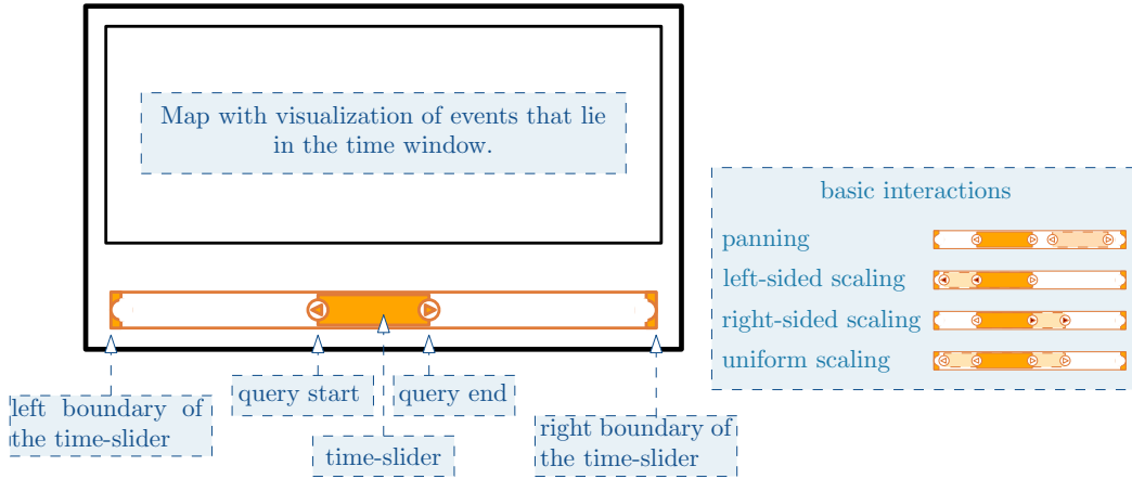
Figure 4.2: Time-slider interface and basic interactions.
