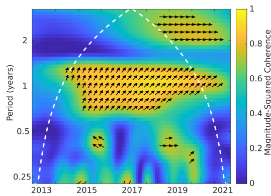
Figure 5.7: Cross Wavelet Transform between monthly precipitation and reservoir water elevation for the period April 2013 to December 2021. Color scale indicates the magnitude squared coherence; arrows indicate the phase difference between the two time series: arrows directed toward right for in-phase relationship; arrows directed toward left for anti-phase relationship. White dashed line shows the cone of influence where the edge effects might disturb the wavelet analysis results.
