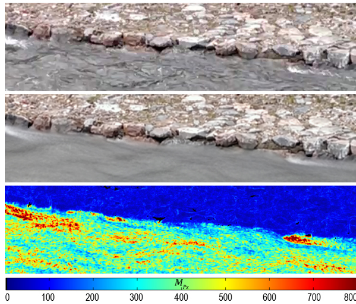
Figure (9.4): Detail view of a co-registered time lapse image sequence taken with 3 fps over 5 s in study area (I). Top down: master image, associated average image & spatio-temporal texture visualized by observed pixel magnitudes M_{Px} .
