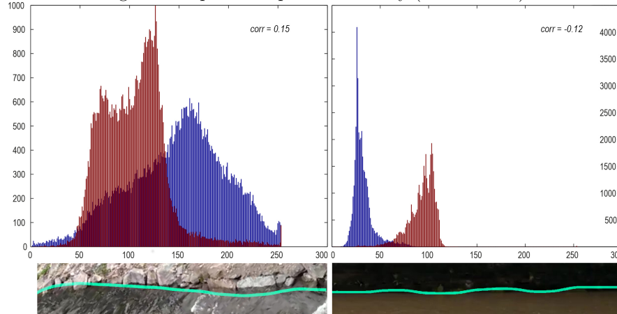
Figure (9.6): Histogram analysis of average image in respect of respective ROIs. Left: gray level distribution of mean values provides no useful information for image segmentation. Right: Study area (III), classifiable due to homogenized image content by averaged gray values.
