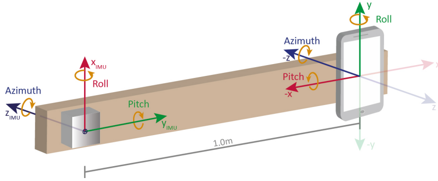
Figure (8.2): Experimental setup.
