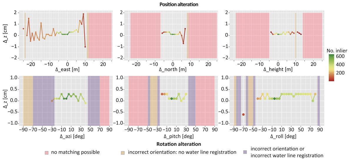
Figure (10.12): Deviation of synthetic water stage (cm) regarding position errors (top) and rotation errors (bottom). No matching in pink; no water line in orange; incorrect water line in purple.
