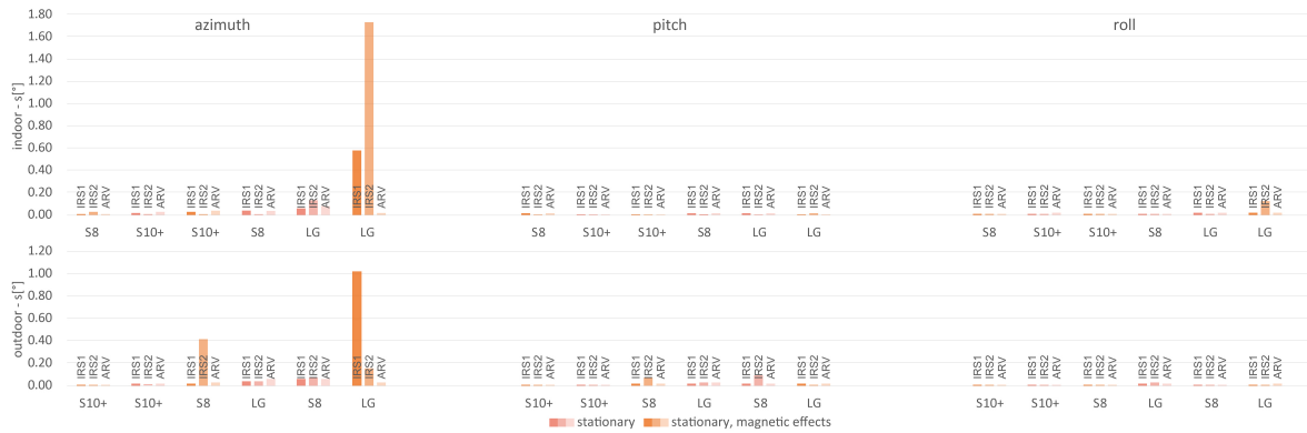
Figure (8.4): Stability investigation of smartphone-based rotation parameters. Stability is defined by the standard deviation s of one measurement series when the smartphone was used in static mode.
