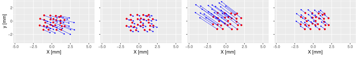
Figure (7.4): Visualisation of image point shifts and zooming effects between the first (red dots) and the last (heads of the blue arrows) measurement within measurement series M1 respectively for (from left to right) the LG Google Nexus 5 camera (cold-started, warm-started) and for the Samsung Galaxy S8 camera (cold-started, warm started). The arrow length is superimposed by a factor of 50.
