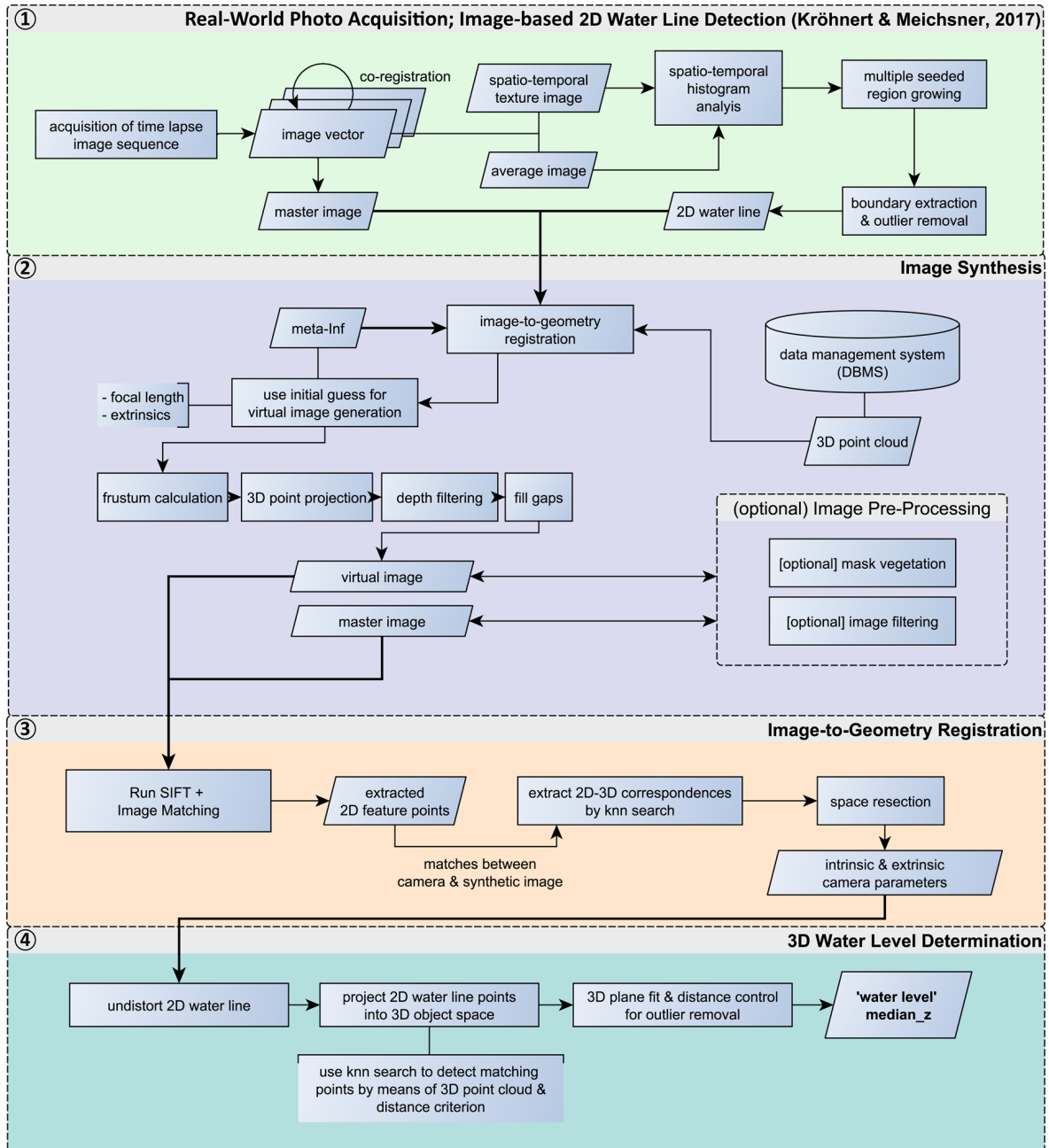
Figure (10.1): Four-step algorithmic concept for camera-based water gauging, implementing image-to-geometry registration.
