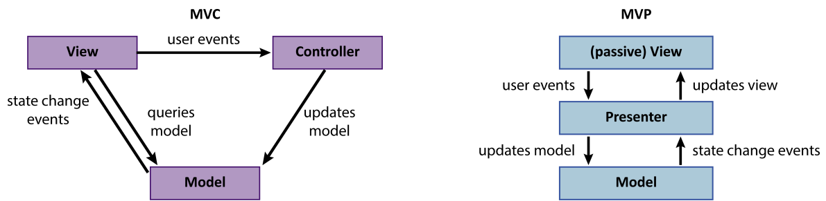
Figure (6.2): MVC and MVP software design patterns, adapted from Chandel (2009).
