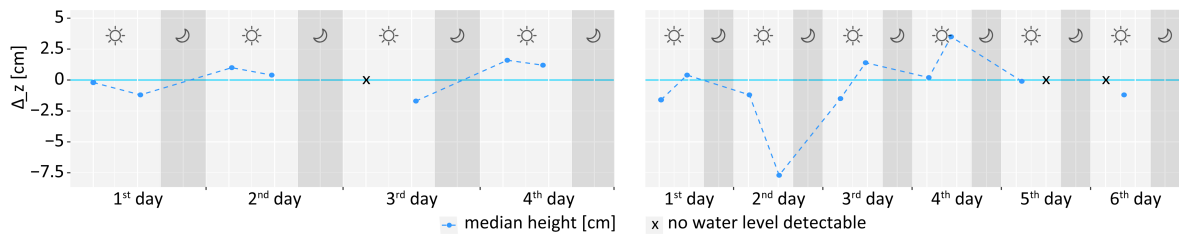
Figure (10.9): Weißeritz observation for 4 days (12th–16th March 2018 – left) and 6 days (26th–31st March 2018 – right). Visualisation of the water-level deviation between the camera-based water levels and the reference values.
