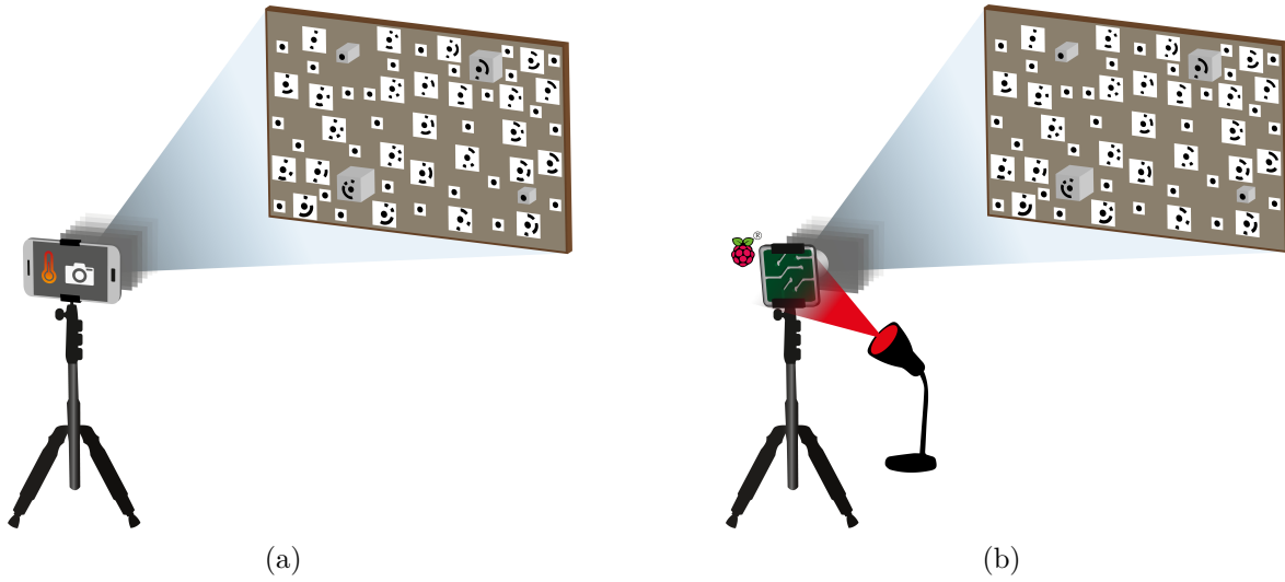
Figure (7.2): Measurement setup to investigate the relation between the IOP and temperature variations occurring from (a) self-heating and (b) ambient temperature variations using smartphone cameras and low-cost RPi cameras, respectively. Camera-to-object distance: about 90 cm. Test field dimensions: 70 × 50 cm, Marker diameter: 10 mm.
