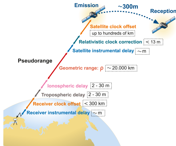
Figure (4.5): Pseudorange measurement impacts, from Subirana et al. (2013).
