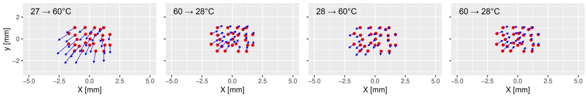
Figure (7.6): Visualisation of image point shifts and zooming effects considering the turning points between the heating and cooling phases of the RPi camera investigation M1. The arrow length is superimposed by a factor of 50.
