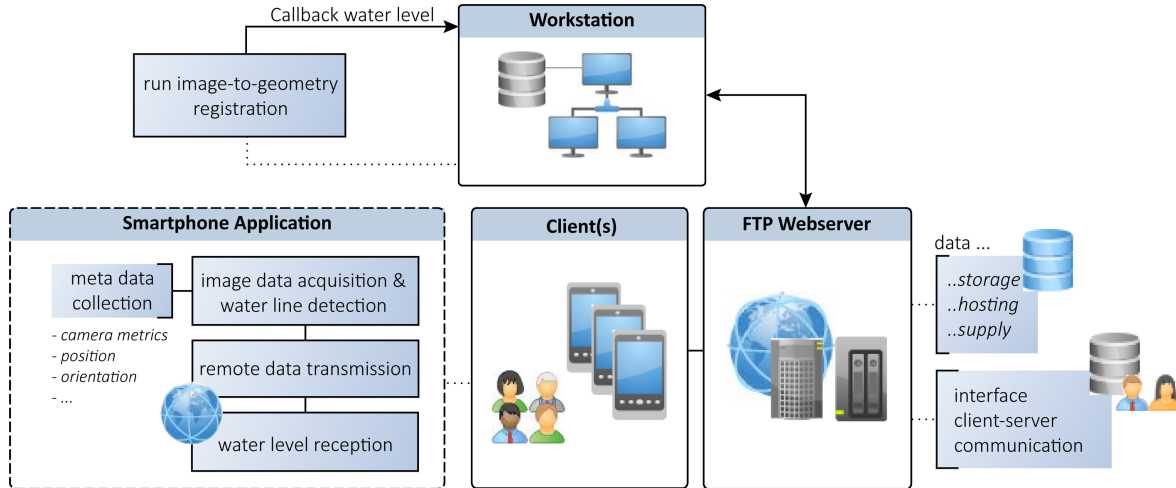
Figure (10.7): Client-server architecture applied to "Open Water Levels" (adapted from Kröhnert and Eltner, 2018).
