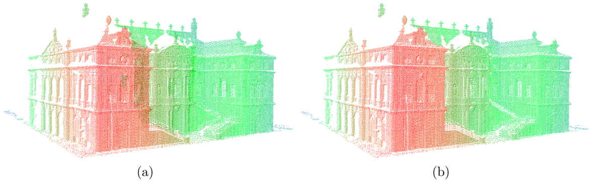
Figure (10.4): Occlusion ambiguities. (a) Translucent, falsely mapped 3D points. (b) Result after filtering. Colouration is a function of the distance from the virtual projection centre to the 3D object points (red – near; blue – far).
