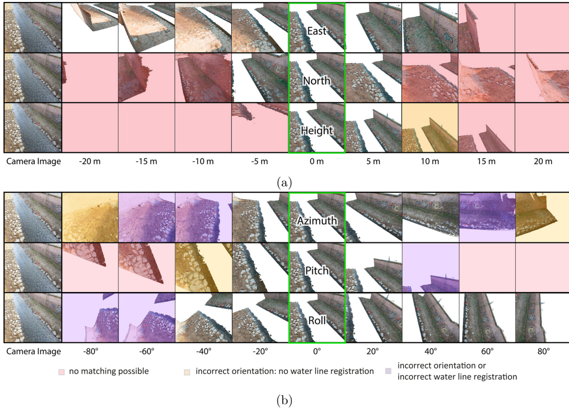
Figure (10.11): Image synthesis influencing water level determination: (a) with erroneous position values; (b) with erroneous rotation values. No matching in pink; no water line in orange; incorrect water line in purple.
