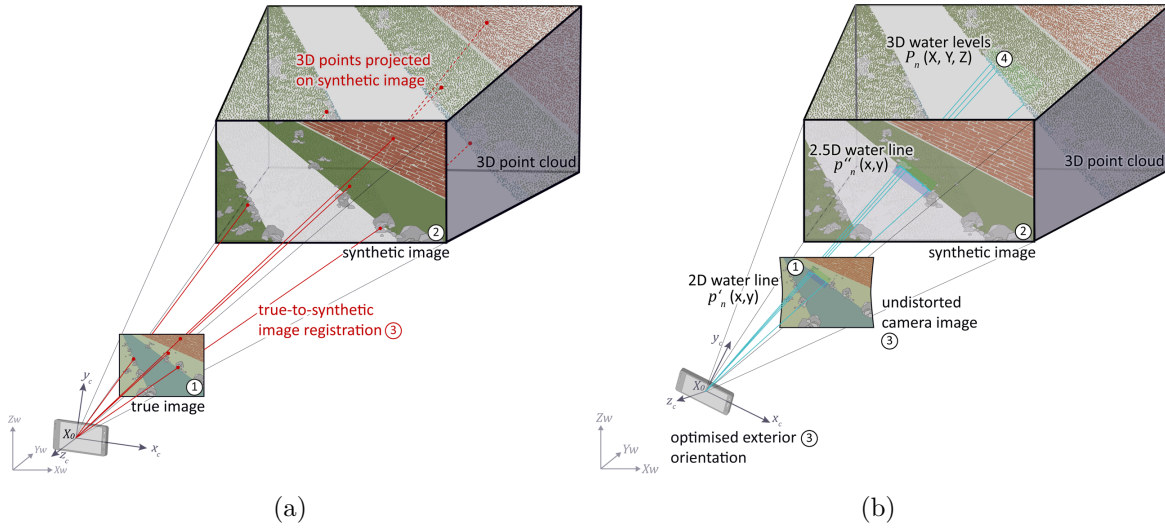
Figure (10.6): Visual workflow summary. Numbering corresponds to the steps given in Figure 10.1.
