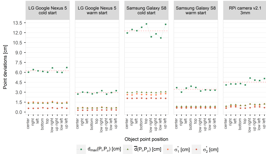
Figure (7.11): Principal standard deviations s_1^* and s_2^* giving the directional error in object space for each projected object point and for each investigated camera.
