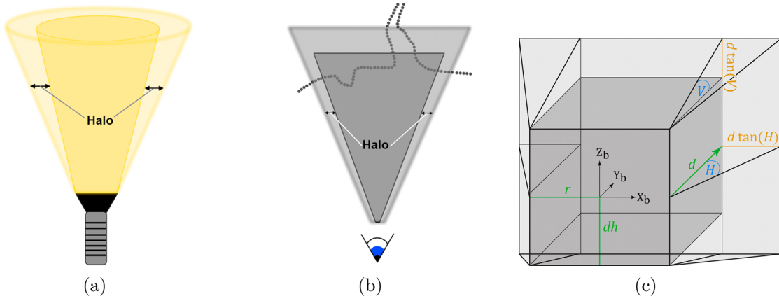
Figure (10.3): View frustum and halo expansion. (a) Visual analogue between partial illumination halo of a light bulb. (b) Partial visibility halo of perspective view and projection. (c) The defined bounding box.
