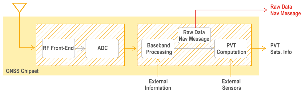
Figure (4.6): Generic block diagram of a smartphone-implemented GNSS receiver, from GSA (2017). ADC means Analogue-to-Digital Converter.
