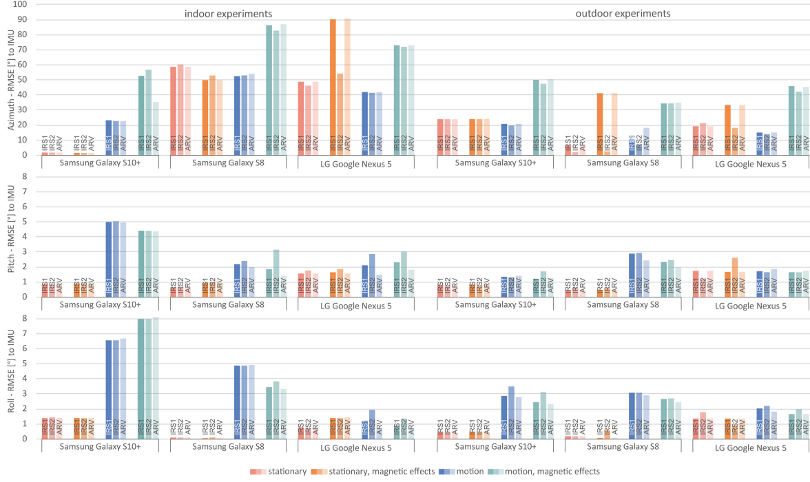
Figure (8.3): Accuracy investigation of smartphone-based rotation parameters. Accuracy is defined by the RMSE calculated from the deviations between the rotation parameters from the smartphone and the reference values from IMU Spatial .
