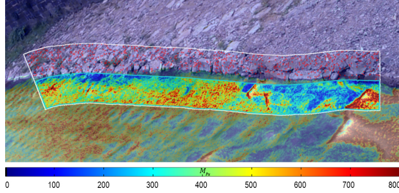
Figure (9.7): Spatio-temporal texture overlay referring to study region (II).
