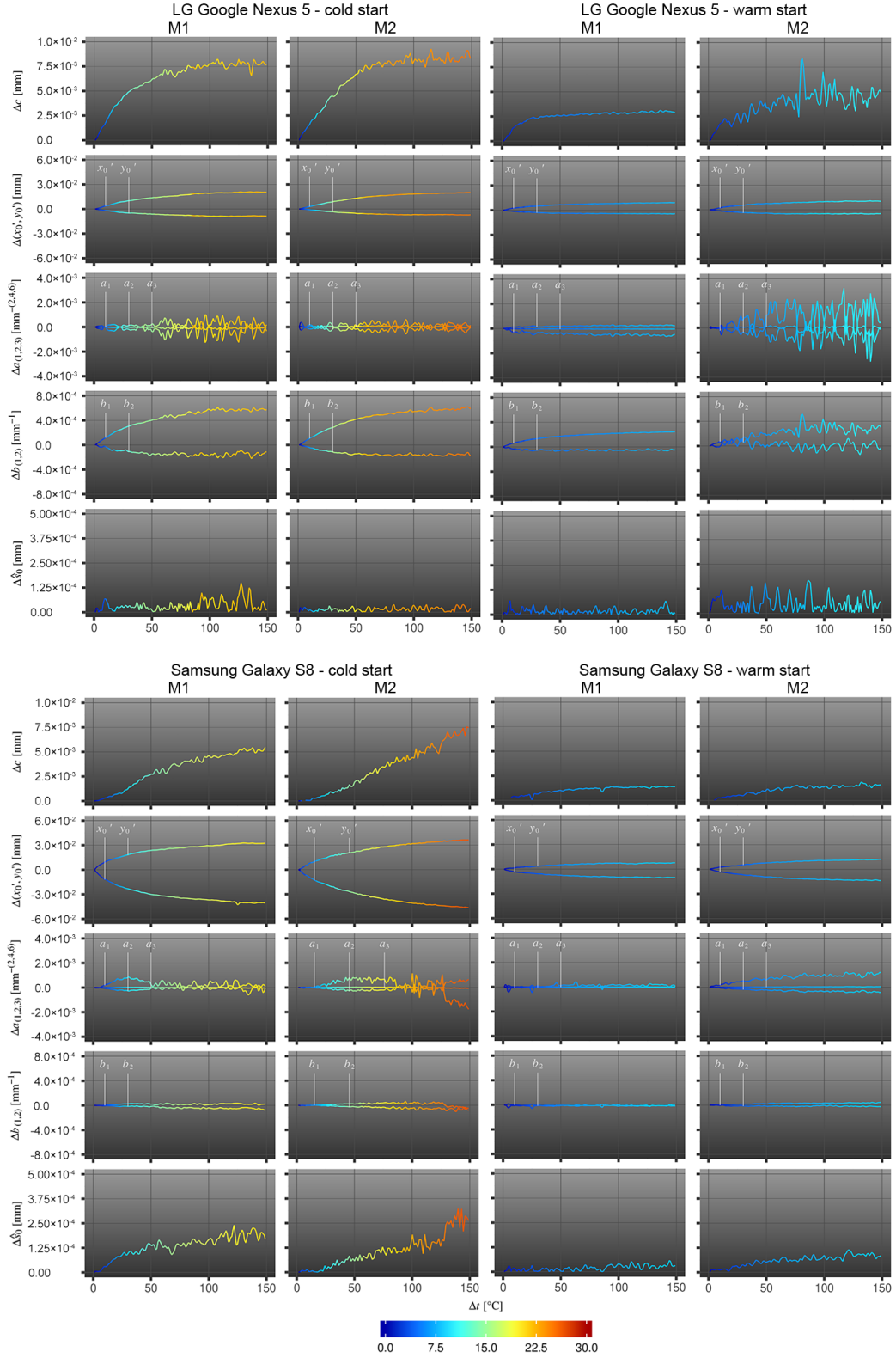
Figure (7.3): IOP-to-temperature assessment; x-axis: number of measurements per measurement series M1/M2; y-axis: estimated deviation per parameter \Delta k compared to the respective initial value; color-code: temperature difference \Delta t (measured at the battery) to the initial temperature value when the phone was started.
