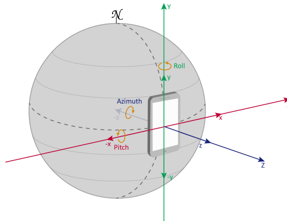
Figure (8.1): Smartphone sensor coordinate system in relation to a world coordinate system.
