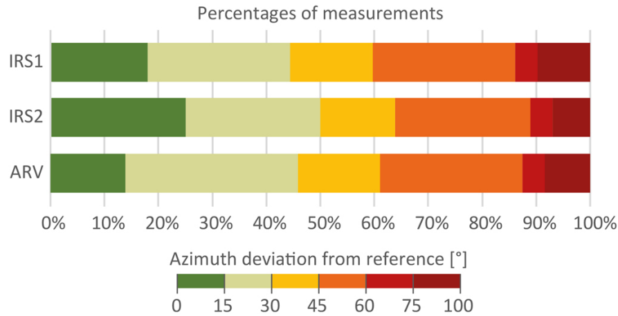
Figure (8.5): Histograms of the total deviations regarding azimuth in relation to the measurements from IRS1, IRS2 and ARV.
