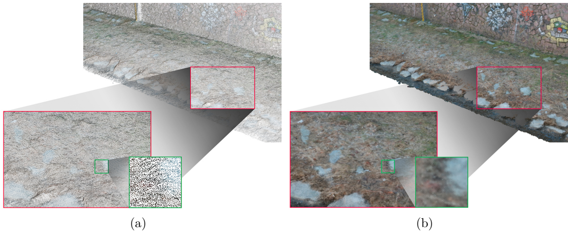
Figure (10.5): Visualisation of the gap-filling algorithm using the example of a 3D point cloud showing a shore area with stones and dried vegetation. (a) Projected points with gaps due to the discrete point cloud density. (b) Gaps between the projected points are filled by the gap-filling algorithm to provide continuous image information. Both images show the projected points of this 3D point cloud at the same scale.
