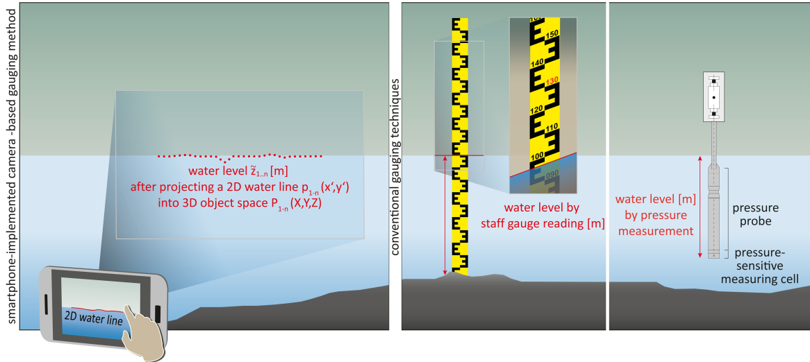
Figure (10.8): Set-ups of the smartphone-implemented camera-based gauging method (left) and two conventional gauging systems (middle and right) installed at the River Weißeritz, Dresden. Pressure gauge visualisation adapted from Morgenschweis (2010).
