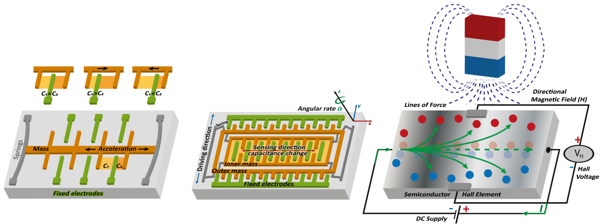
Figure (4.7): Basic structures of MEMSs. From left to right: accelerometer, gyroscope and magnetometer build in smartphones. Figures adapted from Nedelkovski (2015) and Maenaka (2008).
