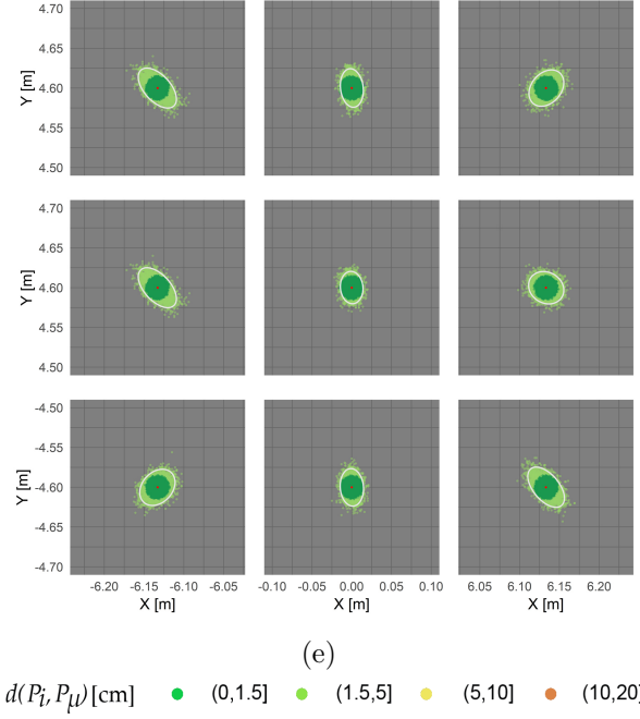
Figure (7.10): Projection of image points p'_i(x', y') onto a virtual object plane in a distance of Z = 10 m with fixed EOP- and simulated IOP (visualisation of every 10th point P_i(X, Y) ). LG Google Nexus 5, cold started (a) and warm started (b); Samsung Galaxy S8, cold started (c) and warm started (d) and Raspberry Pi v2.1 (e). The generated object points were colourised by means of their Euclidean distance d(P_i, P_\mu) to the expected object point coordinates. The white ellipses are the confidence ellipses with 95% probability.
