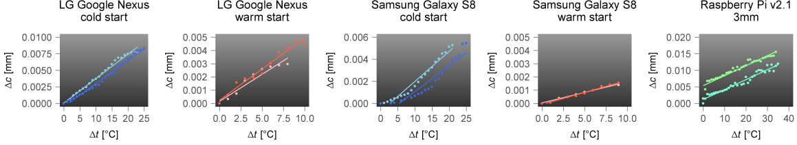
Figure (7.7): Visualisation of the linear dependencies between changing IOP and temperature on the example of principal distance c . Considering the RPi observations, the aggregated data is sorted by temperature change. Light colors refer to the respective measurement series M1 and darker colors refer to the respective measurement series M2.
