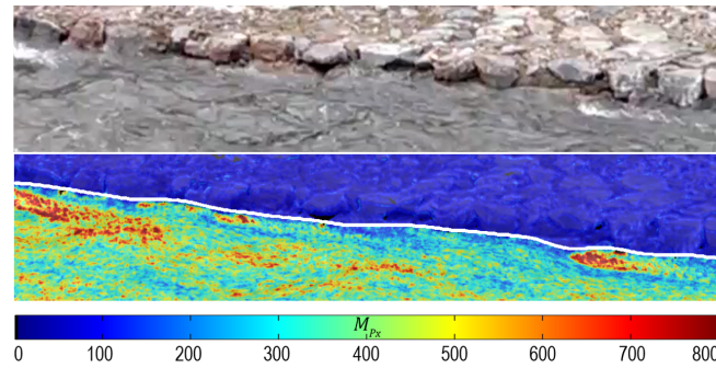
Figure (13.2): Water line detection by spatio-temporal texture analysis.
