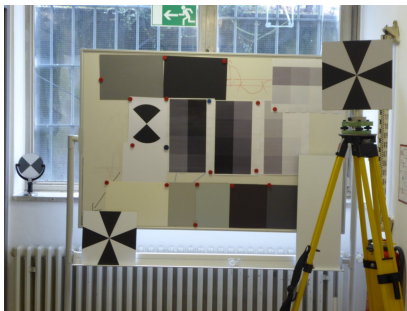
Abbildung 5.1: Cheap setup for an easy determination of the intensity-based range precision [Schmitz et al., 2019].
