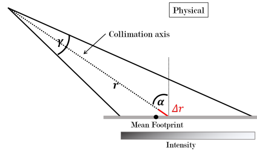
Abbildung 3.10: Impact of the elongated laser beam on the range measurements with the physical explanation where the distance is measured too short.
