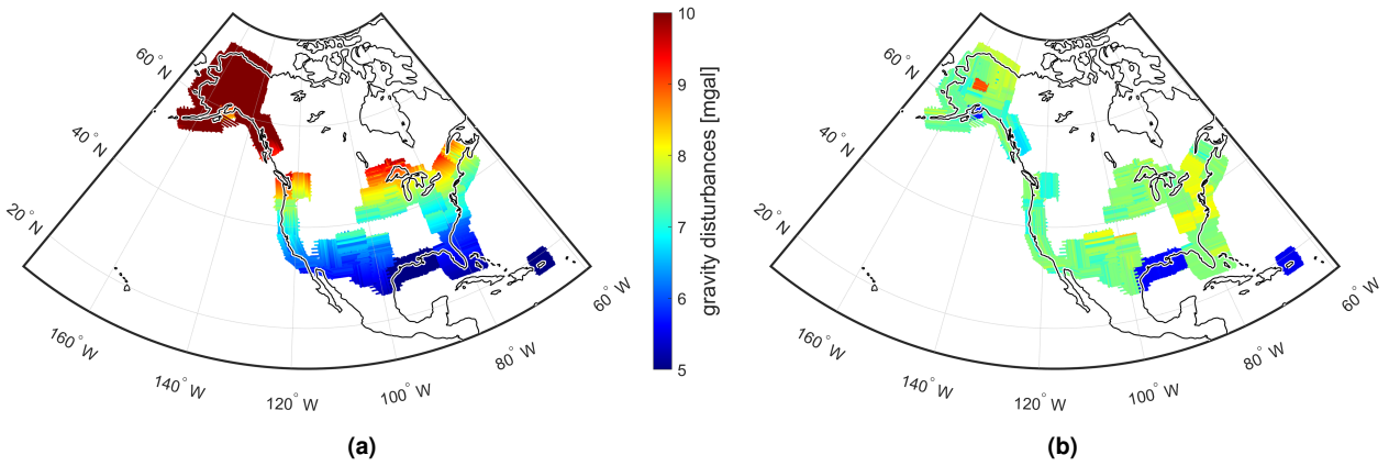
Fig. 4.3 – A-priori signal energy (i.e., square root of the variance entries in C_{il}^{\mathcal{X}} ) modelled by the estimated degree variances (see Fig. 4.4). (a) Calculated using the unmodified geometry. (b) Calculated using the spherically modified geometry.
