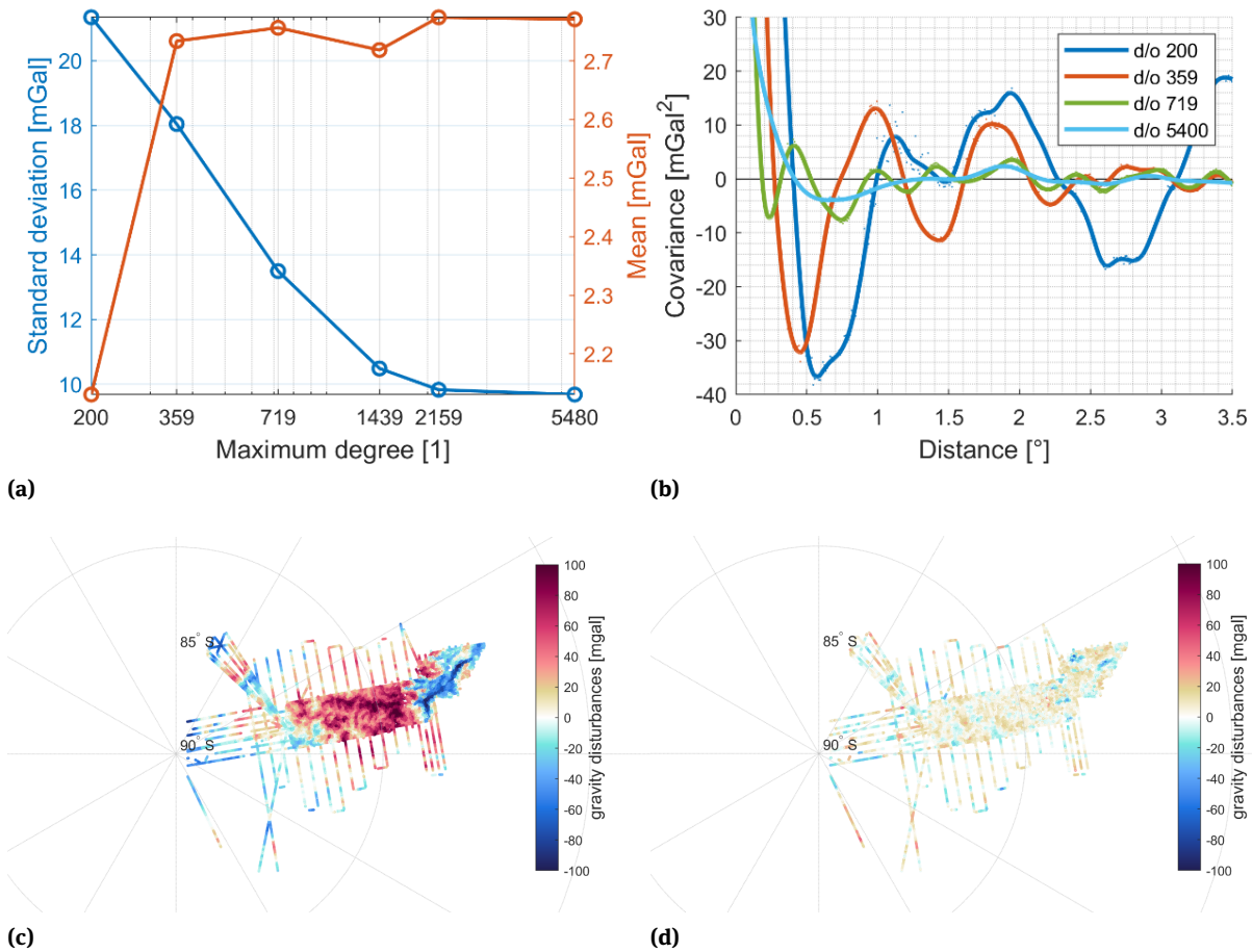
Figure 9: (a) Standard deviation (blue) and mean (red) for varying maximum degree of the SATOP1 model reduction from the AGAP observations. (b) Empirical covariances depending on the spherical distance for different maximum degree reductions (200-359-719-5400). (c) The AGAP observations as provided. (d) Differences to SATOP1 up to d/o 5400.
