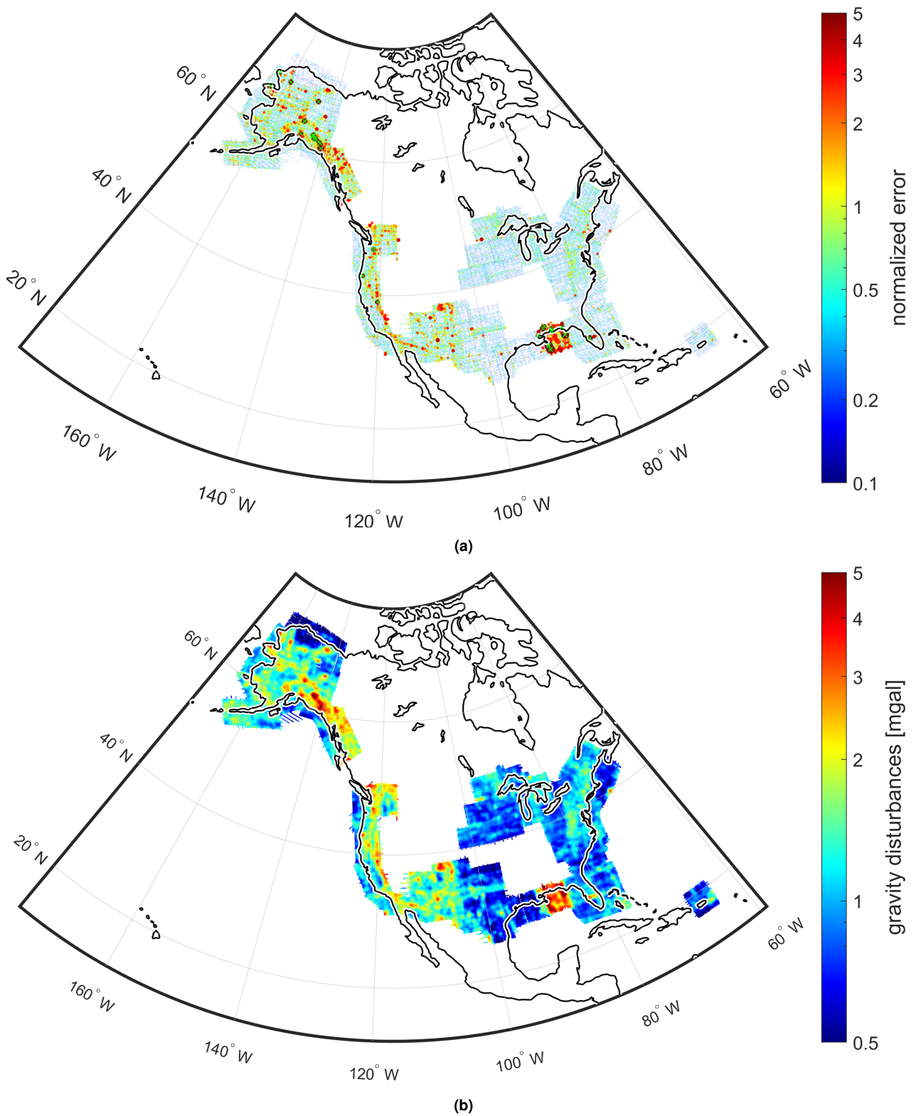
Fig. 4.12 – Post-collocation validation of the GRAV-D observations using PE-LSC and \sigma^0 = 4 mGal. (a) Normalized observation errors \Delta \lambda^M with \sigma^0 = 4 mGal. Assumed outliers with k > 4 are additionally marked with green crosses. (b) Empirical standard deviation \sigma^e (see Eq. 4.19) using a Gaussian averaging kernel with a width of 30 km (HWHM, that is 2 \log 2 \sigma ).
