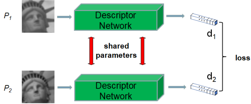
Figure 4.2.: Descriptor Learning Architecture. The Siamese CNN is composed of two branches, P_1 and P_2 . Each branch takes one patch (feature support window) as input and runs it through the descriptor network to obtain the descriptors d_1 and d_2 . This process is repeated for each input patch. The descriptor networks in the two branches share the same weights. The input pairs of patches are matched or unmatched pairs of features. Loss based on the calculated descriptors is then constructed.
