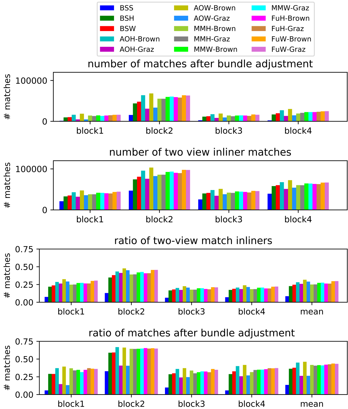
Figure 5.18.: Number and ratio of matches for different blocks. From top to bottom: number of matches after bundle adjustment ( N_{match}^{surv\_BA} ), number of two view inlier matches ( N_{match}^{inl\_2view} ), ratio of two-view inlier matches ( R_{initial}^{inl\_2view} ) and ratio of matches after bundle adjustment ( R_{surv\_BA}^{inl\_2view} ). All four of the bar figures share the same label for different variants, as shown in the top figure. For the two related ratios (3rd and 4th row), the mean values over the four groups are also provided at the end of each bar figure.
