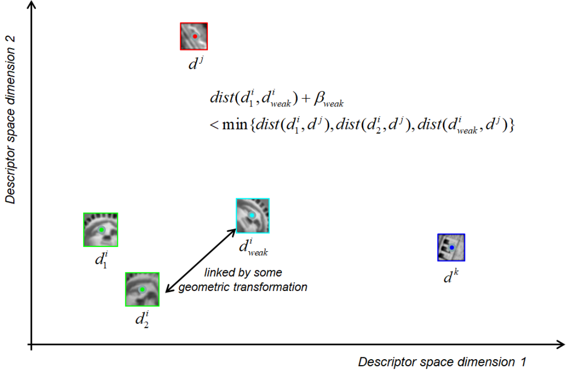
Figure 4.5.: The idea of weak matches. Here the descriptor space is simplified as a two dimensional space. In descriptor space, the descriptors d_1^i and d_2^i represent a pair of matched features, the feature support window of which is shown as two image patches with green borders. The other two features represented by d^j and d^k are unmatched features to d_1^i and d_2^i . Through geometric transformation of the feature support window of d_2^i , another patch - the descriptor of which is d_{weak}^i - is found with the condition that the distance between d_2^i and d_{weak}^i is maximized. Although the feature represented by d_{weak}^i is a weak match, it should still be closer to d_1^i when compared to any unmatched features. Therefore, the border of the descriptor space dominated by d_1^i is d_{weak}^i , and a threshold \beta_{weak} is proposed to form a margin between the feature space of d_1^i and the space of any other unmatched features. This means that the minimum distance between d_j and each one of d_1^i , d_2^i and d_{weak}^i is made to be larger than the sum of dist(d_1^i, d_{weak}^i) and the threshold margin \beta_{weak} .
