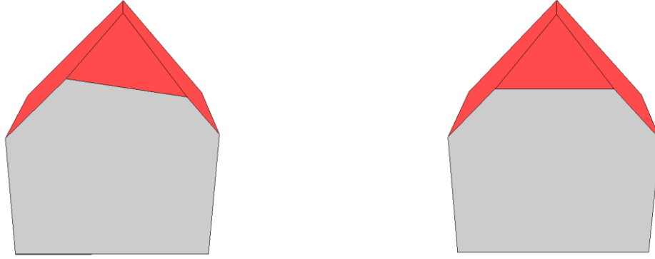
Figure 6.25. Reconstructed building model before (left) and after the local half-space adjustment step (right).
