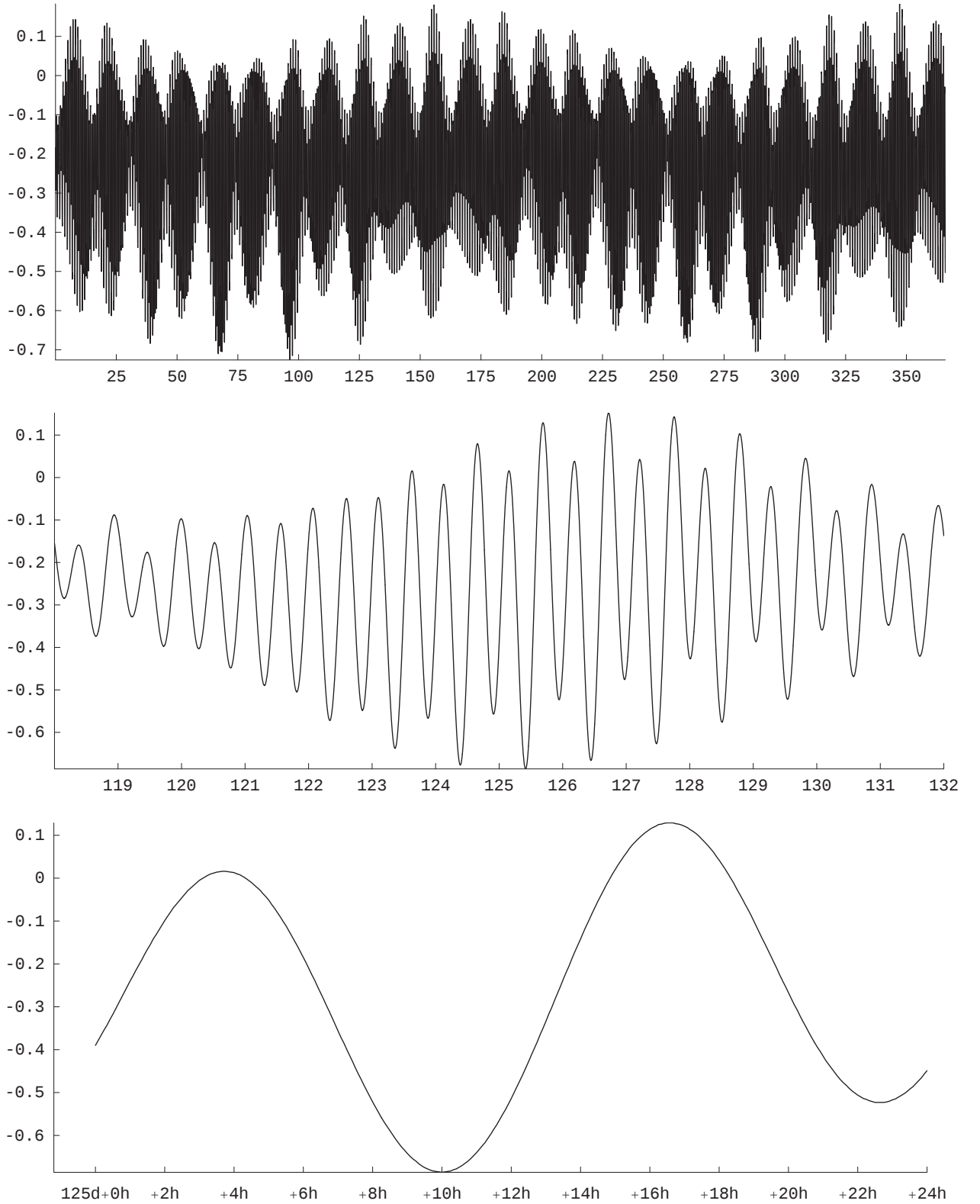
Fig. 5: Differences in tidal potential variations between points P_1 and P_8 (see table 1) in \text{m}^2/\text{s}^2 vs day of year 2012. Throughout a year the maximum peak-to-peak difference is about 0.8 \text{ m}^2/\text{s}^2 (top). The main tidal species (semidiurnal, diurnal, long-term, e.g. fortnightly) are clearly visible (middle). In the course of a single day the maximum tidal potential difference can build up within approximately 7 hours (bottom).
