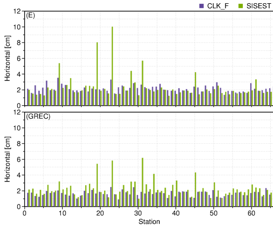
Figure 5.20 Horizontal position accuracy of each station with 30-min updated orbits and clocks for Galileo-only (upper) and GREC (lower) solutions.
