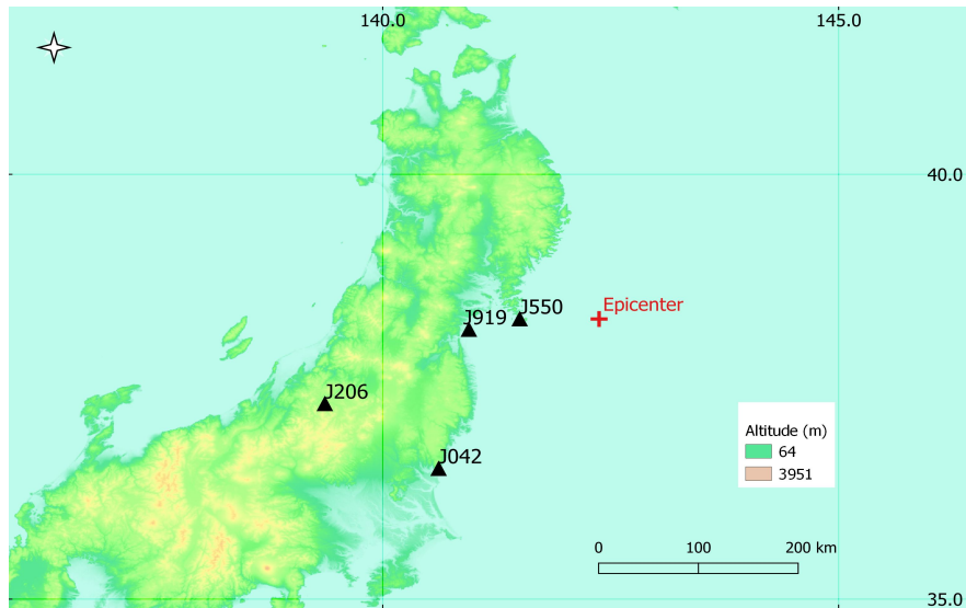
Figure 3.14: Simulated clock sites in Japan with the epicentre of Tohoku earthquake 2011.
