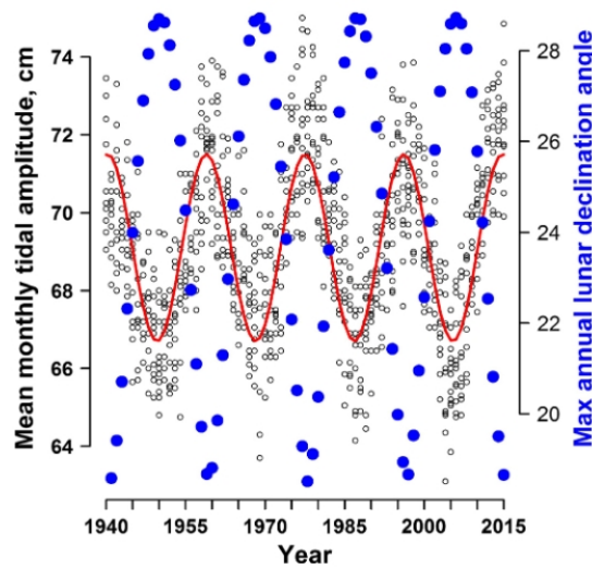
Figure 5.5: Time series showing tidal amplitude and lunar declination angle variations. Data from the NOAA tide gauge at Battery, NYC (Station ID: 8518750) fitted with a harmonic regression (red line, amplitude: 2.4 cm, mean: 69.1 cm, period: 18.6 years) (Rochlin and Morris, 2017).
