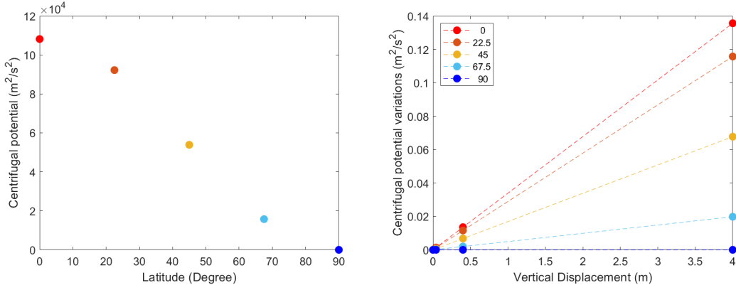
Figure 3.1: Centrifugal potential at selected latitudes in \text{m}^2/\text{s}^2 (left) and centrifugal potential variations at selected latitudes for vertical displacements (d) up to 4 m (right)
