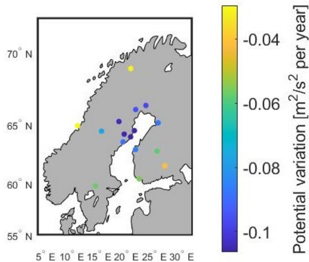
Figure 3.12: Simulated GIA signal over Fennoscandia in terms of effective potential variation per year
