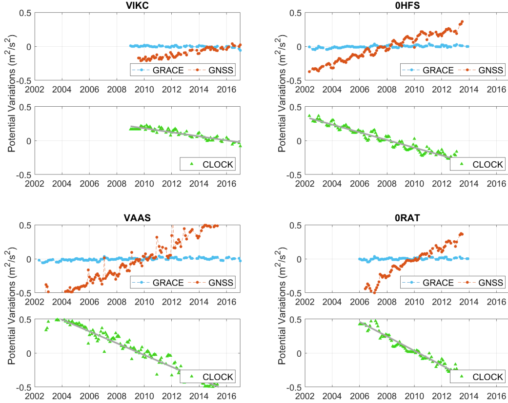
Figure 3.13: Linear potential variations in Fennoscandia at the sites VIKC, VAAS, ORAT and 0HFS dominated by vertical deformation. The upper panels show the variations separately derived from GRACE and GNSS. The lower panels show the combined effect of height changes (GNSS) and mass changes (GRACE) as it could be observed by clocks (CLOCK), with the fitted linear signal in gray.
