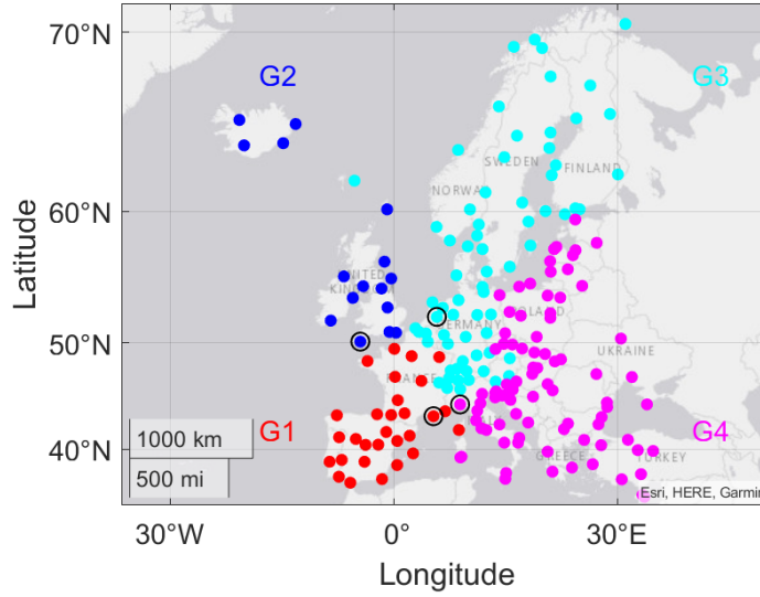
Figure 4.2: Classified EUVN height system. The generated 4 LHSs G1, G2, G3, and G4 are indicated in different colours. The tide gauge locations for each LHS are indicated by a black circle.
