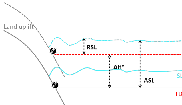
Figure 2.7: Absolute Sea Level (ASL) and Relative Sea Level (RSL) change with respect to tidal datum (TD) in the case of land uplift \Delta H and sea level (SL) rise (Vincent and Müller, 2024)
