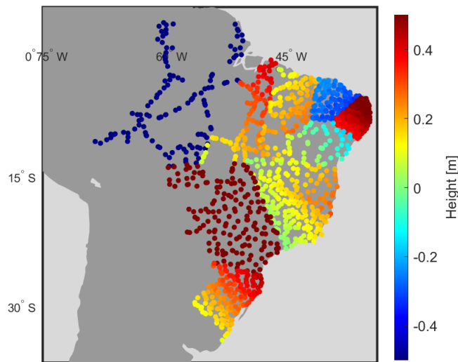
Figure 4.9: Simulated "true" errors before unification for the various classified local heights.
