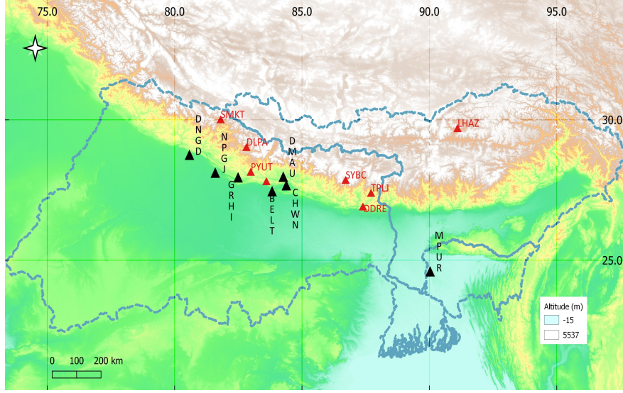
Figure 3.3: Himalayan region with the Ganges-Brahmaputra-Meghna river basin and assumed clock sites (high-altitude stations (red), low-altitude stations (black))
