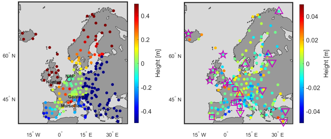
Figure 4.3: True error before unification (left) and the residual errors after unification (right) obtained with the extended model. Different symbols in the right image represent the clock sites in each LHS. The error reduced to \approx \pm 1 cm after the clock-based unification.
