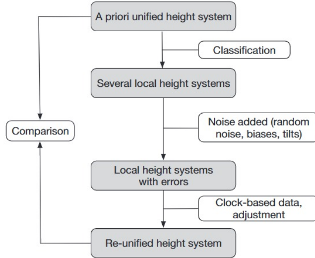
Figure 2.5: The scheme of simulator (Wu et al., 2018)
