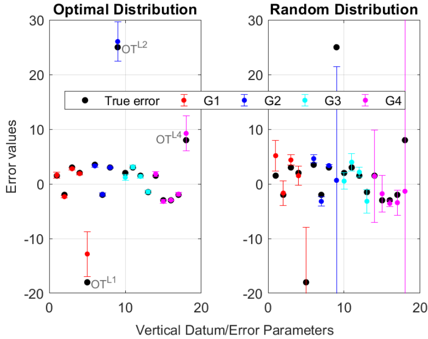
Figure 4.5: Estimated error parameters in an extended model with a total of 18 unknowns with their standard deviations for optimal (left) and random (right) distribution. The assumed true error values are provided for reference. The units are different for tilts (cm/degree) and offsets (cm).
