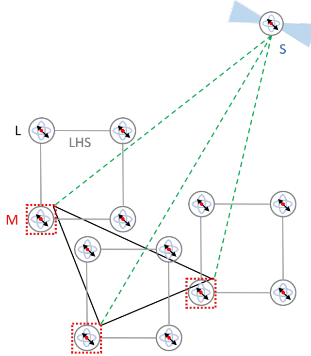
Figure 4.10: Configuration of clock distribution with master clocks (M) and local clocks (L) in each LHS. Local clock connections were assumed with fibre links in the LHS. Master clocks of each LHS can be connected via either optical fibre (black) or free-space links (green).
