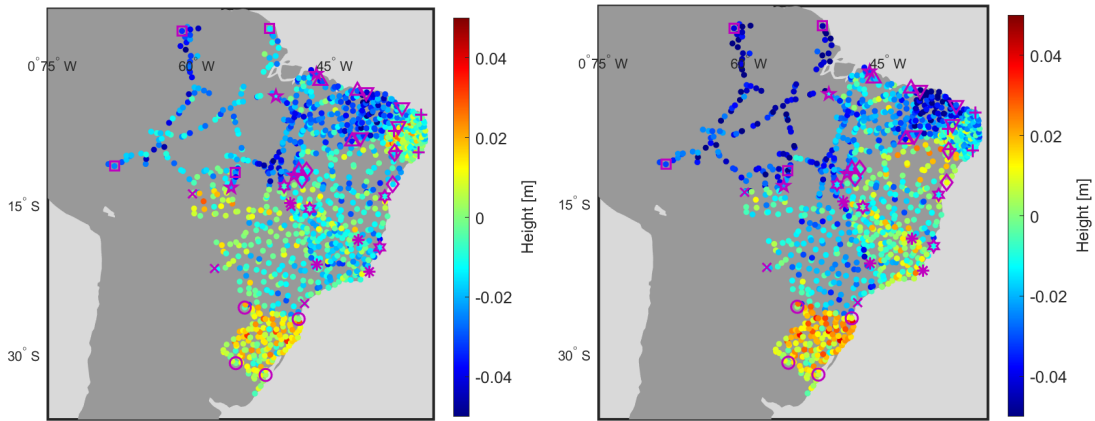
Figure 4.14: Adjusted errors after reunification with correlation coefficients 0.5 (left) and 0.8 (right). Here, CE (Clock Error) is supplied as a random normal distribution of constant variance 0.1 \text{ m}^2/\text{s}^2 .
