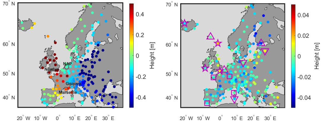
Figure 4.7: "True" error before unification (left) and residual error after unification (right) when clocks with different frequency uncertainties are used in each LHS with more accurate clocks ( 10^{-18} ) placed at LLC (Lower Left Corner) and URC (Upper Right Corner). Different symbols in the right image represent the clock sites in each LHS. The error reduced to \approx \pm 1 cm after clock-based unification.
