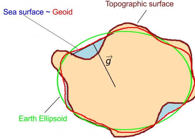
Figure 2.3: Ellipsoid vs. geoid (Favier, 2016)
