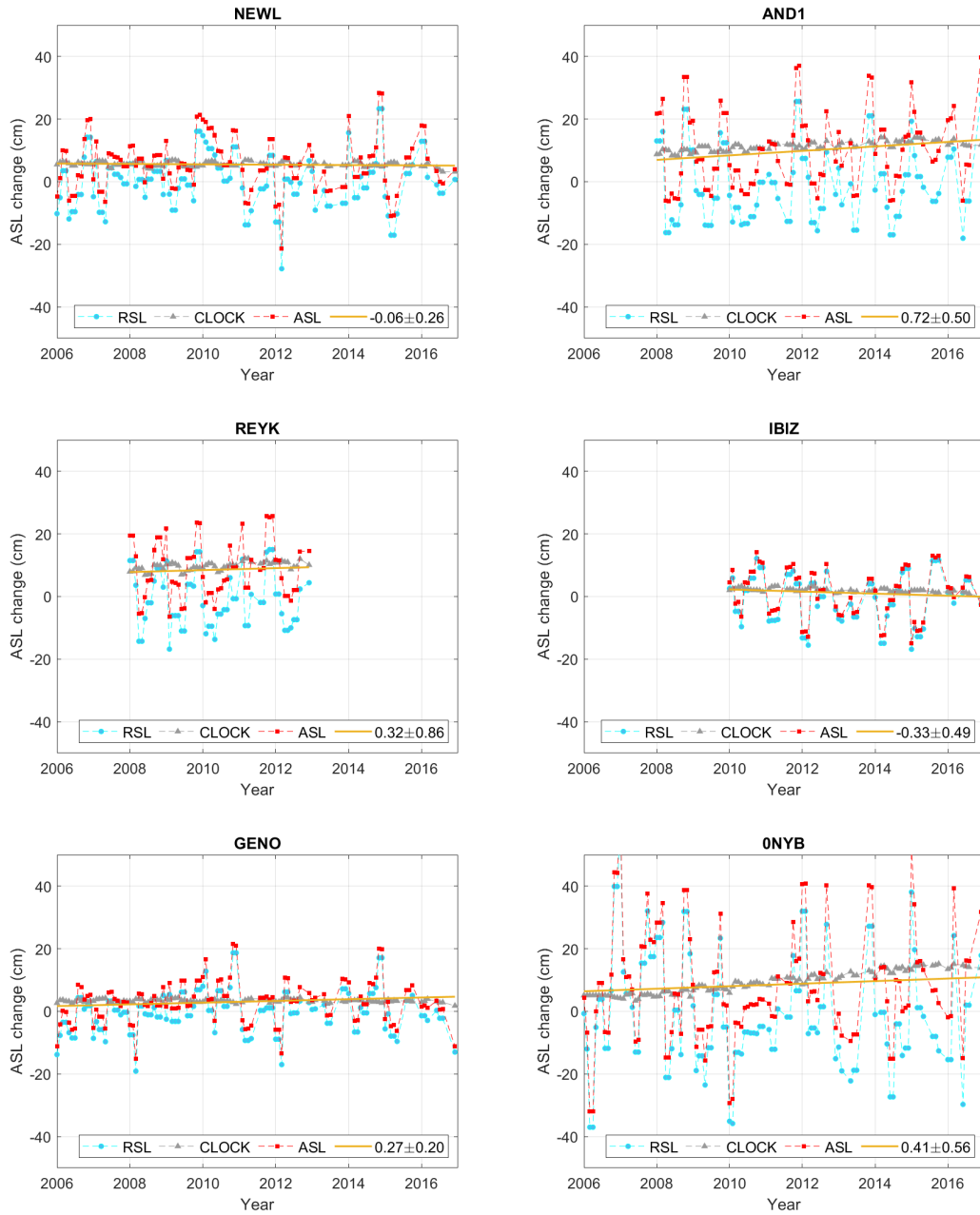
Figure 5.7: Estimated monthly ASL changes (ASL) by reducing the clock observations (CLOCK) from RSL changes (RSL) at the tide gauge sites. The long-term trends of ASL changes (cm/yr) are also given.
