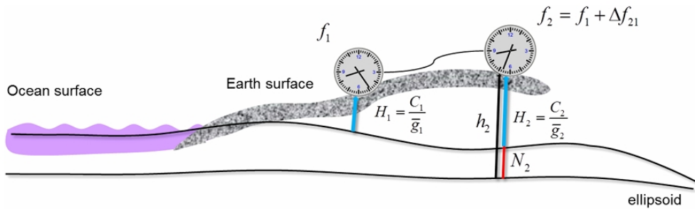
Figure 2.1: Relativistic geodesy with atomic clocks (Müller et al., 2018)
