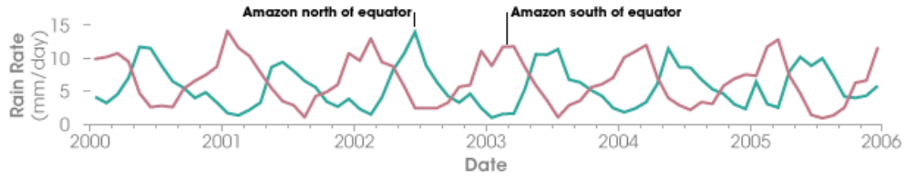
Figure 3.9: Rainfall variability in the north and south of the equator in the Amazon region. Image taken from NASA Earth Observatory (Lindsey, 2007)
