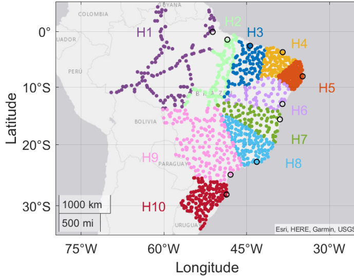
Figure 4.8: Classified Brazilian height system. The 10 generated LHSs: H1, H2, H3, H4, H5, H6, H7, H8, H9 and H10 are indicated in different colours. The tide-gauge locations for each LHS are indicated by black circles.
