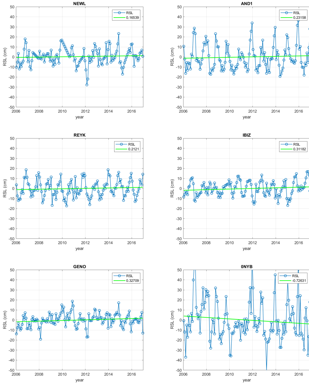
Figure 5.2: RSL change with the trend over the study period (10 years) at the selected clock sites.
