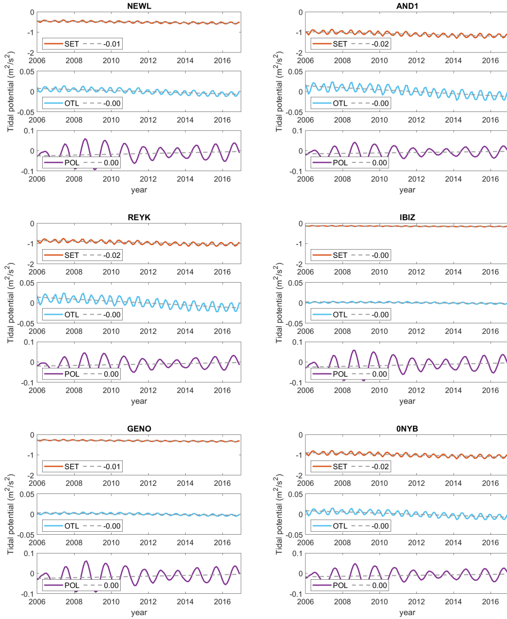
Figure 5.3: Monthly averages of solid-earth tides (SET), ocean-load tides (OTL) and pole tides (POL) with their linear trends at selected clock sites
