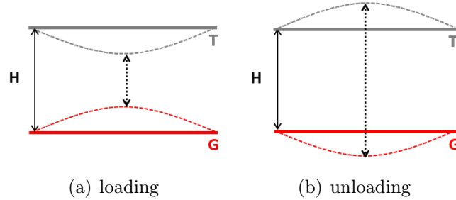
Figure 2.8: Loading and unloading effects on physical heights which depend on the geoid (G) height and vertical displacements of the Earth surface (T) (Vincent and Müller, 2024)
