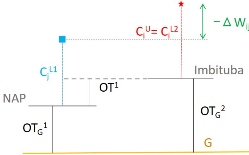
Figure 4.15: Unification to the global geoid using a single clock comparison \Delta W_{ij} between site i in Brazil (L2) and site j in Europe (L1).
