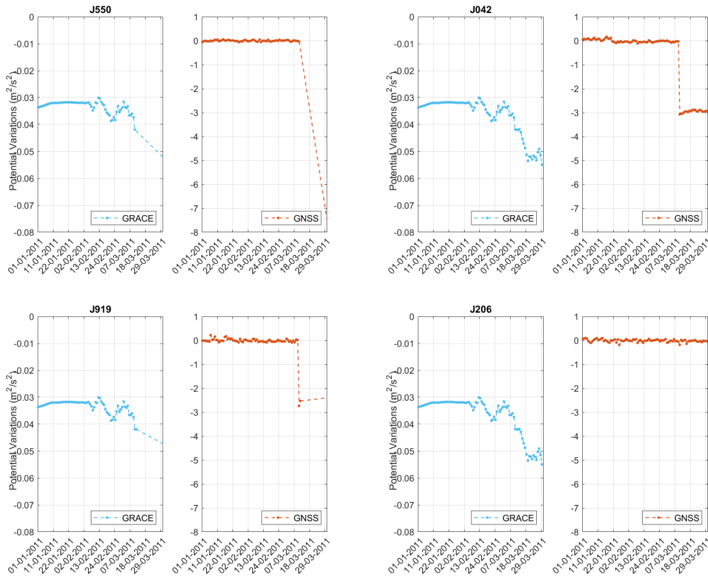
Figure 3.16: Daily potential variations separately derived from GRACE and GNSS in Japan at the sites J550, J042, J919 and J206 01.01.2011 till 30.03.2011.
