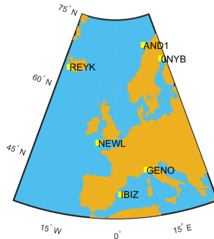
Figure 5.1: Tide-gauge locations considered in this study part: NEWL(Newlyn), AND1 (Andenes), REYK (Reykjavik), IBIZ (Ibiza), GENO (Genova), and, 0NYB (Kalix).
