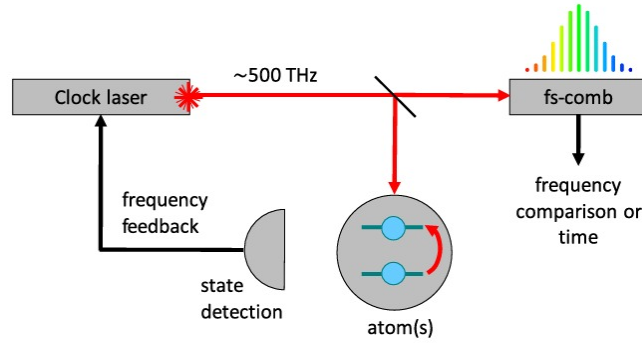
Figure 2.2: Schematic of an optical frequency standard (Mehlstäubler et al., 2018)
