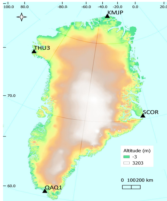
Figure 3.10: Simulated clock sites considered in Greenland
