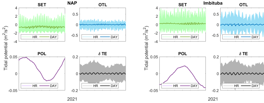
Figure 4.1: Hourly and daily potential variations due to solid earth tide (SET), ocean load tide (OTL) and pole tide (POL) with corresponding model error ( \delta TE ) at NAP, datum point of the European system (left) and the Imbituba, the datum point of Brazilian system (right).
