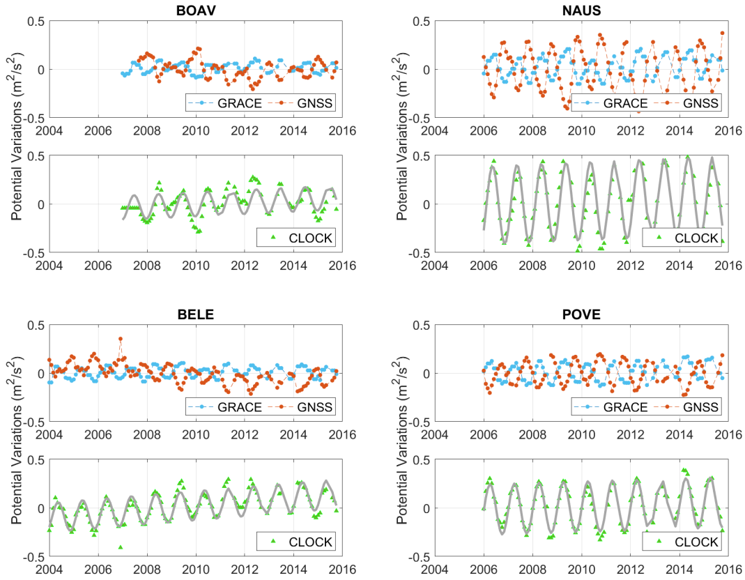
Figure 3.8: Simulated potential variations of hydrological signals at the Amazonian sites BOAV, NAUS, BELE and POVE. The upper panels show the variations separately derived from GRACE and GNSS. The lower panels show the combined effect of height change (GNSS) and mass change (GRACE) as it could be observed by clocks (CLOCK), with the fitted seasonal signal in gray.
