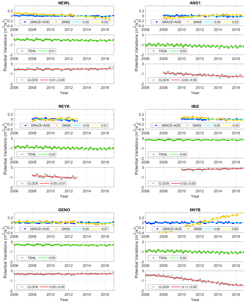
Figure 5.6: Simulated clock observations (CLOCK in each lower panel) by combining the potential variations due to non-tidal effects ( mass changes in TWS (GRACE), atmosphere and ocean (AOD) and associated vertical deformations (GNSS) in each upper panel) and tidal effects (TIDAL=SET+OTL+POL in each middle panel) with their linear trends ( \text{m}^2/\text{s}^2\text{yr} ) at the tide-gauge sites.
