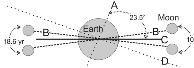
Figure 5.4: Illustration of the Earth's rotation (axis A), its orbit around the Sun (plane C), and the Moon's orbital plane (B) inclined by 5.14^\circ to the ecliptic. The lunar declination angle relative to Earth's equatorial plane (D) varies approximately 10^\circ between 18.18^\circ and 28.36^\circ over an 18.6-year period (Rochlin and Morris, 2017).
