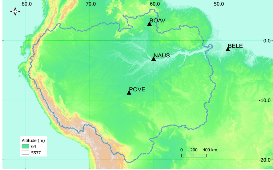
Figure 3.7: Simulated clock sites in the Amazon basin
