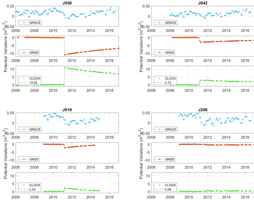
Figure 3.15: Effective potential variations in Japan at the sites J550, J042, J919 and J206 showcasing the pre-seismic, co-seismic and post-seismic effects related to the Tohoku earthquake in 2011. The upper panels show the variations separately derived from GRACE and GNSS. The lower panels show the combined effect of height changes (GNSS) and mass changes (GRACE) as it could be observed by clocks (CLOCK), with the mainshock's effective potential variation indicated.
