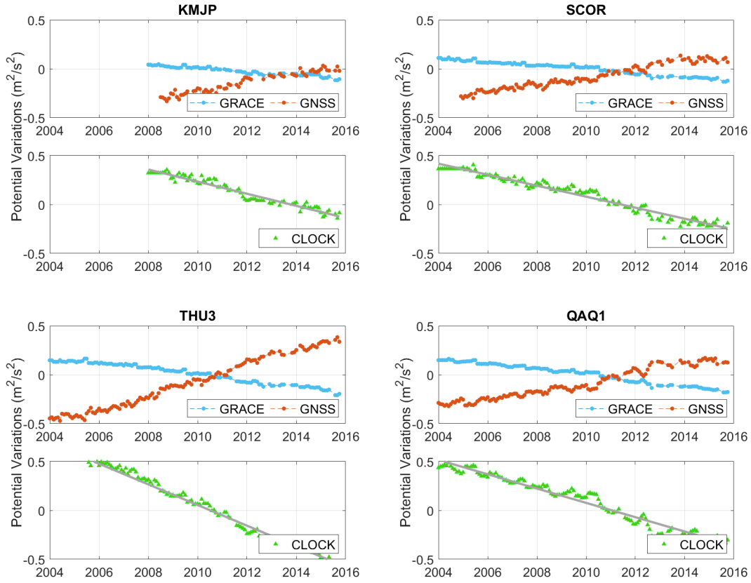
Figure 3.11: Linear potential variations over Greenland at sites KMJP, SCOR, THU3 and QAQ1. The upper panels show the variations separately derived from GRACE and GNSS. The lower panels show the combined effect of height changes (GNSS) and mass changes (GRACE) as it could be observed by clocks (CLOCK), with the fitted linear signal in gray.
