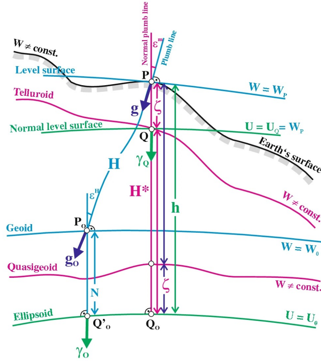
Figure 2.4: Heights and reference surfaces. (Sánchez et al., 2021)
