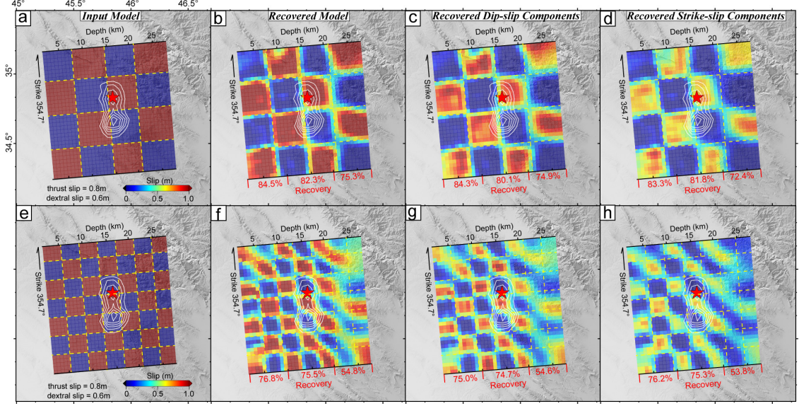
Figure 5.9: Checkerboard tests for the coseismic model resolution. Coarse (a) and fine (e) input models with 1-m slip are used for simulating synthetic surface displacements. The slip patterns (b and f), dip- (c and g) and strike-slip (d and h) components are recovered by the synthetic InSAR displacements.
