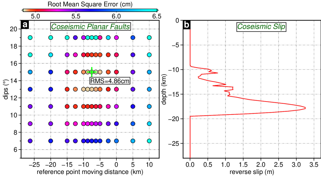
Figure 6.7: Searching results of planar fault geometry for coseismic kinematic models. The green plus sign indicates the best planar fault for coseismic deformation. The reference point on the initial fault derived from last chapter (Guo et al., 2022) with mesh coordinates (x, y) = (69.89 \text{ km}, -13.2 \text{ km}) is defined. (b) is the coseismic fault slip along depth.
