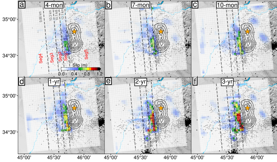
Figure 5.15: Spatiotemporal evolution of aftershocks and kinematic afterslip model. Black contours and orange star represent the coseismic slip model at 1-m intervals and the epicenter of the Mw 7.3 mainshock, respectively. The black dots indicated the aftershocks are from IRSC catalogue. The black dashed lines which divide the fault plane into 5 parts (seg 1-5) represent the fault depth.
