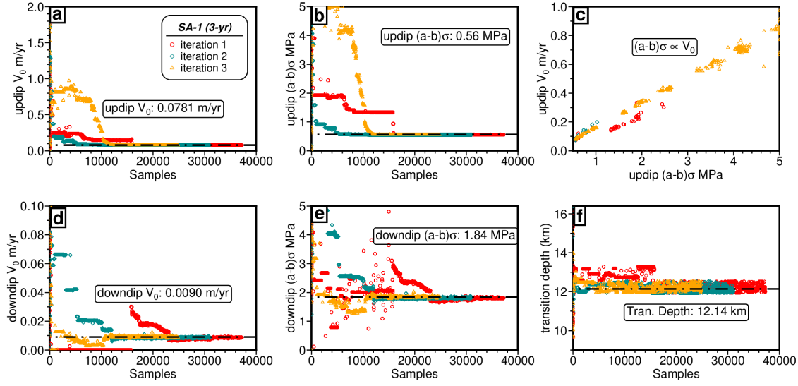
Figure 5.17: Convergence process with simulated annealing algorithms for V_0 and (a-b)\sigma updip (a and b) and downdip (d and e) of the coseismic rupture, as well as the transition depth (f), based on the 3-year postseismic deformation time series. The trade-off correlation between updip V_0 and (a-b)\sigma are shown in (c). The black dash-dotted line represents the optimal parameter.
