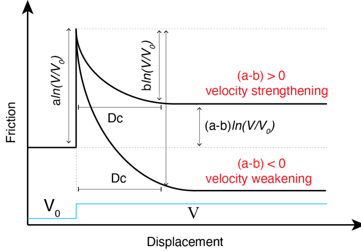
Figure 3.3: A schematic diagram illustrating the main features of rate-and-state friction in laboratory experiments.
