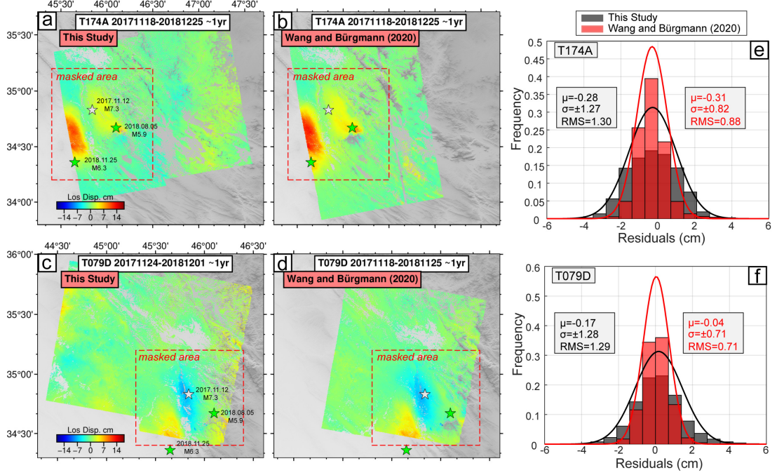
Figure 5.23: ~1-year cumulative postseismic LOS displacements of ascending track T174A (a and b) and descending track T079D (c and d) from our study and Wang and Bürgmann (2020). The red dashed boxes in (a-d) represent the masked areas with deformation fields. The residuals (e and f) are calculated from the non-deforming areas with T174A and T079D.
