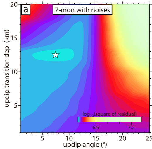
Figure 5.13: The results of searching the dip angles and transition depths of updip fault geometry with the 7-month observations perturbed with the Gaussian noises which are based on the standard deviations of far-field noises.
