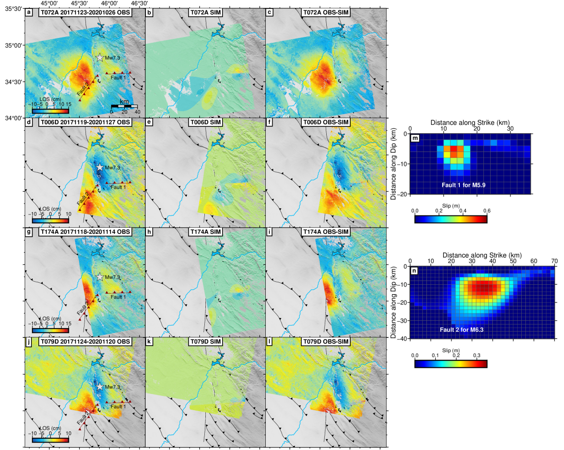
Figure 5.4: 3-year postseismic deformation of 2017 Sarpol-e Zahab earthquake for T072A, T006D, T174A and T079D (a, d, g, j); the simulated surface displacements of the Mw 5.9 and Mw 6.3 earthquake for T072A, T006D, T174A and T079D (b, e, h, k), which are from the fault models (m-n) proposed by Fathian et al. (2021); (c, f, i, l) are the cleaner results after the reducing of the simulations (b, e, h, k) from original observations (a, d, g, j). The gray star is the epicenter of the mainshock. The red faults (Fault 1 and Fault 2) are surface traces of fault models from Fathian et al. (2021).
