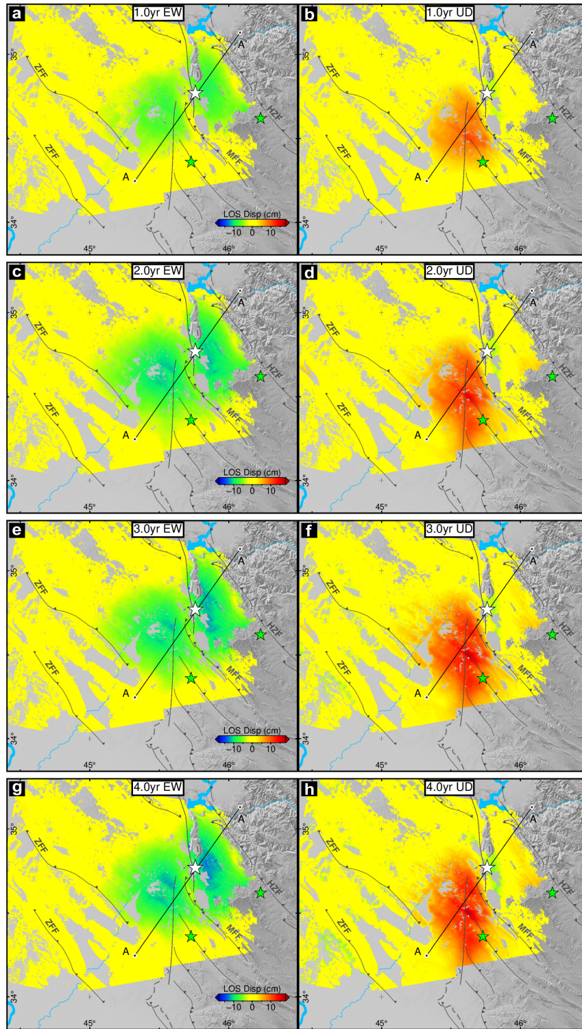
Figure 6.3: The 2.5D deformation (quasi-eastward (EW), eastward movement is positive; and quasi-upward (UD), upward movement is positive) fields 1 to 4 years after the mainshock decomposed from ascending Track T072A and descending Track T079D. The white and green stars are the mainshock and the two \sim M 6 aftershocks respectively.
