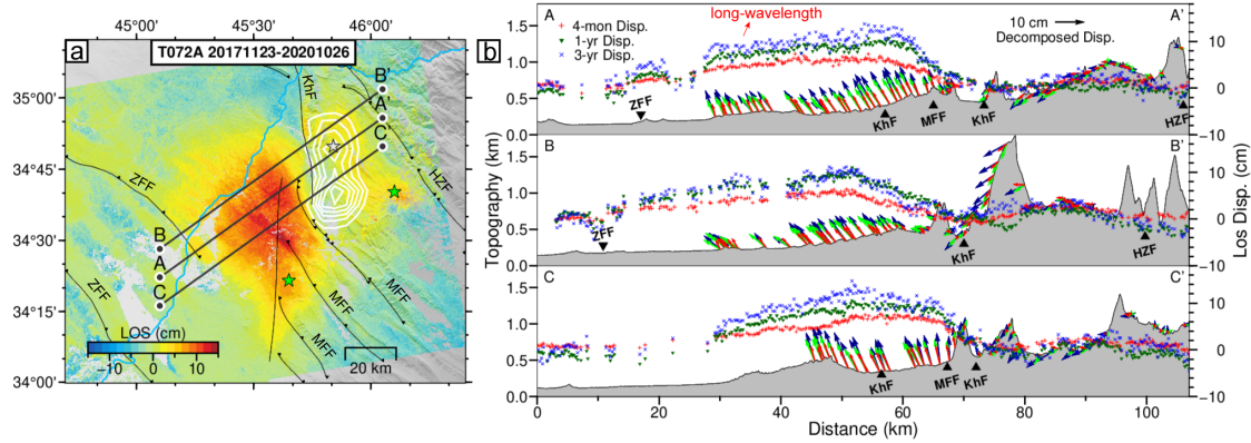
Figure 5.26: The contribution of postseismic deformation to topography. (a) \sim 3 -year cumulative postseismic deformation of ascending track T072A. White contours and gray star represent the coseismic slip model at 1-m intervals and the epicenter of the Mw 7.3 mainshock, respectively. The green stars are the two \sim M 6 aftershocks. (b) shows the contribution of postseismic deformation to topography along profile AA', BB' and CC' in (a). The red, green and dark blue vectors are the 2.5-dimension deformation (quasi-eastward and quasi-upward) of 4 months, 1 year and 3 years after the mainshock, separately, which are decomposed from ascending track T072A and descending track T079D.
