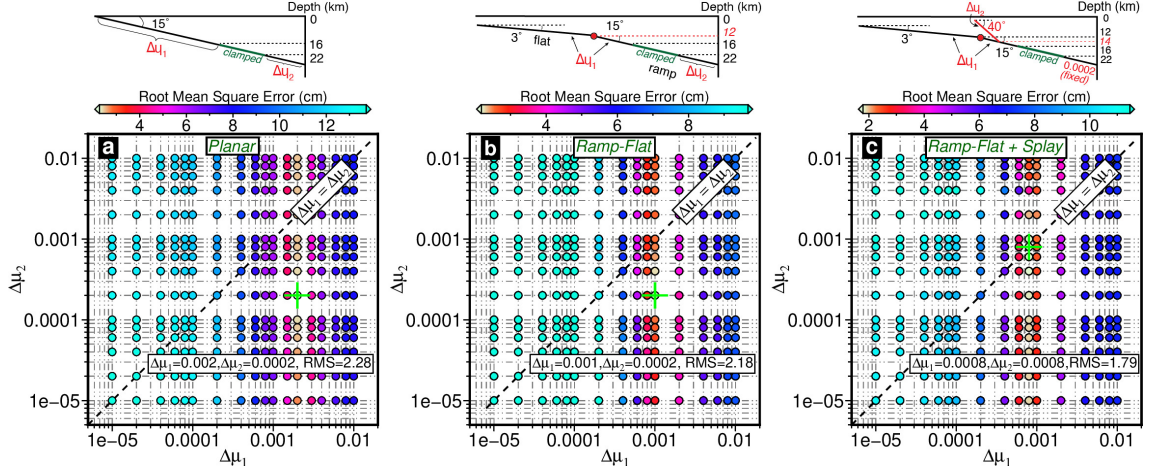
Figure 6.9: Optimal frictional strengthening search results for various best-constrained faults: (a) a planar fault, (b) a ramp-flat fault and (c) composite model with splay and ramp-flat faults. The green plus signs denote the best search results described in the white background text box.
