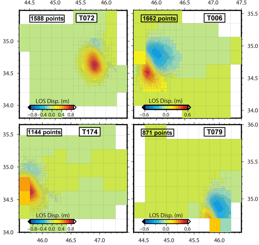
Figure 5.6: The downsampled points from 4-track coseismic interferograms with quadtree sampling approach (Jónsson et al., 2002), totally 5265 points.
