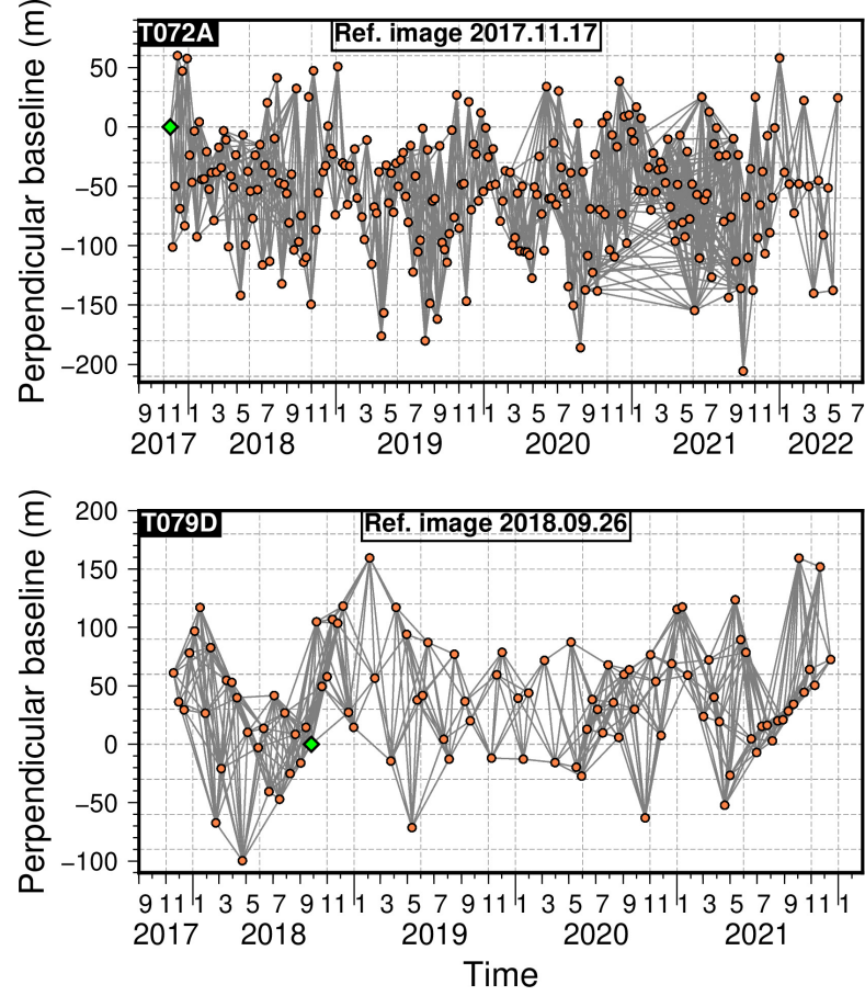
Figure 6.2: The baseline networks for the two sentinel-1 tracks (T072A and T079D). The green diamond represents the reference image.
