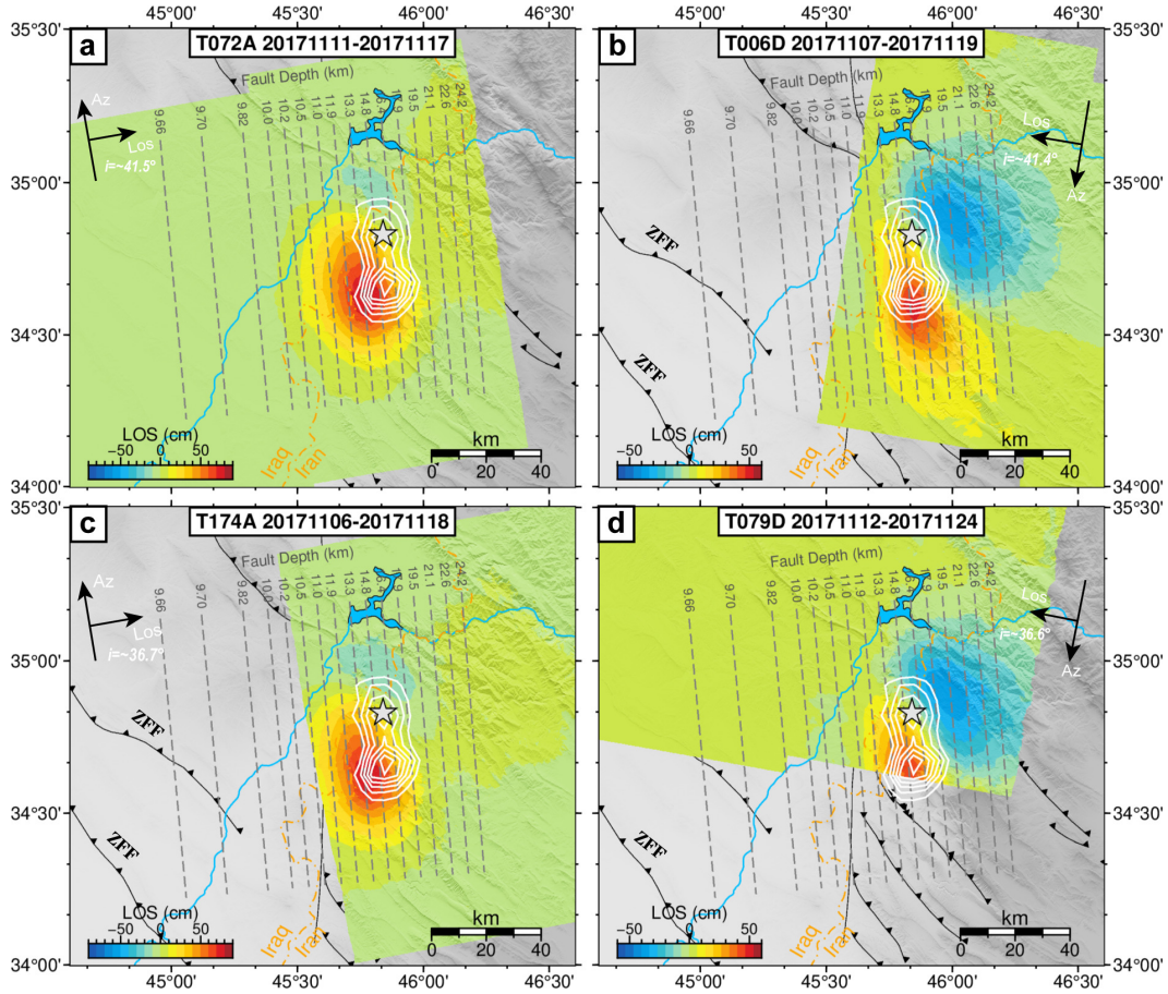
Figure 5.1: Coseismic interferograms from (a) T072A, (b) T006D, (c) T174A and (d) T079D of the 2017 Sarpol-e Zahab earthquake. Gray dashed lines represent the fault depth of the ramp-flat model. White contours and gray star represent our preferred coseismic slip model at 1-m intervals and the epicenter of the Mw 7.3 mainshock, respectively.
