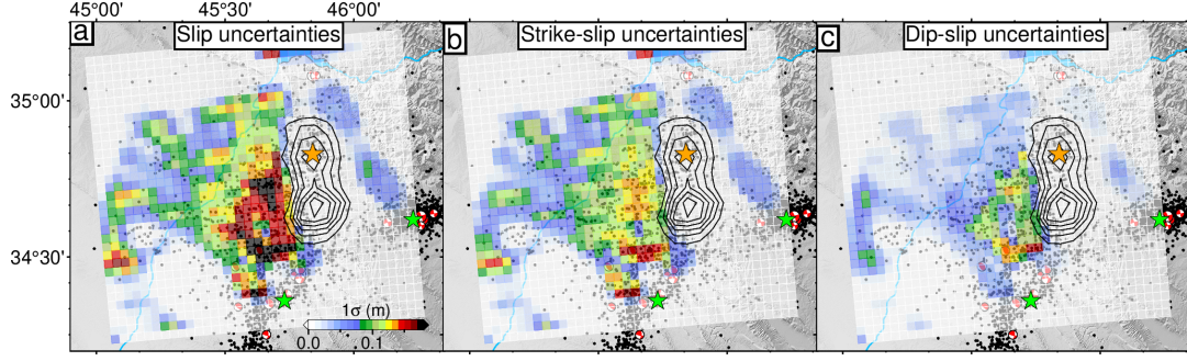
Figure 5.24: Standard deviation calculated with 100 perturbed datasets to simulate the influence of observation noises to model slip. (a), (b) and (c) are the total slip uncertainties, strike- and dip-slip uncertainties, respectively. Black contours and orange star represent the coseismic slip model at 1-m intervals and the epicenter of the Mw 7.3 mainshock, respectively. Green stars represent the locations of the two \sim M 6 aftershocks. The black dots and red beach balls indicated the aftershocks are from IRSC catalogue.
