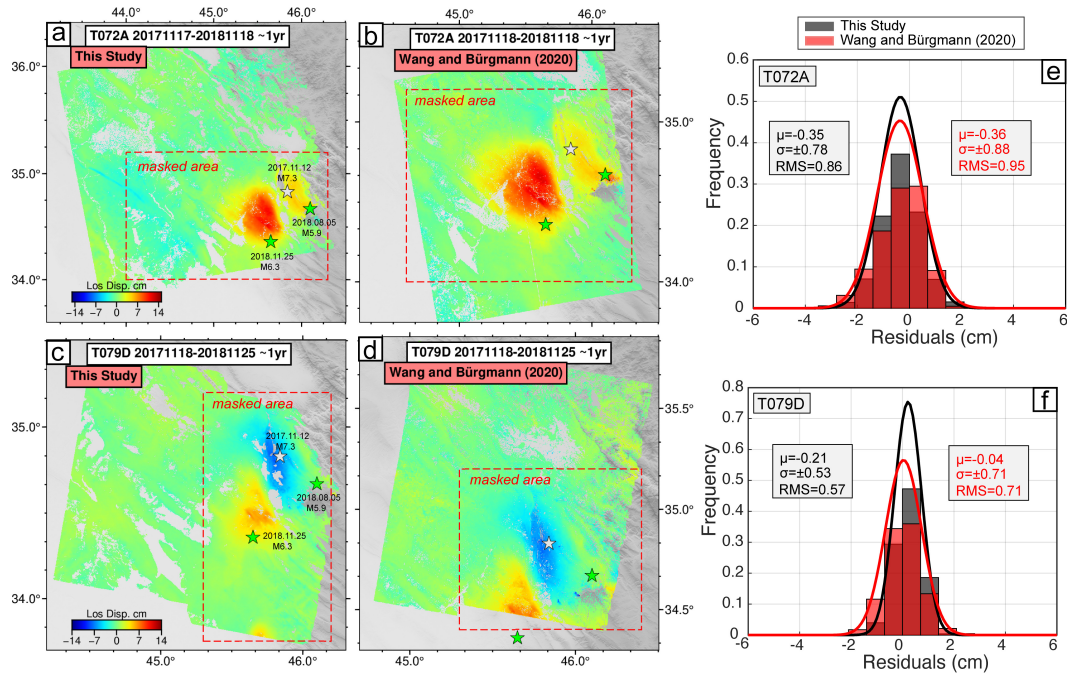
Figure 6.15: ~1-year cumulative postseismic LOS displacements of ascending track T072A (a and b) and descending track T079D (c and d) from our study and Wang and Bürgmann (2020). The red dashed boxes in (a-d) represent the masked areas with deformation fields. The residuals (e and f) are calculated from the non-deforming areas with T072A and T079D.
