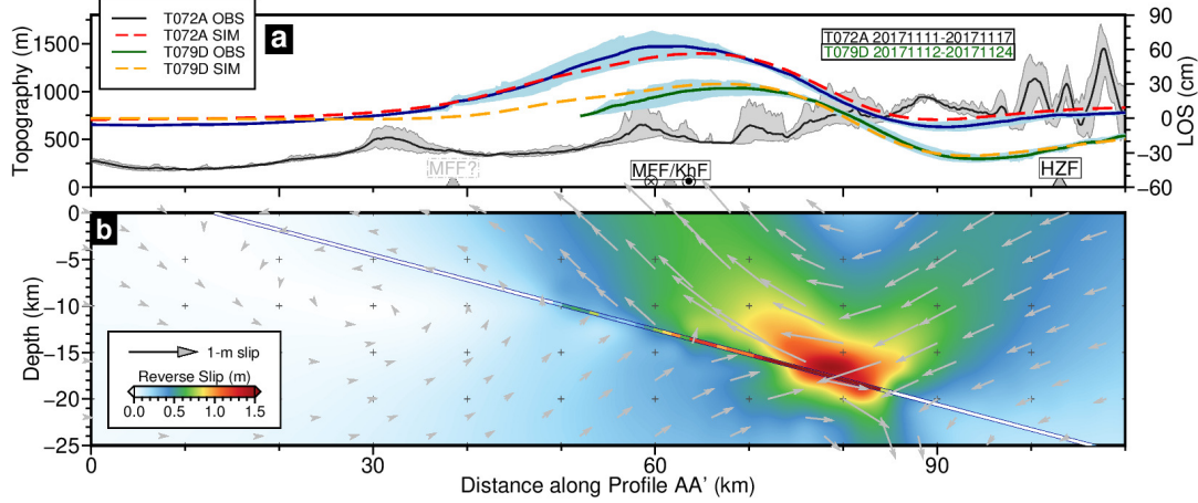
Figure 6.8: Kinematic models and simulations based on planar faults for coseismic deformation along profile the AA'. (a) coseismic InSAR observations and simulations based on the (b) coseismic slip model which is from the best searching result of Figure 6.7. The envelope curves of the InSAR observations and topography (gray) in (a) indicate the minimum, maximum and mean value of the swath with width of 8 km.
