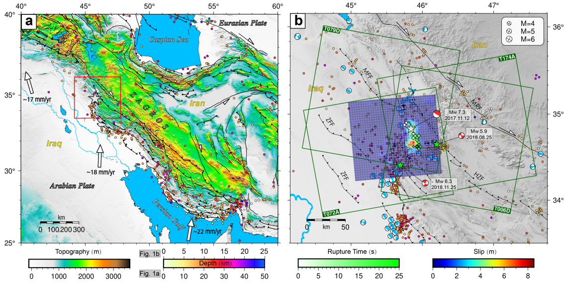
Figure 4.1: Tectonic background of the 2017 Sarpol-e Zahab earthquake. (a) The colored dots are earthquakes (from 1976 to 2021) from the Global Centroid Moment Tensor (GCMT) catalog ( https://www.globalcmt.org ). The red box indicates the area of figure b. (b) Detailed tectonic map of the seismogenic area. The blue beach balls are from the GCMT catalog. Colored dots are earthquakes (from 2006 to 2021 with M > 3.5 ) from the Iranian Seismological Center (IRSC, http://irsc.ut.ac.ir ). Dark green boxes indicating the spatial extent of Sentinel-1 imagery and the coseismic slip distribution are from Guo et al. (2022). Black beach balls are from Nissen et al. (2019). Red beach balls are the focal mechanisms of the 2017 Sarpol-e Zahab mainshock and two \sim M 6 aftershocks. The green rhombuses represent the rupture time of the mainshock, which is mapped from Nissen et al. (2019).
