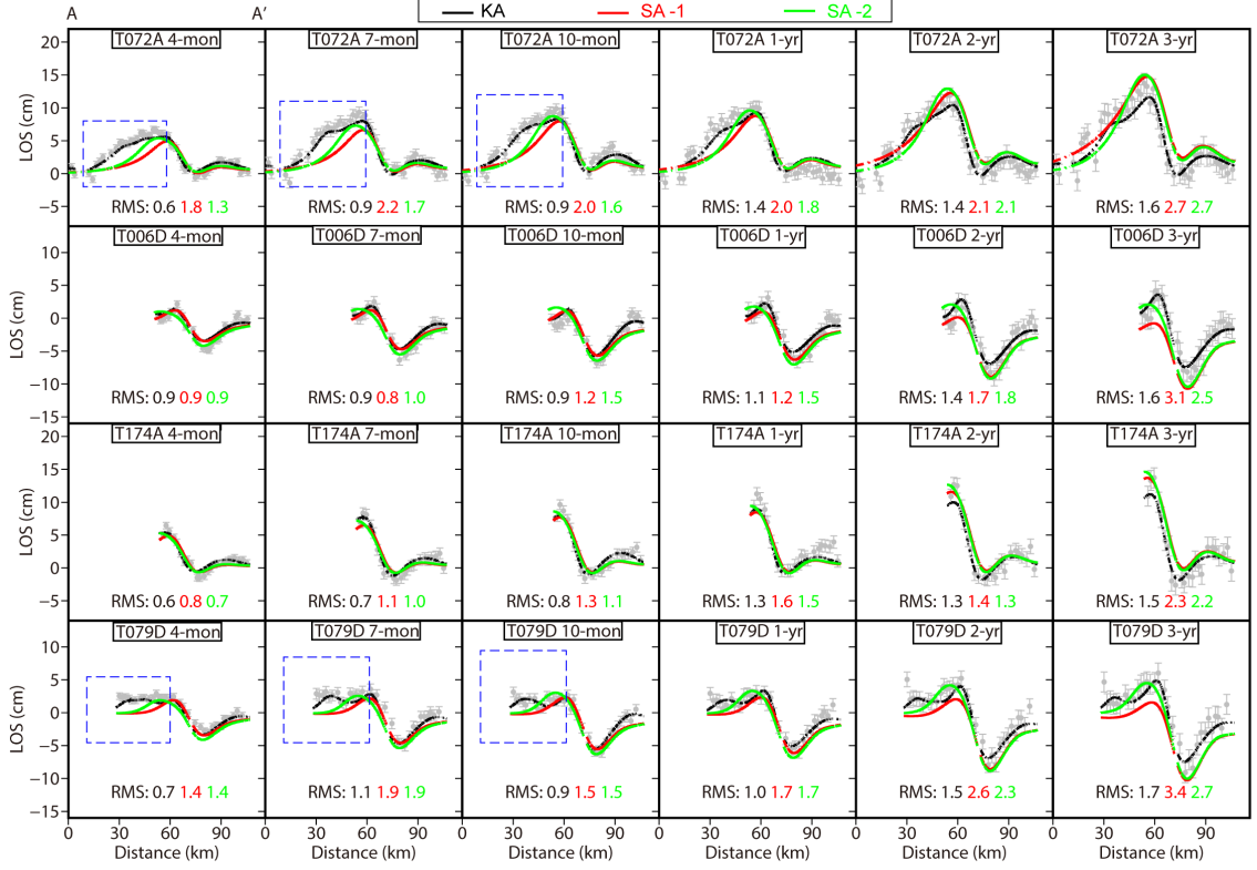
Figure 5.16: Fitting between InSAR observations and simulations from 4 months to 3 years after the mainshock along profile AA' in Figure 5.3a-d. The gray error bars are based on the InSAR observations, which represent the far-field noises from VCM. The black, red and green lines represent the simulations from Kinematic Afterslip (KA) and Stress-driven Afterslip model 1 (SA-1 model) and Stress-driven Afterslip model 2 (SA-2 model), respectively. The blue dashed boxes indicate the underfitting between observations and simulations from stress-driven afterslip models.
