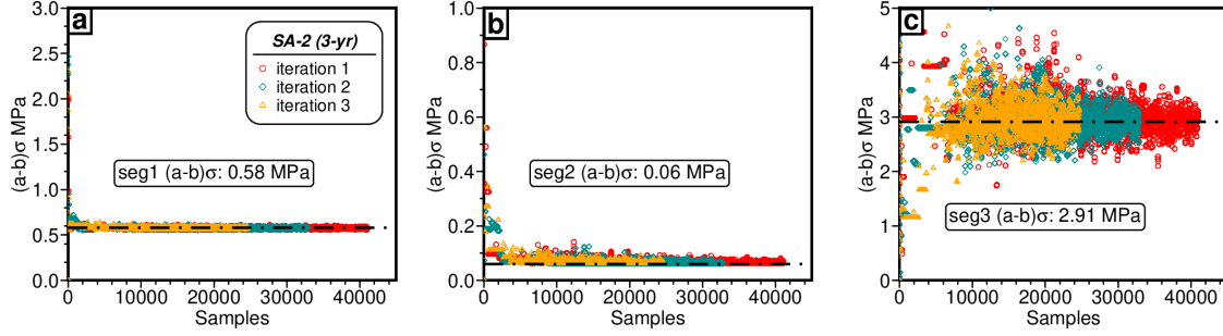
Figure 5.20: Convergence process with simulated annealing algorithms for (a - b)\sigma of seg 1-3 updip of the coseismic rupture. The black dash-dotted line represents the optimal parameter.
