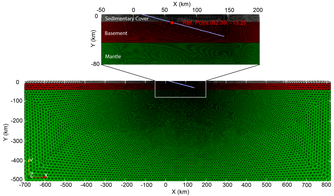
Figure 6.6: An example of a 2D mesh showing a planar fault dipping 15^\circ , with the mesh coordinates of reference point (62.39 km, -13.2 km). The reference point in this mesh is horizontally moved 7.5 km to the left (west) from the original reference point (69.89 km, -13.2 km).
