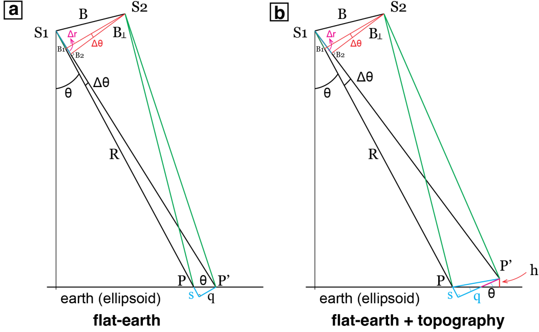
Figure 2.3: InSAR phase variation between two targets ( P and P' ) and satellites ( S1 and S2 ) with (a) flat earth and (b) topographic effects. R represents the slant range between the satellite and the ground target. The distance between SAR satellites S1 and S2 is baseline B , while B_{\perp} represents the component perpendicular to the slant range direction. q and s are the distances between P and P' that are perpendicular and parallel to the slant range direction, respectively. This figure is modified from Lu and Dzurisin (2014).
