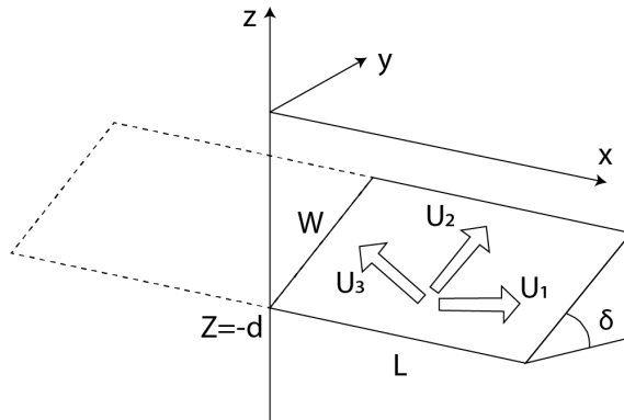
Figure 3.1: Geometry of Okada source model.
