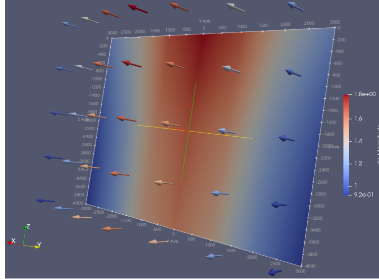
Figure 3.5: Fault slip magnitude based on second example using PyLith software.
