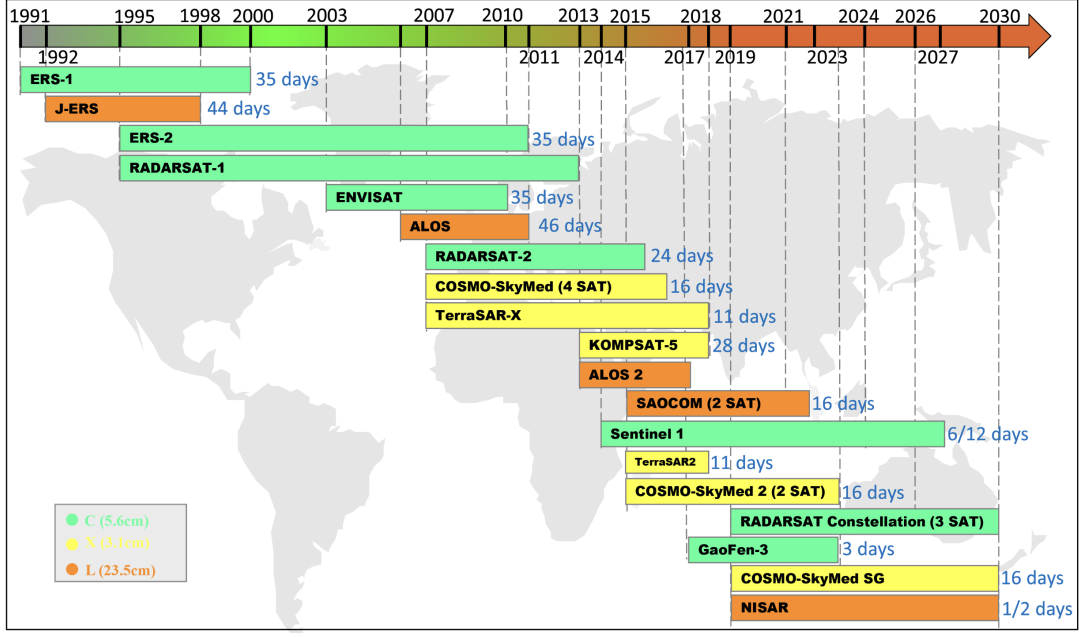
Figure 2.2: Part of past, current and upcoming spaceborne SAR missions, the duration at the end of each mission (days) is the repeat cycle of the satellites.
