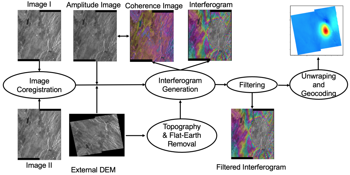
Figure 2.5: A simplified DInSAR data processing flowchart to get the coseismic deformation field of this 2017 Mw 7.3 Sarpol-e Zahab earthquake using a ascending Sentinel-1 image (T072A).
