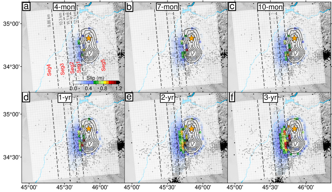
Figure 5.19: Similar to SA-1 model in Figure 5.18, this is the spatiotemporal evolution of aftershocks and stress-driven afterslip model 2 (SA-2 model).
