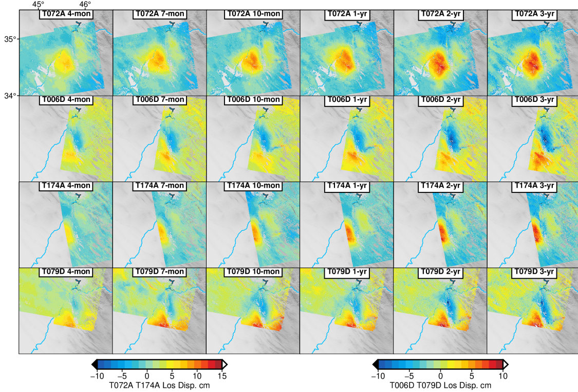
Figure 5.5: InSAR time series of T072A, T006D, T174A and T079D after reducing the coseismic deformation of the 25 August 2018 Mw 5.9 and 25 November 2018 Mw 6.3 earthquake. Please note the different color bars of ascending and descending tracks.
