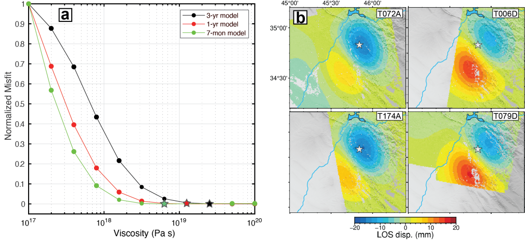
Figure 5.21: Searching result of viscosity and the corresponding simulations due to viscoelastic relaxation. (a) The trade-off between normalized misfit of 7-month, 1-year and 3-year postseismic observations and the viscosities. The green, red and black stars represent the best viscosity based on 7-month, 1-year and 3-year postseismic observations. (b) The simulated LOS displacements of T072A, T006D, T174A and T079D due to the viscoelastic relaxation 3 year after the mainshock, using a layer model with the best estimates of the rheological viscosity from Lv et al. (2020). The viscoelastic simulations are similar to the results of Wang and Bürgmann (2020). The viscosities of Maxwell lower crust between 30 km to 40 km and Maxwell upper mantle lower than 40 km are 1 \times 10^{19} and 3 \times 10^{19} Pa s, respectively. The gray star is the epicenter of the 2017 Sarpol-e Zahab earthquake.
