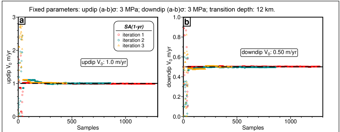
Figure 5.27: Convergence process with simulated annealing algorithms for updip and downdip of the fault with fixed constitutive parameters (a-b)\sigma and the transition depth, based on the simulations perturbed with observation noises. The black dash-dotted line represents the optimal parameter.
