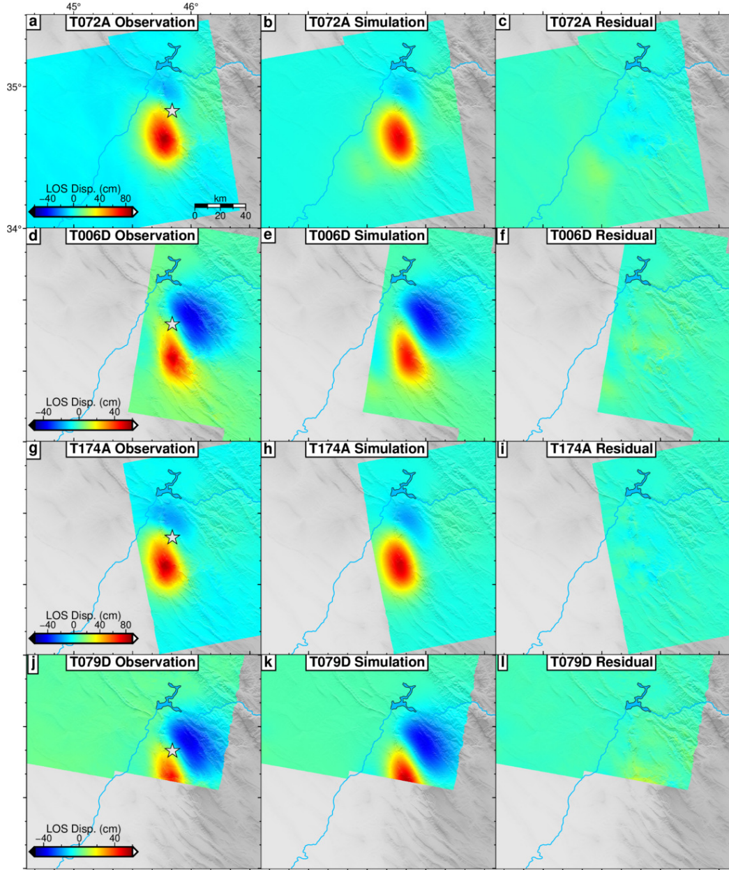
Figure 5.8: The observations (first column), simulations (second column) and residuals (third column) of T072A (a-c), T006D (d-f), T174A (g-i) and T079D (j-l) based on the coseismic model. The gray star is the epicenter of the mainshock.
