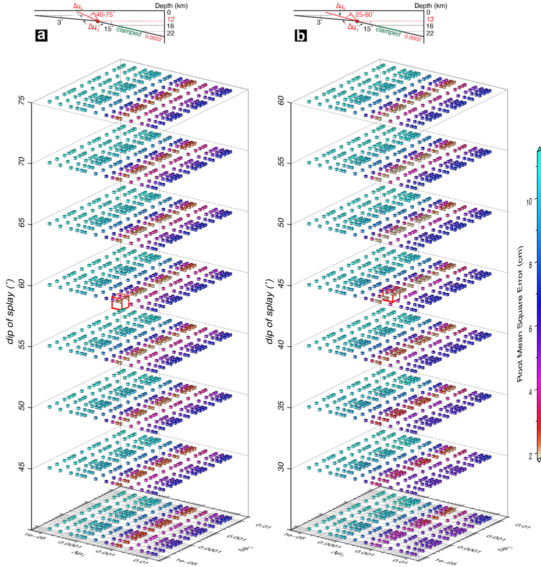
Figure 6.12: Searching results between dip angles of splay fault and the friction coefficients of the updip flat and the splay fault. The rooting depths of the splay faults are (a) 12 km and (b) 13 km, respectively. The red cubes indicate the best searching results. The best results for (a) are \Delta\mu_1 = 0.001 , \Delta\mu_2 = 0.00001 and the RMS error of 1.93 cm with a splay fault dipping 60°; for (b) are \Delta\mu_1 = 0.0008 , \Delta\mu_2 = 0.00004 and the RMS error of 1.88 cm with a splay fault dipping 45°.
