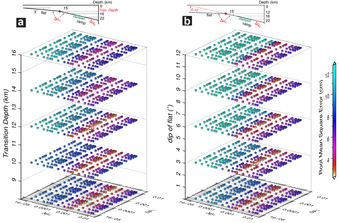
Figure 6.11: (a) Searching results between transition depths and the friction coefficients up- and down-dip of coseismic rupture, based on ramp-flat faults. The red cube indicates the best result (with RMS error of 2.18 cm) in which \Delta\mu_1 = 0.001 , \Delta\mu_2 = 0.0002 for the up- and down-dip segments of the fault, respectively, the transition depth between the up- and down-dip portions is 12 km. (b) Searching results between dip angles of flat portion and the friction coefficients up- and down-dip of coseismic rupture, based on ramp-flat faults. The red cube indicates the best result (with RMS error of 2.18 cm) in which \Delta\mu_1 = 0.001 , \Delta\mu_2 = 0.0002 for the up- and down-dip segments of the fault, respectively, the dip angle of the updip flat is 3°.
