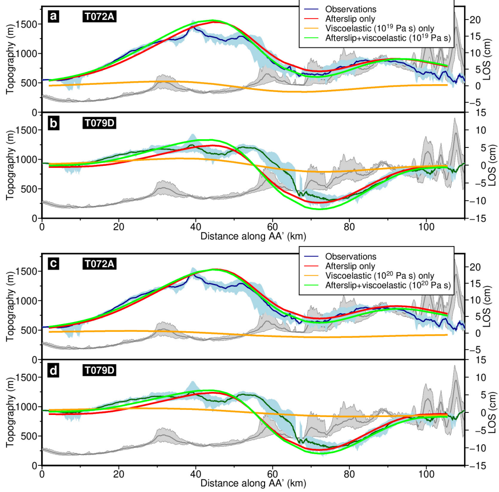
Figure 6.14: The comparisons between InSAR observations, afterslip and viscoelastic simulations. Different viscosities 1 \times 10^{19} (a and b) and 1 \times 10^{20} Pa S (c and d) between 25-45 km in the lower crust are tested based on the ramp-flat fault.
