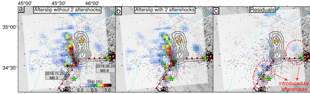
Figure 5.22: \sim 3-year kinematic afterslip models after (a) and before (b) removing the coseismic deformation of the two \sim M 6 aftershocks; (c) the difference between (a) and (b). Black contours and orange star represent the coseismic slip model at 1-m intervals and the epicenter of the Mw 7.3 mainshock, respectively. Green stars and dark red faults represent the locations of the two bigger aftershocks and the corresponding fault traces from Fathian et al. (2021). The black dots and red beach balls indicated the aftershocks are from IRSC catalogue.
