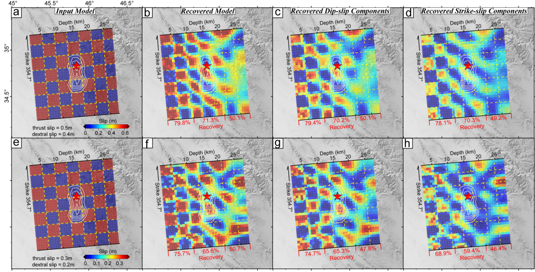
Figure 5.25: Checkerboard tests for the postseismic model resolution. The input models with \sim 0.6 -m (a) and \sim 0.4 -m (e) slip are used for simulating synthetic surface displacements. The slip patterns (b and f), dip- (c and g) and strike-slip (d and h) components are recovered by the synthetic InSAR displacements. The recovery is defined as \text{recovery} = \left(1 - \frac{\sum_{i=1}^n |S_i - S'_i|}{\sum_{i=1}^n |S_i|}\right) \times 100\% , where S_i and S'_i represent the input slip and inverted slip of i_{th} patch, respectively, and the n is the number of patches with input slip.
