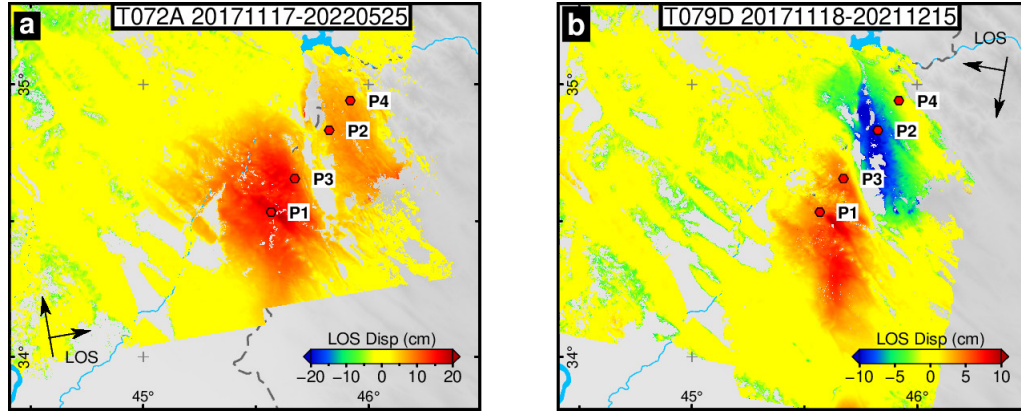
Figure 6.4: The selected points of (a) T072A and (b) T079D along Profile AA', which are used for plotting the InSAR time series in Figure 6.5.
