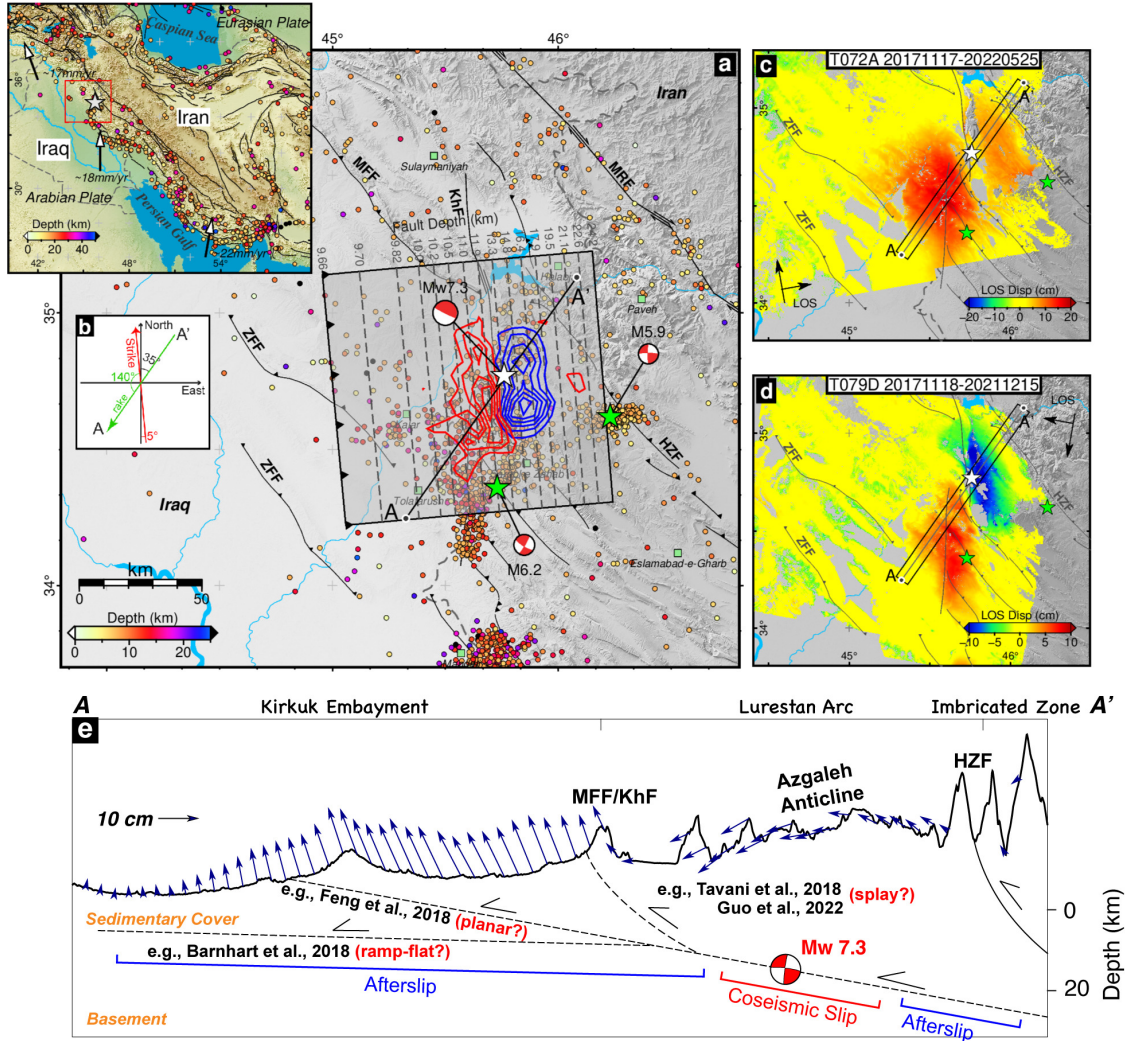
Figure 6.1: Tectonic background and the InSAR results of the 2017 Mw 7.3 Sarpol-e Zahab earthquake, postseismic InSAR observations and conceptual faults derived and modified from previous studies. (a) tectonic setting of the mainshock. The finite element method models used in this study are constructed along profile AA'. The white and green stars are the mainshock and the two ~M 6 aftershocks respectively. The black box represents the ramp-flat fault plane proposed by our previous study (Guo et al., 2022). The blue and red contours with 1- and 0.2-m intervals indicate the coseismic slip and cumulative 3-year kinematic afterslip from Guo et al. (2022), respectively. The colored dots are the earthquakes (from 2006 to 2022) from IRSC with magnitudes larger than M 3. (b) is a schematic diagram showing the strike direction and slip direction of the fault proposed by our previous work (Guo et al., 2022). (c) is the ~4.5-year cumulative postseismic deformation of ascending track T072A. (d) is same with (c) but it shows a descending track T079D. (e) indicates the conceptual faults derived and modified from previous studies, including planar fault (e.g., Feng et al., 2018), ramp-flat fault (e.g., Barnhart et al., 2018; Wang and Bürgmann, 2020) and splay fault (e.g., Tavani et al., 2018). The dark blue vectors are the 2.5-dimension deformation 4 years after the mainshock, which are decomposed from ascending Track T072A and descending Track T079D. The width of the swath in (c) and (d) is 8 km. The red beach balls are the focal mechanisms of the 2017 Mw 7.3 mainshock and two ~M 6 aftershocks. ZFF: Zagros Foredeep Fault; MRF: Main Recent Fault; HZF: High Zagros Fault; and MFF: Mountain Front Fault; KhF: Khanaqin fault.
