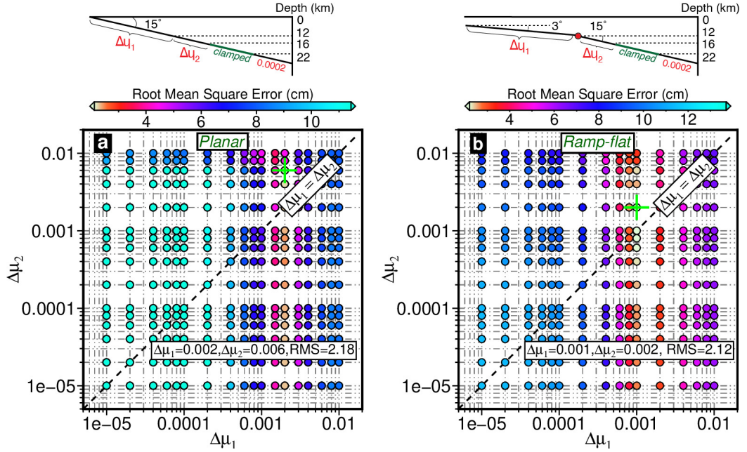
Figure 6.17: Searching results of friction heterogeneity based on the three-segment planar and ramp-flat faults in which the friction variation of the downdip portion is fixed as 0.0002. (a) planar fault and (b) ramp-flat fault. The green plus signs denote the best search results described in the white background text box.
