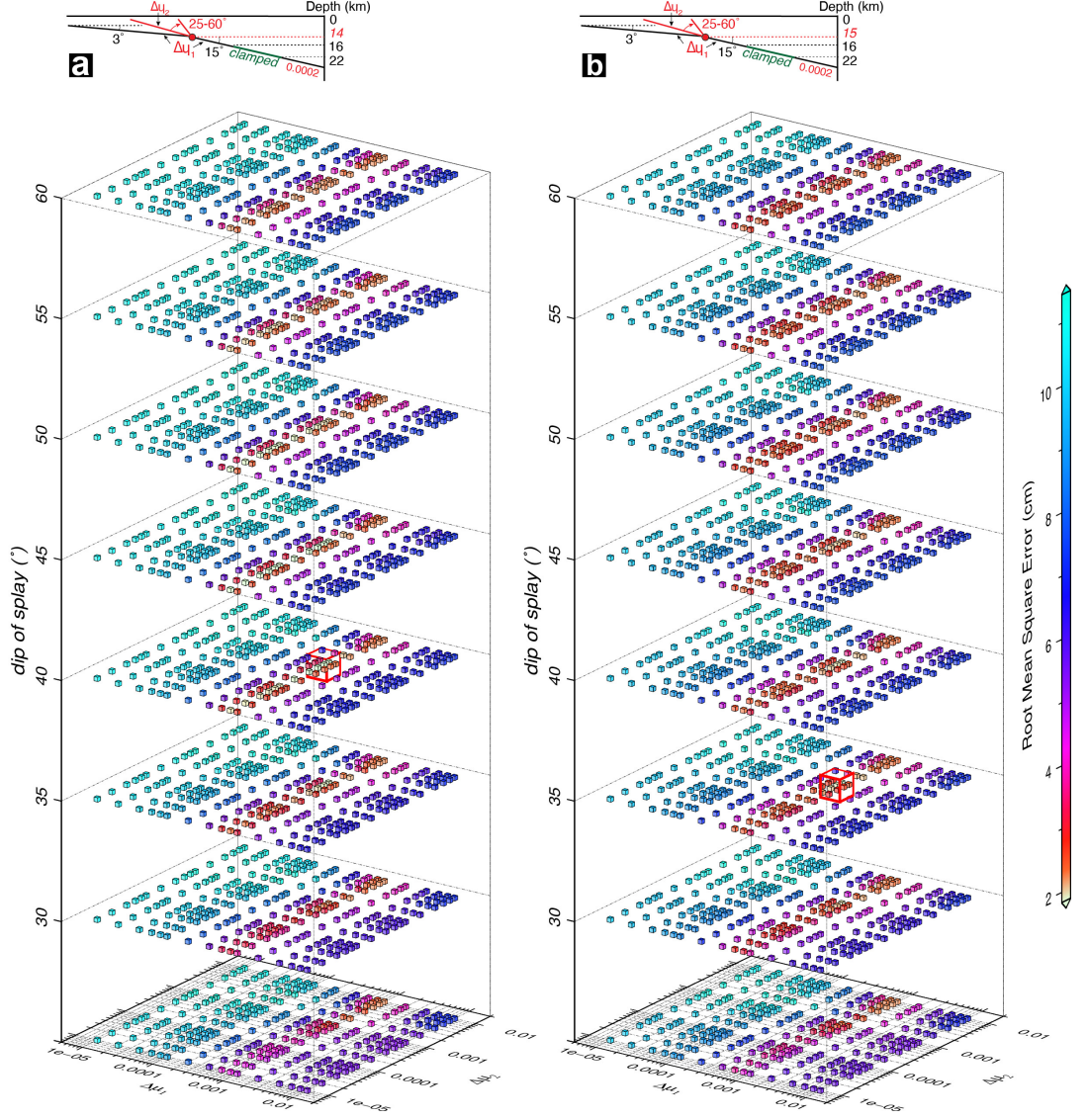
Figure 6.13: Same to Figure 6.12 but the rooting depths of the splay faults are (a) 14 km and (b) 15 km, respectively. The red cubes indicate the best searching results. The best results for (a) are \Delta\mu_1 = 0.0008 , \Delta\mu_2 = 0.0008 and the RMS error of 1.79 cm with a splay fault dipping 40^\circ ; for (b) are \Delta\mu_1 = 0.0008 , \Delta\mu_2 = 0.001 and the RMS error of 1.81 cm with a splay fault dipping 35^\circ .
