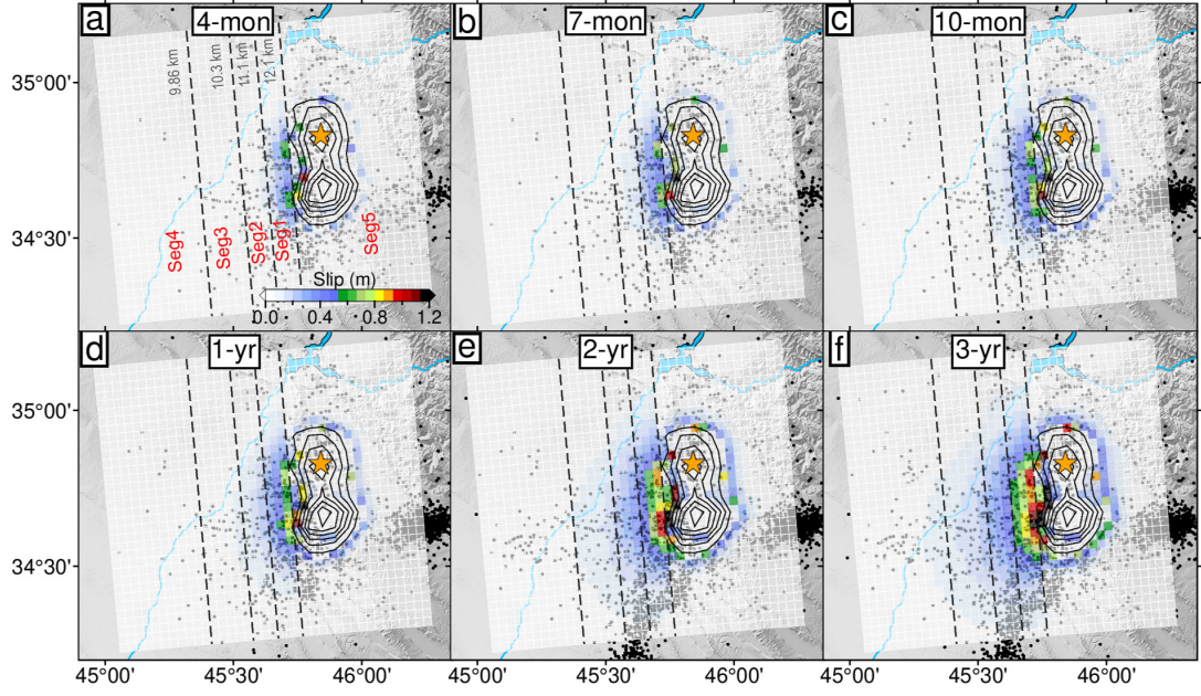
Figure 5.18: Spatiotemporal evolution of aftershocks and stress-driven afterslip model 1 (SA-1 model). Black contours and orange star represent the coseismic slip model at 1-m intervals and the epicenter of the Mw 7.3 mainshock, respectively. The black dots indicated the aftershocks are from IRSC catalogue. The black dashed lines which divide the fault plane into 5 parts (seg 1-5) represent the fault depth.
