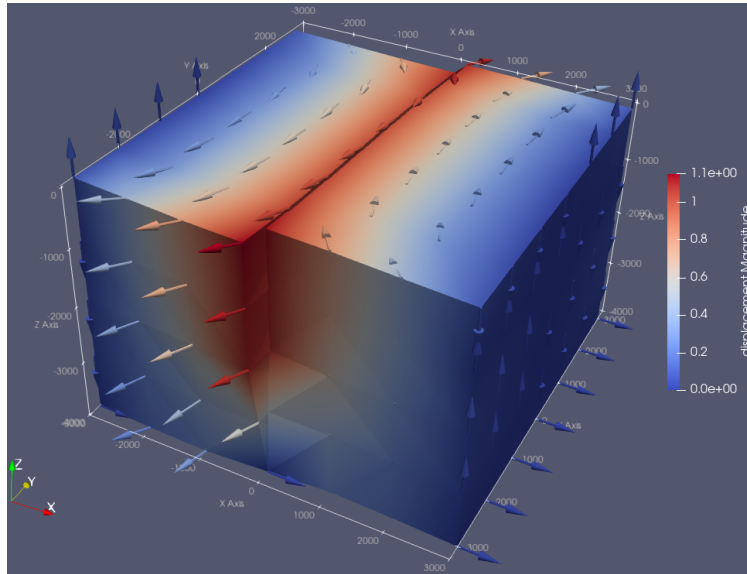
Figure 3.4: Displacement magnitude based on first example using PyLith software.
