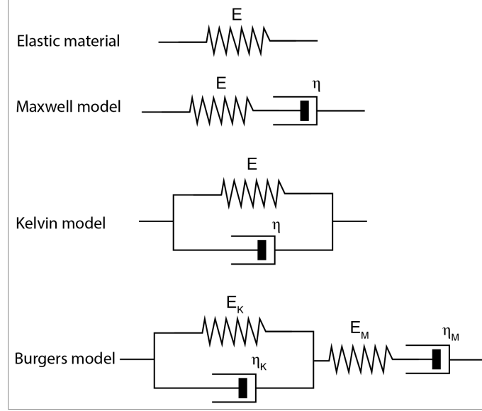
Figure 3.2: Various models of elastic and non-elastic deformation. E and \eta represent Young's modulus and viscosity coefficient, respectively.
