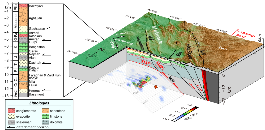
Figure 5.29: 3-D block diagram showing the tectonics, fault geometry, kinematic afterslip of 3 years after the mainshock and stratigraphic column in northwestern Zagros. The geological cross-section data is from National Iranian Oil company. The GPS velocity (SAGZ site) is from Khorrami et al. (2019). The simplified stratigraphic profile with approximate depths for Lurestan Salient is modified and referred from previous studies: Casciello et al. (2009); Vergés et al. (2011); Sadeghi and Yassaghi (2016); Le Garzic et al. (2019). Red star represents the epicenter of the 2017 Sarpol-e Zahab earthquake. Stratigraphy ages and main faults are abbreviated as follows: Plio, Pliocene; O-Pa, Oligocene-Eocene-Palaeocene; K, Cretaceous; J, Jurassic; Tr, Triassic; P, Permian; Or-Ca, Ordovician-Cambrian; PreC, PreCambrian; MRF: Main Recent Fault; HZF: High Zagros Fault; MFF: Mountain Front Fault.
