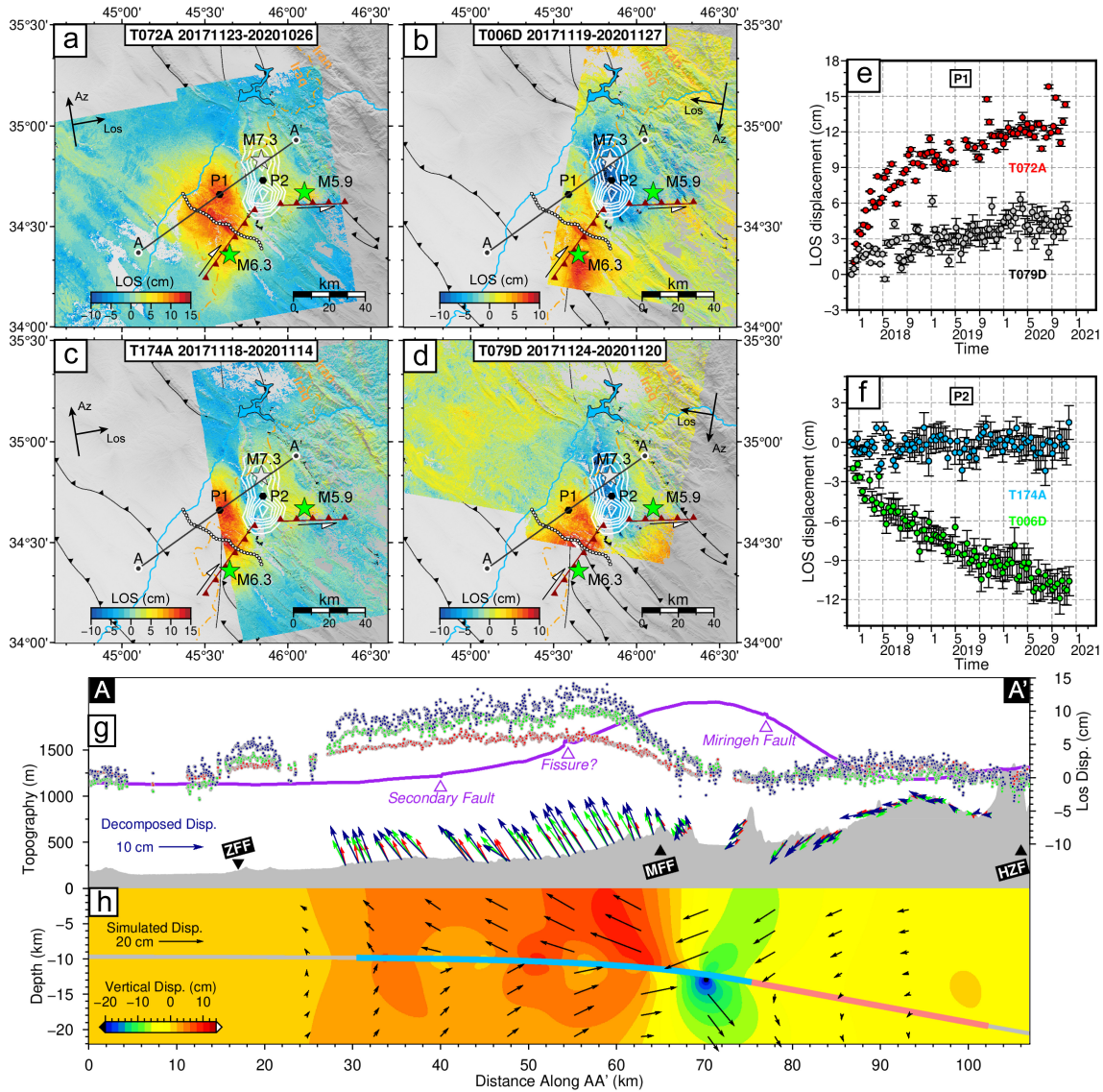
Figure 5.3: Postseismic InSAR observations. (a-d) represent the \sim 3 -year cumulative postseismic LOS displacements of T072A, T006D, T174A and T079D, respectively. White contours and gray star represent our preferred coseismic slip model at 1-m intervals and the epicenter of the Mw 7.3 mainshock, separately. Green stars and dark red faults represent the locations of the two bigger aftershocks and the corresponding fault traces from Fathian et al. (2021). White dots (black outline) are the surface trace of the secondary fault indicated by the coseismic interferogram discontinuity and field survey (Vajedian et al., 2018). Profile AA' which is nearly orthogonal to the geological structures corresponds to the surface observations and simulations of Figure 5.16. (e-f) are the LOS displacement time series of P1 and P2, respectively, the error bars are the standard deviations from pixels within a radius of 30 meters. (g) shows the contribution of postseismic deformation to topography along profile AA'. The red, green and dark blue dots represent the postseismic LOS displacements of 4 months, 1 year and 3 years after the mainshock, respectively. The purple line indicates the coseismic LOS displacements which are scaled by a factor of 5. The red, green and dark blue vectors are the 2.5-dimension deformation (quasi-eastward and quasi-upward) of 4 months, 1 year and 3 years after the mainshock, separately, which are decomposed from ascending track T072A and descending track T079D. (h) shows the 3-dimension displacements in depths along profile AA', which is simulated from the 3-year kinematic afterslip model. The gray line indicated a ramp-flat fault, the light red and light blue lines show the approximate scopes of coseismic rupture and postseismic afterslip, respectively.
