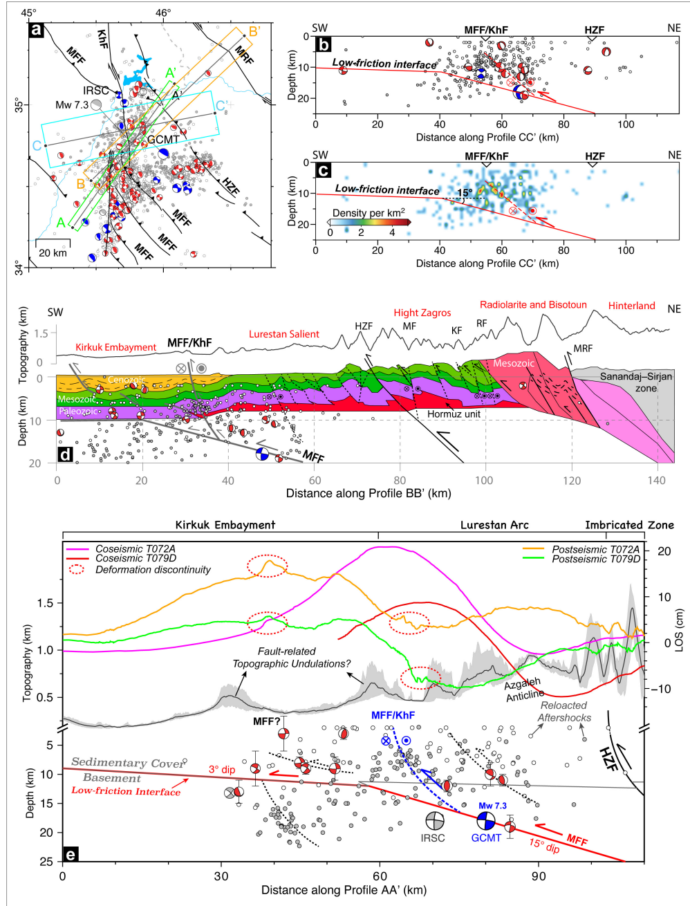
Figure 6.16: Relocated aftershocks, structural cross-section as well as the conceptual fault structures along various profiles in the seismogenic zone. (a) Tectonic map showing the relocated aftershock distributions, faults, as well as the three profiles. The swath widths along Profile AA', BB' and CC' are 8 km, 16 km and 30 km, respectively. The gray dots represent the relocated aftershocks from Fathian et al. (2021) and Jamalreyhani et al. (2022), respectively. The gray, blue and red beach balls are the focal mechanisms from the IRSC, GCMT catalog and Jamalreyhani et al. (2022), respectively. (b) and (c) are the distribution and the density map of relocated aftershocks of Profile CC' along depth, respectively. (d) shows the relocated aftershocks and geologic cross section which is modified from Yang et al. (2018) along Profile BB'. (e) represents the relationship between the topography, seismicity, surface deformation and the regional conceptual interpreted fault structures. The magenta and dark red solid lines indicate the coseismic LOS displacements derived from our previous work (Guo et al., 2022), scaled by a factor of 3. The dashed lines are the conceptual faults. HZF: High Zagros Fault; KF: Kermanshah Fault; MRF: Main Recent Fault; MF: Marekhi Fault; RF: Ravansar Fault; KhF: Khanaqin Fault. 93
