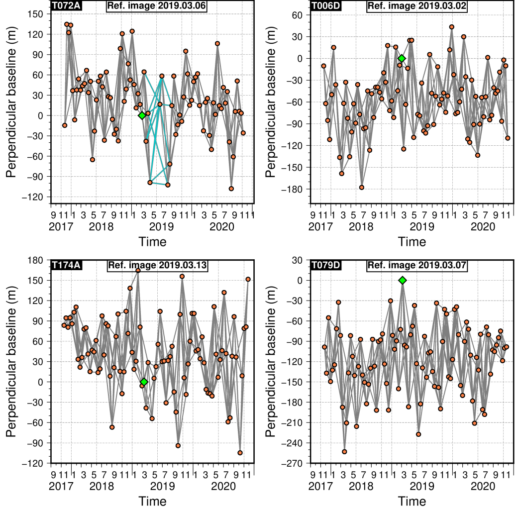
Figure 5.2: The 3-year baseline networks for the 4 sentinel-1 tracks. The green diamond represents the reference image. For T072A, we re-selected 13 interferogram pairs (cyan lines) with 9 SLC data between 18 March 2019 and 02 September 2019 to form at least 3 interferogram pairs for every single SLC data.
