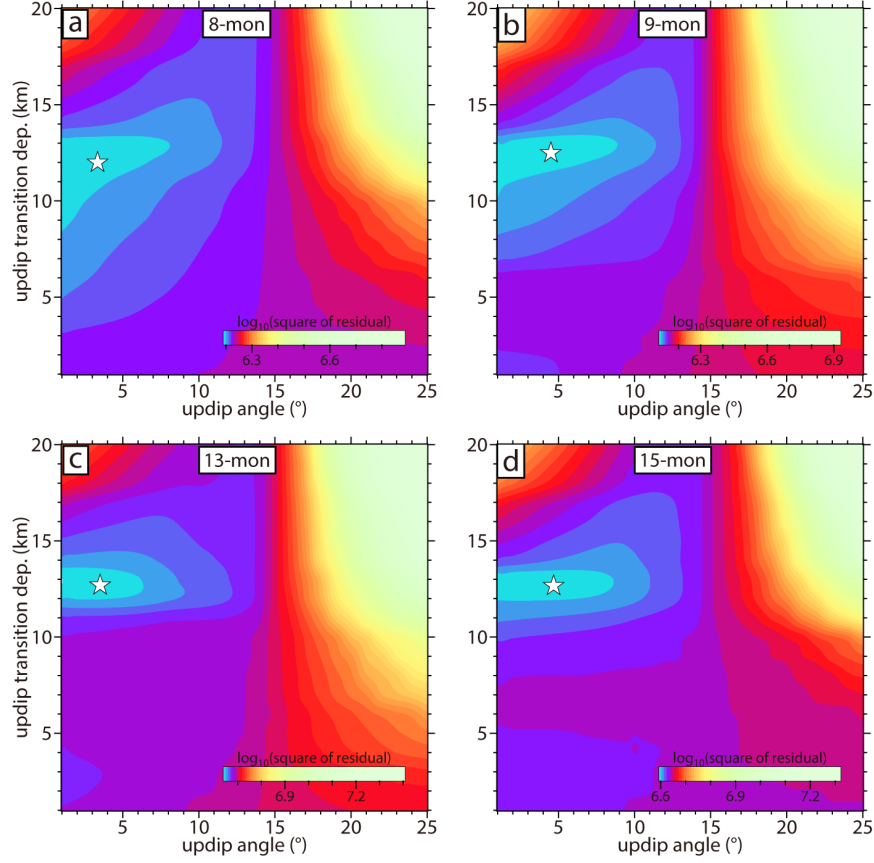
Figure 5.14: The results of searching the dip angles and transition depths of updip fault geometry with the observations of 8, 9, 13 and 15 months after the mainshock.
