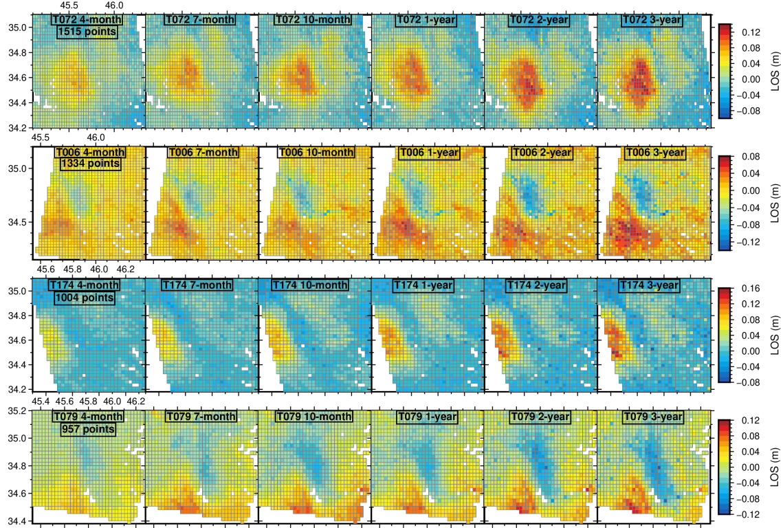
Figure 5.10: The downsampled points from 4-track postseismic InSAR time series. Please note different color bars for each row.
