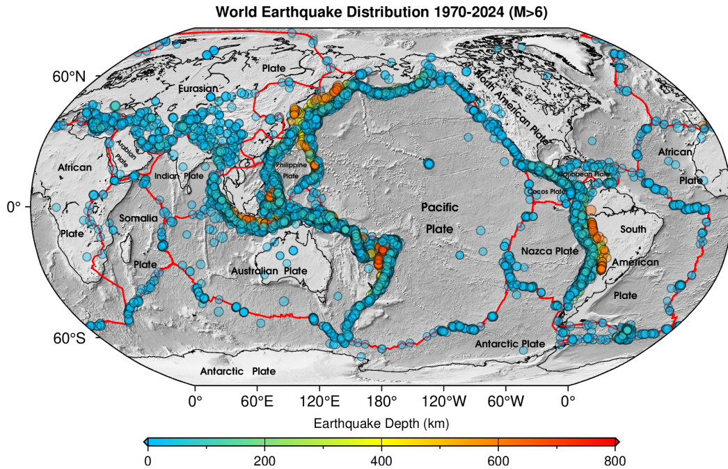
Figure 1.1: World earthquake distribution map from 1970 to 2024 for magnitudes greater than 6.0. The colored dots indicating the earthquakes which are sourced from the U.S. Geological Survey (USGS) earthquake catalog. The red lines represent plate boundaries from Bird (2003).
