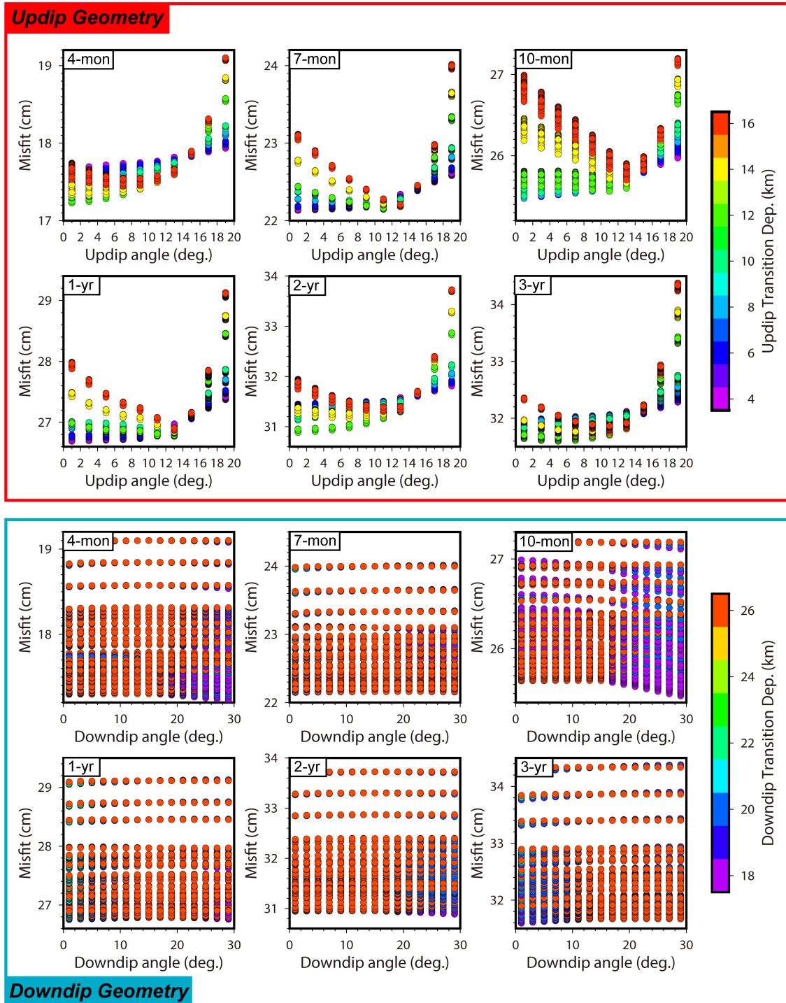
Figure 5.11: Misfit for searching the dip angles and transition depths of updip and downdip fault geometry with the observations of 4, 7, 10 months and 1, 2, 3 years after the mainshock.
