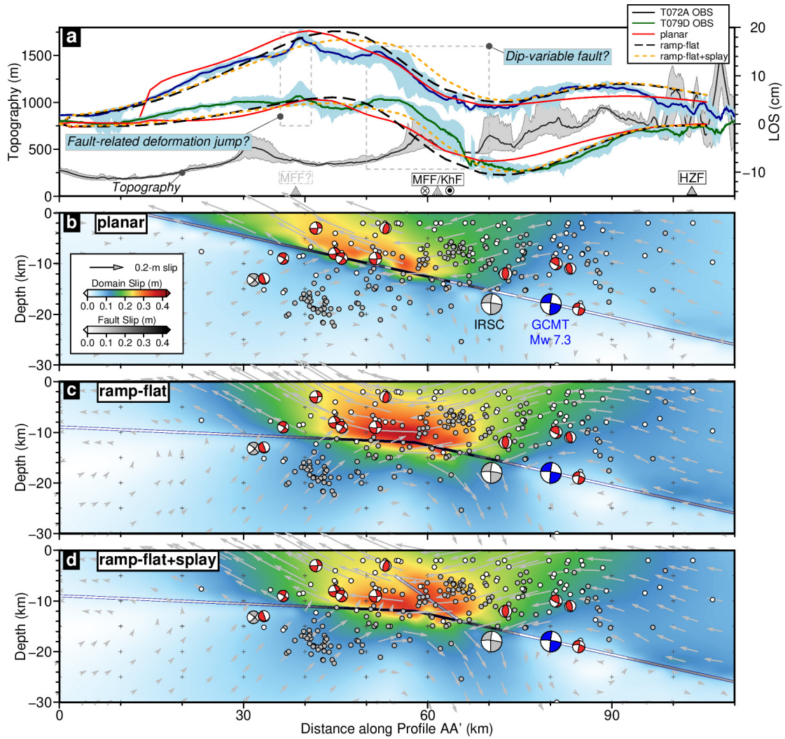
Figure 6.10: Postseismic InSAR observations ( \sim 4.5 years after the mainshock) and different mechanical afterslip models. (a) Comparison between InSAR observations and the model simulations based on (b) the best planar fault model, (c) the best ramp-flat fault model and (d) the best composite model of a ramp-flat and a splay fault. The mechanical models are based on the search results presented in Figure 6.9. The envelope curves of the InSAR observations in (a) indicate the minimum, maximum and mean value of the swath with width of 8 km. The gray and white dots are the relocated aftershocks from Fathian et al. (2021) within approximately 2 months and Jamalreyhani et al. (2022) with M \geq 3 . The gray, blue and red beach balls are the focal mechanisms from the IRSC, GCMT catalog and Jamalreyhani et al. (2022), respectively. HZF: High Zagros Fault; MFF: Mountain Front Fault; KhF: Khanaqin fault.
