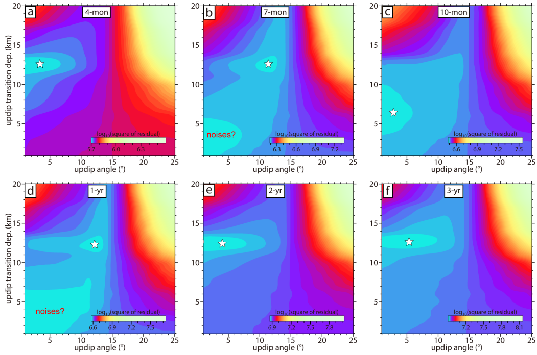
Figure 5.12: Misfit for searching the updip angles and transition depths with the postseismic observations of 4, 7, 10 months and 1, 2, 3 years after the mainshock. Star indicates the best searching result.
