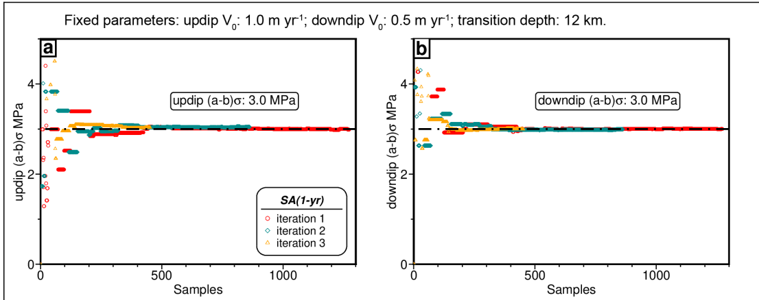
Figure 5.28: Same to Figure 5.27 but with updip and downdip V_0 and transition depth being fixed.
