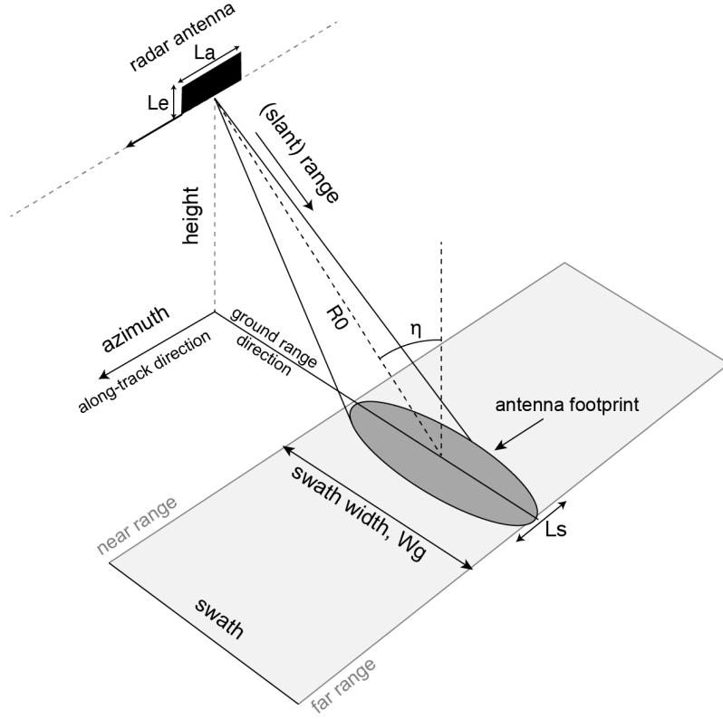
Figure 2.1: Simplified SLAR acquisition geometry.
