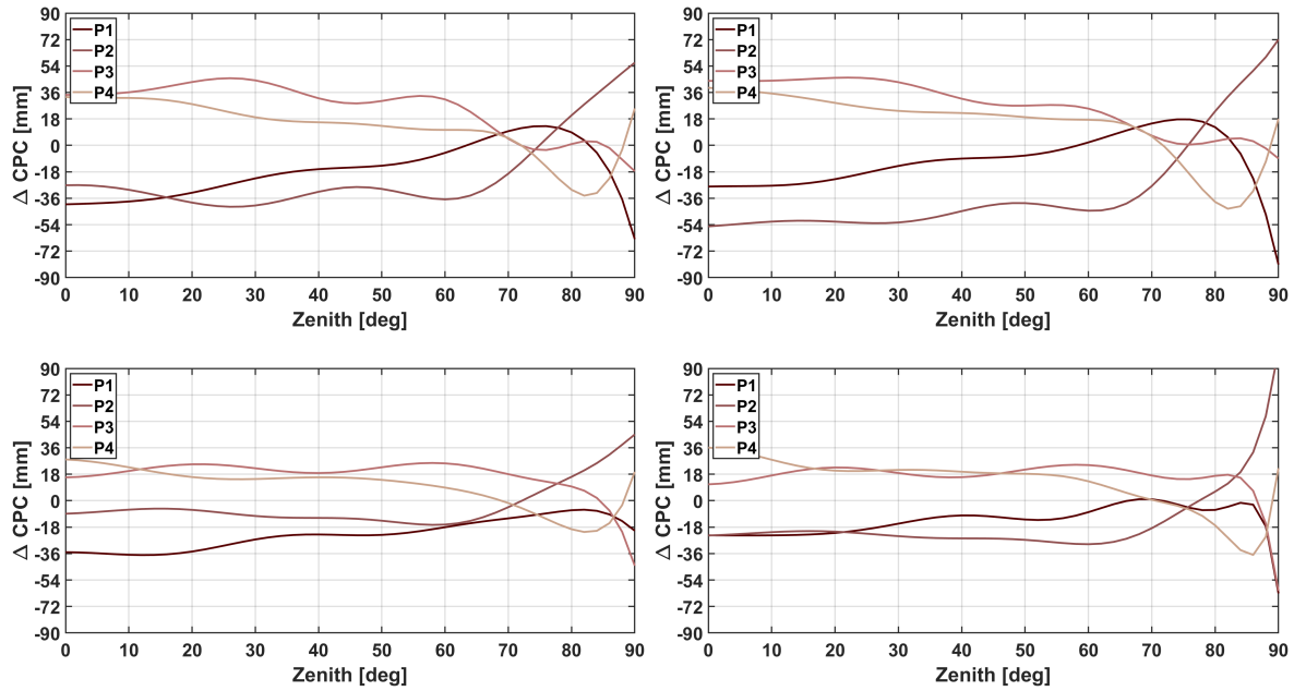
Figure A.7: Comparison w.r.t to type mean CPC pattern for Galileo C5. The elevation dependent pattern (NOAZI) is presented, calibrated with default (top) and optimized (bottom) receiver settings with \Delta\text{SD} as estimation inputs (left) and \Delta\text{MPLC} (right) with multipath map threshold of 1.5 m.
