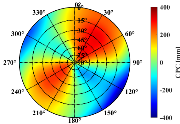
Figure 4.22: CPC pattern of the u-blox ANN-MB1 antenna (category 3), estimated in an anechoic chamber by the DLR.
