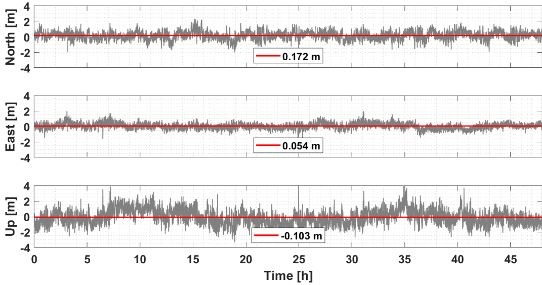
Figure 6.26: Estimated topocentric coordinates w.r.t the reference ITRF2020 coordinates at epoch 27.09.2024 (MSD4) for the category 2 antenna with no additional CPC. The mean value is presented in red.
