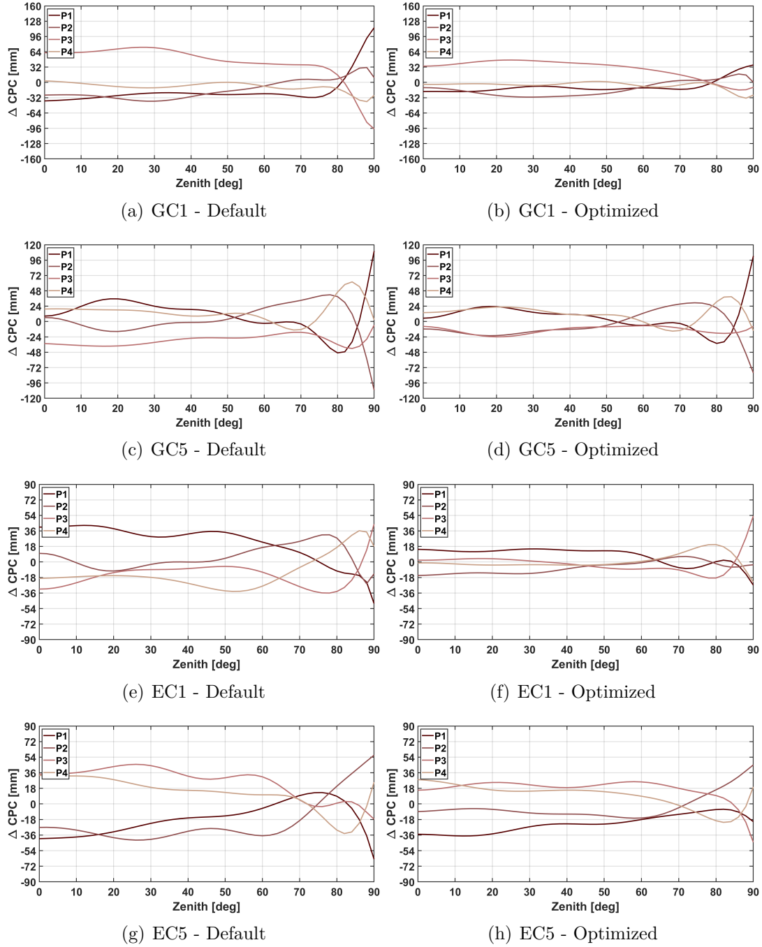
Figure 6.6: Comparison w.r.t to type mean CPC pattern for GPS C1 (a, b), C5 (c, d), Galileo C1 (e, f), C5 (g, h). The elevation dependent pattern (NOAZI) is presented, calibrated with default (left) and optimized (right) receiver settings. P1 to P4 are 24-hours calibrations on consecutive days for a category 2 antenna.
