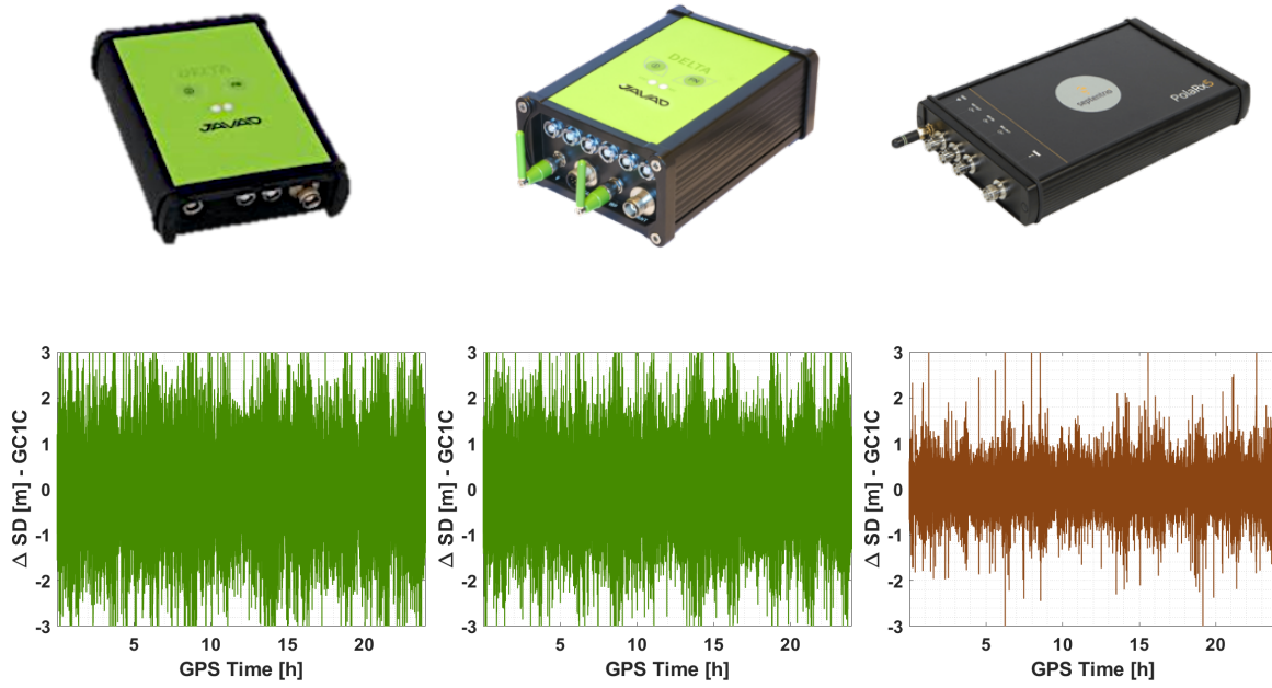
Figure 4.13: \Delta SD from a calibration of an u-blox category 3 antenna for the GPS C1 signal with Javad Delta TRE G3T (left), Javad DeltaS-3S (middle) and Septentrio PolaRx5TR receiver (Right). The \Delta SD of all visible satellites are plotted with the manufactures' default receiver settings [Receiver pictures: JAVAD GNSS (2024a), JAVAD GNSS (2024b), Septentrio (2024)].
