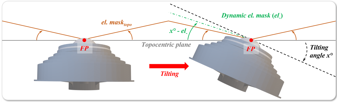
Figure 3.11: Concept of a TEM (orange) and DEM (green), based on Menge (2003).
