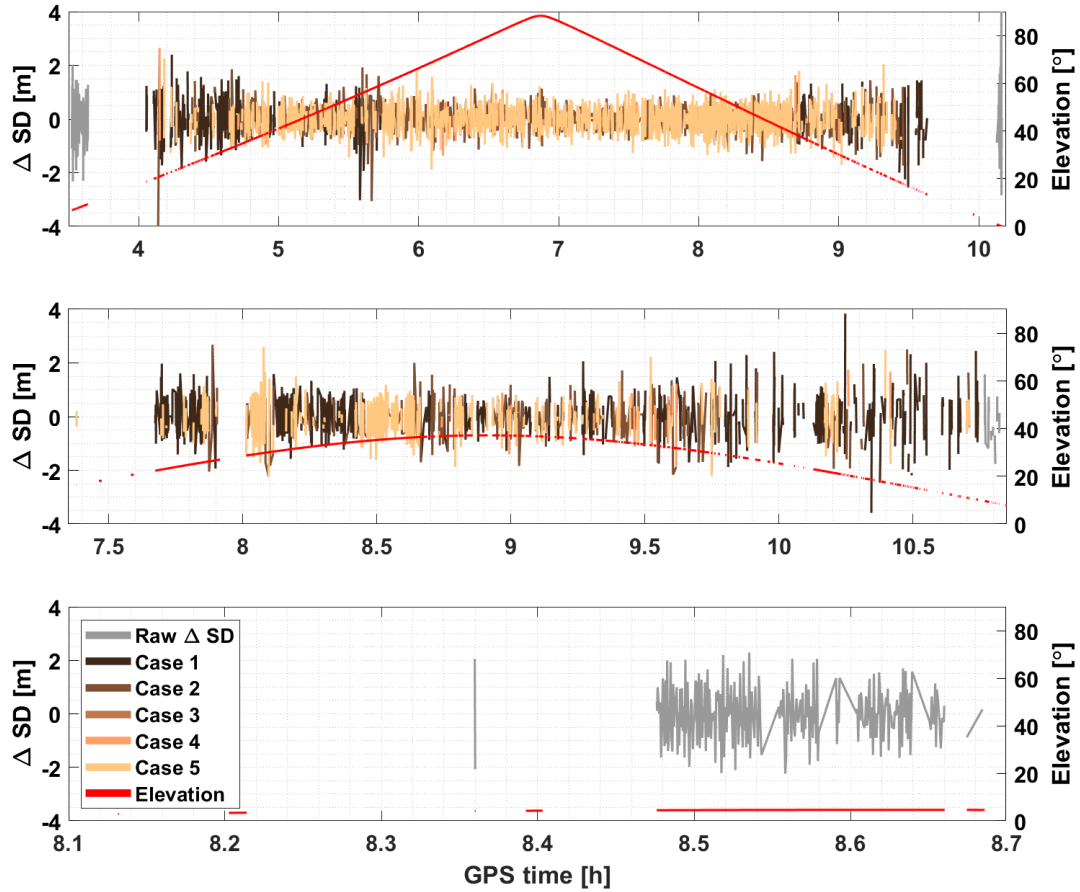
Figure 6.2: \Delta SD after applying different strategies to eliminate problematic observations for GPS C1 signal and satellite PRN2 (top), PRN19 (middle) and PRN12 (bottom). Case 1: TEM ( 10^\circ ); Case 2: Case 1 + MP maps from DLR; Case 3: Case 2 + avoid \Delta SD > 6 s; Case 4: Case 3 + avoid short satellite arcs < 20 epochs; Case 5: Case 4 + avoid static time delay < 0.2 s.
