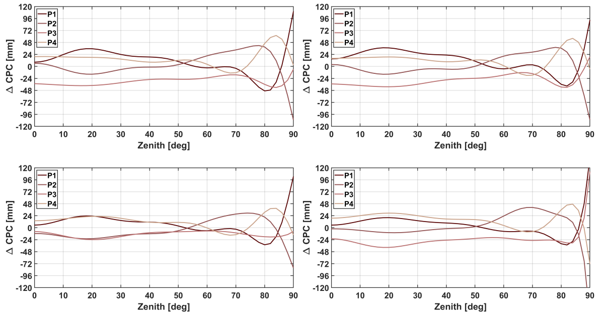
Figure A.5: Comparison w.r.t to type mean CPC pattern for GPS C5. The elevation dependent pattern (NOAZI) is presented, calibrated with default (top) and optimized (bottom) receiver settings with \Delta SD as estimation inputs (left) and \Delta MPLC (right) with multipath map threshold of 1.5 m.
