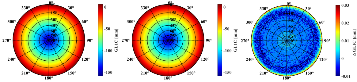
Figure 4.3: Example of a closed loop simulation for a LEIAR25.R3 antenna calibration. (Left) GPS L1 input pattern. (Middle) Estimated pattern with \Delta SD_{sim} based on input pattern. (Right) Difference pattern.
