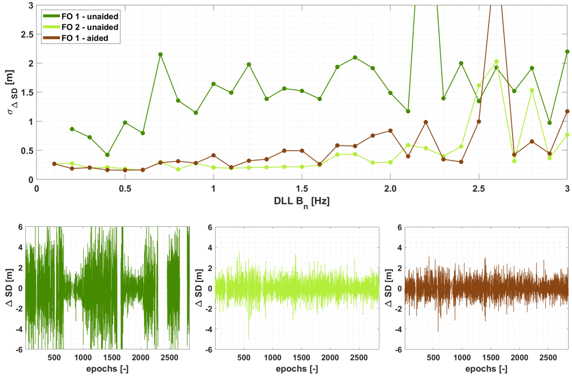
Figure 4.25: Impact of different DLL bandwidths on the observables indicated as weighted averaged \sigma_{\Delta SD} over all visible satellites for an unaided DLL with filter order 1 (dark green), filter order 2 (bright green) and an aided DLL (brown). (Top) \sigma_{\Delta SD} with different DLL bandwidth B_n . (Bottom) \Delta SD with DLL bandwidth of 1 Hz for GPS satellite PRN16. Presented is the C1 signal for the three cases (same colors).
