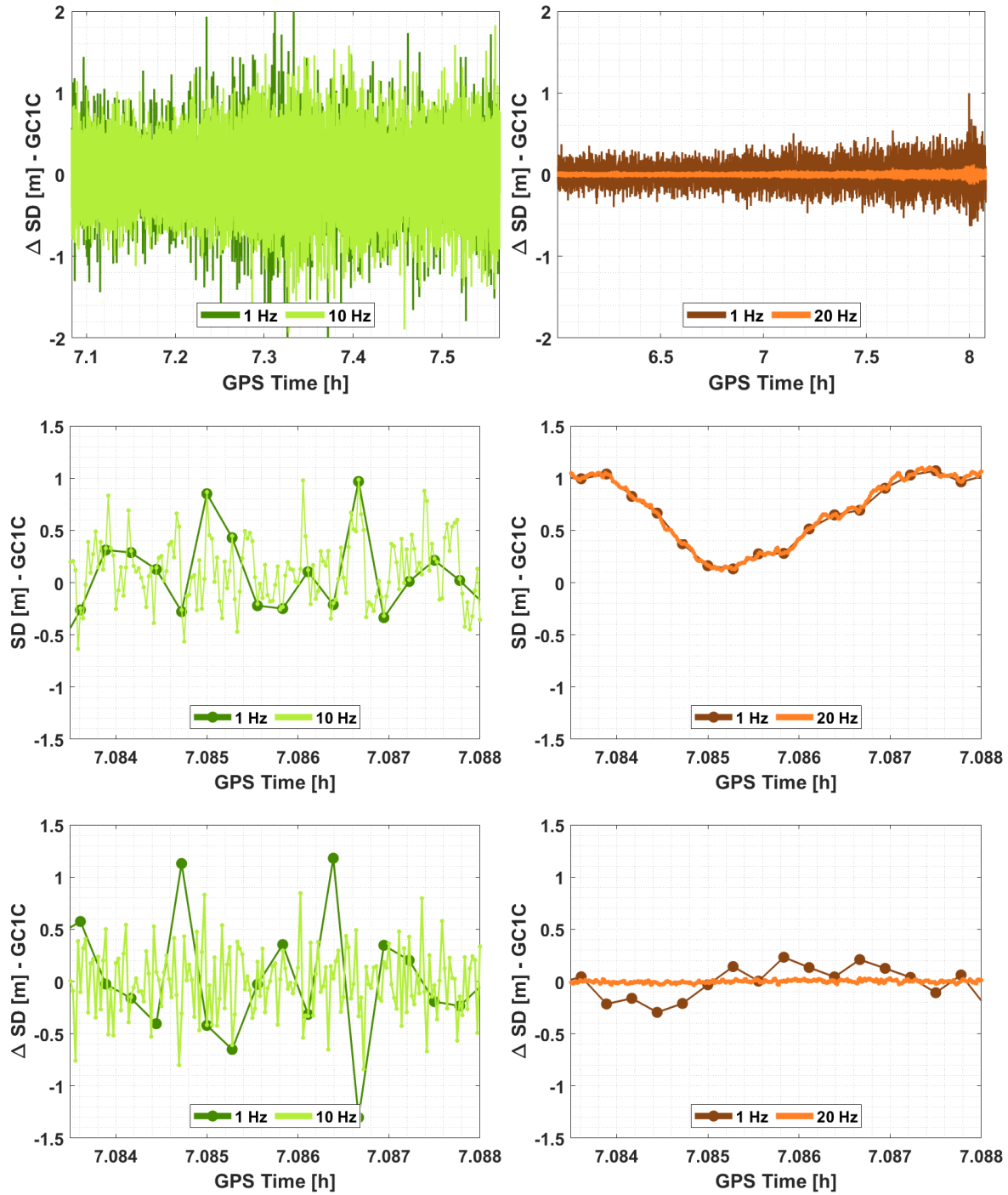
Figure 4.14: Static experiment for the GPS C1 signal for PRN5 satellite with a category 2 antenna with Javad Delta TRE G3T (left) and Septentrio PolaRx5TR receiver (right). Both receivers operate with a DLL bandwidth of 0.25 Hz. The experiments have been carried out on different days. The top row shows the \Delta SD over the whole static time, the middle row depicts the SD in a zoom on a specific time span and the last row presents the corresponding \Delta SD . 1 Hz and 10 Hz for Javad respectively 20 Hz for Septentrio are presented.
