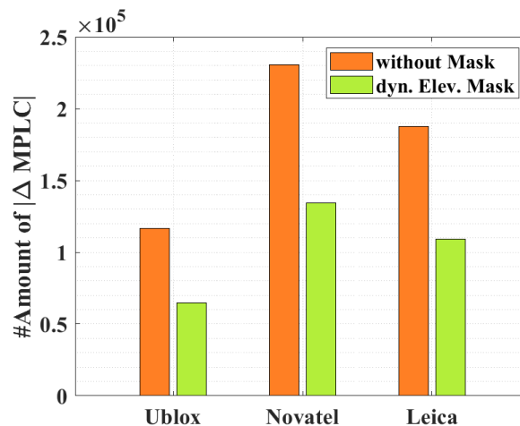
Figure 5.8: Amount of \Delta\text{MPLC} with and without a dynamic elevation mask for three different antennas, calibrated over 24 hours.
