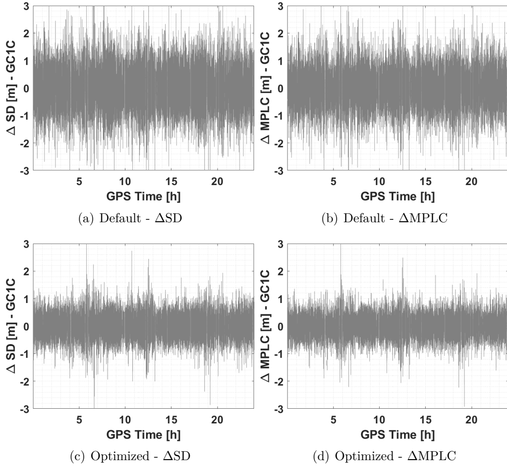
Figure 6.11: \Delta SD (left) and \Delta MPLC (right) of a 24-hour calibration for a category 2 antenna with default (top) and optimized receiver settings (bottom).
