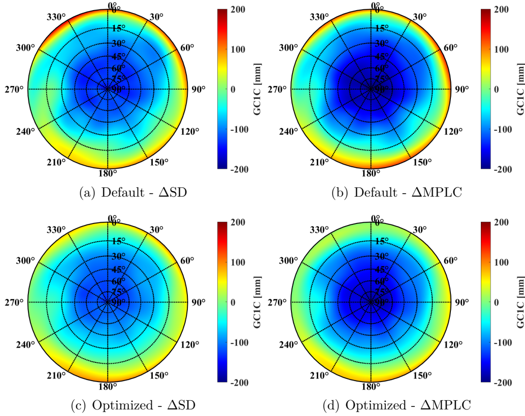
Figure 6.12: Estimated mean pattern of GPS C1, calibrated with default (top) and optimized (bottom) receiver settings with \Delta SD as estimation inputs (left) and \Delta MPLC (right) with multipath map threshold of 1.5 m.
