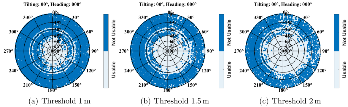
Figure 5.15: Multipath map for the Novatel antenna for three different thresholds: (a) 1 m (b) 1.5 m and (c) 2 m in a no tilting scenario and a heading of 0^\circ .
