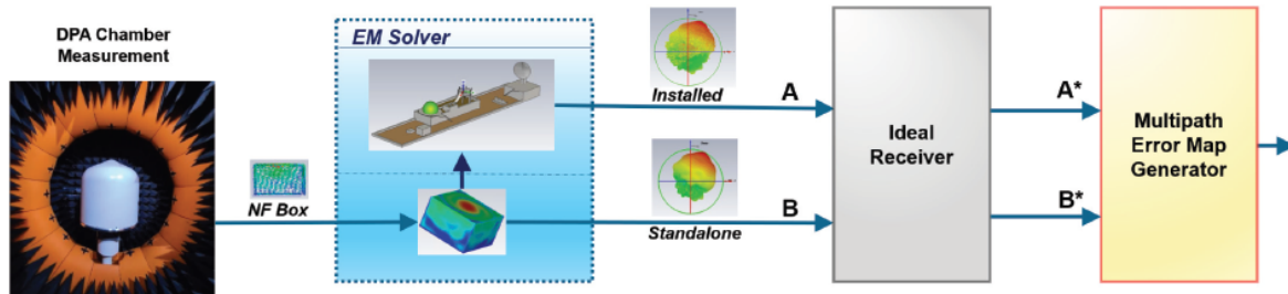
Figure 5.12: Scheme of fullWaveIP algorithm to generate multipath error maps (Addo et al., 2024b).
