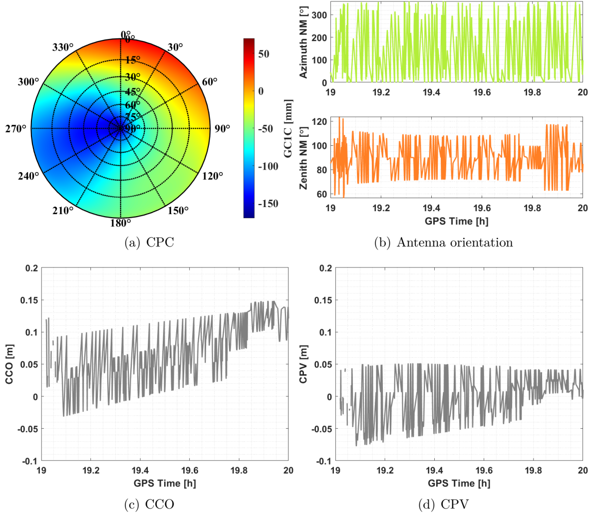
Figure 4.1: Example of the behaviour of GPS C1 CCO (c) and CPV (d) from GPS PRN5 for a LEIAR25.R3 antenna during a robot calibration, based on the pattern presented in (a). The actual AUT pose is presented as a function of zenith angle and azimuth of the antenna's NM (b).
