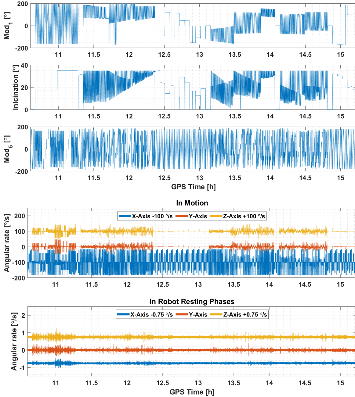
Figure 4.16: Robot module angles during a calibration (top) with the measured angular rates from the IMU (IMU) (bottom).
