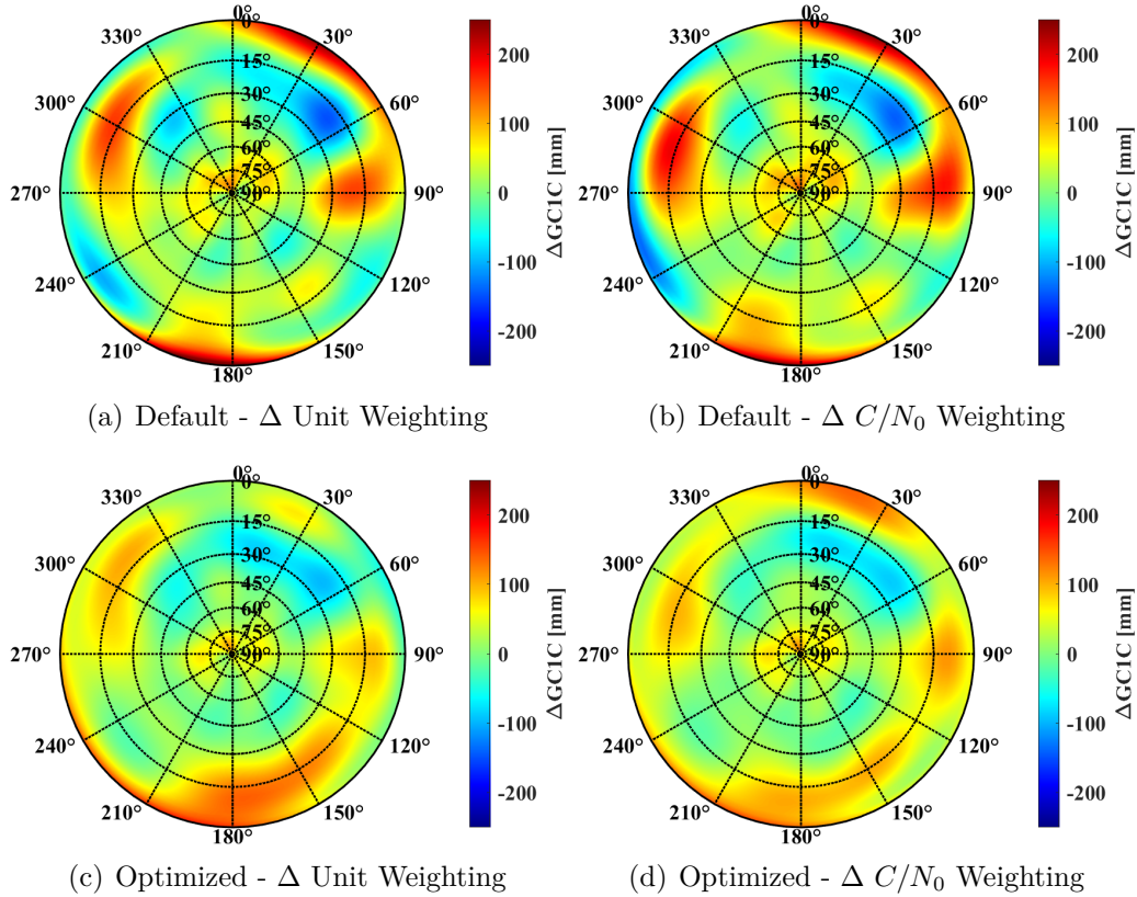
Figure 6.21: Differences between the CPC patterns estimated on two consecutive days of the category 3 antenna for GPS C1. Subfigure (a) and (c) presented the results when using a unit weighting, whereas (b) and (d) shows the pattern when using a C/N_0 dependent weighting. Default receiver settings are used for (a) and (b) and optimized receiver settings for (c) and (d). A multipath map threshold of 2 m is applied.
