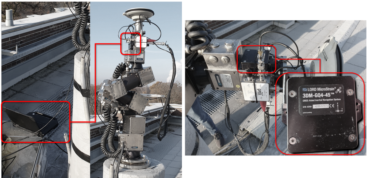
Figure 4.15: Experimental setup (left) with the definition of the IMU axis (right).
