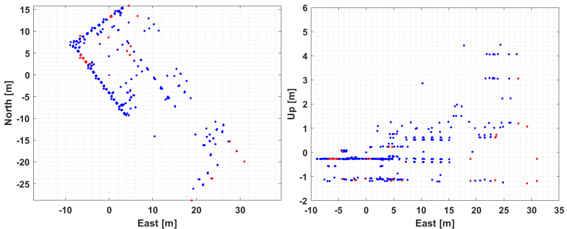
Figure 5.2: Measured points (blue) and calculated points (red) within the practical survey. (Left) Horizontal position of the points. (Right) Vertical position of the points.
