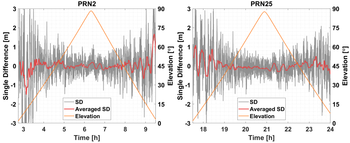
Figure 6.28: Single differences of GPS satellite PRN2 (left) and PRN25 (right) in grey, with their moving average single differences in red.
