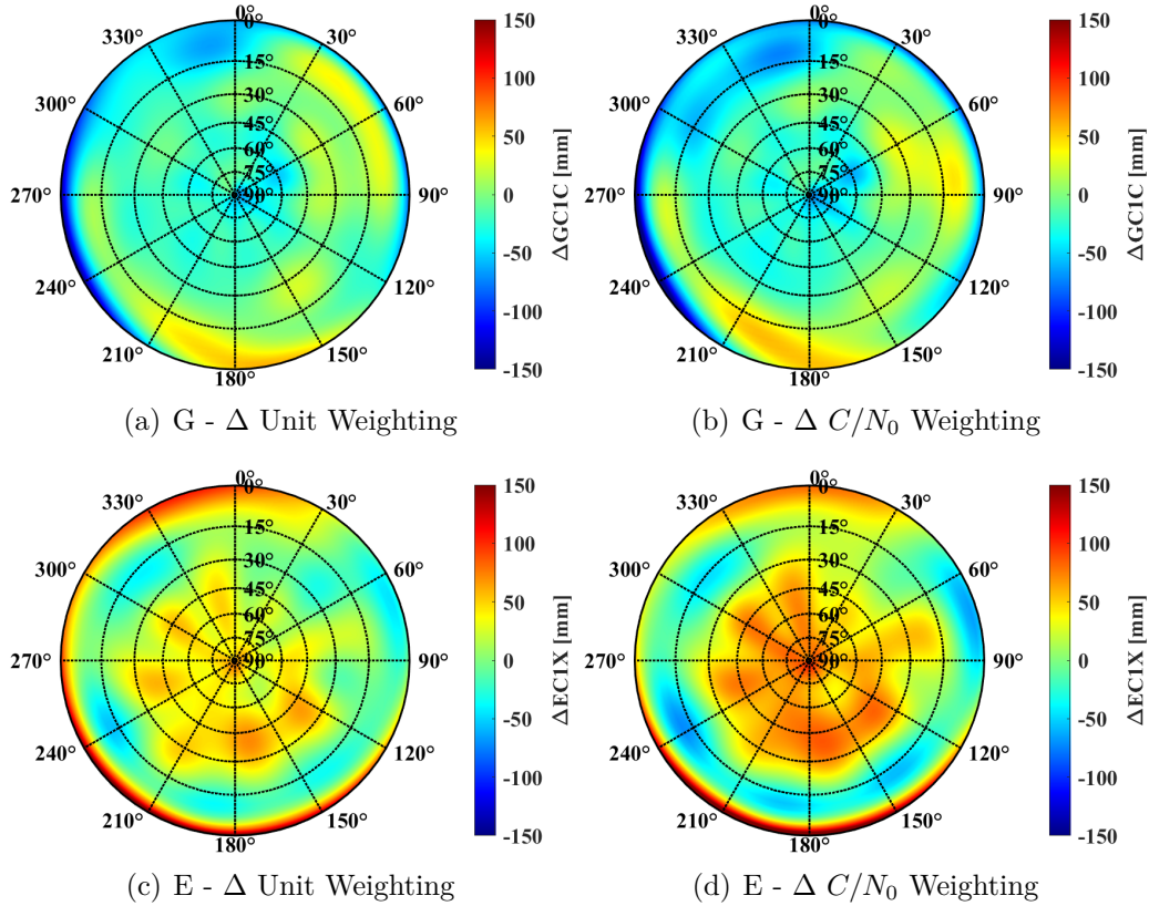
Figure 6.19: Differences between the CPC patterns estimated on two consecutive days of the category 1 antenna for GPS C1 (top) and Galileo C1 signal (bottom). Subfigure (a) and (c) presented the results using a unit weighting, whereas (b) and (d) shows the difference pattern when using a C/N_0 dependent weighting. Optimized receiver settings are used with a multipath map threshold of 2 m.
