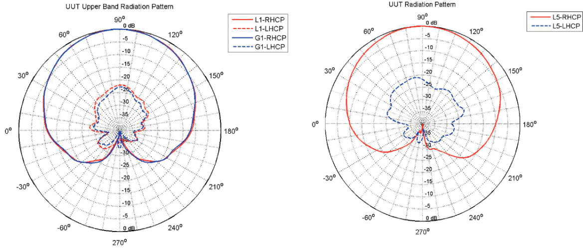
Figure 2.1: Radiation pattern from the NOV703GGG.R2 antenna for GPS (L) and GLONASS (G) on L1 carrier frequency (left) and GPS on L5 carrier frequency (right) (Novatel, 2011).
