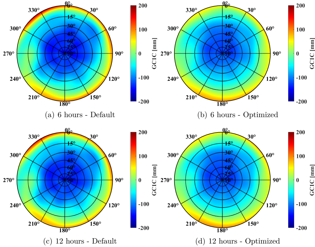
Figure 6.8: Estimated Mean CPC pattern for GPS C1 calibrated with default (left) and optimized (right) receiver settings. The pattern is calculated from all 6-hour calibration (a), (b) and 12-hour in (c), (d) extracted from P1 to P4.
