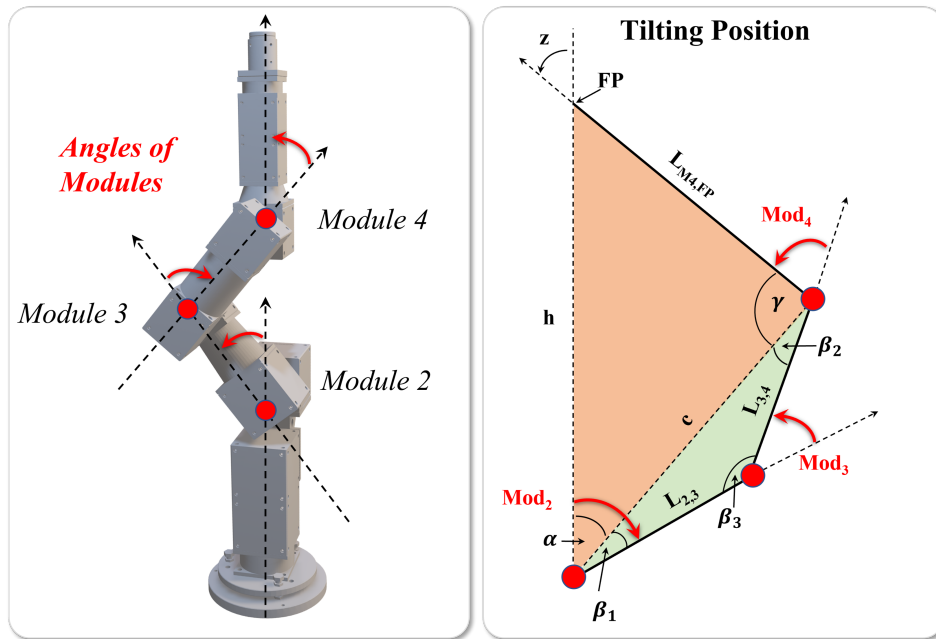
Figure 3.9: Definition of the angular positions of the tilting modules.
