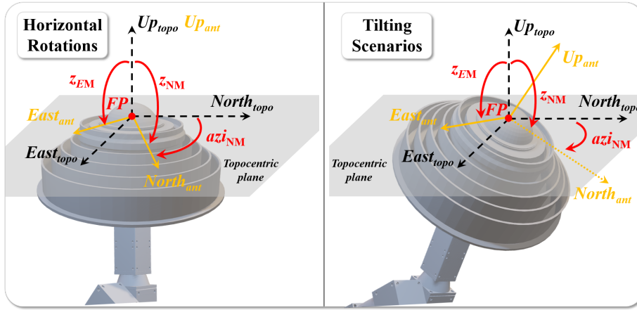
Figure 3.10: Definition of the antenna coordinate system during a calibration in horizontal (left) and tilting (right) scenarios.
