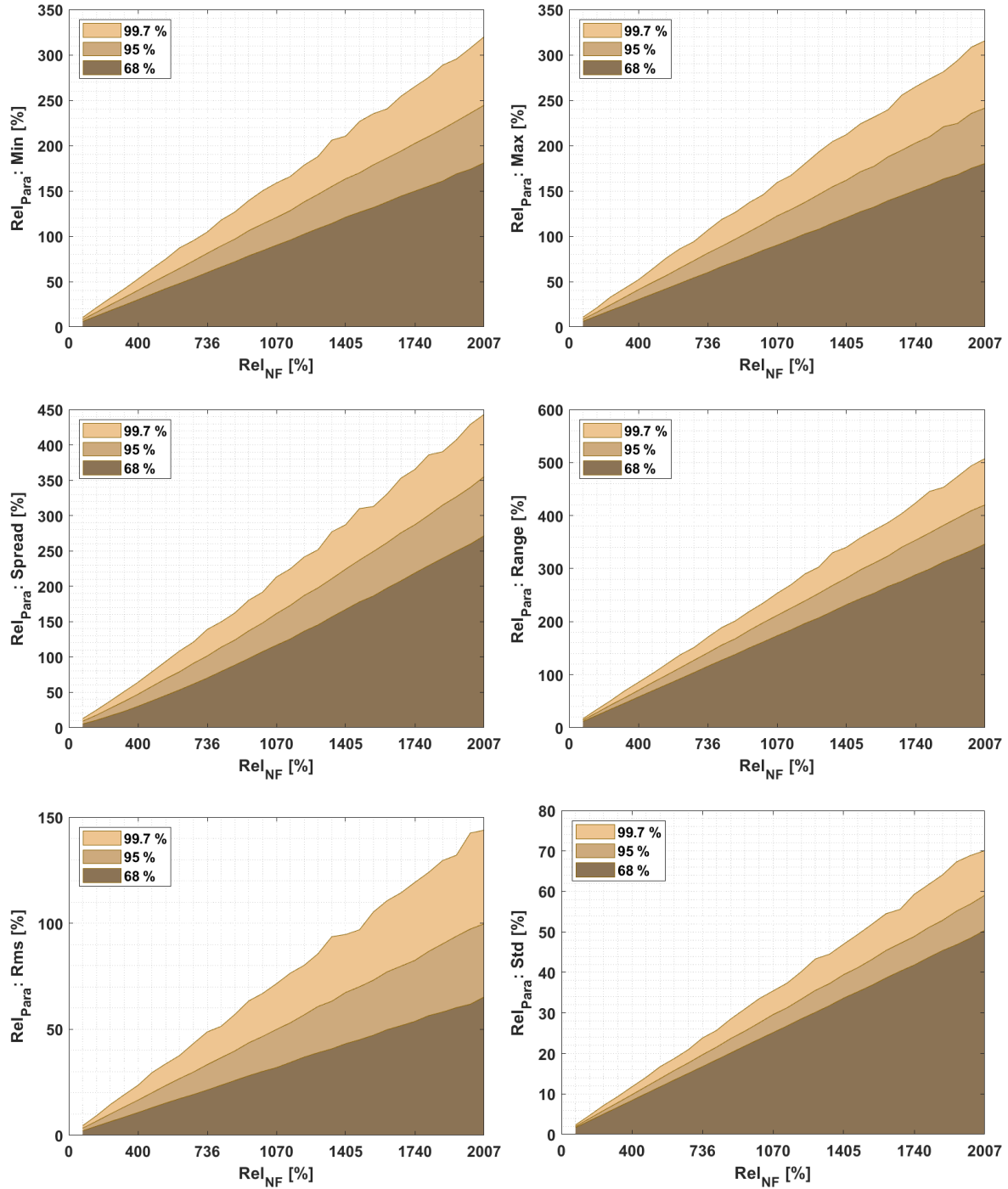
Figure A.2: Results for relative comparison metrics for the category 1 antenna with additional WN, based on input pattern in Figure A.1 with different noise factors. Because the noise factor is varying up to 3 m and P_{Peak} is 149.44 mm, Rel_{NF} is varying to 2007 %.
