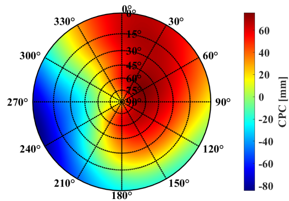
Figure A.1: CPC pattern of a category 1 antenna provided by DLR.
