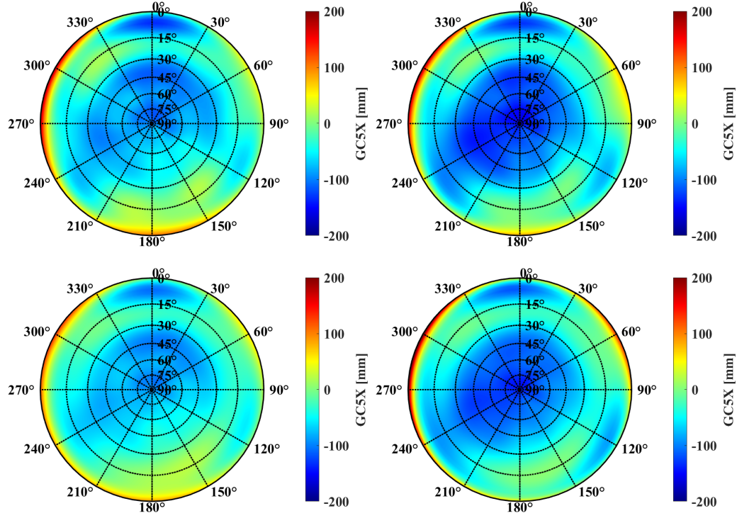
Figure A.4: Estimated mean pattern of GPS C5, calibrated with default (top) and optimized (bottom) receiver settings with \Delta SD as estimation inputs (left) and \Delta MPLC (right) with multipath map threshold of 1.5 m.
