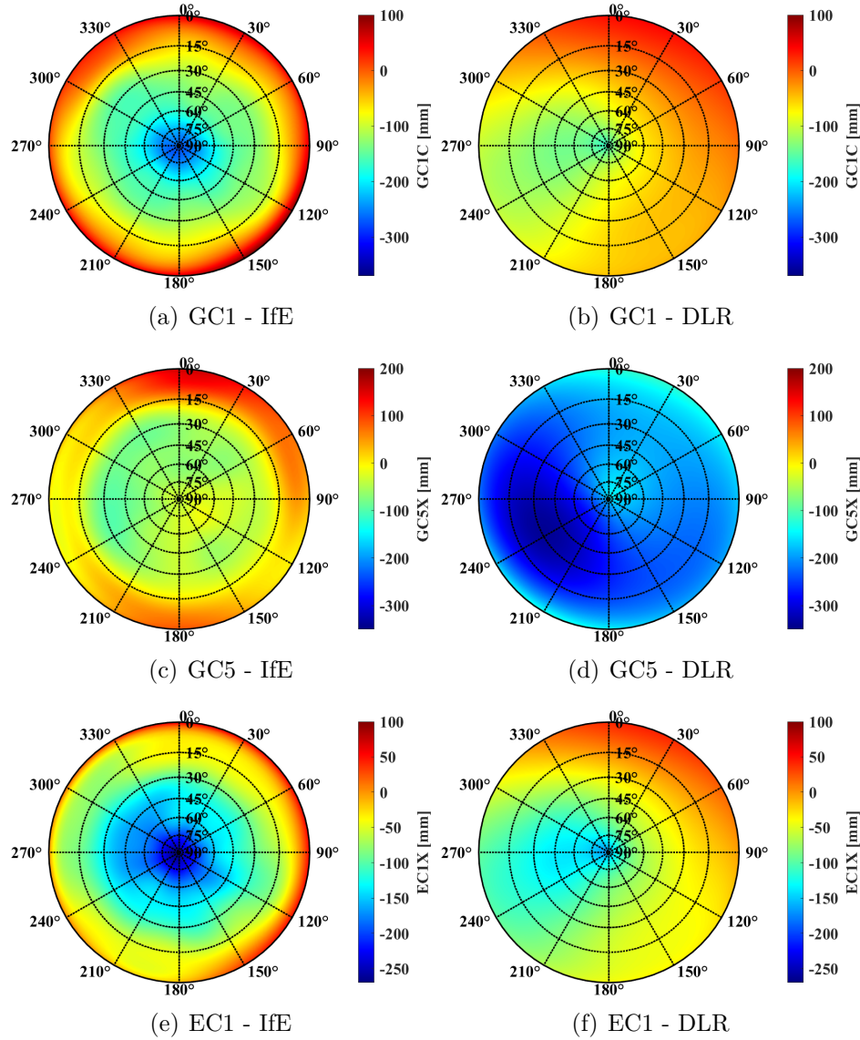
Figure 6.22: Estimated Mean CPC pattern for GPS C1 (a) and C5 (c) and Galileo C1 (e) calibrated at IfE with optimized receiver settings and calibrated in an anechoic chamber by DLR (b, d, f) for a category 1 antenna.
