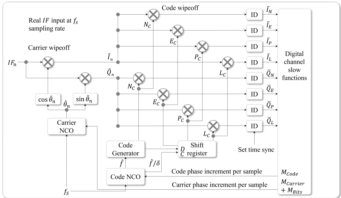
Figure 2.3: Closed loop fast function of a digital channel within GNSS receivers using real IF as input, based on Häberling (2016) and Kaplan and Hegarty (2017).
