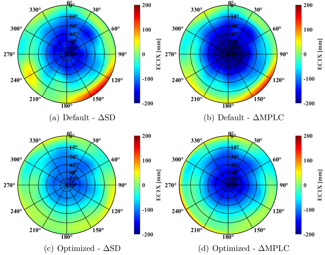
Figure 6.13: Estimated mean pattern of Galileo C1, calibrated with default (top) and optimized (bottom) receiver settings with \Delta SD as estimation inputs (left) and \Delta MPLC (right) with multipath map threshold of 1.5 m.
