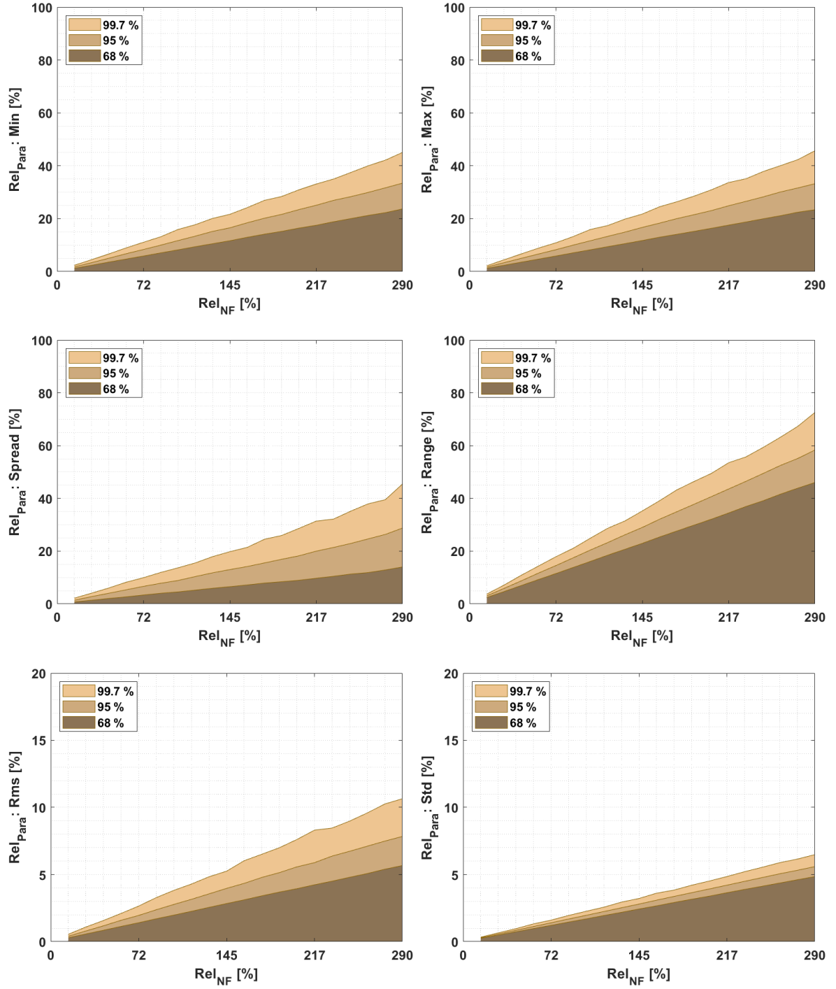
Figure 4.21: Comparison metric parameters as relative values with different noise factors for CN0 based noise.
