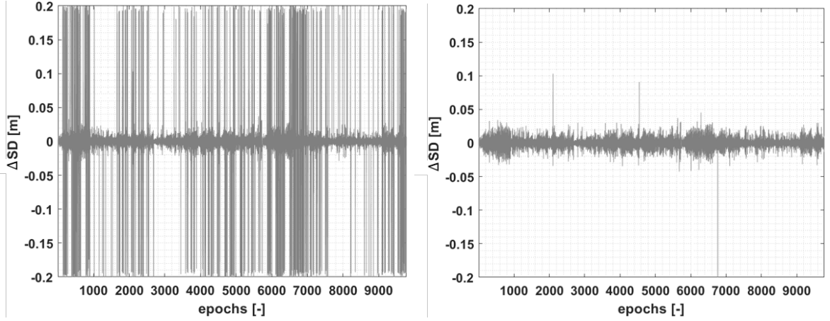
Figure 3.13: \Delta SD before the PWU cycle slip fixing (left) and after (right).
