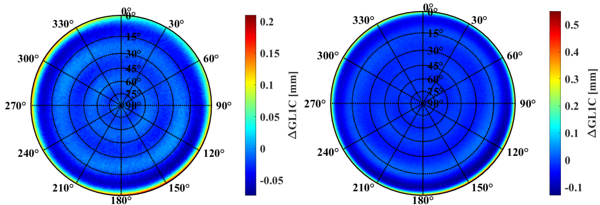
Figure 4.4: Closed loop differences with negative elevation obtained by extrapolating PCV from zero-degree elevation (left) and by mirroring PCV from positive elevations (right). Please note the different scales.
