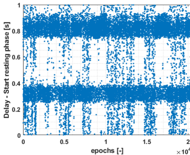
Figure 6.1: Delay between start of the robot resting phase and the actual observation.
