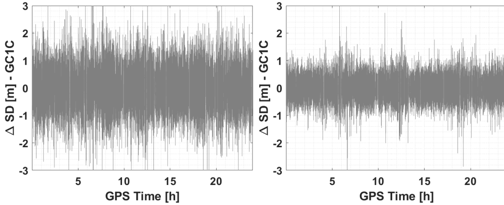
Figure 6.4: \Delta SD of a 24-hour calibration for a category 2 antenna with default (left) and optimized receiver settings (right).
