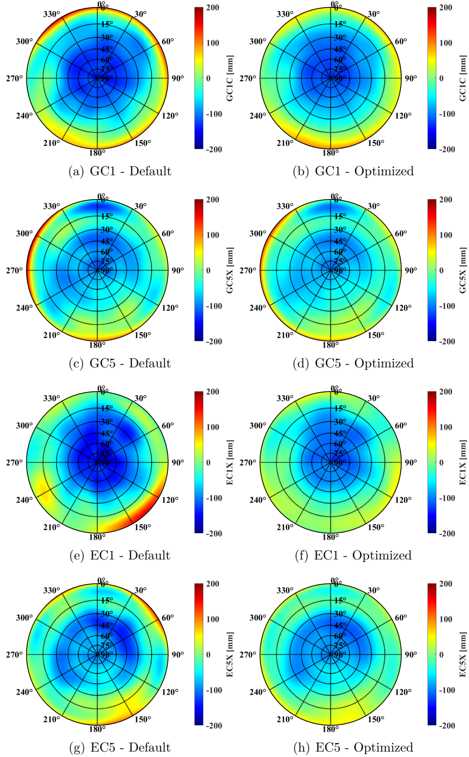
Figure 6.5: Estimated Mean CPC pattern for GPS C1 (a, b), C5 (c, d), Galileo C1 (e, f) and C5 (g, h) calibrated with default (left) and optimized (right) receiver settings. The pattern is calculated from four 24-hours calibrations on consecutive days for a category 2 antenna.
