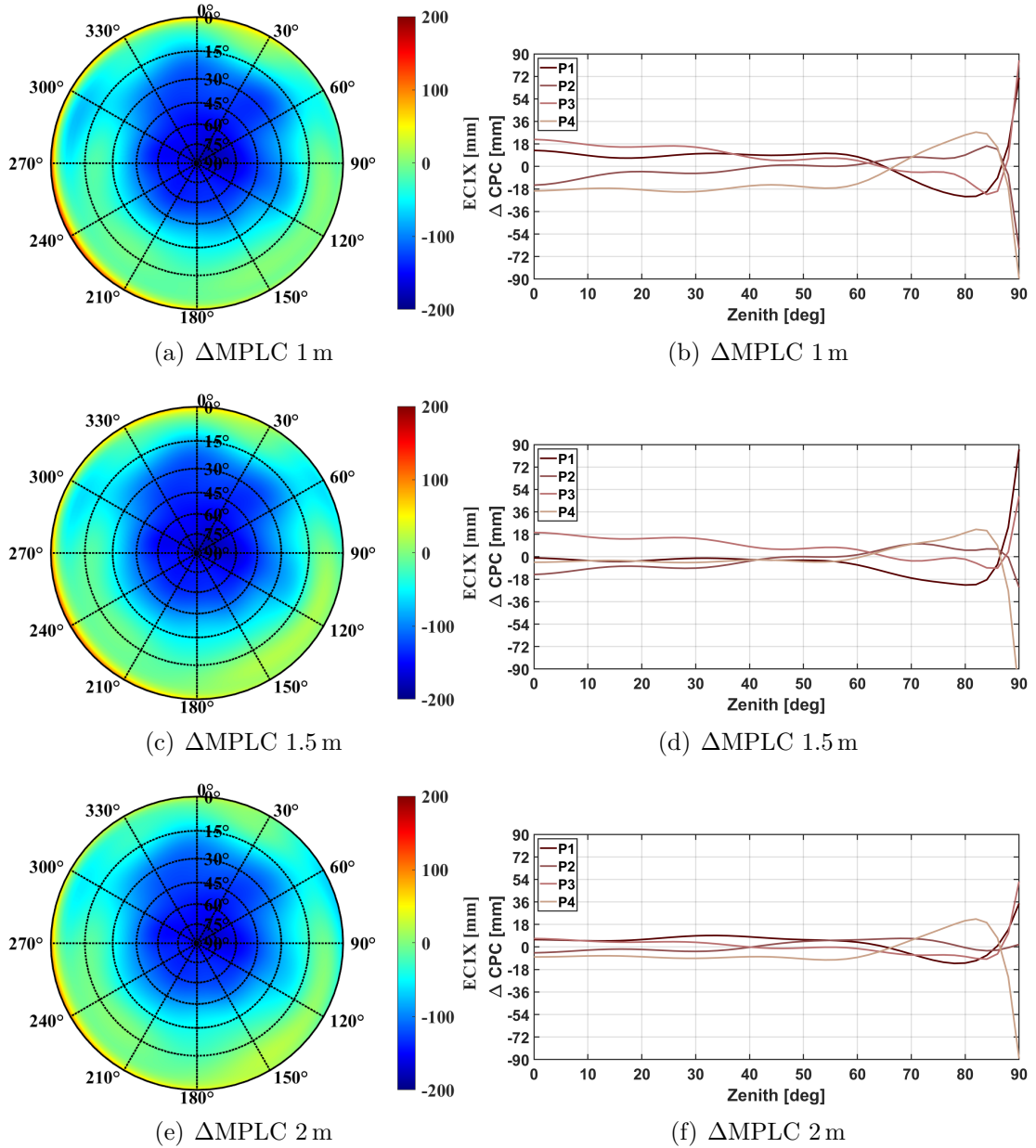
Figure 6.16: Estimated mean pattern (left) and the corresponding NOAZI repeatability (right) of Galileo C1, calibrated with optimized receiver settings with \Delta\text{MPLC} as estimation inputs. Multipath map thresholds of 1 m (a, b), 1.5 m (c, d) and 2 m (e, f) are applied.
