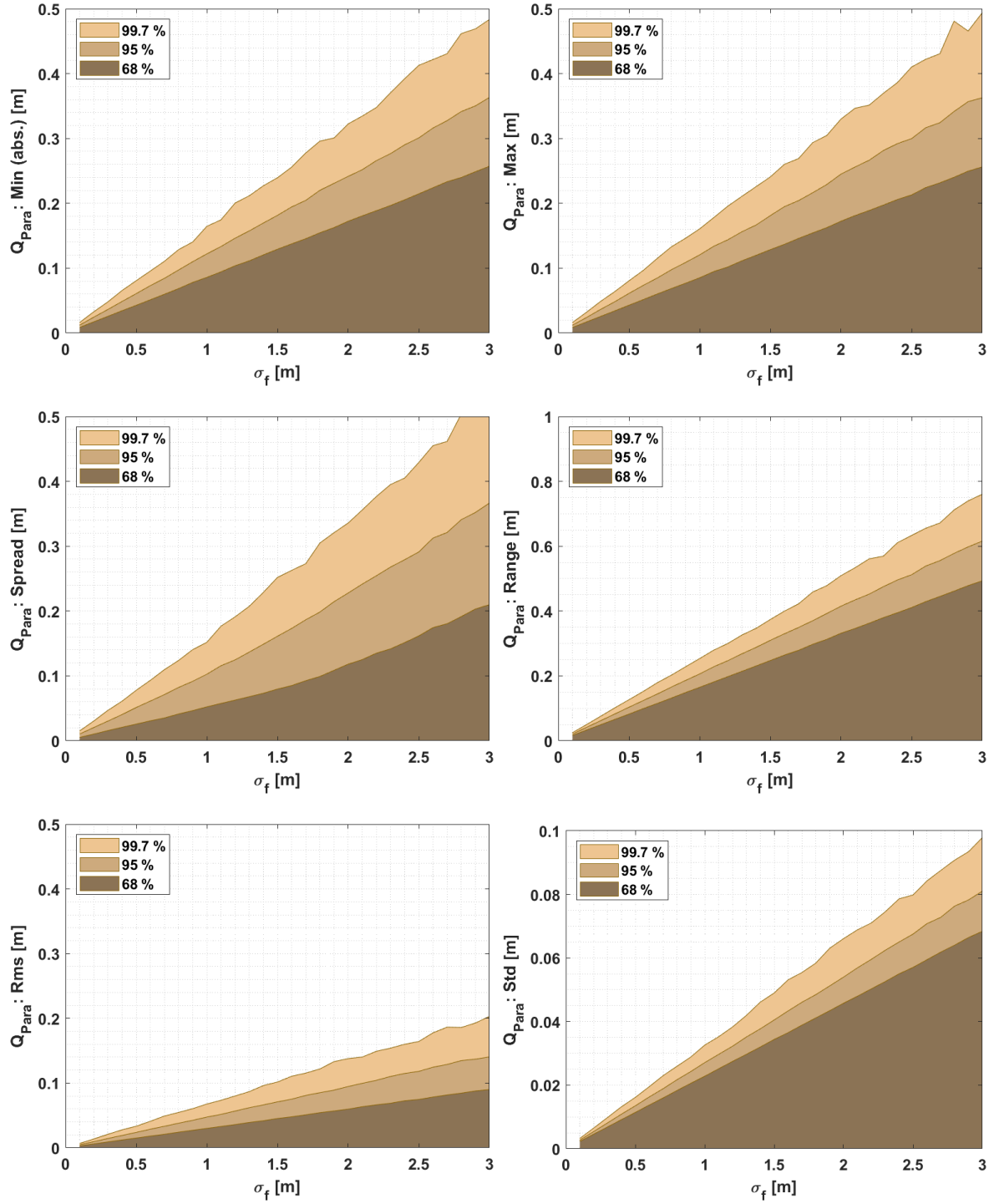
Figure 4.19: Results for absolute comparison metrics for the category 3 antenna, based on CPC provided by DLR with different noise factors. Note: Values only valid for this specific pattern (absolute).
