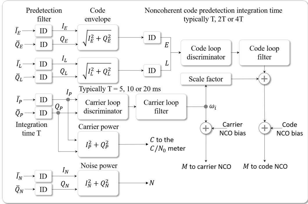
Figure 2.4: Closed loop slow function of a digital channel within GNSS receivers, based on Kaplan and Hegarty (2017).
