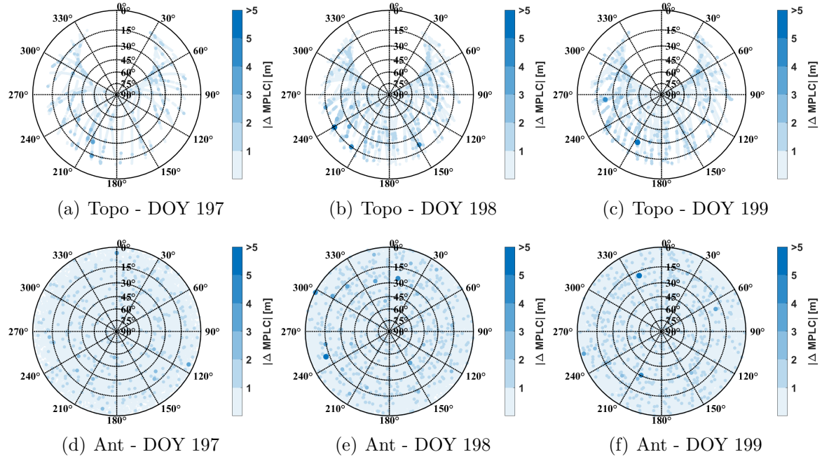
Figure 5.7: Absolute \Delta\text{MPLC} values using a dynamic elevation mask in topocentric (top) and antenna frame (bottom) for GPS with the signals C1C, L1C and L2W (top) for a category 2 antenna. The data were observed within a calibration from DOY 197 (left) to DOY 199 (right). Please note that only 11 hours are used in DOY 197.
