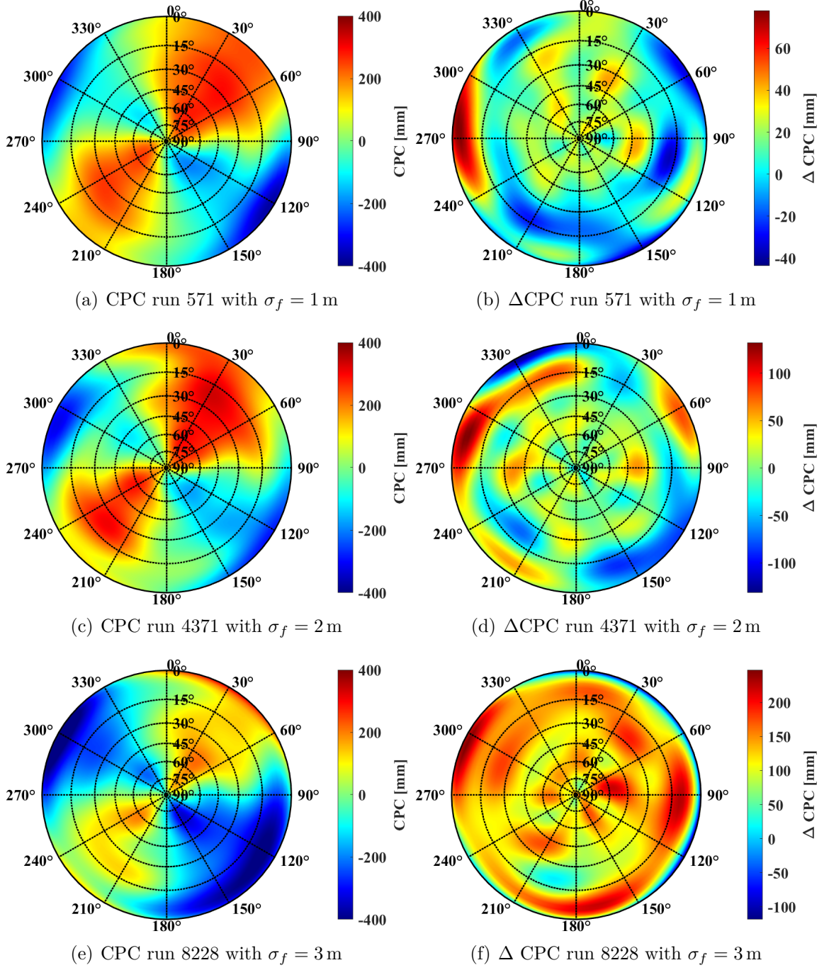
Figure 4.24: CPC pattern (left) and their differences to the original pattern (right), when \sigma_f = 1 m (a, b), \sigma_f = 2 m (c, d) and \sigma_f = 3 m (e, f) is added.
