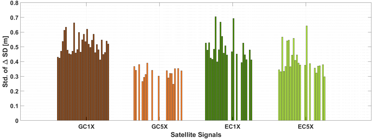
Figure 4.10: Standard deviations of all visible satellites for the C1 and C5 signal of GPS and Galileo for a 24-hour calibration of a category 2 antenna. The calibration has been carried out with a Javad Delta TRE G3T receiver with default settings.
