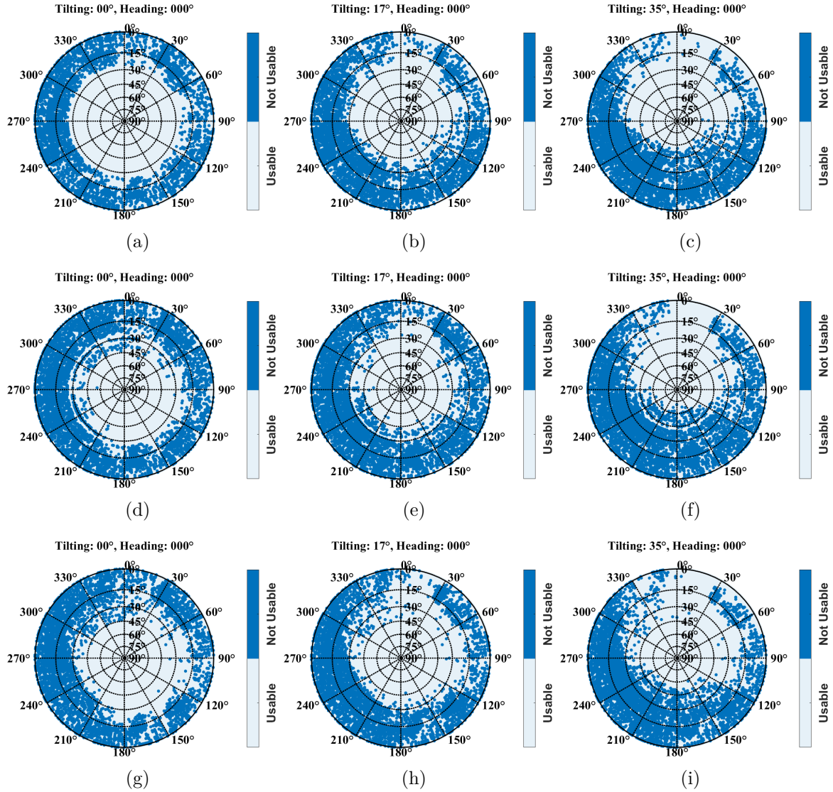
Figure 5.17: Multipath maps for three different antennas and tilting scenarios (2m threshold). The top column represent the maps for the u-blox antenna, the second for Novatel and the last column for the Leica antenna. The tilting angle increase from left 0° to middle 17° and right 35° in North direction.
