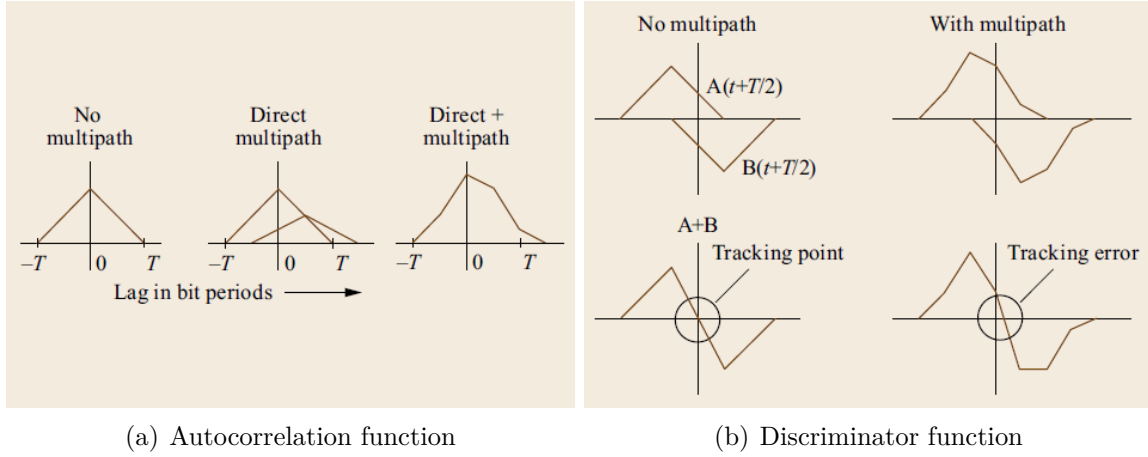
Figure 2.5: Autocorrelation (a) and discriminator function (b) with and without the presence of multipath (Braasch, 2017).
