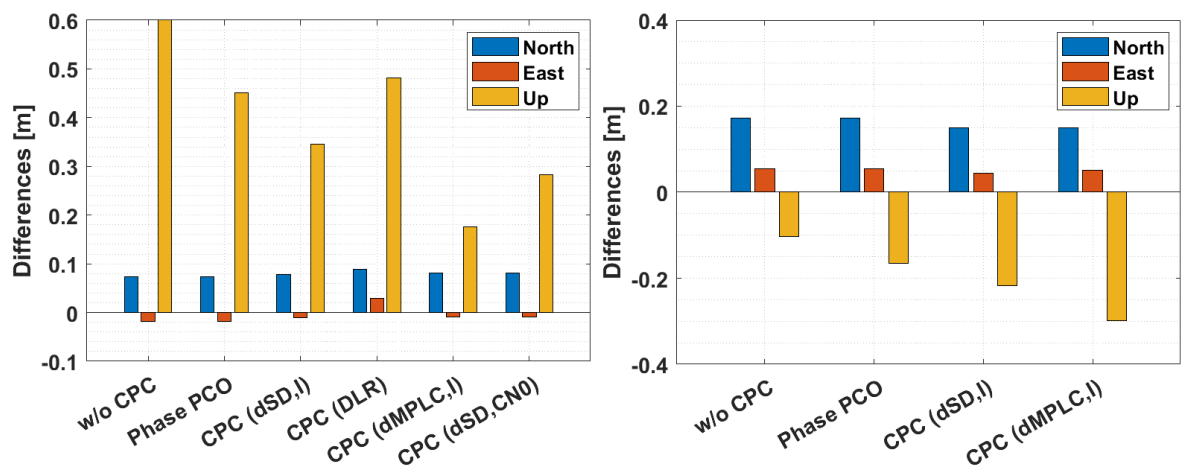
Figure 6.27: Estimated mean topocentric coordinates w.r.t the reference ITRF2020 coordinates at epoch 27.09.2024 for the category 1 (left) and category 2 antenna (right) by applying different CPC pattern.
