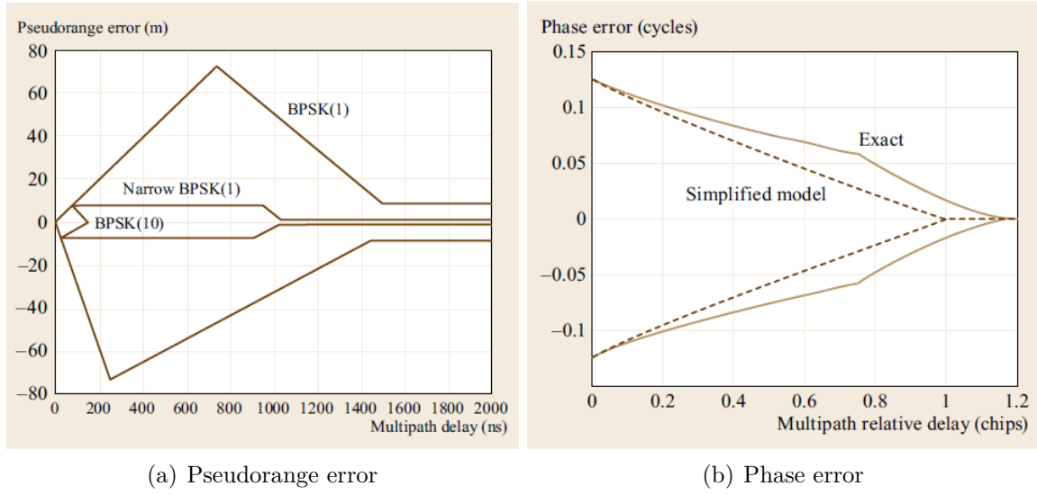
Figure 2.6: Pseudorange error (a) in presence of multipath with half the amplitude of the direct signal. Phase error (b), when using a coherent DLL and a correlator spacing of 1 chip (Braasch, 2017).
