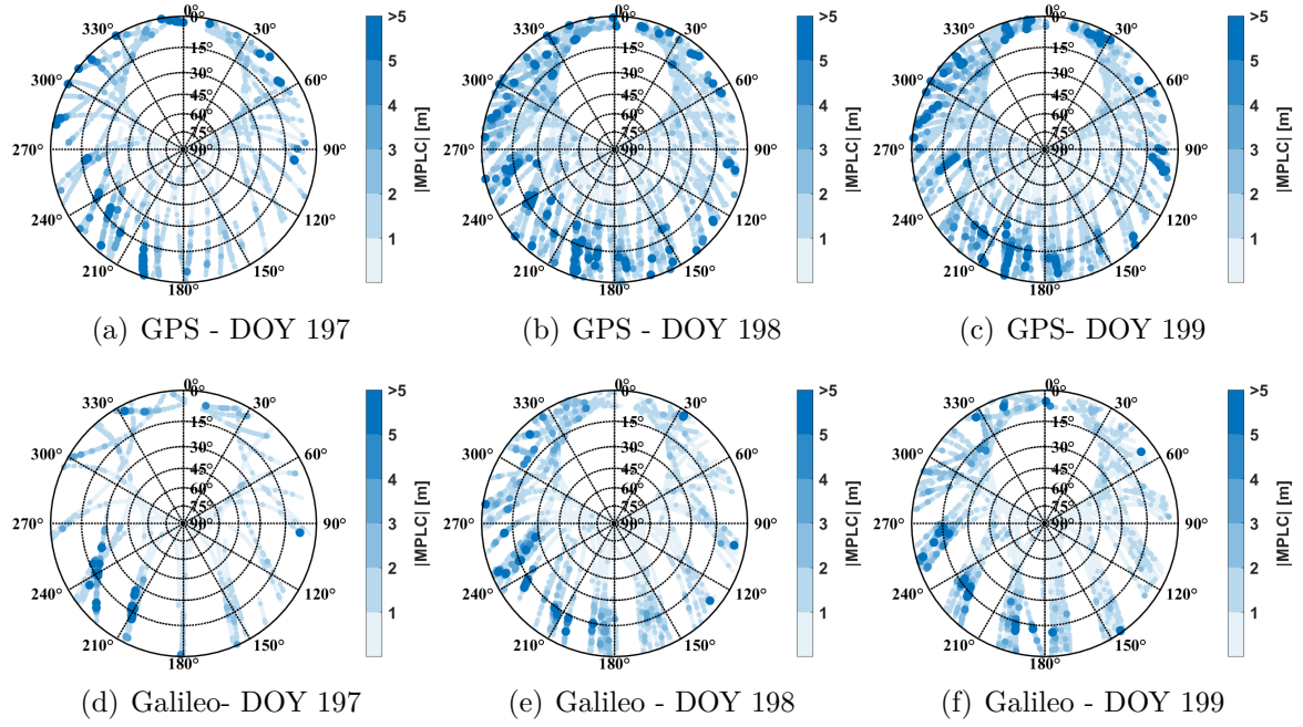
Figure 5.4: Absolute MPLC values in topocentric frame for GPS with the signals C1C, L1C and L2W (top) and for Galileo with C1C, L1X and L5X (bottom) for a category 2 antenna. The data were observed within a calibration from DOY 197 (left) to DOY 199 (right). Please note that only 11 hours are used in DOY 197.
