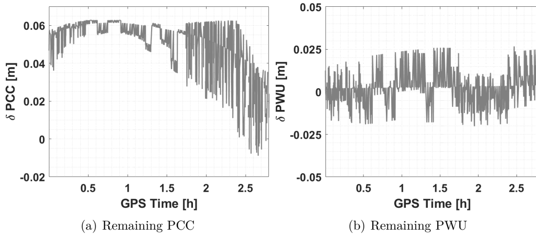
Figure 6.10: Corrections applied to MPLC for GPS satellite PRN18.
