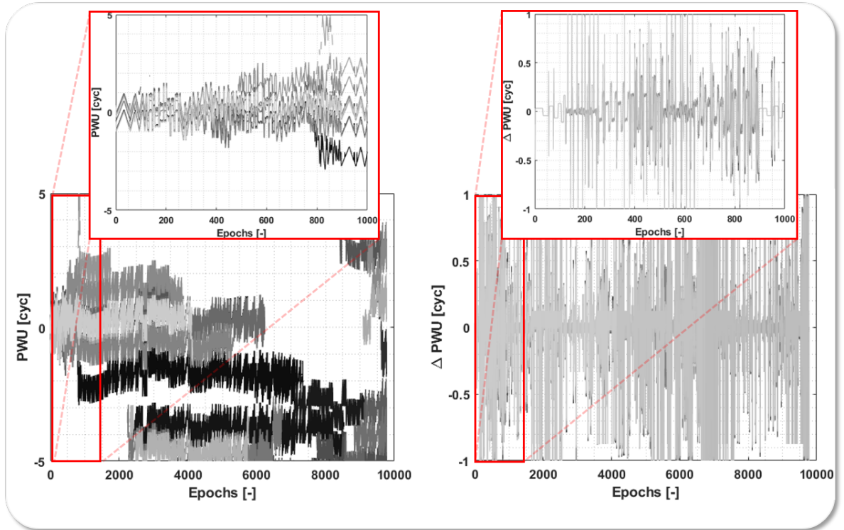
Figure 3.14: The left figures show the PWU caused by the robot motion during the antenna calibration after the cycle slip fixing. The right figures show the corresponding time differenced PWU.
