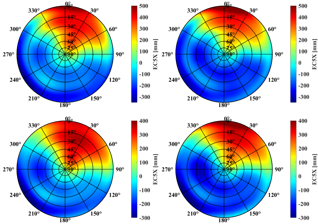
Figure A.11: Mean CPC pattern of the category 3 antenna for the Galileo C5 signal. The left subfigures present the results when using a unity weighting, whereas the right subfigures show the pattern when using a C/N_0 dependent weighting with default (top) and optimized receiver settings (bottom). A multipath map threshold of 2m is applied. Please note different scale between.
