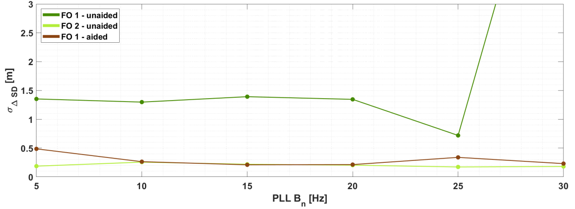
Figure 4.26: Weighted averaged \sigma_{\Delta SD} over all visible satellites for an unaided DLL with filter order 1 (dark green), filter order 2 (bright green) and an aided DLL (brown) with different PLL bandwidth B_n with a fixed DLL bandwidth of 1 Hz.
