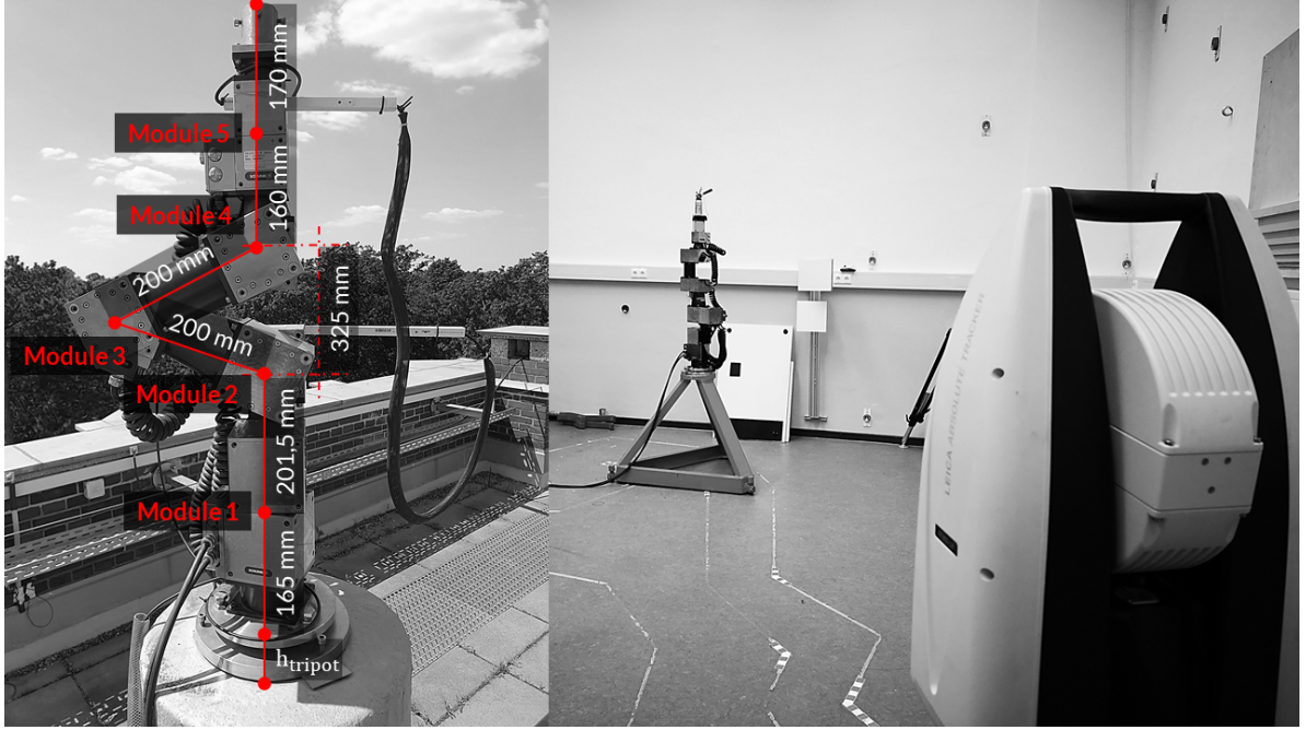
Figure 3.6: Calibration robot mounted on MSD7 with its nominal module lengths in a default calibration position (Left). Calibration of robot within the 3D laboratory from the GIH with a laser tracker in 2022 (Right).
