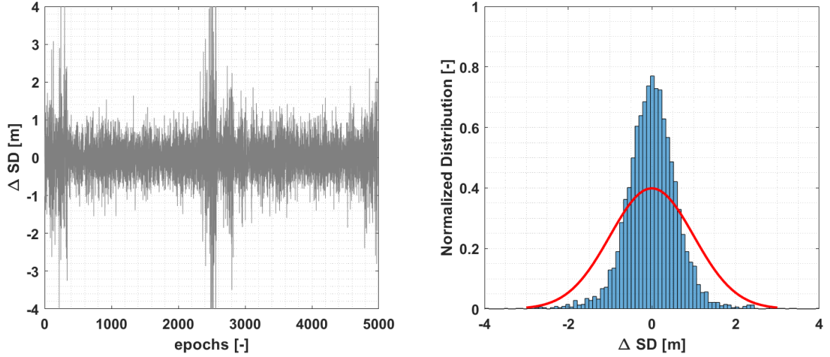
Figure 4.6: Example of the behaviour of GPS C1 \Delta SD from GPS PRN11 (left) for u-blox ANN-MB1 antenna during a robot calibration. (Right) Distribution of the \Delta SD in blue and standard normalized distribution in red.
