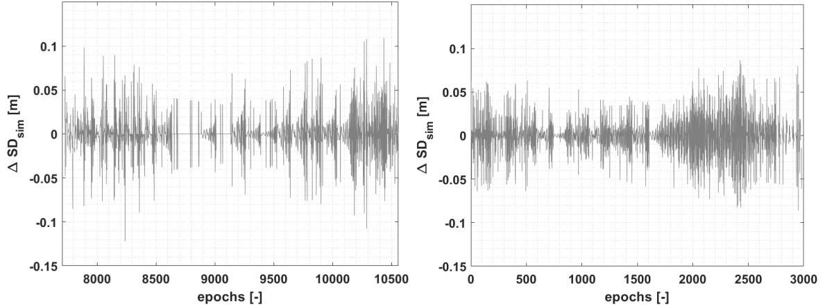
Figure 4.2: Example of the behaviour of GPS C1 \Delta SD_{sim} from GPS PRN10 (left) and PRN24 (right) for a LEIAR25.R3 antenna during a robot calibration.
