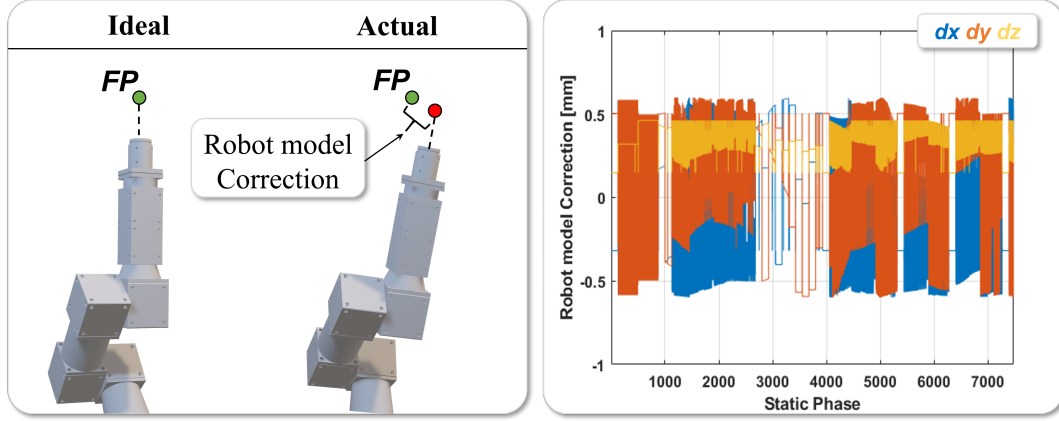
Figure 3.7: Sketch of the displacement between actual FP (red dot) and ideal FP (green dot) within a calibration process (left). Amount of three-dimensional robot model correction (displacement) in millimeters in robot resting phases during a standard antenna calibration (right).
