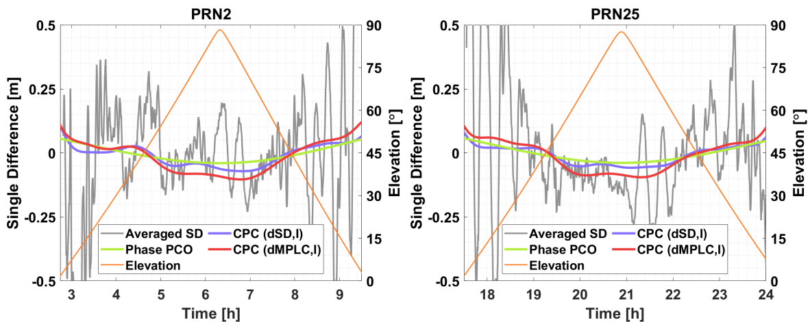
Figure 6.29: Moving average single differences of GPS satellite PRN2 (left) and PRN25 (right) in grey, with different CPC.
