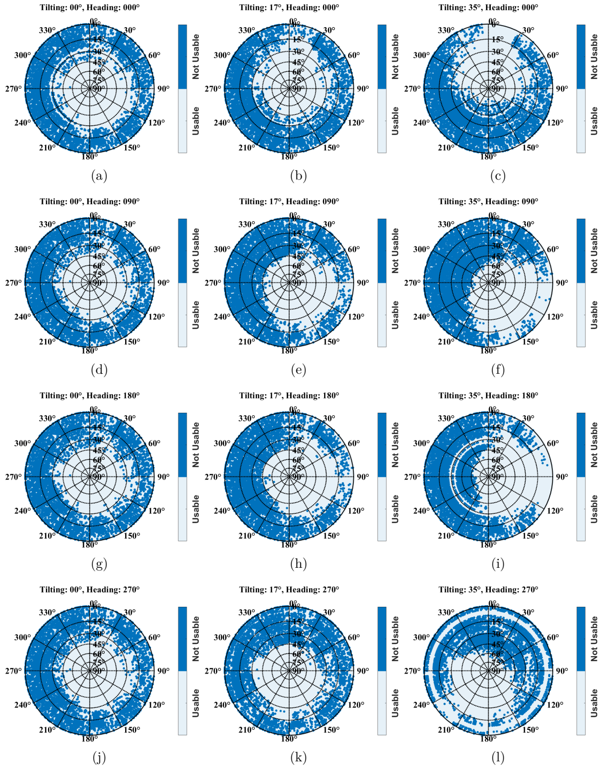
Figure 5.16: Multipath map for the Novatel antenna in different tilting and heading scenario with a threshold of 2 m.
