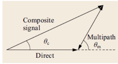
Figure 2.7: Sketch of the phasor diagram with the direct and multipath phasor. Their vector sum defines the composite signal (Braasch, 2017).
