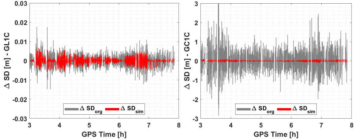
Figure 4.5: \Delta SD (grey) and simulated \Delta SD (red) from a calibration of an LEIAR25.R3 NONE (S/N: 9330001) for the GPS L1 (left) and C1 signal (right). The GPS satellite PRN25 is depicted. The calibration has been carried out with a Javad Delta TRE G3T receiver with default settings.
