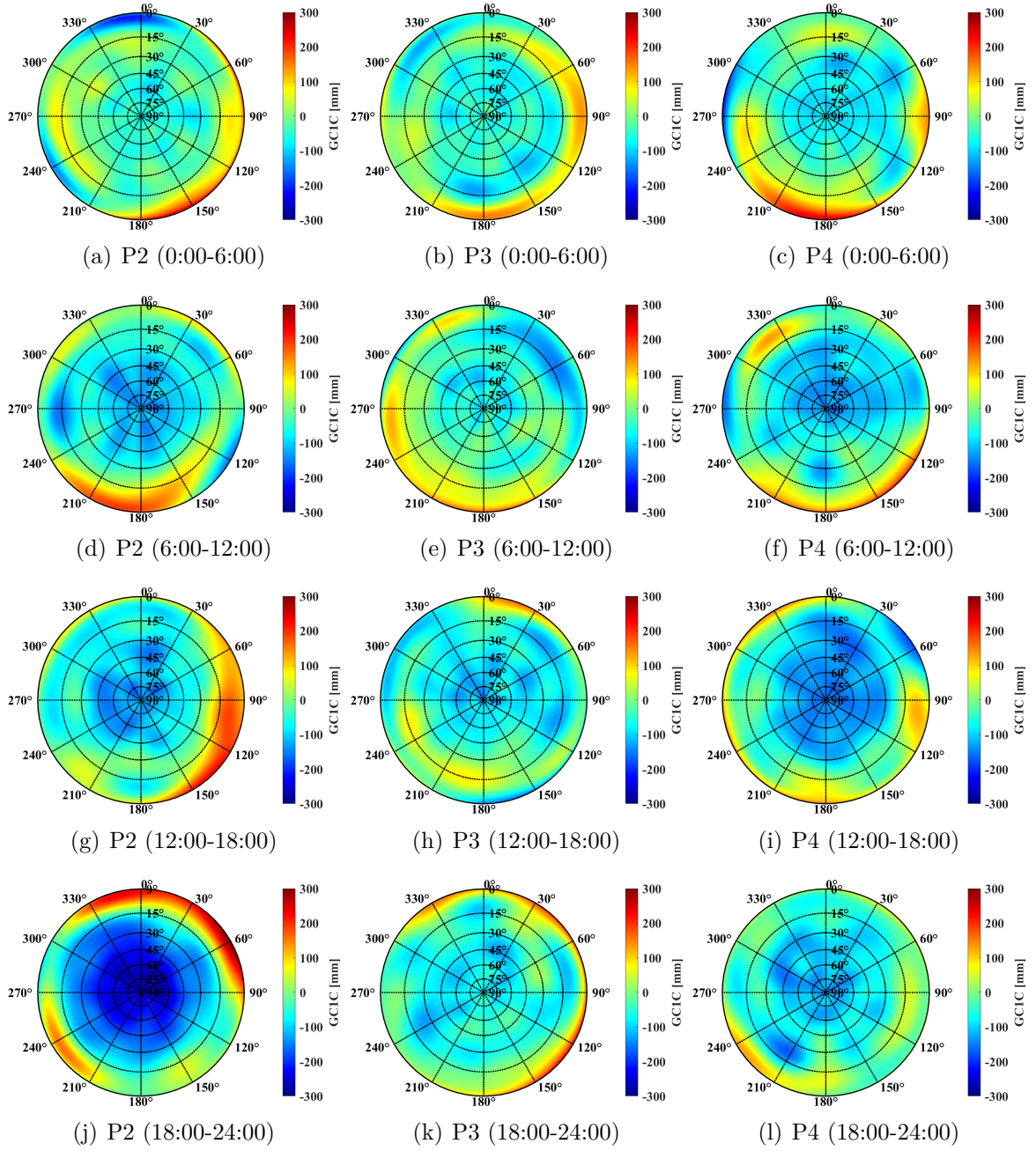
Figure 6.9: Estimated individual CPC pattern for GPS C1 calibrated with optimized receiver settings in 6-hour intervals extracted from P2 (left), P3 (middle) and P4 (right).
