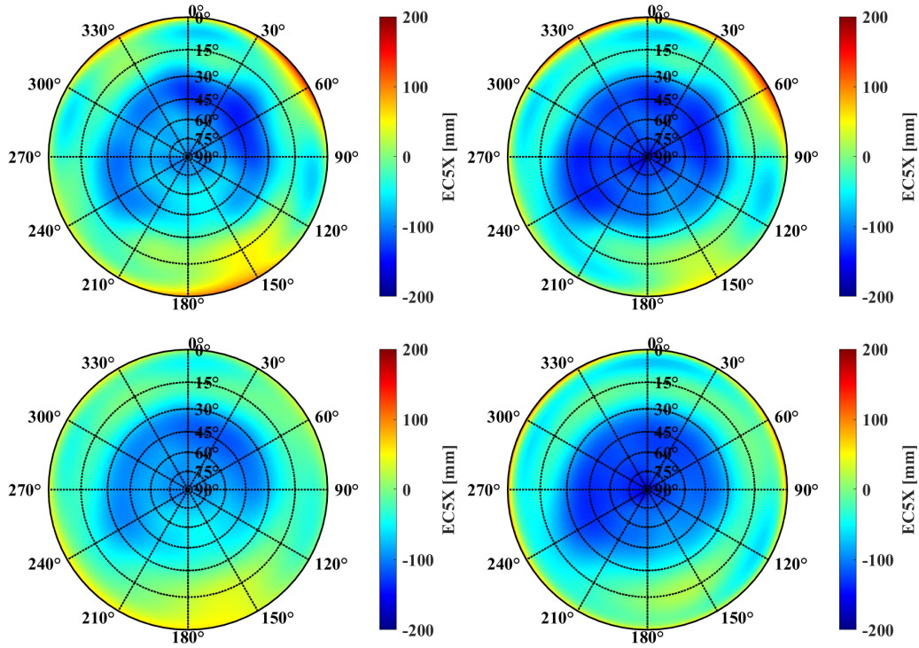
Figure A.6: Estimated mean pattern of Galileo C5, calibrated with default (top) and optimized (bottom) receiver settings with \Delta\text{SD} as estimation inputs (left) and \Delta\text{MPLC} (right) with multipath map threshold of 1.5 m.
