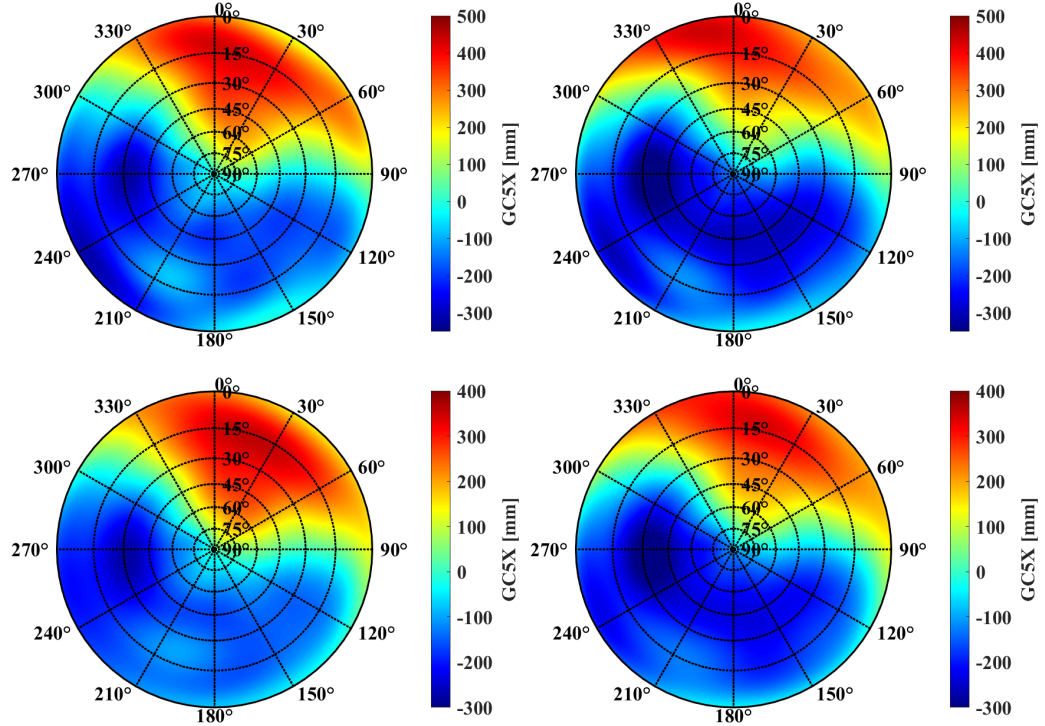
Figure A.9: Mean CPC pattern of the category 3 antenna for the GPS C5 signal. The left subfigures present the results when using a unity weighting, whereas the right subfigures show the pattern when using a C/N_0 dependent weighting with default (top) and optimized receiver settings (bottom). A multipath map threshold of 2 m is applied. Please note different scale between.
