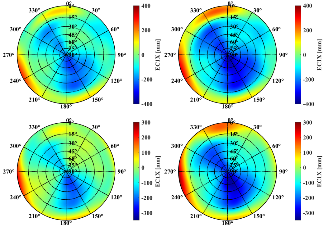
Figure A.10: Mean CPC pattern of the category 3 antenna for the Galileo C1 signal. The left subfigures present the results when using a unity weighting, whereas the right subfigures show the pattern when using a C/N_0 dependent weighting with default (top) and optimized receiver settings (bottom). A multipath map threshold of 2m is applied. Please note different scale between.
