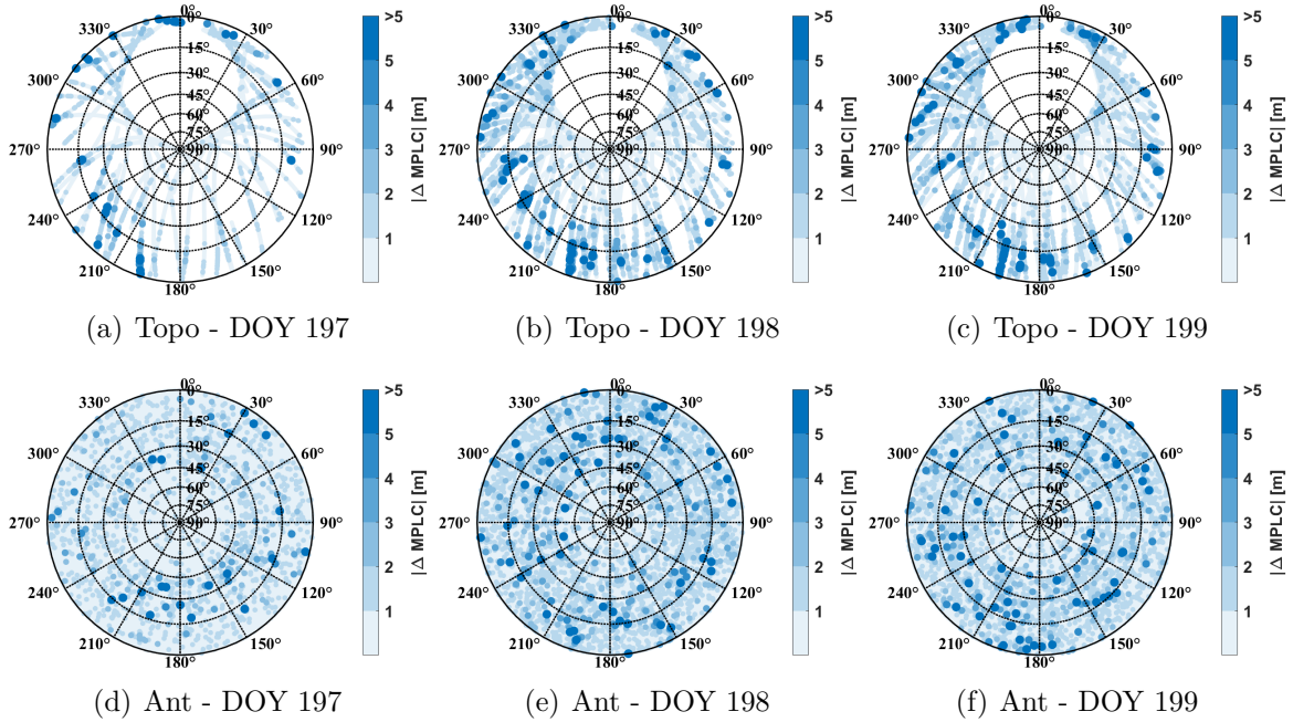
Figure 5.6: Absolute \Delta MPLC values in topocentric (top) and antenna frame (bottom) for GPS with the signals C1C, L1C and L2W (top) for a category 2 antenna. The data were observed within a calibration from DOY 197 (left) to DOY 199 (right). Please note that only 11 hours are used in DOY 197.
