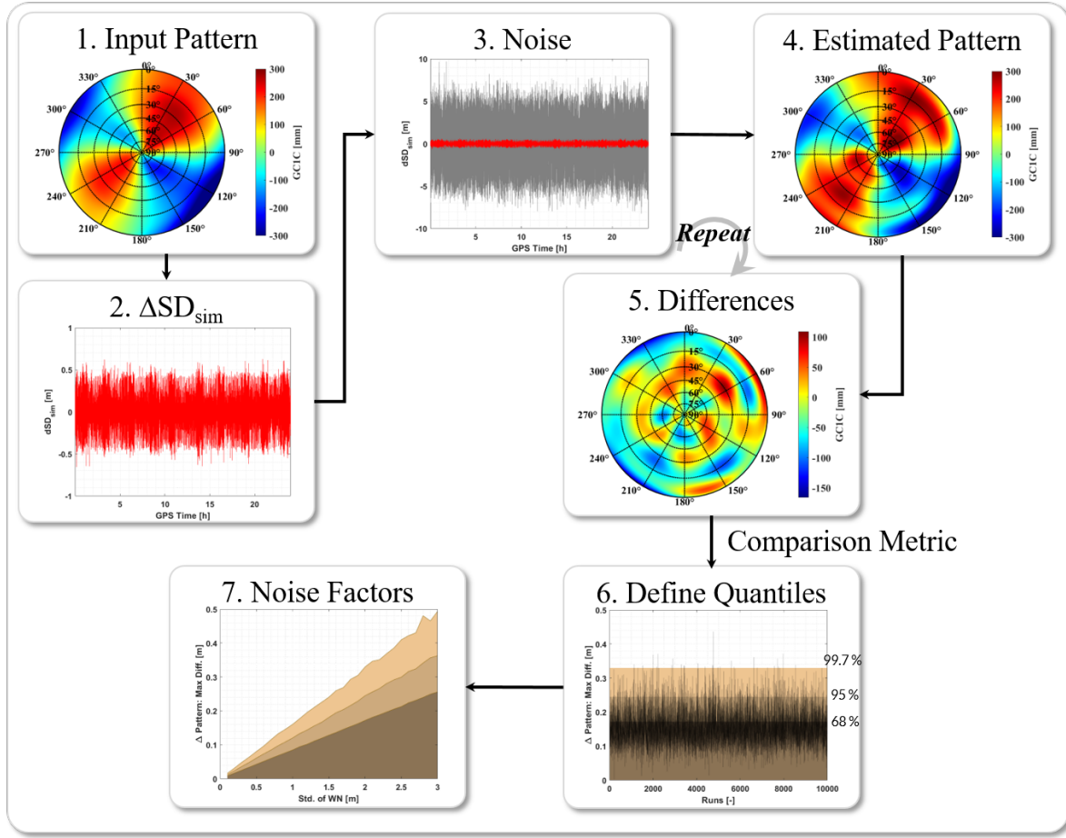
Figure 4.18: Workflow of noise simulation analysis.
