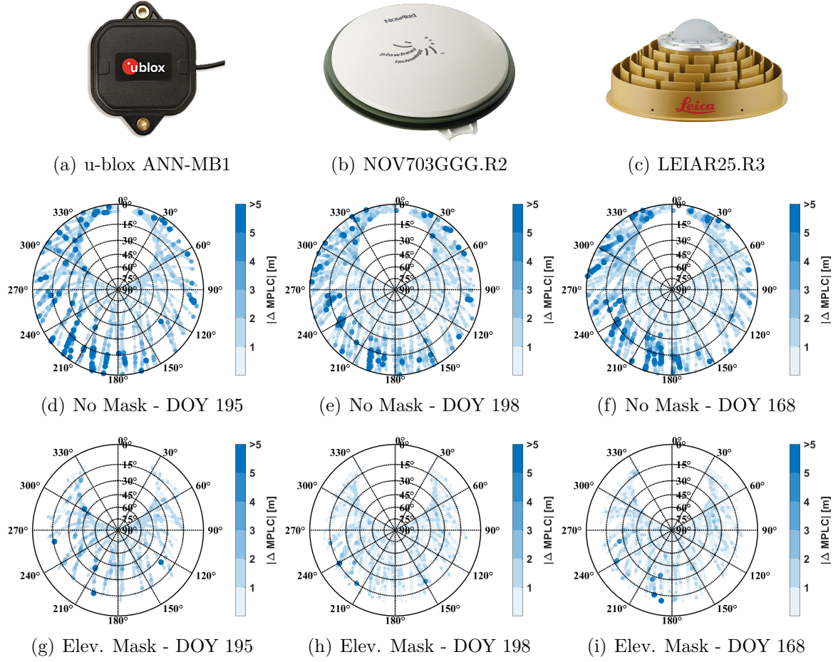
Figure 5.9: Absolute \Delta\text{MPLC} values in topocentric frame for GPS with the signals C1C, L1C and L2W for Novatel and Leica and L5X for u-blox antenna. Each column represents one antenna. The middle row shows the \Delta\text{MPLC} without an elevation mask, the data in the last row are calculated using the dynamic elevation mask [Antenna pictures: U-Blox AG (2024), Novatel (2011), Leica Geosystems AG (2024)].
