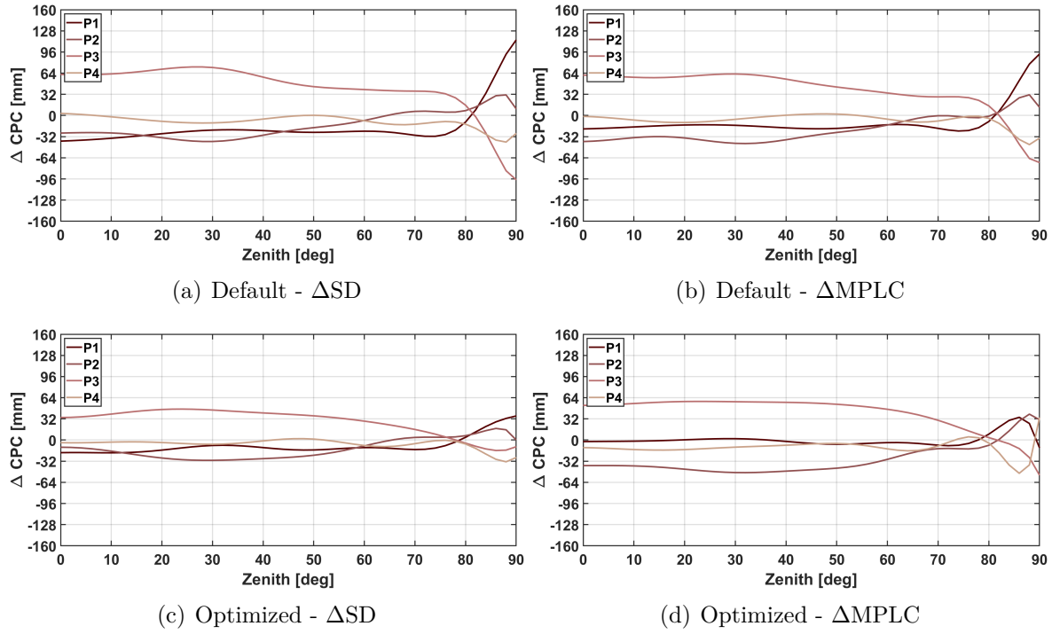
Figure 6.14: Comparison w.r.t to mean CPC pattern for GPS C1. The elevation dependent pattern (NOAZI) is presented, calibrated with default (top) and optimized (bottom) receiver settings with \Delta SD as estimation inputs (left) and \Delta MPLC (right) with multipath map threshold of 1.5 m.
