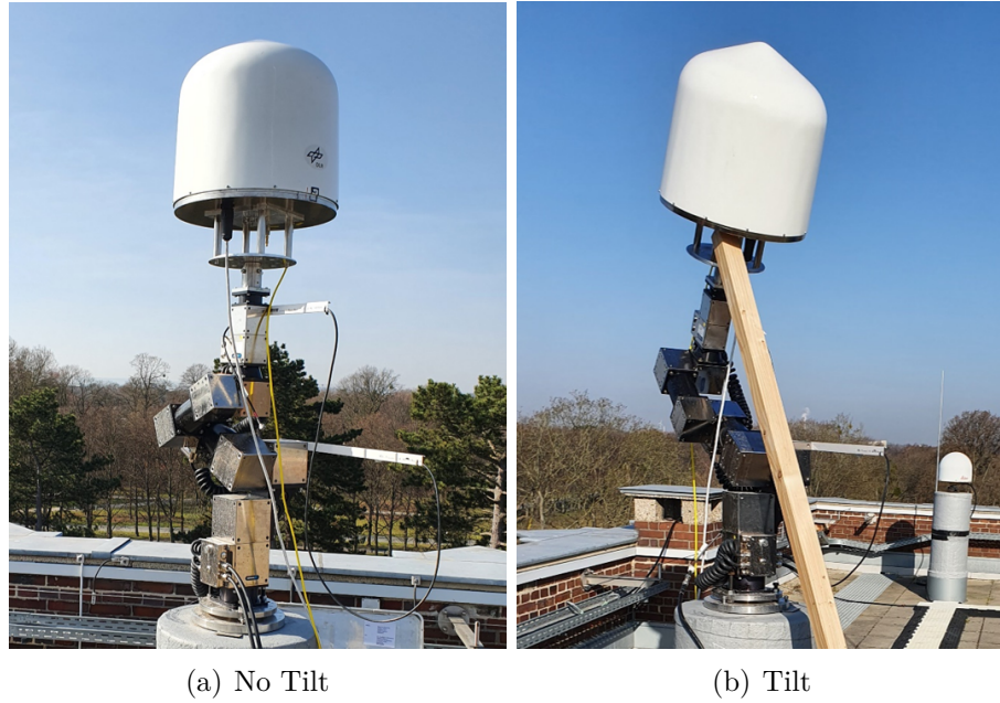
Figure 5.13: Experimental setup of DLR's antenna probe on the antenna calibration robot.
