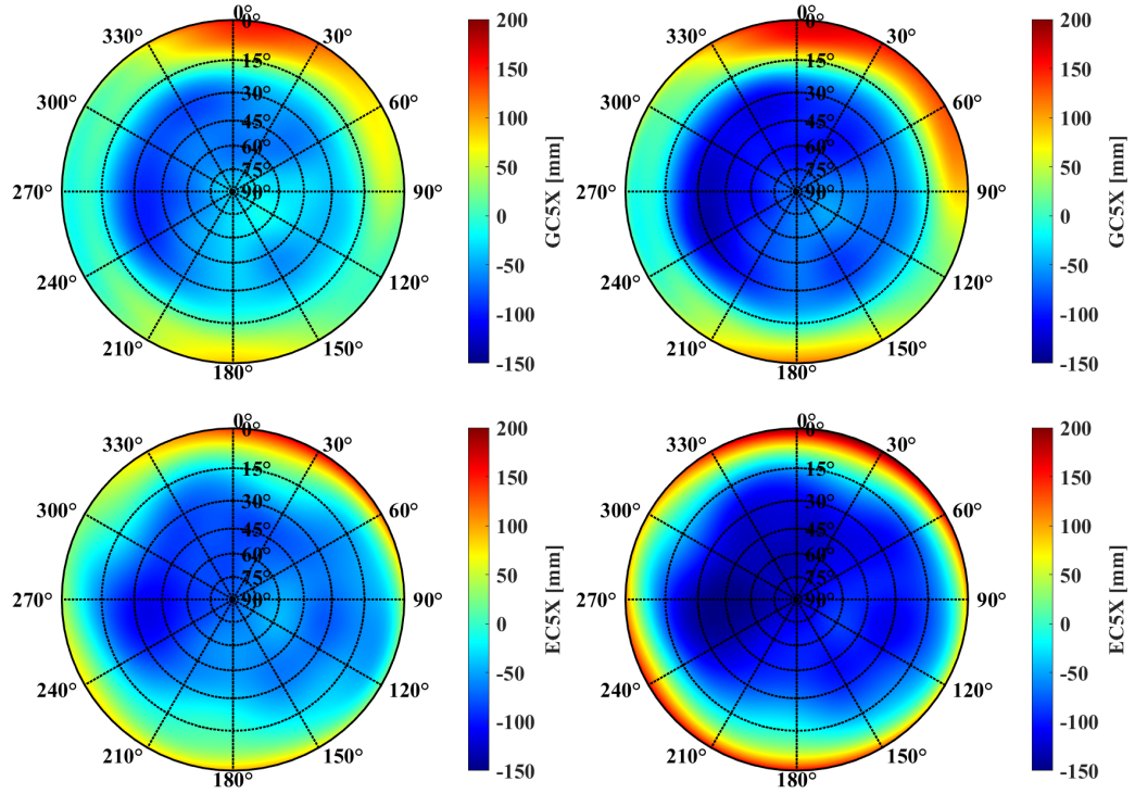
Figure A.8: Mean CPC pattern of the category 1 antenna for GPS C5 (top) and Galileo C5 signal (bottom). The left subfigures presented the results using a unity weighting, whereas the right subfigures show the pattern when using a C/N_0 dependent weighting. Optimized receiver settings are used with a multipath map threshold of 2 m.
