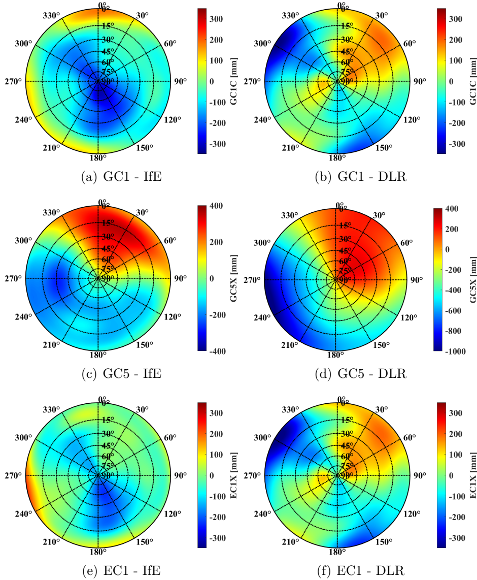
Figure 6.23: Estimated Mean CPC pattern for GPS C1 (a) and C5 (c) and Galileo C1 (e) calibrated at IfE with optimized receiver settings and calibrated in an anechoic chamber by DLR (b, d, f) for a category 3 antenna.
