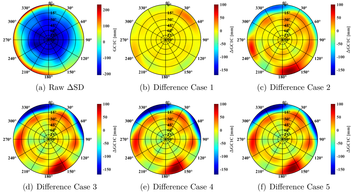
Figure 6.3: Impact of different observation elimination techniques on the CPC. GPS C1 CPC pattern with raw \Delta SD are presented in (a), whereat the other plots show the differences to pattern (a) by applying different elimination techniques, defined as particular cases earlier.
