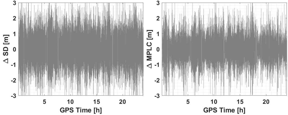
Figure 3.15: \Delta SD from a calibration of an u-blox ANN-MB1 NONE (S/N:2133) for the GPS C1 signal (Left) and \Delta MPLC of the same calibration (right). All visible satellites are presented by overlapping.
