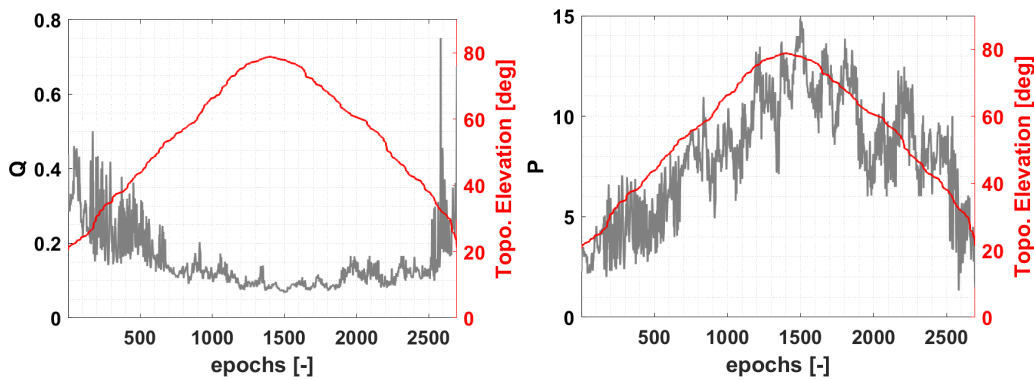
Figure 6.17: Example of the diagonal elements of the cofactor matrix Q (left) and weighting matrix P (right) for GPS satellite PRN1 during a calibration of a category 1 antenna using optimized receiver settings and a C/N_0 dependent weighting for the GPS C1 signal.
