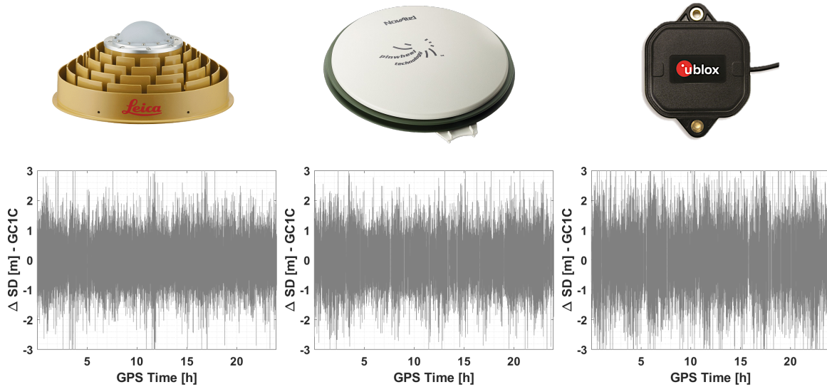
Figure 4.9: \Delta\text{SD} from a calibration for a category 1 (left), category 2 (middle) and category 3 (right) antenna. The calibrations have been carried out with two Javad Delta TRE G3T receivers with manufacture's default settings. The GPS C1 signal from all visible satellites are plotted [Antenna pictures: Leica Geosystems AG (2024); Novatel (2011); U-Blox AG (2024)].
