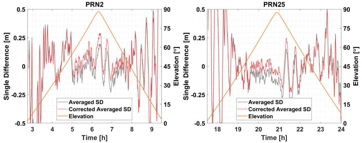
Figure 6.30: Moving average single differences of GPS satellite PRN2 (left) and PRN25 (right) in grey, and by applying CPC in red.
