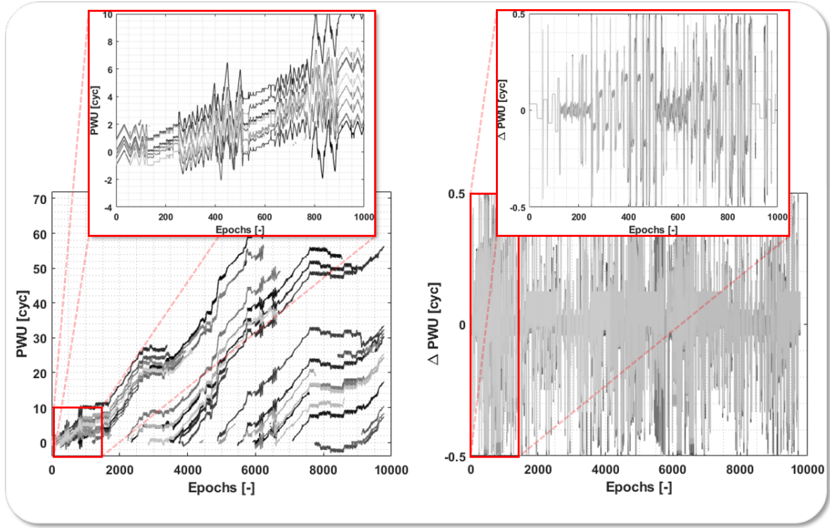
Figure 3.12: The left figures show the PWU caused by the robot motion during the antenna calibration. The right figures show the corresponding time differenced PWU.
