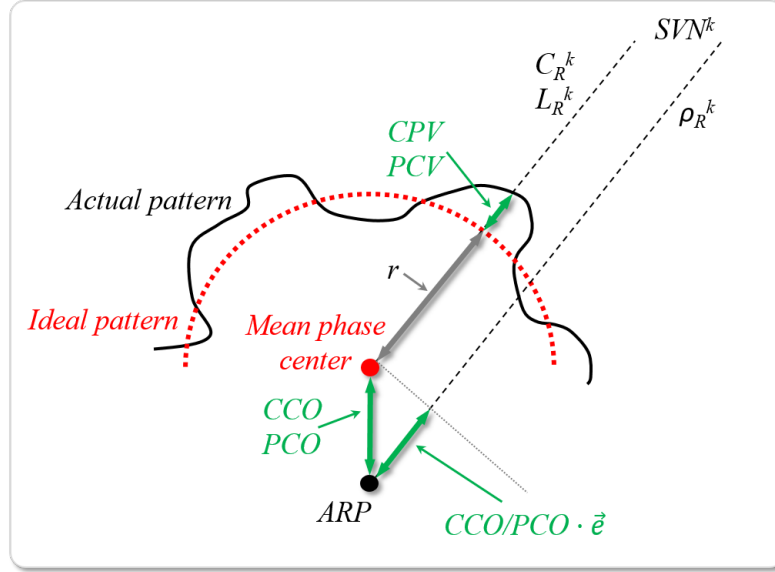
Figure 3.1: Geometric interpretation of CCO/PCO, CPV/PCV and parameter r .
