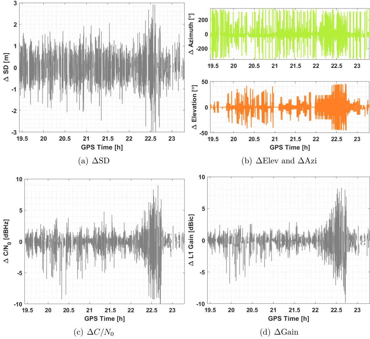
Figure 4.7: Example of the relation between C1 \Delta SD (a) and the signal strength (c) and antenna gain (d) from GPS PRN22 for an u-blox ANN-MB1 antenna during a robot calibration. The azimuth and elevation changes in the antenna frame for this satellite is presented in (b).
