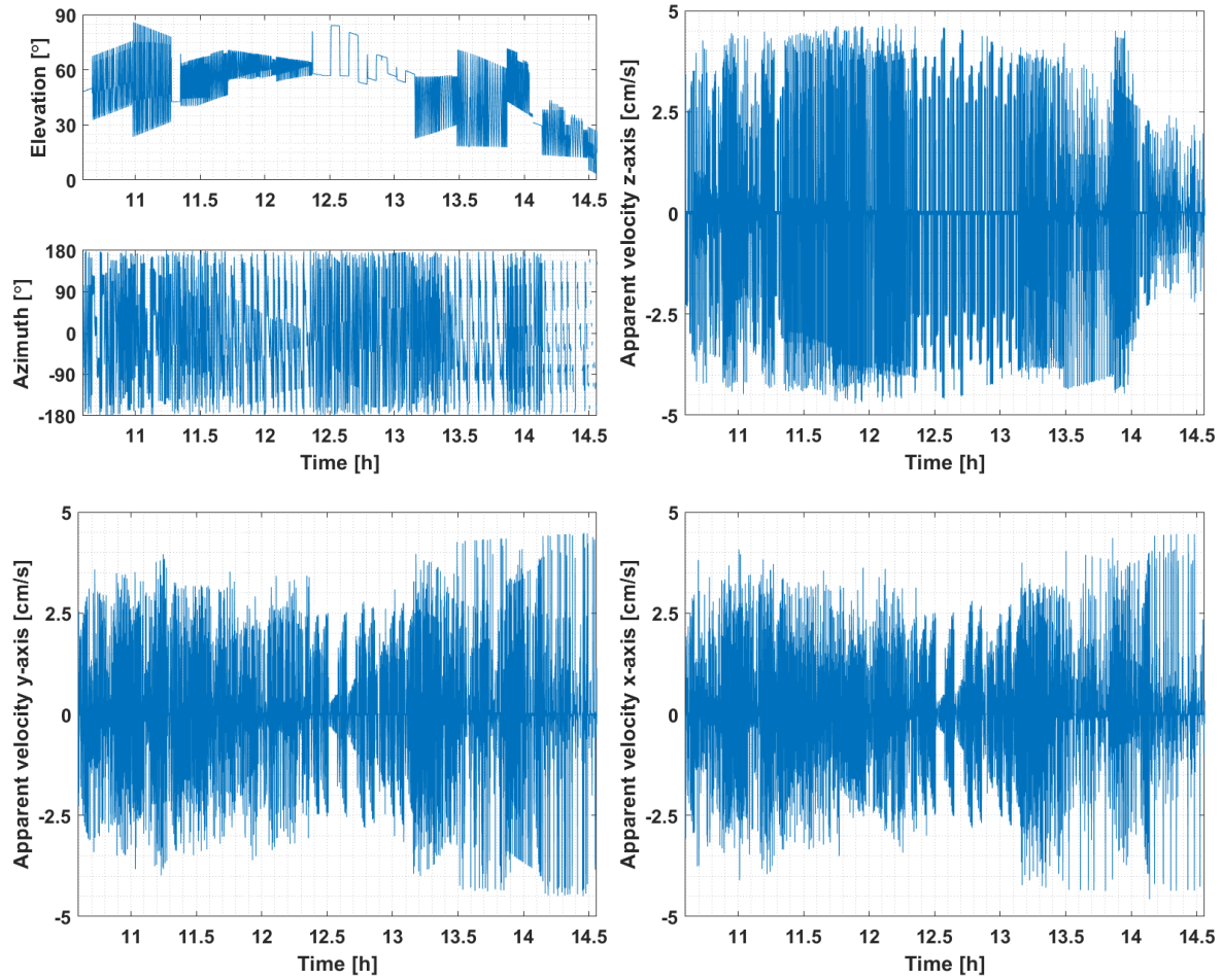
Figure 4.17: Robot module angles during a calibration (top) with the measured angular rates from the IMU (bottom).
