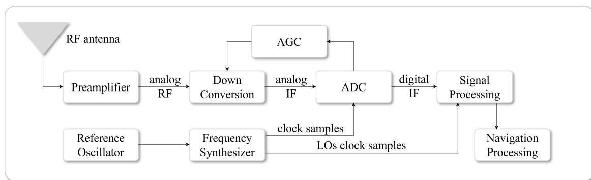
Figure 2.2: Principal components of a GNSS receiver based on Häberling (2016).
