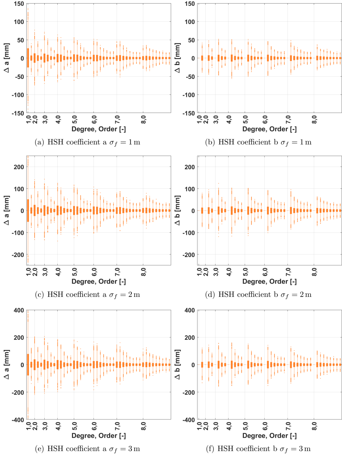
Figure 4.23: Differences of HSH coefficients a_{nm} (left) and b_{nm} (right), when \sigma_f = 1 m (a, b), \sigma_f = 2 m (c, d) and \sigma_f = 3 m (e, f) is added. The x-axis shows degree and order of the coefficient starting from e.g. 7,0 to 7,7 with 7,1 ... 7,6 in between. Please note the different y-axis scales.
