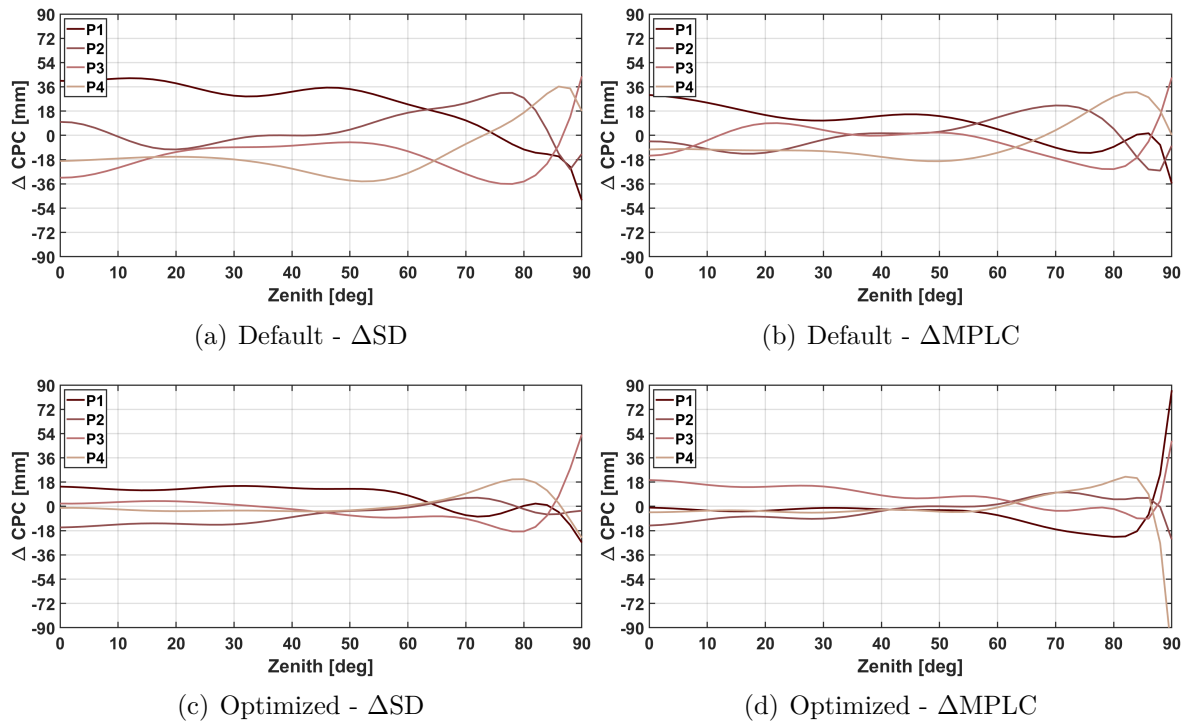
Figure 6.15: Comparison w.r.t to mean CPC pattern for Galileo C1. The elevation dependent pattern (NOAZI) is presented, calibrated with default (top) and optimized (bottom) receiver settings with \Delta SD as estimation inputs (left) and \Delta MPLC (right) with multipath map threshold of 1.5 m.
