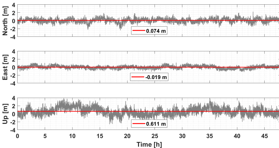
Figure 6.25: Estimated topocentric coordinates w.r.t the reference ITRF2020 coordinates at epoch 27.09.2024 (MSD7) for the category 1 antenna with no additional CPC. The mean value is presented in red.
