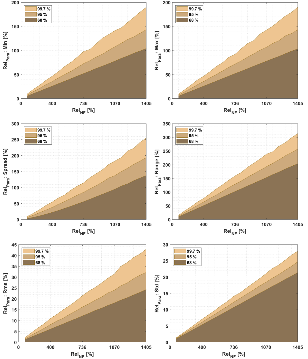
Figure A.3: Results for relative comparison metrics for the category 1 antenna with additional C/N_0 noise, based on input pattern in Figure A.1 with different noise factors. Because the noise factor is varying up to 2 m and P_{Peak} is 149.44 mm, Rel_{NF} is varying to 1405%.
