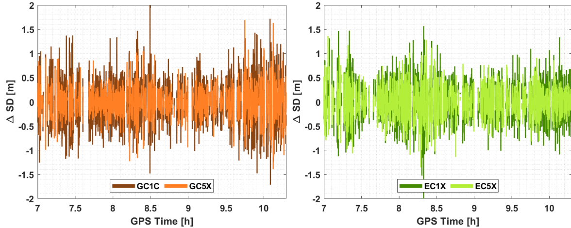
Figure 4.12: \Delta SD of the GPS C1 and C5 signal of the satellite PRN10 from a category 2 antenna calibration (left) and Galileo C1 and C5 signal of the satellite PRN26 (right). The calibration has been carried out with a Javad Delta TRE G3T receiver with default settings.
