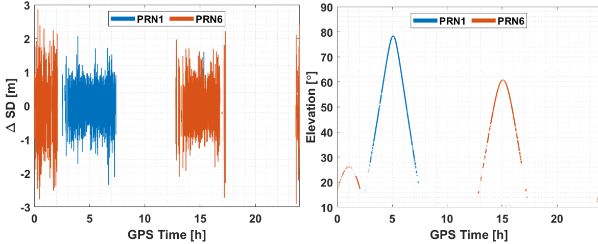
Figure 4.11: C1 \Delta SD for GPS satellite PRN1 and 6 (left) and their corresponding topocentric elevation (right) for a category 2 antenna.
