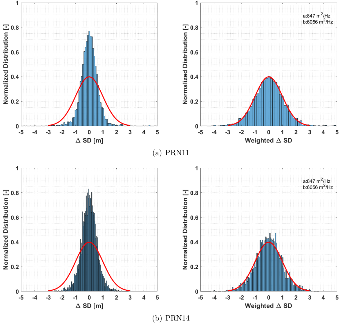
Figure 4.8: \Delta SD distribution of the GPS C1 signal of satellite PRN11 (a) and PRN14 (b) for an u-blox ANN-MB1 antenna before (left) and after (right) C/N_0 weighting. The standard normal distribution is presented in red ( \sigma = 1 m).
