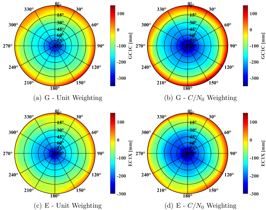
Figure 6.18: Mean CPC pattern of the category 1 antenna for GPS C1 (top) and Galileo C1 signal (bottom). Subfigure (a) and (c) presented the results using a unit weighting, whereas (b) and (d) shows the pattern when using a C/N_0 dependent weighting. Optimized receiver settings are used with a multipath map threshold of 2 m.
