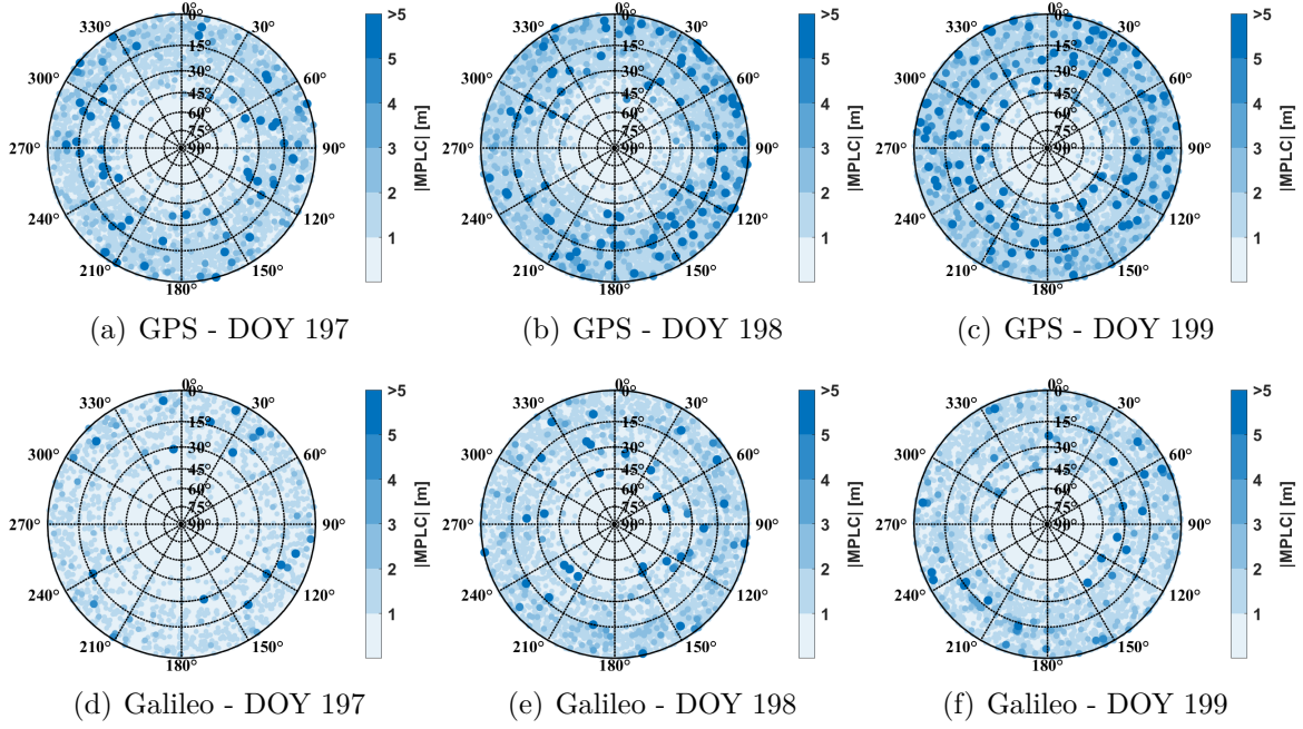
Figure 5.5: Absolute MPLC values in antenna frame for GPS with the signals C1C, L1C and L2W (top) and for Galileo with C1C, L1X and L5X (bottom) for a category 2 antenna. The data were observed within a calibration from DOY 197 (left) to DOY 199 (right). Please note that only 11 hours are used in DOY 197.
