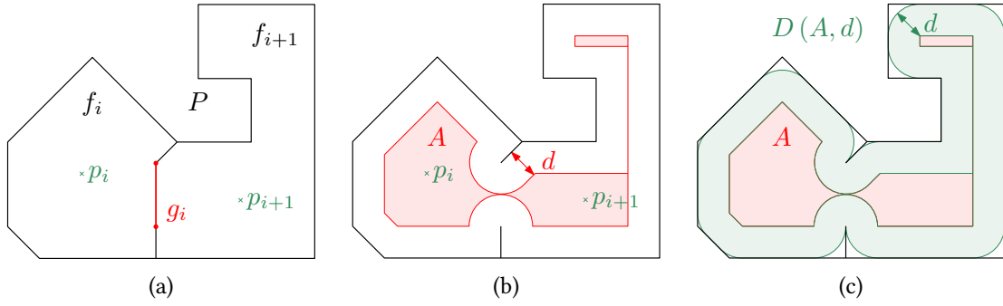
Figure 10.6: (a) Two faces f_i and f_{i+1} that are incident to each other and share a common gate g_i . By removing g_i , we get a face P . (b) The buffer distance d is the largest distance that can be buffered inside of P such that the resulting geometry A is connected, contains a point on g_i , and contains p_i and p_{i+1} . (c) The area within distance d of A (green) is contained inside of P , and all grid points covered by it are octilinearly connected if the underlying grid has a grid spacing of w = 2d .
