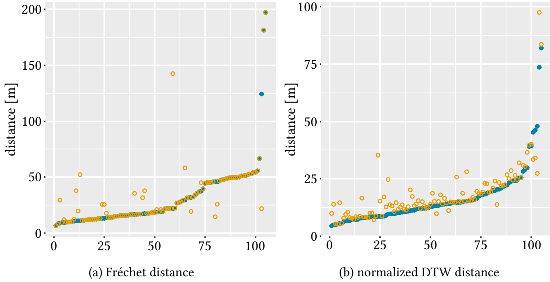
Figure 4.7: Fréchet distance (a) and normalized DTW distance (b) between input trajectories and the matched paths produced with the tessellation-based approach (blue) and Baseline+ (orange). In both cases, the trajectories (distributed over the x-axis) are sorted by the Fréchet distance (resp. normalized DTW distance) of the tessellation-based approach.
