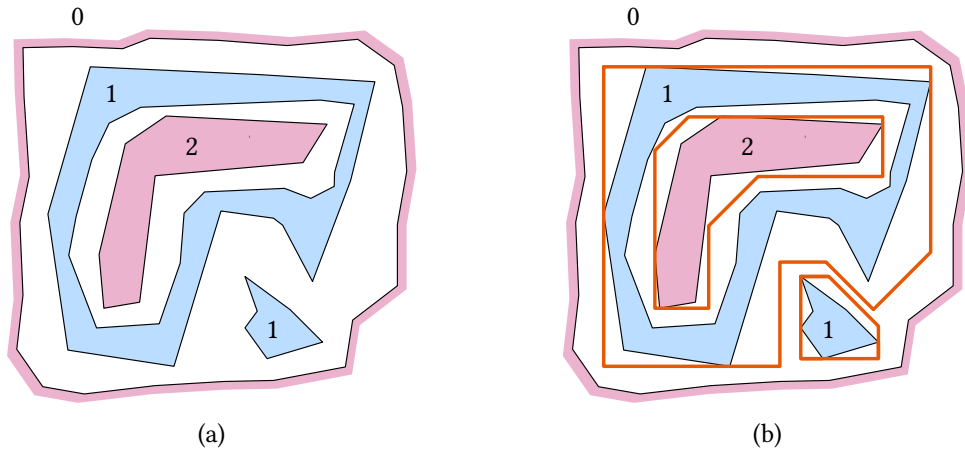
Figure 9.13: The reachable (blue) and unreachable (red) parts of the road graph consist of multiple components. (a) Each component has a level. (b) Each internal component is enclosed by a schematized polygon.
