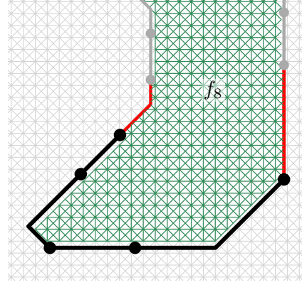
Figure 10.4: For each face (here f_8 ), a grid graph (green) is extracted from a pre-computed grid (light grey). At gates (red), the grid graph can touch the outer boundary of the face.
