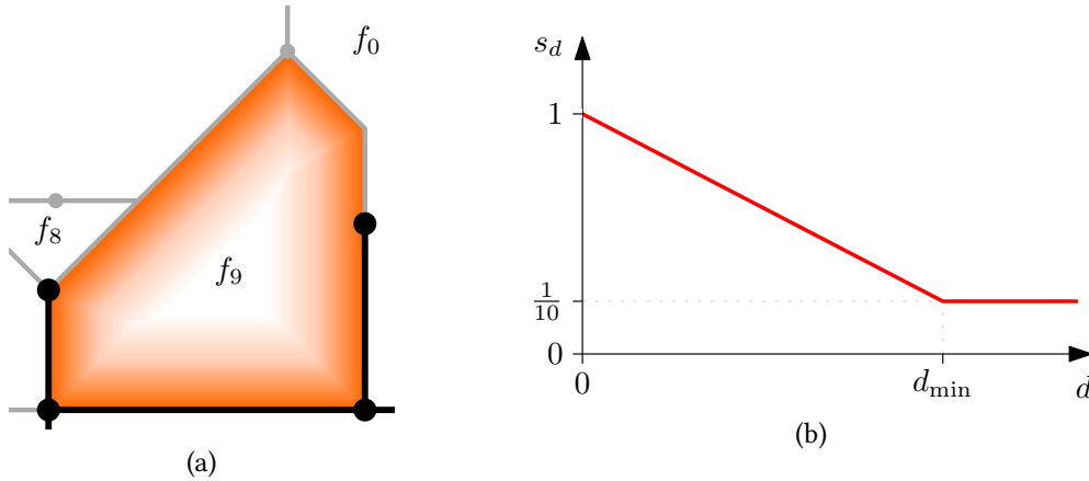
Figure 10.8: (a) Visualization of the distance to boundary cost (orange). The cost is the highest at the face boundary, while it is neutral in the face center. (b) The distance to boundary scale factor s_d . Edges closer to the face boundary than d_{\min} are penalized.
