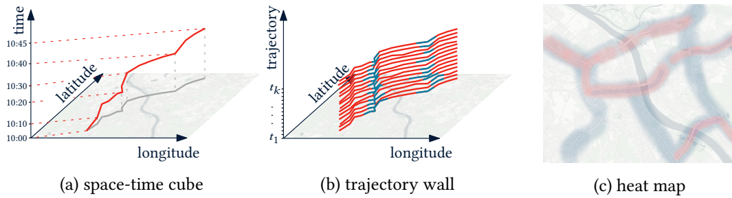
Figure 7.2: Sketches for different visualization approaches for trajectories. (a) In the space-time cube, the vertical dimension indicates time. (b) In the trajectory wall, the vertical dimension displays multiple trajectories. Additional properties like transportation mode (e.g., blue for walking and red for running) can be color-coded to improve exploration. (c) In heat maps, the point density is displayed, making identifying areas with high activity easy. Background map: ©OpenStreetMap contributors ©CARTO
