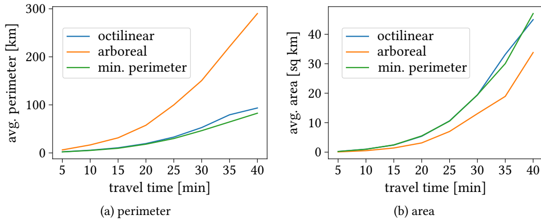
Figure 9.18: Perimeter and area for different visualization types.
