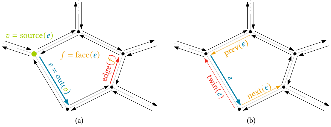
Figure 2.5: A doubly connected edge representation of the graph is shown in gray. (a) Pointers between the DCEL elements (vertices, half edges, and faces) store their topological relationship. (b) Each half edge stores pointers to neighboring half edges to allow navigating the graph.
