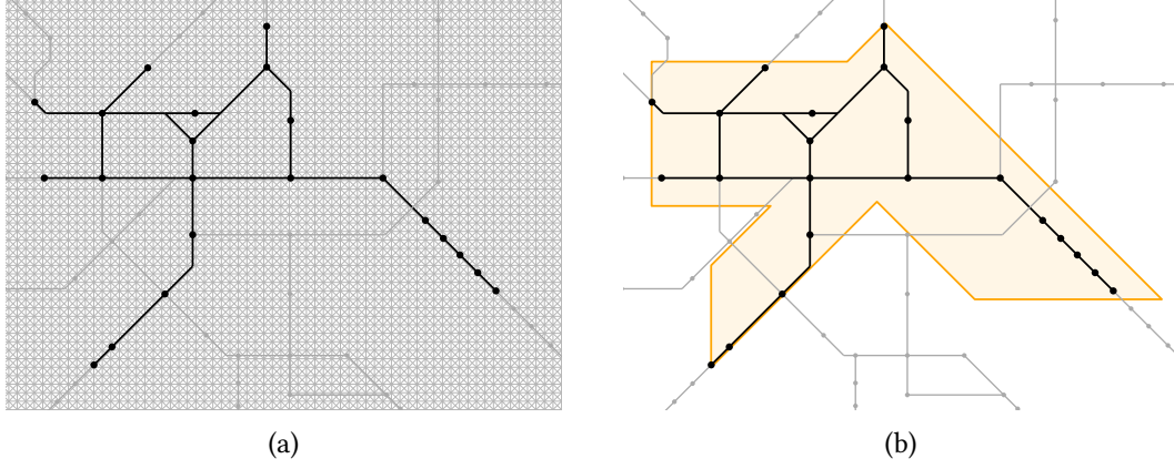
Figure 10.9: Evaluation instance showing the tram network of Cologne. (a) Reachable stations (black) and grid (light grey). (b) Polygon enclosing the reachable stations with a minimal number of bends.
