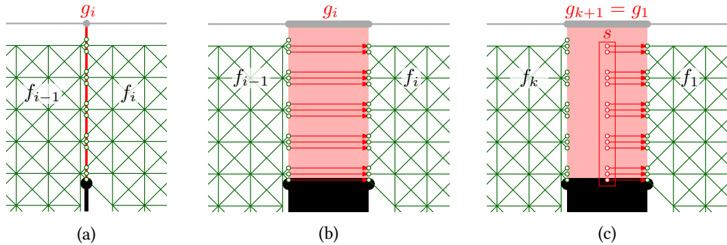
Figure 10.5: Creating the routing graph \mathcal{R} . (a) Along gates (red), the grid graph is extracted so its edges touch the gate. (b) Detailed view of the gate. Two gate vertices of consecutive grid graphs are connected by a gate edge (red). (c) The first and last grid graphs are not connected. Instead, the source vertices s are added.
