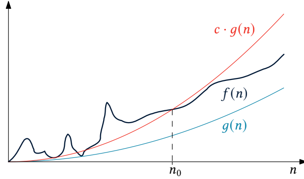
Figure 2.1: Illustration of the upper bound relationship denoted by the O -notation. The function f is O(g) (here: g = n^2 ) as a constant multiple of g bounds its growth rate for n > n_0 . The function f may represent the exact running time of an algorithm, which, in general, is not feasible to compute. The O -notation provides a tool for assessing and quantifying the algorithm's efficiency by characterizing its upper-bound behavior instead.
