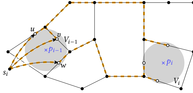
Figure 4.2: The incremental step of our algorithm. From the dummy vertex s_i , the shortest paths to all vertices in V_i are computed with one single-source shortest path query (see the dashed lines). The weight of each path plus the state-based energy of the corresponding terminal is used as the weight of a dummy edge in the next iteration.
