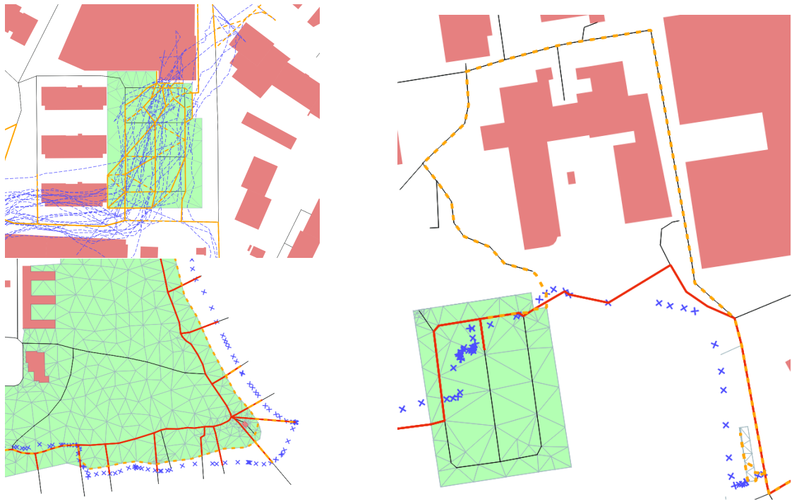
Figure 4.9: Upper left: Trajectories (dashed blue lines) traversing the same free space. The yellow edges indicate their matched paths. Lower left: A trajectory (blue crosses) following the shoreline of the lake. The Baseline+ approach matches this trajectory to far-away paths and several groins, while the tessellation-based approach produces a more sensible match. Right: Without sufficient tessellation edges, a trajectory traversing a large free space might be matched to a path with a rather large detour.
