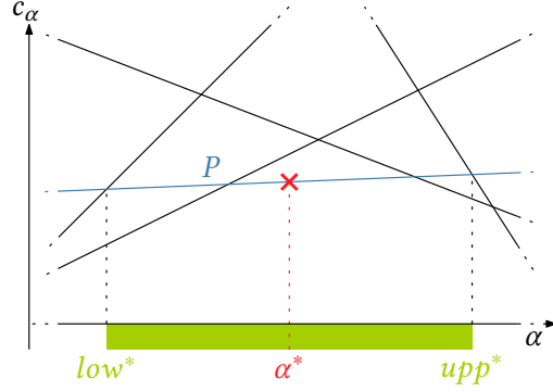
Figure 6.3: The output of WITNESSSEARCH that we use as input for our algorithm: a balance factor \alpha^* for which path P (blue) is \alpha -optimal and the interval I = [low^*, upp^*] (green) that is guaranteed to contain the optimality range I_{opt} of P completely. In specific, low^* and upp^* are values where the line for P crosses another line of the line arrangement and \alpha^* = \frac{low^* + upp^*}{2} .
