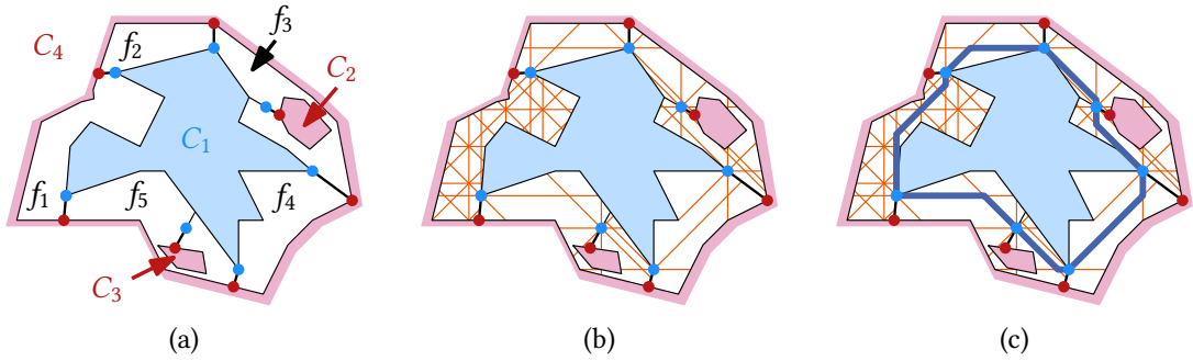
Figure 9.10: Creating an octilinear polygon that encloses the component C_1 (blue) of all reachable vertices and edges. (a) The faces f_1, \dots, f_5 surround the component C_1 . (b) Each face is subdivided by an octilinear grid (Step 1). Furthermore, these grids are connected to one large grid G that is split by the port between f_1 and f_5 (Step 2). (c) An octilinear polygon is constructed by computing a bend-minimal path through G .
