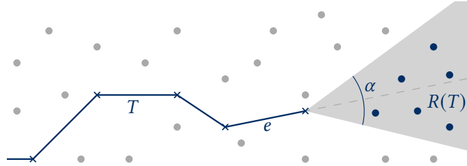
Figure 3.2: Schematic representation of a direction-based attack. The sites (round dots) inside R(T) (colored black) are candidate sites this attack function returns. R(T) is based on the terminating segment e of trajectory T .
