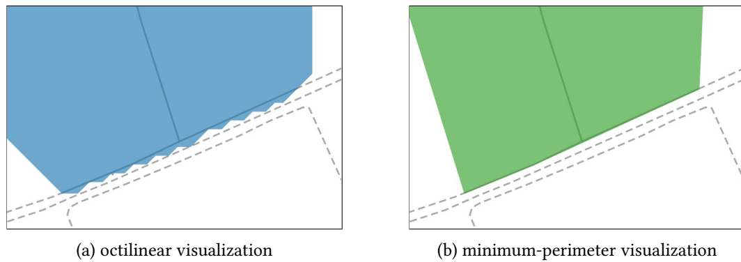
Figure 9.20: In rare cases, the octilinear visualization has a step-like outline, while the minimum-perimeter visualization does not suffer from this.
