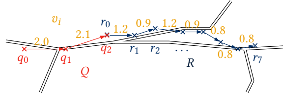
Figure 2.9: The trajectory depicted in Figure 2.8 with velocity per segment (orange). The trajectory is split into two subtrajectories Q (red) and R (blue), using the speed variance as the criterion. Within each subtrajectory, the speed varies by at most one unit. The displayed segmentation is a minimum segmentation for this criterion.
