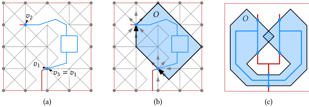
Figure 9.12: Routing step. (a)–(b) The polygon O must not contain unreachable parts. For the routing step the edges incident to ports are directed accordingly. (c) The path O is not necessarily simple.
