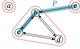
Figure 2.3: Vertex c is reachable from e through path P . The strongly connected components are marked in red.
