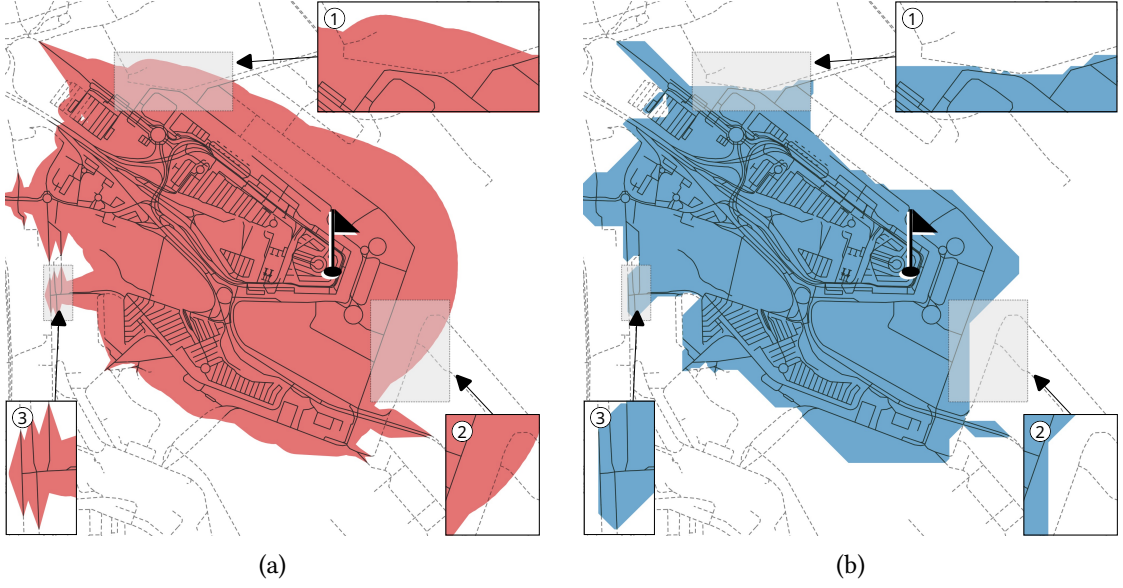
Figure 9.3: A single time-zone of 15 minutes starting at the flag. Unreachable roads are dashed. (a) Time-zone created by buffering the remaining travel time for each point of the road network. ①–②: The time zone covers unreachable roads. ③: Time zone has ramified outgrowths. (b) Time-zone created by our approach. ①–②: Time-zone only covers reachable roads. ③: Schematization simplifies the visualization.
