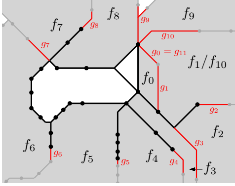
Figure 10.3: The faces in F that separate the reachable component from the unreachable parts of the network are highlighted (grey). They are identified in clockwise order around the component.
