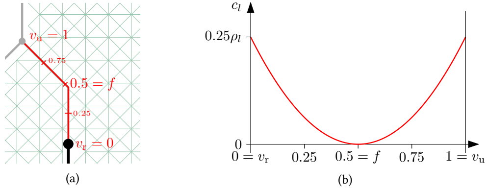
Figure 10.7: (a) A gate g = (v_r, v_u) with visualised fractions. For f = 0.5 , the optimal passage location is precisely in the middle of the gate. (b) The gate passage location cost function c_l for f = 0.5 . At f , the optimal passage location, the cost is zero.
