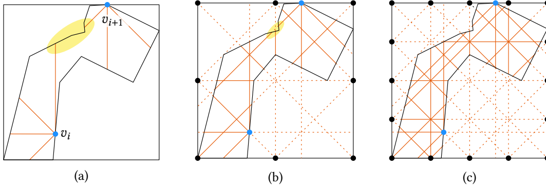
Figure 9.11: The face f_1 of the example shown in Figure 9.10 is subdivided by octilinear rays based on vertices on the bounding box. (a) Shooting octilinear rays from v_i and v_{i+1} does not yield a connected line arrangement (see yellow highlight). (b)–(c) The bounding box of f_1 is successively refined by vertices shooting octilinear rays until they connect v_i and v_{i+1} .
