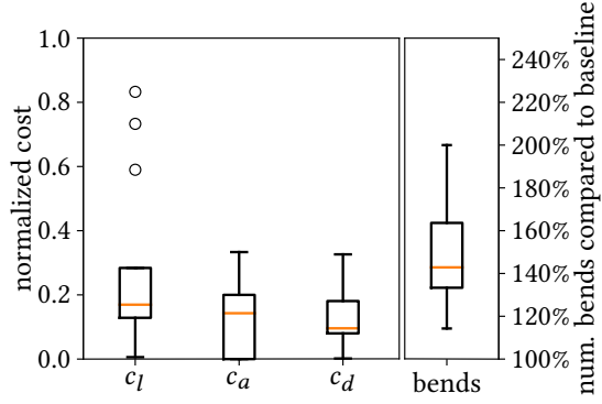
Figure 10.13: Quality for the individual cost functions using c_b^w with \rho_b = 10 , \rho_l = 50 , \rho_a = 14 , and \rho_d = 1 .
