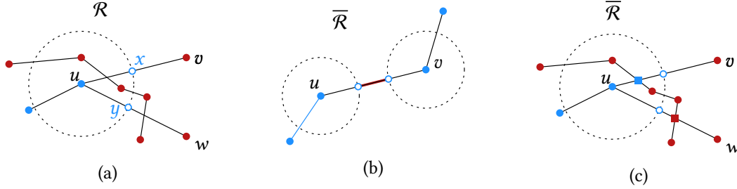
Figure 9.8: The reachability is modeled by subdividing edges. (a) The vertex x (resp. y ) subdivides the edge (u, v) (resp. (u, w) ) at the last reachable position. (b) Special case: The vertices u and v are reachable from different directions. (c) The coloring of \mathcal{R} is transferred to \overline{\mathcal{R}} , and the vertices (squares) introduced for the planarization are colored.
