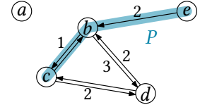
Figure 2.4: A weighted graph with edge weight function w . Path P has a weight of w(P) = 3 according to these weights.
