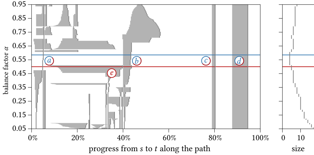
Figure 6.10: (left) Milestone plot for the path presented in Figure 6.9. The milestone segmentations over all \alpha values are shown. The gray marks indicate the milestone positions as found by a forward search. The light gray areas denote the milestone suites for the corresponding milestones. The blue line represents an optimal milestone segmentation at \alpha = 0.58 with milestones in a , b , c , and d . For \alpha = 0.5 (red), an additional milestone in e is needed. (right) The number of milestones needed per \alpha .
