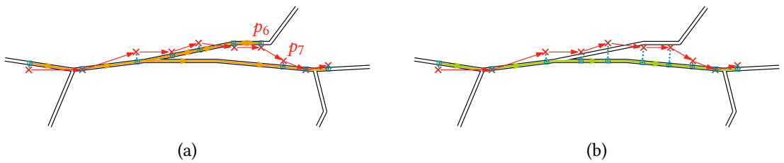
Figure 2.10: Map matching is demonstrated using the trajectory illustrated in Figure 2.8. Blue, dotted lines display the relation between the trajectory and matched points. (a) Naive approach by mapping each trajectory point to the closest road segment. The resulting path (shown in orange) in the network performs a detour deviating from the original movement. (b) An improved matching (shown in green) that closely resembles the original movement. Achieving such a solution requires advanced matching algorithms, such as the one presented in Chapter 4.
