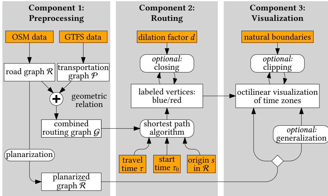
Figure 9.6: Illustration of workflow. The Preprocessing Component creates different graph structures used in the Routing Component and the Visualization Component. The Routing Component marks all reachable vertices blue and all unreachable vertices red. The Visualization Component creates a time zone for each travel time.
