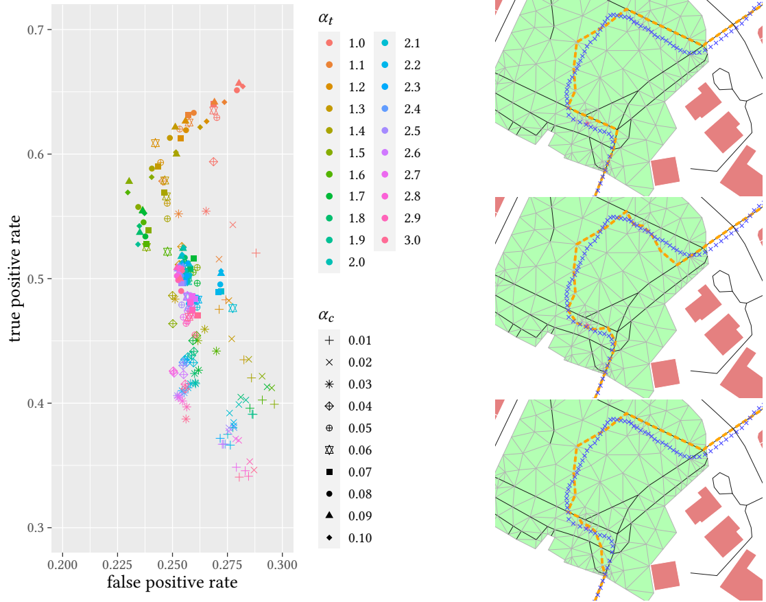
Figure 4.6: Left: Classification results for off-road section identification for different parameter configurations. Right: Effect of the parameter choice illustrated for an example instance. In the upper image ( \alpha_t = 1.5, \alpha_c = 0.01 ), the trajectory points (blue crosses) are matched to the cheap road network edges whenever possible. In the middle image ( \alpha_t = 1.5, \alpha_c = 0.10 ), the increased candidate cost leads to a matching which deviates from the measurements as little as possible. In the lower image ( \alpha_t = 1.1, \alpha_c = 0.01 ), the decreased tessellation edge cost leads to more deviation from the road network as in the upper image. Despite those differences, the middle part is matched to the same edges for all three configurations.
