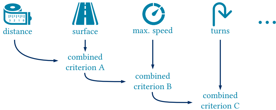
Figure 11.1: Iterative scheme to consider an arbitrary number of routing criteria. First, the balance factor for two initial criteria is learned and used to create a combined criterion. This combined criterion can iteratively be merged with additional criteria.
