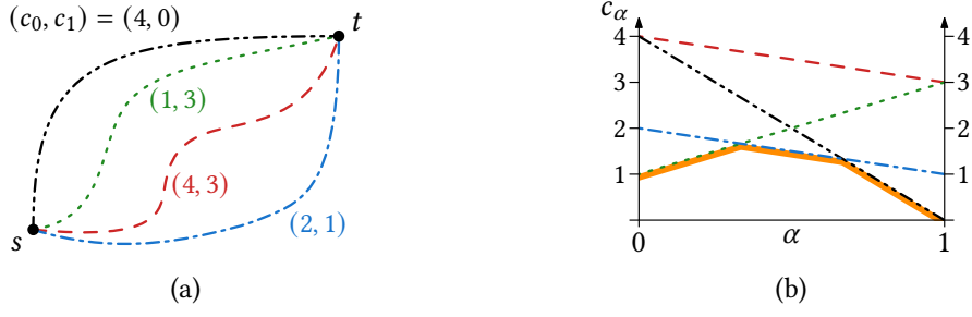
Figure 6.2: (a) A set of s - t paths with costs (c_0, c_1) and (b) the corresponding line arrangement; colors are chosen accordingly. In (b), the lower envelope \mathcal{E} is highlighted in orange.
