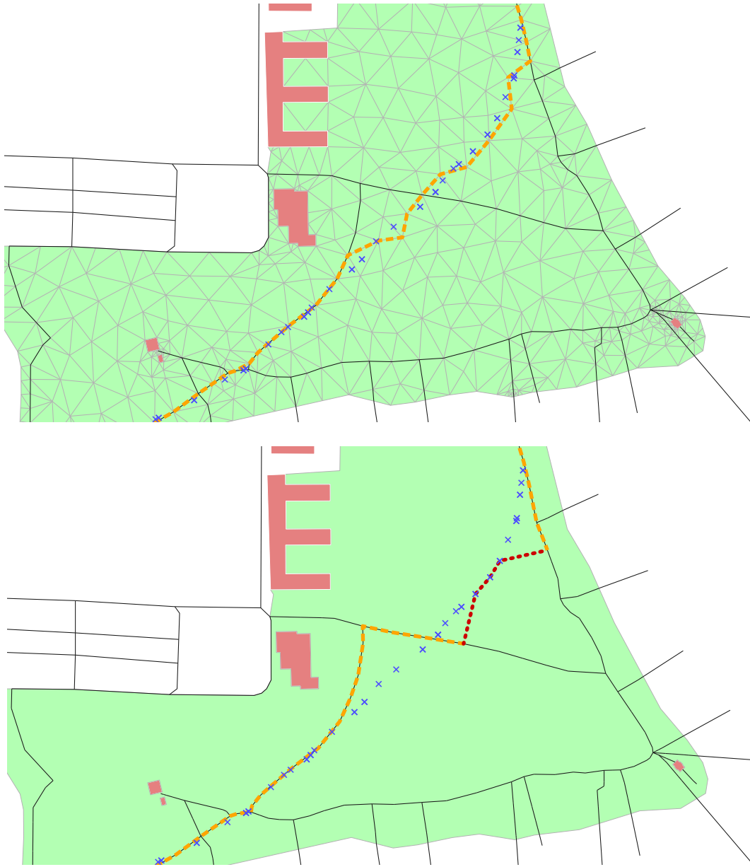
Figure 4.8: Original trajectory measurements (blue crosses) and matched paths produced by the tessellation-based approach (upper image) and Baseline+ (lower image). In tessellation-based matching, the shape of the original trajectory is faithfully preserved, and the unrestricted movement is correctly identified and matched to tessellation points and edges. Using Baseline+, the first part of the unrestricted movement is wrongfully matched to the path network, and subsequently, the shape is locally distorted when the switch from restricted to unrestricted movement occurs.
