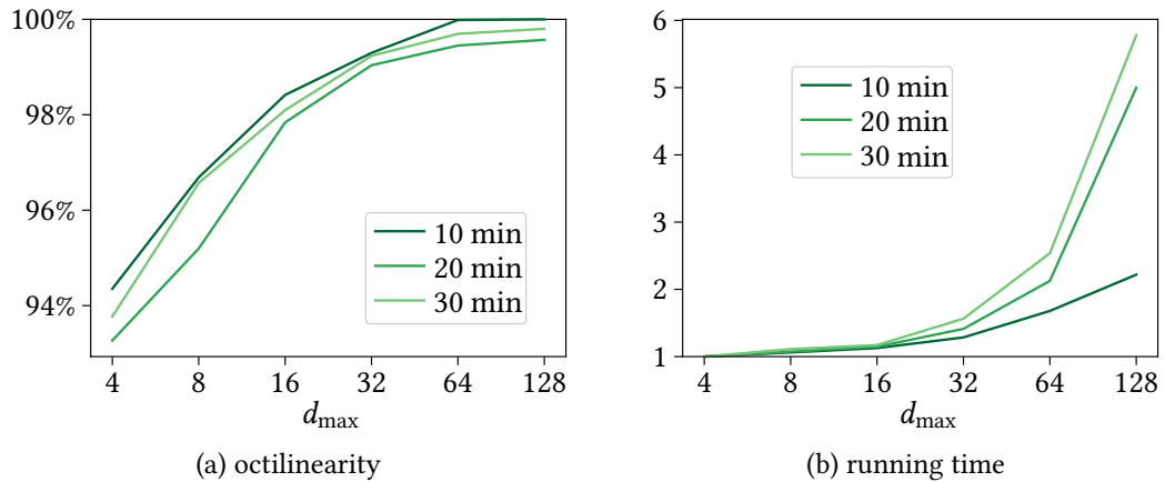
Figure 9.16: Evaluation of the maximum degree of refinement d_{\max} . (a) Share of the boundary's length that is visualized octilinearly. (b) Running time compared to the running time using the lowest d_{\max} .
