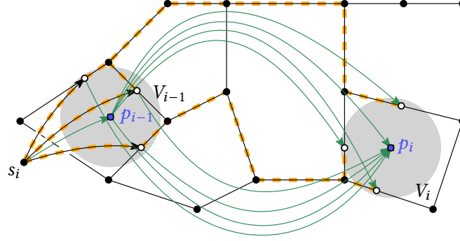
Figure 4.4: Extended graph to support unmatched segments. In addition to the candidates in the road network, every trajectory point is treated as a candidate itself. Additional edges (green) are introduced, connecting unmatched candidates (blue) to all candidates of the previous and next trajectory points.
