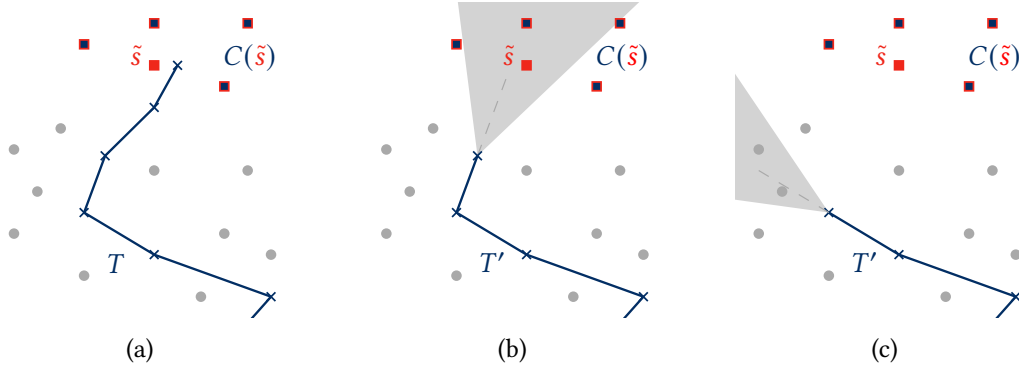
Figure 3.3: Schematic illustration of the geometric S-TT algorithm. (a) The original trajectory T leads to a destination site \tilde{s} , which has to be hidden among the sites in the protection set C(\tilde{s}) , depicted as squares. The S-TT algorithm suppresses the trajectory's endpoint iteratively until (b) the site closest to the endpoint is not part of the protection set C(\tilde{s}) and (c) a V-shaped region that is aligned with the last segment of the truncated trajectory T' contains either all or, as in the depicted case, none of the sites in C(\tilde{s}) .
