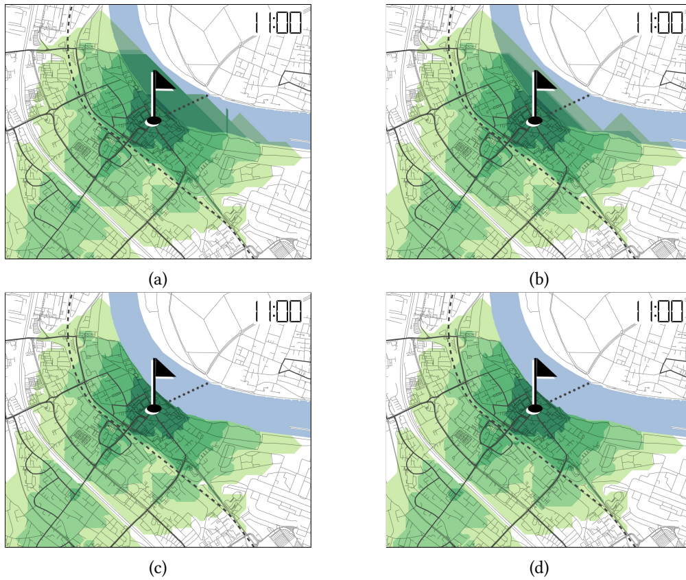
Figure 9.21: Case study. The travel-time map is created for four time zones with T = \{5, 10, 15, 20\} in minutes and start time Monday 11 a.m. (a) Independently generated time zones. (b) Time zones nested in the next bigger time zone. (c) Clipping to the river. (d) Result after applying the closing operation.
