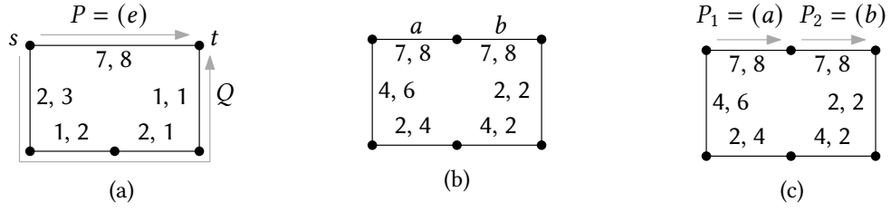
Figure 6.7: (a) A graph with a path P = (e) that does not admit a milestone segmentation and (b) the result of our method that ensures the feasibility of the problem. Comma-separated numbers represent c_0 and c_1 . (c) Milestone decomposition after applying our method. Path P is split into two subpaths, with the newly introduced vertex being the milestone.
