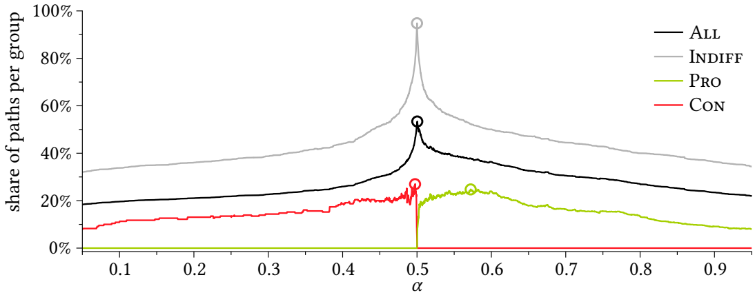
Figure 6.12: Share of paths per group that are optimal for the given \alpha . The maxima are marked with a circle and are achieved for \alpha \approx 0.4974 (CON, red), \alpha \approx 0.5721 (PRO, green), \alpha = \frac{1}{2} (INDIFF, gray), and \alpha = 0.5004 (all trajectories, black).
