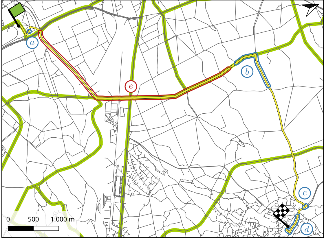
Figure 6.9: The user's path (yellow) has an optimal milestone segmentation with four milestones: a , b , c , and d (blue). Disregarding minor shiftings of a and/or b , this is a valid optimal segmentation for each \alpha \in [0.511, 0.607] (compare with Figure 6.10). The subpath (a, b) is \alpha -optimal for 0.511 \leq \alpha \leq 0.607 only. Therefore, for \alpha = 0.5 , i.e., the geodesic shortest path, an additional milestone e (red) is needed.
