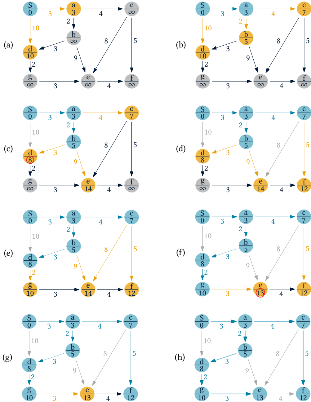
Figure 2.6: Dijkstra's algorithm starting at vertex S. Vertices in blue are settled, i.e. the shortest distance from S is already known. For vertices in orange, a path from S is found, but a shorter path might exist. Colored incoming edges represent the final (blue) or current best (orange) predecessor on the shortest path. The tentative distance to each vertex is displayed below it. (c) Settling vertex b reveals a shorter path to d, prompting an update in d's tentative distance and predecessor. (h) On completion, the predecessor edges form the shortest-path tree from S.
