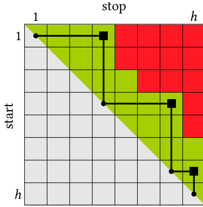
Figure 6.5: Depiction of a start-stop matrix of a path consisting of h = 8 vertices for a fixed \alpha \in [0, 1] . Green elements indicate that \alpha \notin \mathcal{M}[i, j] whereas red elements indicate the opposite. The black line represents a minimum path segmentation into three subpaths (v_1, v_4, v_7, v_8) resulting from a forward search.
