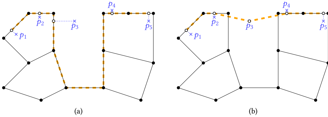
Figure 4.3: (a) Forcing the input trajectory (blue) to the network causes a detour in the output path (dashed). (b) Adding unmatched candidates and connecting segments prevents the detour.
