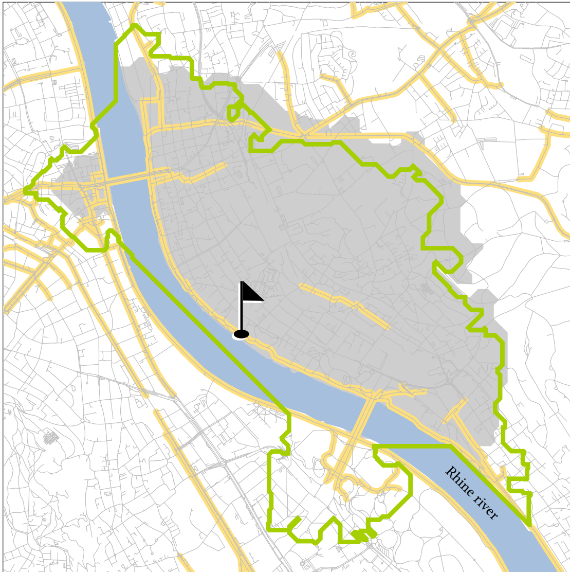
Figure 9.23: Visualizing different routing profiles. The gray area indicates the region accessible by a cyclist I of the group INDIFF ( \alpha = 0.5 ) covering a maximum distance of 3km from the specified starting point. In contrast, the green outline shows the reachable area for a cyclist P of the group Pro ( \alpha = 0.5721 ) with the same maximum effort and starting point. Notably, the dedicated cycle paths (yellow) running along the Rhine River extend P 's reach to exceed that of I along the river while the absence of cycle paths away from the river limits P 's reach in those directions.
