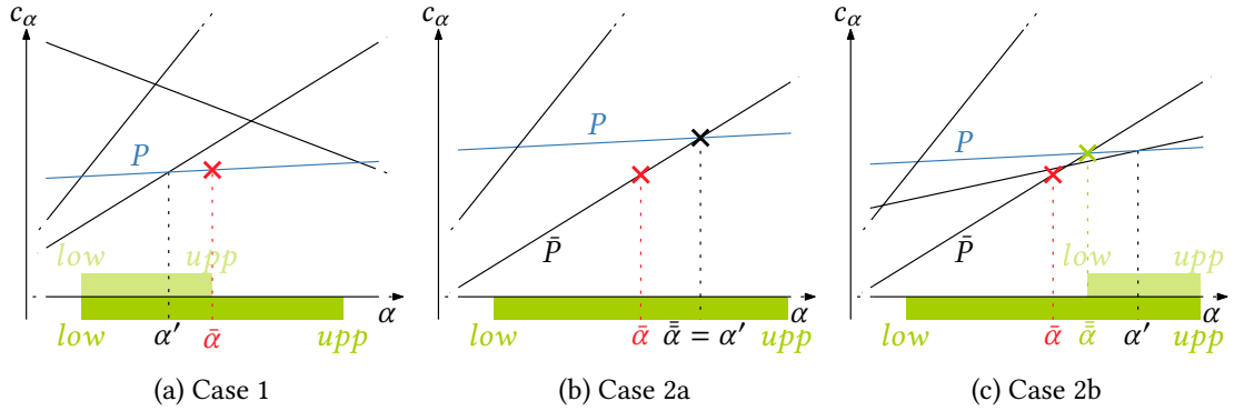
Figure 6.4: Search for the lower bound of the optimality range. The search interval is marked green (its current state is darker than the next). (a) If P is optimal with respect to c_{\bar{\alpha}} , the search for the lower bound continues in [low, \bar{\alpha}] . (b) If P is optimal with respect to c_{\bar{\alpha}} , the lower bound of the optimality range is found, and the algorithm terminates. (c) At \bar{\alpha} , the path P is dominated by \bar{P} . The search continues in [\bar{\alpha}, upp] where \bar{\alpha} marks the intersection of P and \bar{P} .
