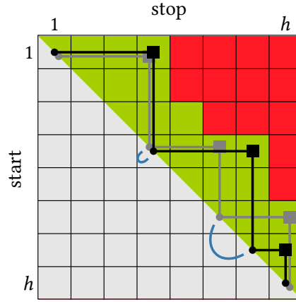
Figure 6.6: In addition to the segmentation of the forward search (black, see also Figure 6.5), the segmentation when searching backward (gray) is displayed. The blue lines indicate the milestone suites. Note that the first milestone suite degenerated into a single vertex.
