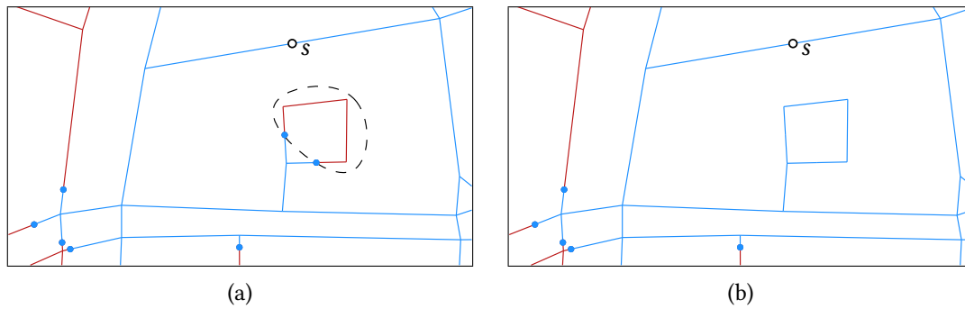
Figure 9.14: Closing operation. (a) A small group of unreachable (red) vertices in the blue area. (b) After the closing operation the hole is filled.
