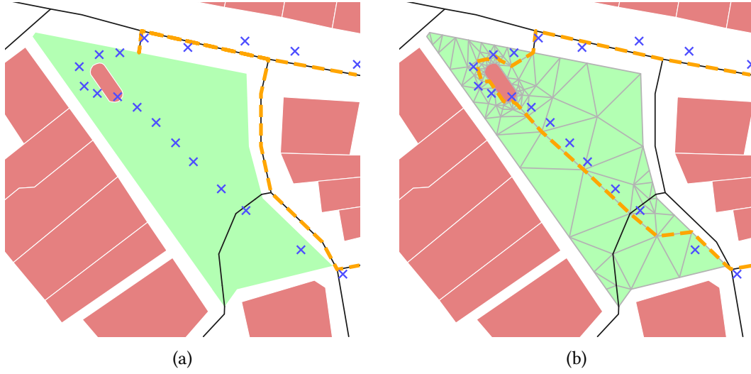
Figure 4.5: (a) Roads in the network data. Movement on the open space (green) cannot be matched appropriately (dashed). (b) Extended road network. Open spaces are tessellated in order to add appropriate off-road candidates. Note that the green polygon has a hole that remains untessellated since it is not open space. Also, note that additional vertices are added to prevent skinny triangles.
