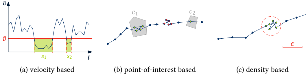
Figure 3.1: Sketches of different stay-point-detection approaches. (a) In velocity-based approaches, trajectory points with velocities lower than a specified threshold are identified as stops. Slow movement, such as during s_2 , may lead to false positives. (b) In point-of-interest-based approaches, stop candidates are modeled. Some stops, like the ones marked red, may not be identified if no candidate is present. (c) In density-based approaches, stops are detected where the trajectory remains within an area of extent \epsilon for a predefined minimum duration.
