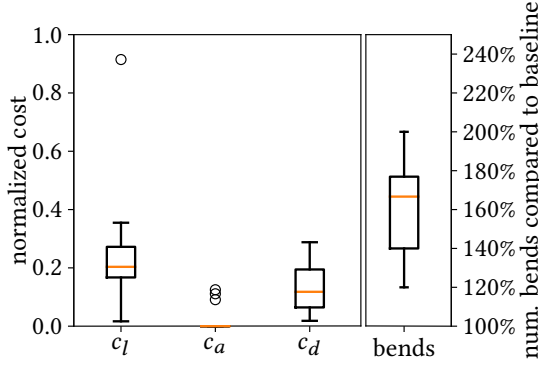
Figure 10.12: Quality for the individual cost functions using c_b^u with \rho_b = 10 , \rho_l = 50 , \rho_a = 14 , and \rho_d = 1 .
