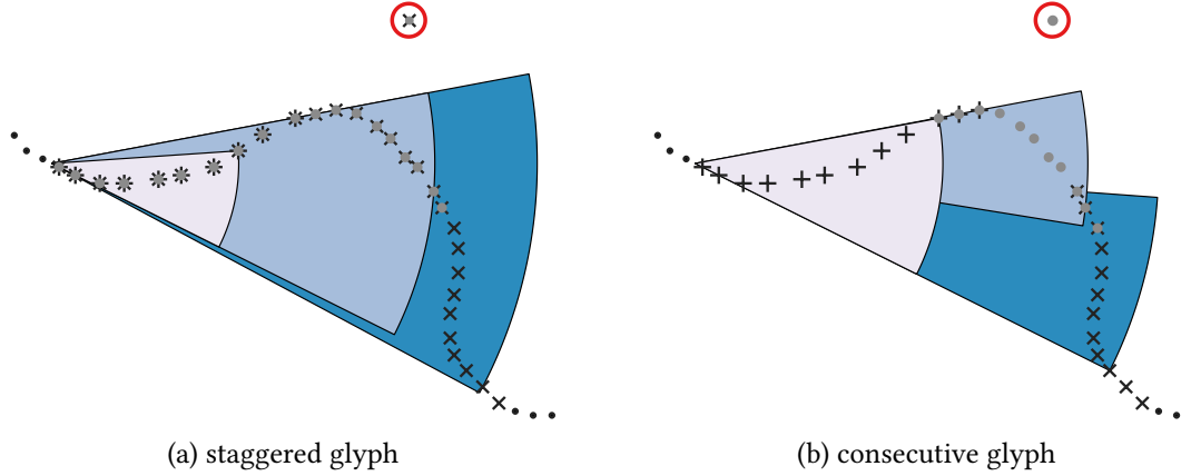
Figure 8.4: Considered vertices of the first disk sector (black plus), the second disk sector (gray dots), and the third disk sector (black cross) for the advanced glyphs. Not all vertices need to be covered by the disk sectors, so the outlier (marked red) is not included in the glyphs.
