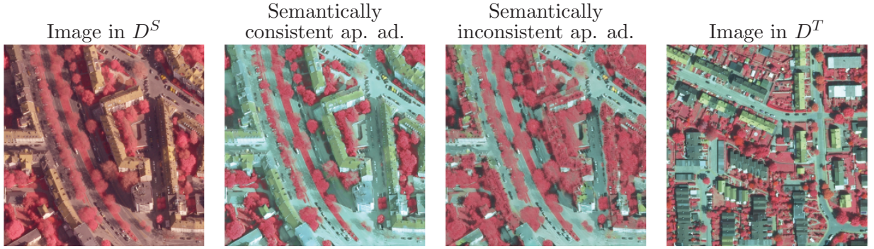
Figure 1.1: Example of semantically consistent and inconsistent appearance adaptation (ap. ad.). The right image serves as an example for appearance of objects in D^T . In the semantically inconsistent adaptation, after adaptation the buildings look like trees in D^T . After applying the appearance adaptation in a semantically consistent way, the buildings look like buildings in D^T .
