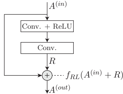
Figure 2.5: Illustration of a residual block in a ResNet CNN architecture. Conv.: Convolutional layer. ReLU, f_{RL} : Rectified linear unit (cf. Section 2.3.4).
