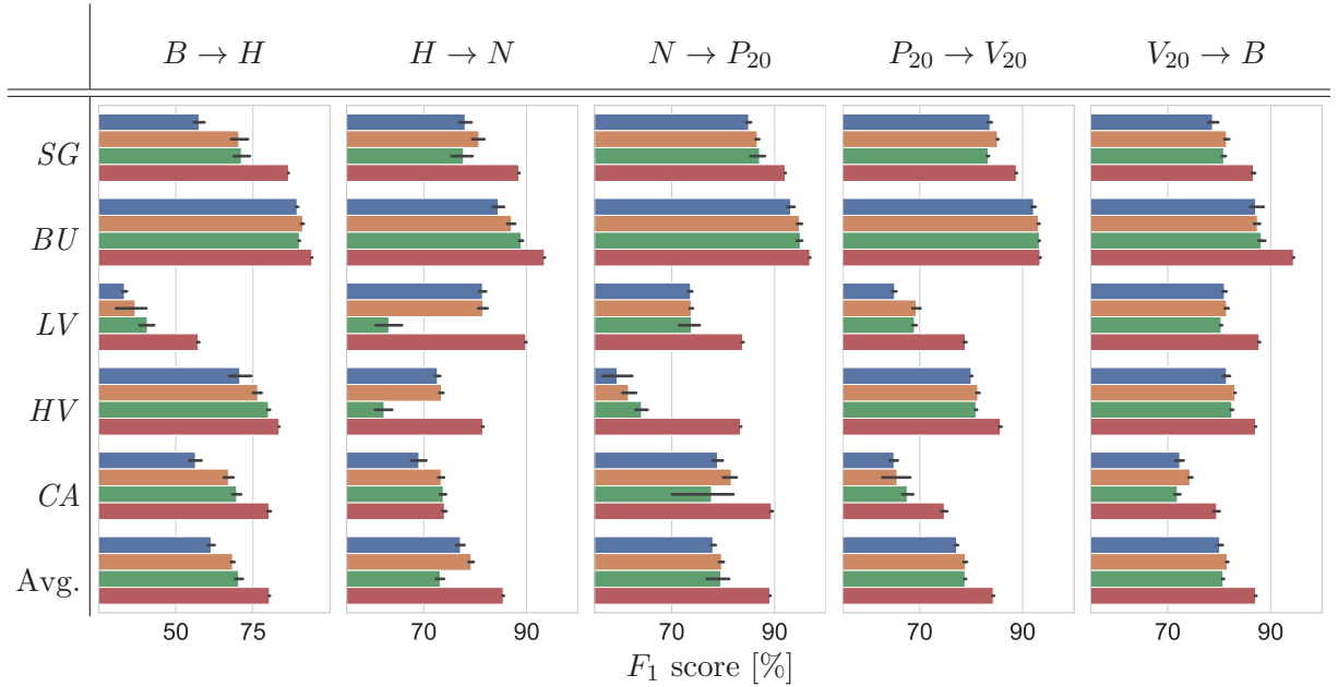
Figure 6.7: Class-wise F_1 scores and \bar{F}_1 score for different adaptation scenarios. The blue bars correspond to the classifiers trained in D^S and the red bars to the classifiers trained in D^T . The orange bars correspond to the classifiers that were trained in D^S and adapted to D^T using the proposed method for UDA in variant V_{RD} . The green bars correspond to the classifiers that were adapted using variant V_{RD,ABN} . Note that the scaling of the horizontal axis is different for the first adaptation setting. The black bars indicate the standard deviation based on five repetitions of the experiment. In particular, the length of the bars corresponds to twice the standard deviation. Class abbreviations as in Table 5.1.
