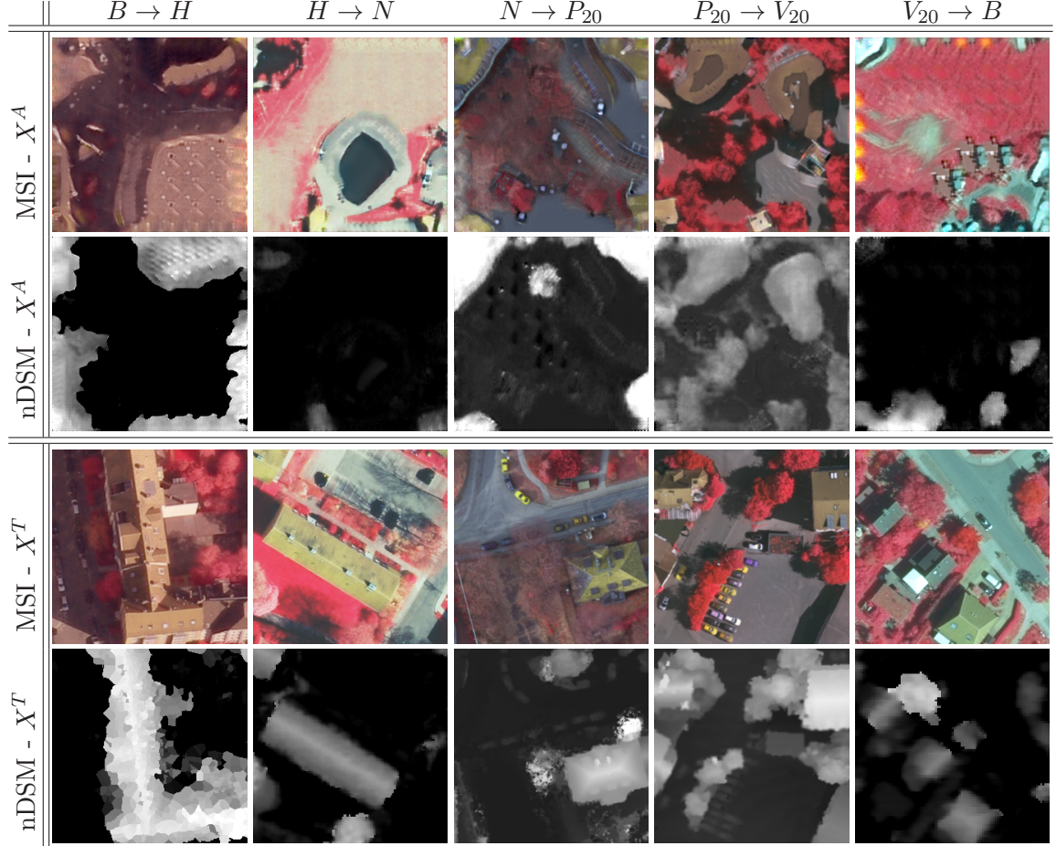
Figure 6.4: Examples for auxiliary images X^A (rows 1, 2) generated by the auxiliary generator G in different adaptation scenarios in variant V_{AG} and exemplary images from X^T (rows 3, 4). The image size is 256 \times 256 px . Rows 1 and 3 show the infrared red and green channels as false colour images, and rows 2 and 4 show visualisations of the nDSMs.
