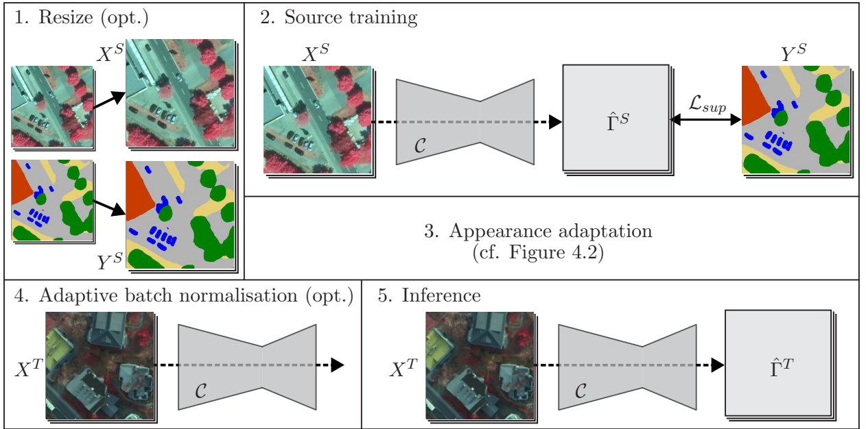
Figure 4.1: Overview of the processing steps of the proposed method. X^S and Y^S denote the images and reference label maps in the source domain and X^T are the images in the target domain. In the first step, the data from D^S are pre-scaled to match the resolution from D^T . Then, in the source training, the classifier \mathcal{C} predicts the maps of probabilistic class scores \hat{\Gamma}^S for X^S and the supervised loss \mathcal{L}_{sup} is minimised. After the two steps for domain adaptation, the classifier \mathcal{C} is used to predict the maps of probabilistic class scores \hat{\Gamma}^T for X^T based on which the final class predictions are computed. opt.: optional processing step.
