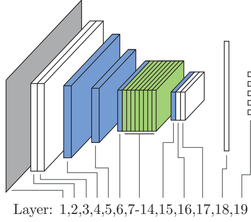
Figure 2.7: Illustration of the Xception architecture. The layer numbers correspond to the numbers in Table 2.3. Blue and green layers correspond to Xception blocks of type A and B, respectively. White layers correspond to regular convolutional layers.
