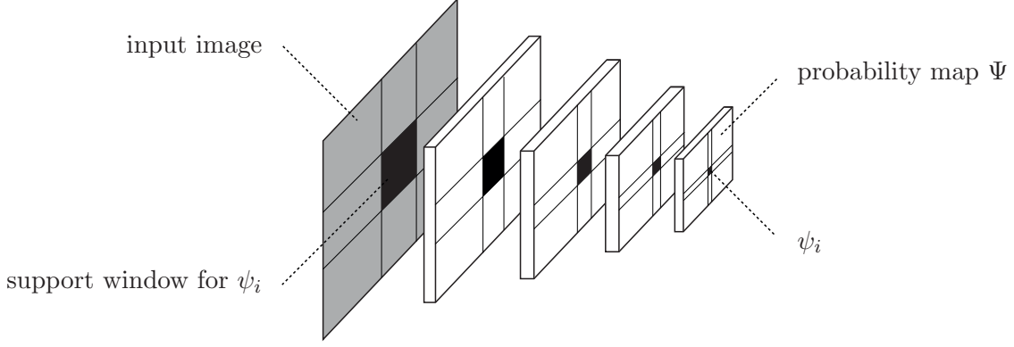
Figure 2.10: Illustration of the PatchGAN discriminator (Isola et al., 2017) for adversarial appearance adaptation. The core idea is to predict a map of probabilistic class scores \Psi by feeding the input image through a sequence of convolutions. Each value \psi_i \in \Psi corresponds to the probability of the corresponding support window to come from a specific domain.
