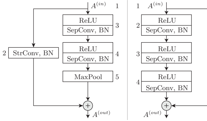
Figure 2.6: Illustration of the Xception blocks of type A (left) and B (right). The numbers next to the boxes are the layer indices used in Tables 2.1 and 2.2. StrConv: Strided convolution with step size of 2; SepConv: Depthwise separable convolution; BN: 2D batch normalisation. MaxPool: Max pooling with a stride of 2. ReLU: Rectified linear unit.
