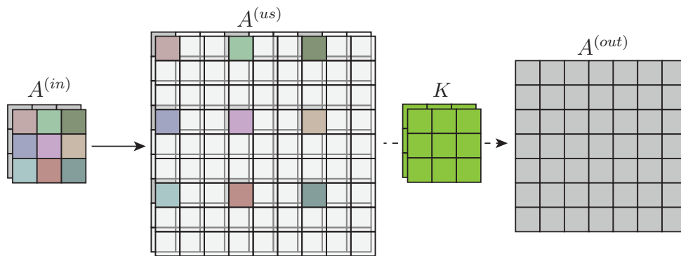
Figure 2.8: Schematic illustration of a transposed convolutional layer. The input activation map A^{(in)} with two channels is upsampled by appending s_h = 2 rows filled with zeros to every row and appending s_w = 2 columns filled with zeros to every column. The output activation map A^{(us)} then serves as input to a regular convolution, in the example using a single kernel K . Note that identical colours in A^{(in)} and A^{(up)} indicate that the corresponding value is copied from A^{(in)} to A^{(up)} .
