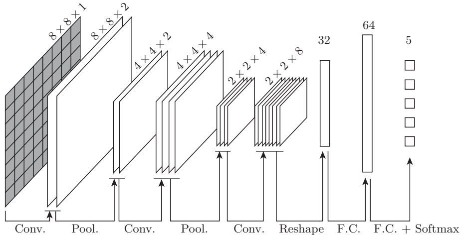
Figure 2.2: Exemplary CNN architecture for multi-class image categorisation. The network maps a single-channel image of size 8 \times 8 \times 1 to a probability distribution according to a class structure with n_L = 5 classes. The image is first processed by a sequence of convolutional (Conv.) and pooling (Pool.) layers (cf. Sections 2.3.1 and 2.3.2). The activation map produced by the last convolutional layer is reshaped, i.e. the values are rearranged in a one-dimensional array, and processed by two fully connected (F.C.) layers that correspond to a simple MLP. The output of the second fully connected layer is normalised by the softmax function to obtain the class probabilities. At the top of each tensor in the figure, the respective shape is given. In particular, for three-dimensional tensors the shape is given in the form of height \times width \times depth and for one-dimensional vectors only the number of entries is given.
