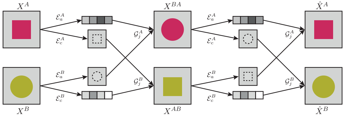
Figure 2.11: Illustration of image adaptation based on cross cycle consistency. The goal is to learn to disentangle appearance and content for images from two domains and to predict images with specific content and appearance. The actual image adaptation is performed by predicting an image that has the content of an image from one domain and the appearance of an image from the other domain, e.g. the image X^{BA} has the content of X^B but the style from X^A . If this process is performed twice for an image pair X^A, X^B , the outputs \hat{X}^A, \hat{X}^B should be similar to the original images. Note that in the example, the appearance refers to the colour and the content to the shape of the depicted object.
