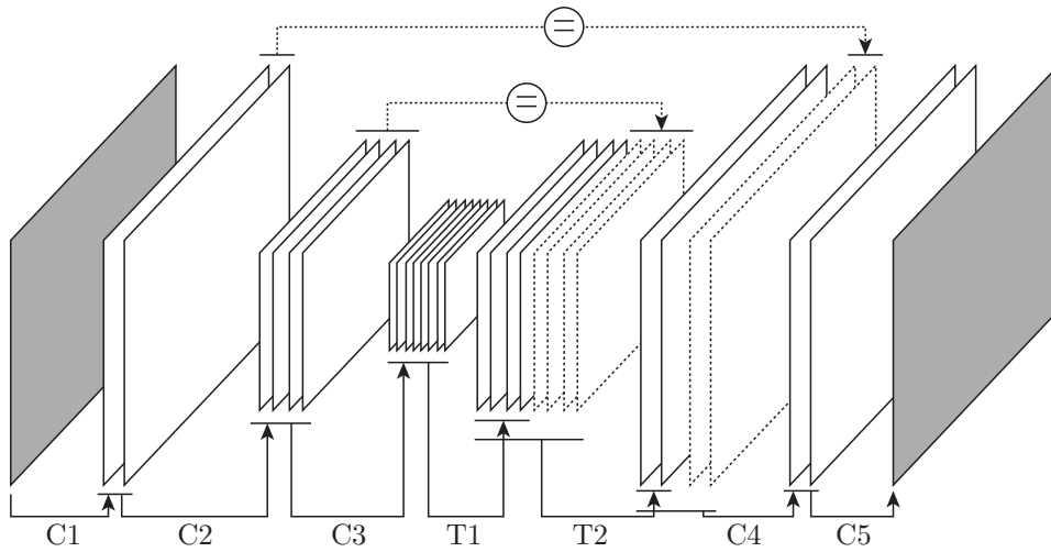
Figure 2.9: Illustration of an encoder-decoder FCN with skip connections. The solid arrows indicate the processing by convolutional layers (C1-C5) and transposed convolutional layers (T1, T2). The skip connections are represented by dotted arrows. The activation maps with a dotted outline are obtained by copying the respective activation maps from the encoder.
