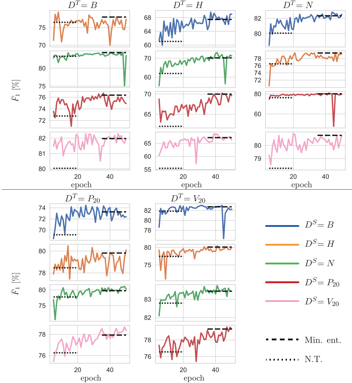
Figure 6.9: Evaluation of the stopping criterion. Coloured lines correspond to the performance of the classifier in D^T in the UDA process as a function of the training epoch. Broken black lines correspond to the performance if the entropy based stopping criterion is applied (Min. ent.), and the dotted black lines indicate the performance of naïve transfer (N.T.).
