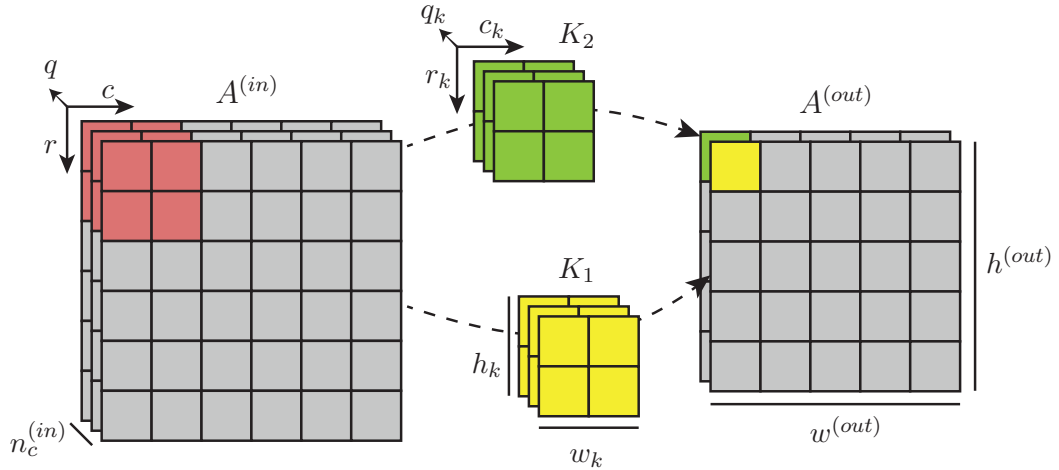
Figure 2.3: Schematic illustration of a convolutional layer with two kernels. The input activation map A^{(in)} has n_c^{(in)} = 3 channels, the output activation map A^{(out)} has n_c^{(out)} = 2 channels. Each kernel has a spatial size of h_k \times w_k with h_k = w_k = 2px .
