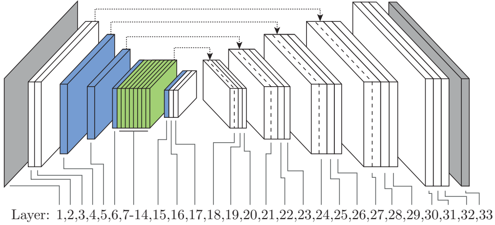
Figure 4.3: Illustration of the Xception U-Net architecture. The layer numbers correspond to those in Table 2.3. Blue and green layers correspond to Xception blocks of type A and B, respectively. The dotted lines represent skip connections.
