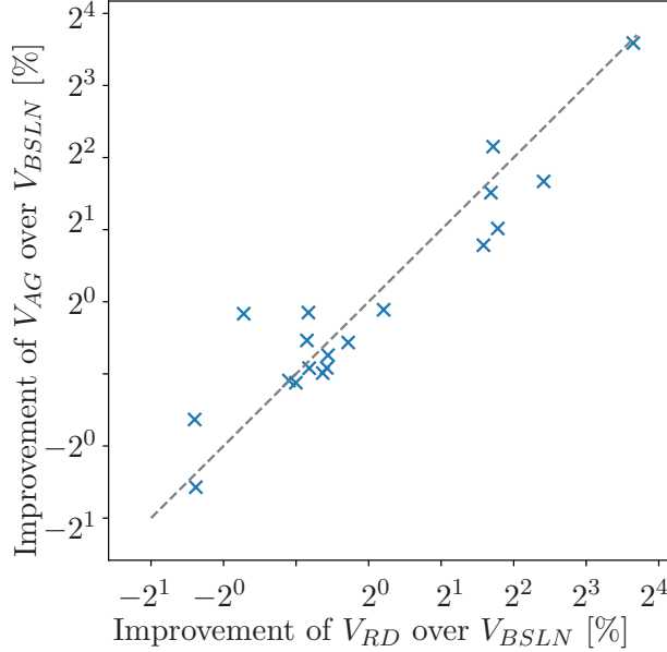
Figure 6.5: Comparison of the improvement of the classification performance of V_{AG} and V_{RD} to the baseline V_{BSLN} with respect to \bar{F}_1 .
