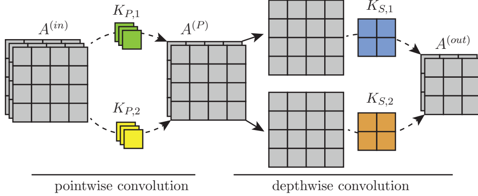
Figure 2.4: Schematic illustration of a depthwise separable convolutional layer. The pointwise convolution with two kernels produces the intermediate output A^{(P)} . Each channel in A^{(P)} is then convolved individually using a kernel in the depthwise convolution step. The dotted arrows in the figure correspond to a convolution and the regular arrows are used to indicate the splitting of the channels of A^{(P)} .
