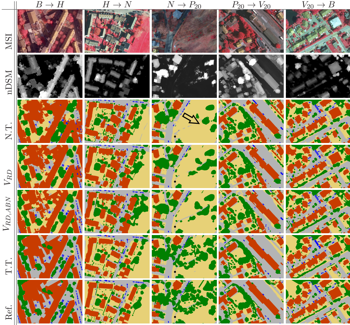
Figure 6.6: Exemplary image patches and predictions for five adaptation scenarios using classifiers that were trained using different variants. The first row shows the MSI data for the image patch and the second row shows the nDSM. N.T.: Naïve transfer (classifier was trained only in D^S ). V_{RD} : First variant of the proposed method (classifier trained in D^S and adapted to D^T using the variant V_{RD} ). V_{RD,ABN} : Second variant of the proposed method (classifier trained in D^S and adapted to D^T using the variant V_{RD,ABN} ). T.T.: Target training (classifier was trained only in D^T ). Ref.: Reference label map.
