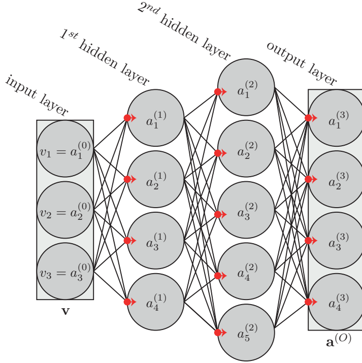
Figure 2.1: Schematic illustration of a multi-layer perceptron M with n_{HL} = 2 hidden layers designed to map a feature vector with three elements to a vector with four elements. The red dots indicate the computation of the output of each neuron according to Equation 2.5. It shall be noted that this architecture serves as an example for a very shallow DNN. Common architectures have a much higher number of layers and much more neurons per layer, and consequently they have a much higher number of parameters.
