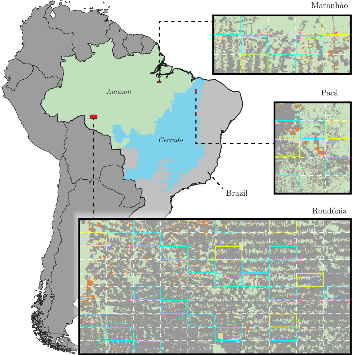
Figure 5.4: Test sites for deforestation detection; the figure shows the locations of the three test sites and an overview of the rasterized reference data. Colour code for the reference: no deforestation (green), past deforestation (grey), deforestation (orange). The broken lines show outlines of the tiles that were created to split the images into the subsets for training, validation and testing. Colour-code for tiling: Training (cyan), validation (yellow), testing (no colour).
