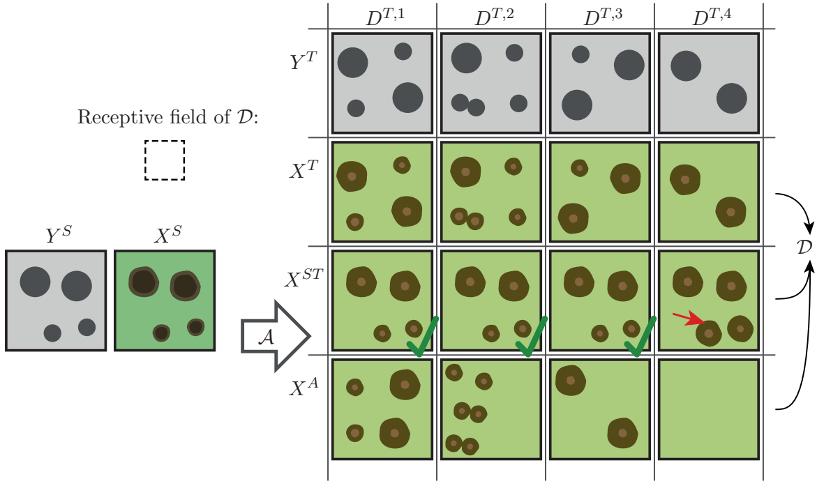
Figure 4.6: Toy example to illustrate how auxiliary images X^A help the appearance adaptation to achieve semantic consistency. An image X^S is adapted to multiple target domains D^{T,1} - D^{T,4} , each associated with a target image X^T and an underlying label map Y^T . Y^S denotes the underlying label map of X^S and X^{ST} is the output to be expected for the appearance adaptation network \mathcal{A} for the different target domains. Colour-codes as in the description of Figure 4.5.
