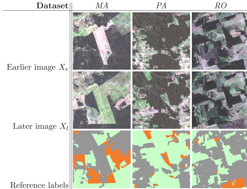
Figure 5.3: Exemplary samples from datasets for deforestation detection; the side length of the patches is 224px ( 6720m ). Note that only the red, green and blue channels are visualised. Colour-codes of the reference: Unknown (grey), deforestation (orange), no deforestation (green)
