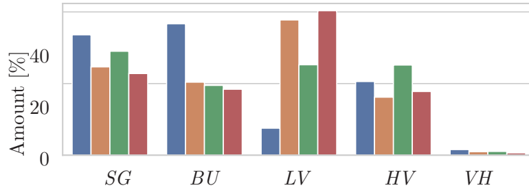
Figure 6.8: Global label distributions for the scenario H \rightarrow N . The blue bars show the label distribution in H and the red bars correspond to the one in N . The orange and green bars correspond to the label distribution in the predictions using the variants V_{RD} and V_{RD,ABN} , respectively, for the test set from N .
