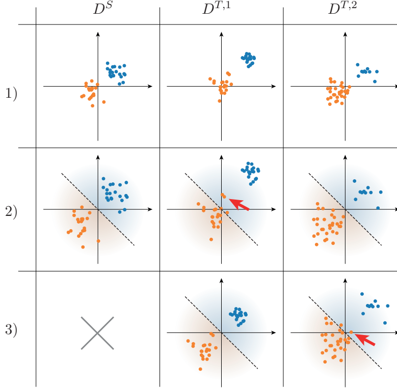
Figure 2.12: Toy example illustrating the working principle of adaptive batch normalisation. 1) 2D data points from the domain according to the column. 2) Data normalised using the means and standard deviations from D^S . 3) Data normalised using means and standard deviations from D^T . The broken line illustrates the decision boundary learned in D^S . The colour of the dots illustrates the true class. Red arrows point to misclassified samples.
