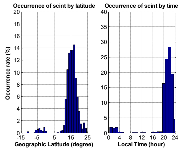
d2. The occurrence of scintillation on 31 st
