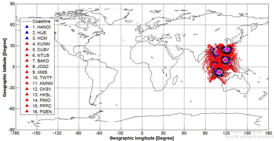
Figure 3.4b. Satellite traces of 16 GNSS stations over the research area (Different color refers to different satellite elevation: red: <20°, black: [20°,30°], blue: [30°,40°], yellow: [40°,50°], magenta: >50°)
