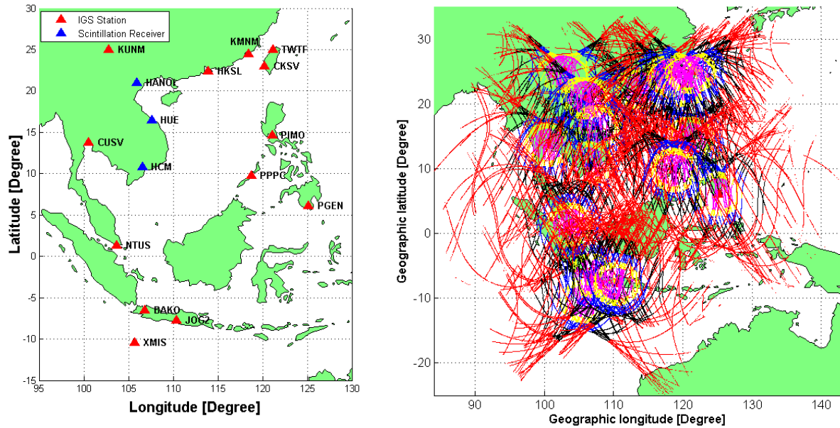
Figure 3.4a. Distribution (left) and satellite traces (right) of 16 GNSS stations over the research area (Different color refers to different satellite elevation: red: <20°, black: [20°,30°], blue: [30°,40°], yellow: [40°,50°], magenta: >50°)
