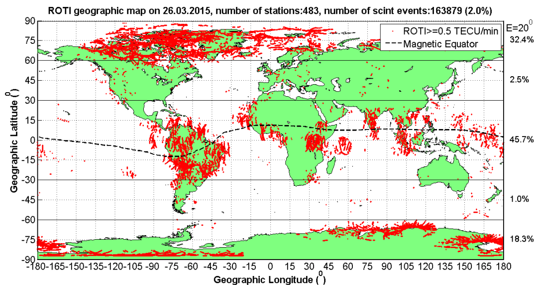
Figure 5.8a. Spatial distribution of global ionospheric irregularities (refers to as of Fig. 1.2) (only \text{ROTI} \geq 0.5 TECU/min are displayed)
