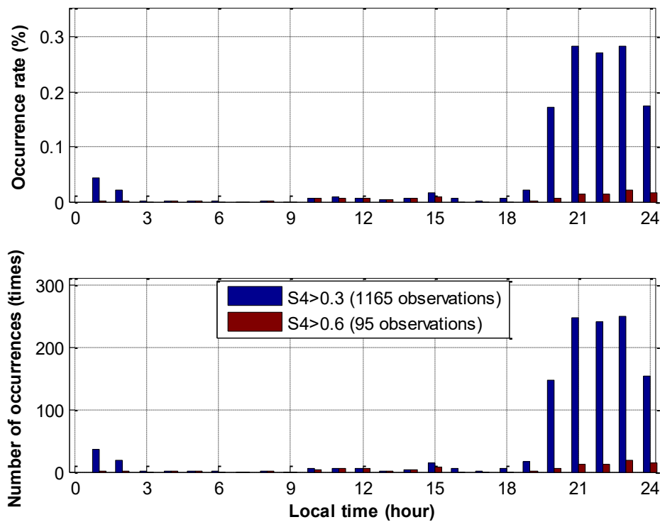
Figure 4.6c. Local time frequency of scintillation events appearance at HCM in 2015
