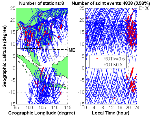
c1. Regional ROTI map on 26 th
