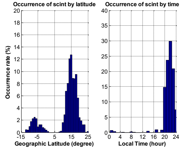
c2. The occurrence of scintillation on 26 th
