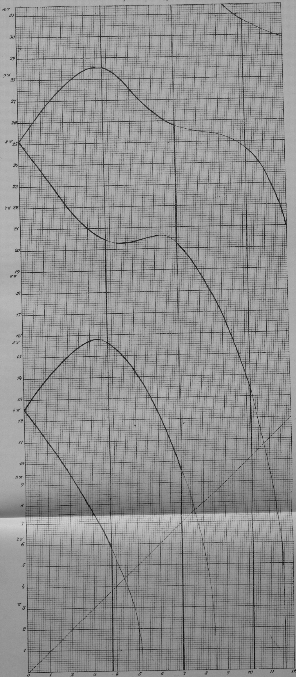
Fig. 12. J_1 = 0 ; U_2 = 0 .
