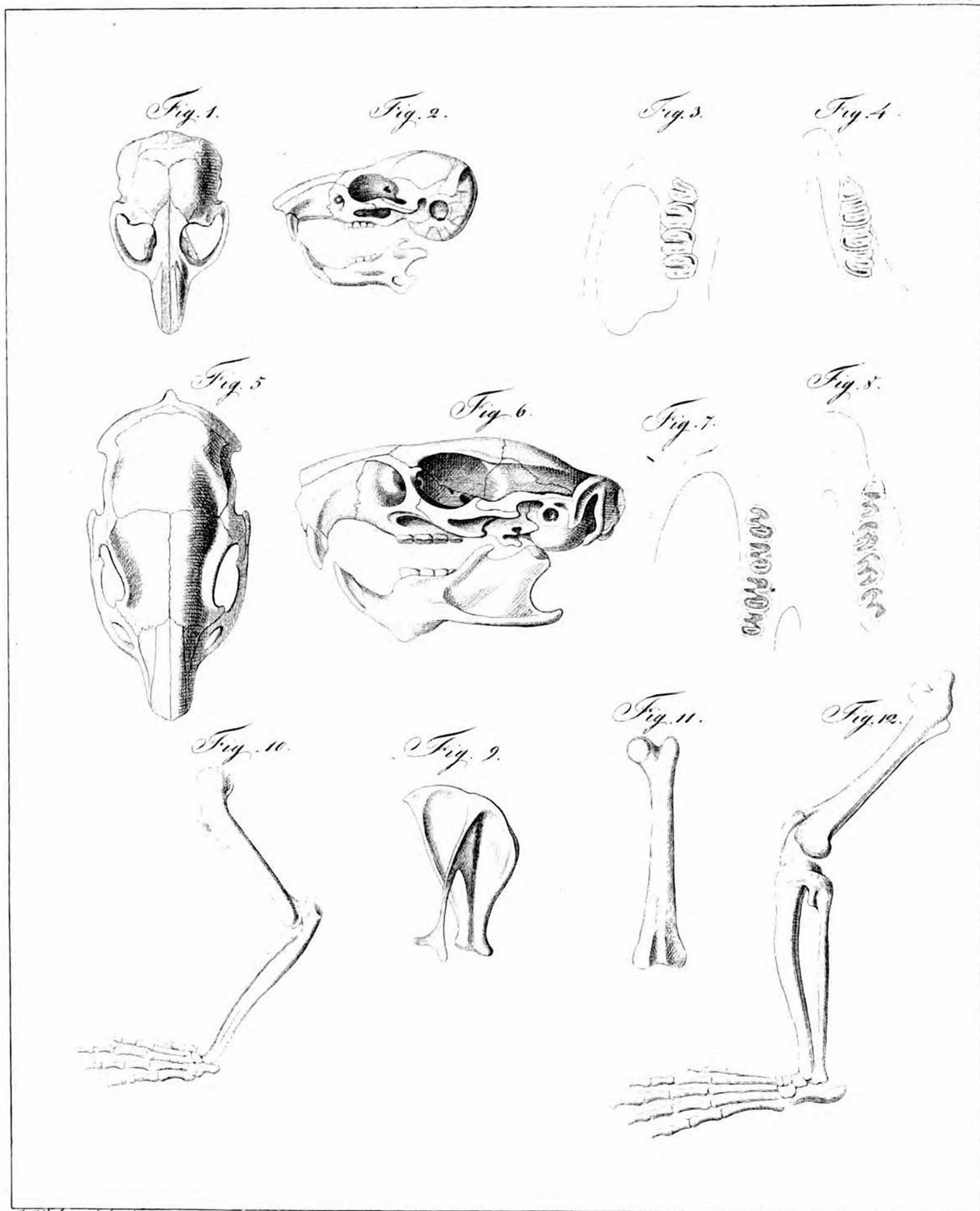
Fig. 1-4. Myotis / Elicmys / melanurus. Fig. 5-12. L. obscura. Althaus V. der mathem. phys. Klasse Bd. III. 24 Dr. Wagner's Vign.
